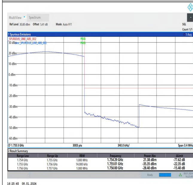
Band4_1.4MHz_QPSK_20393_6RB#0
