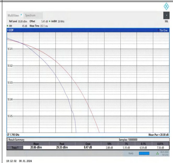
Band4-20MHz-16QAM-20300-100RB#0-PASS
