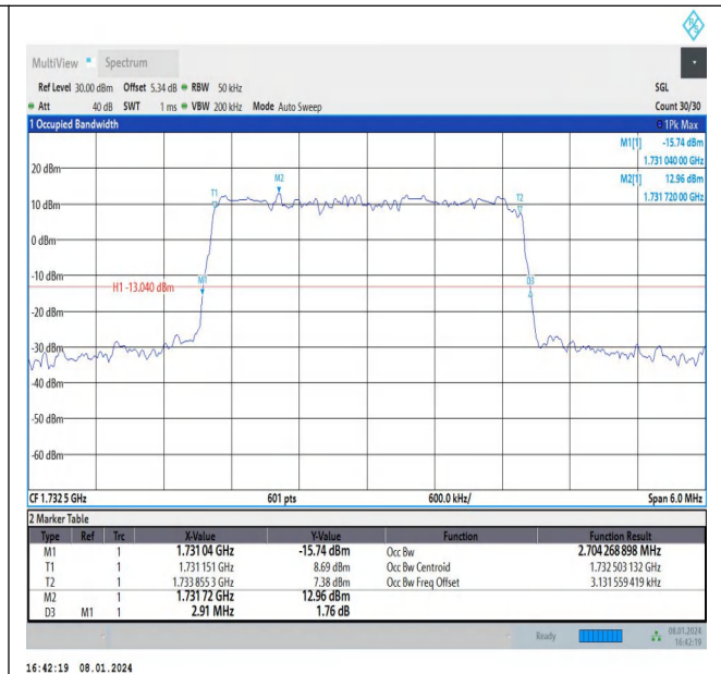
Band4-3MHz-16QAM-20175-15RB#0-PASS
