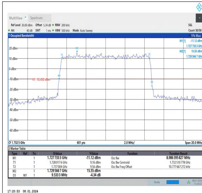
Band4-10MHz-QPSK-20175-50RB#0-PASS
