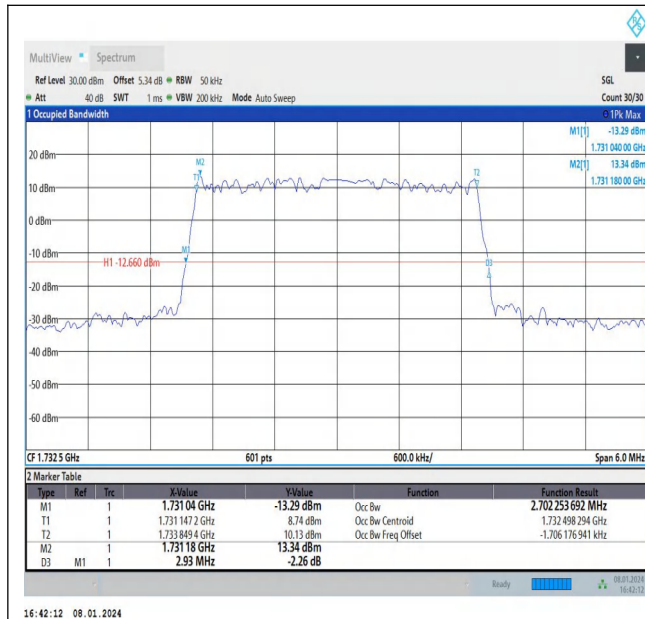
Band4-3MHz-QPSK-20175-15RB#0-PASS
