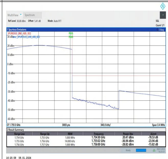
Band4_1.4MHz_16QAM_20393_6RB#0
