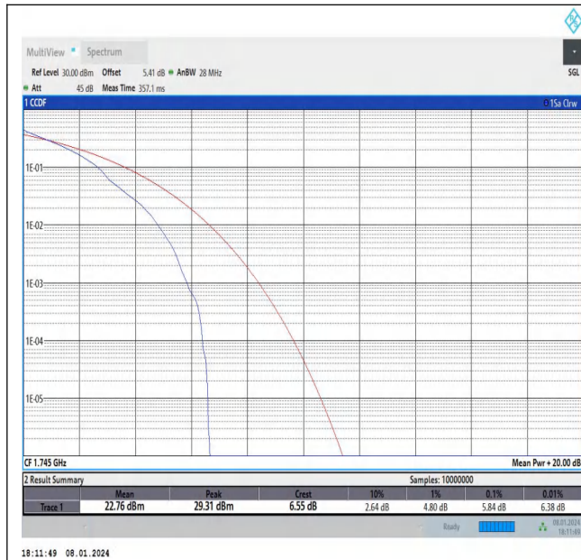
Band4-20MHz-QPSK-20300-1RB#0-PASS
