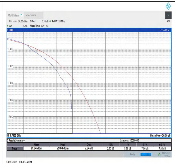
Band4-20MHz-16QAM-20175-1RB#0-PASS
