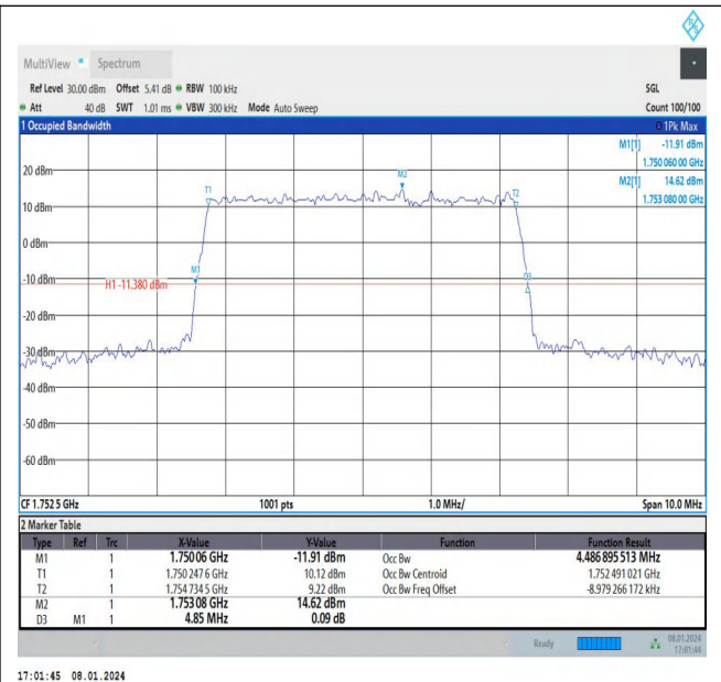
Band4-5MHz-16QAM-20375-25RB#0-PASS
