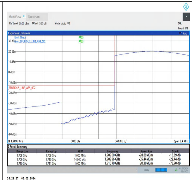
Band4_1.4MHz_16QAM_19957_6RB#0
