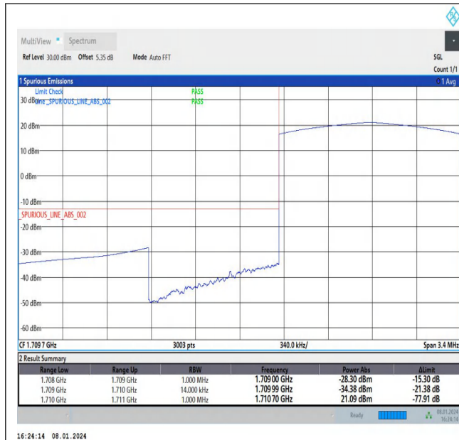
Band4_1.4MHz_QPSK_19957_6RB#0
