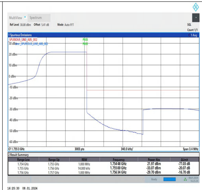
Band4_1.4MHz_16QAM_20393_1RB#5
