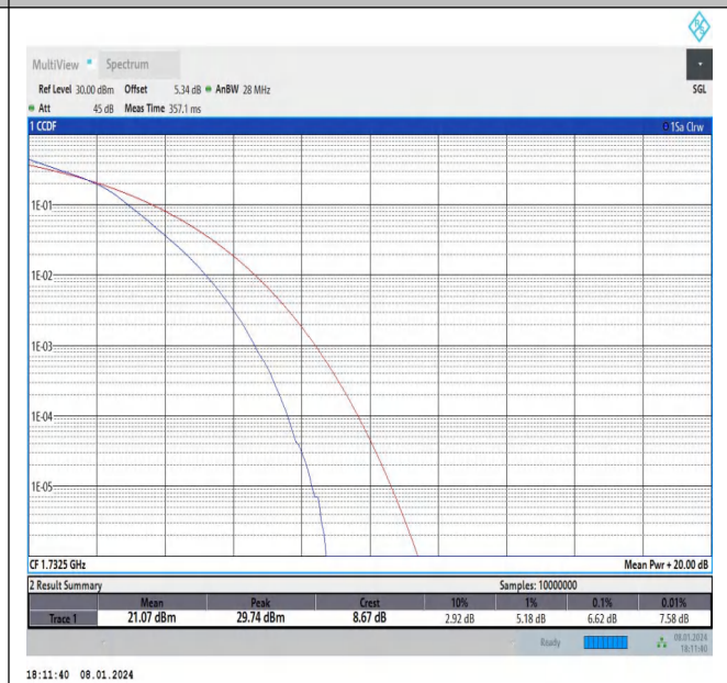
Band4-20MHz-16QAM-20175-100RB#0-PASS
