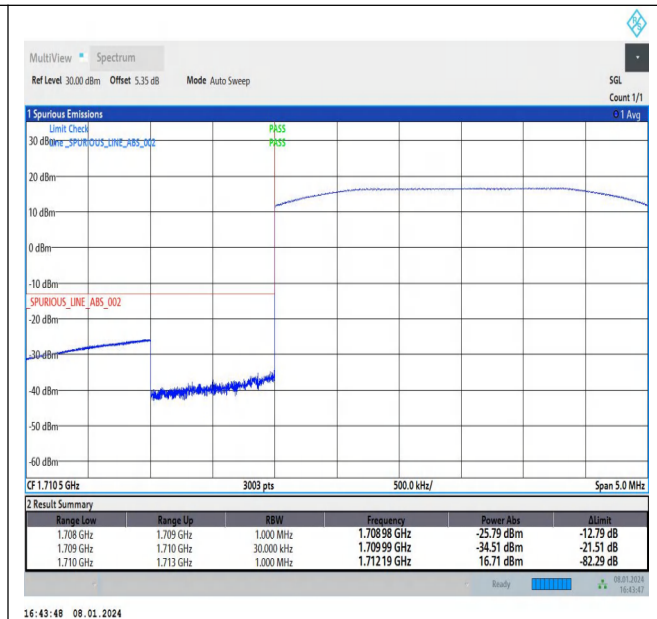
Band4_3MHz_16QAM_19965_15RB#0
