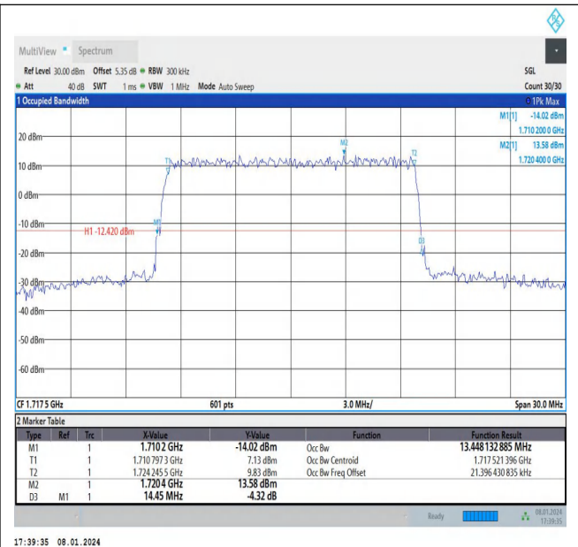
Band4-15MHz-16QAM-20025-75RB#0-PASS
