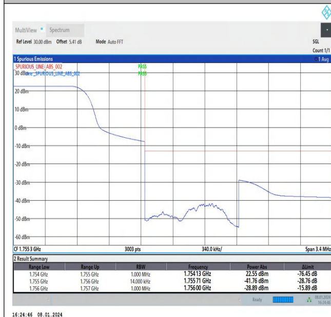
Band4_1.4MHz_QPSK_20393_1RB#0
