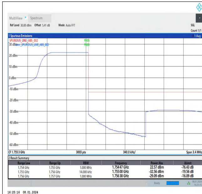
Band4_1.4MHz_QPSK_20393_1RB#5
