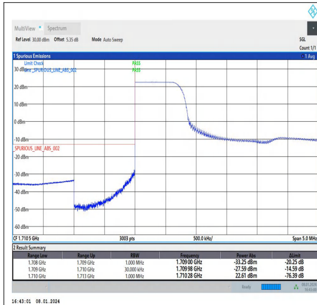
Band4_3MHz_QPSK_19965_1RB#0
