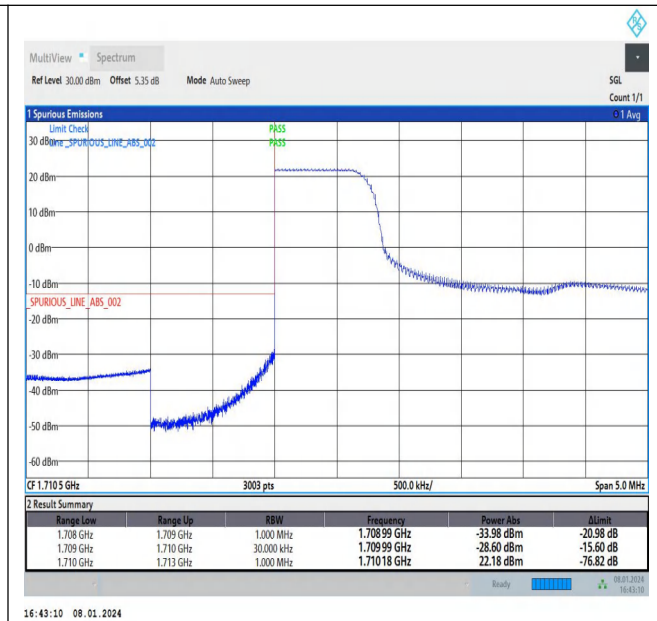
Band4_3MHz_16QAM_19965_1RB#0
