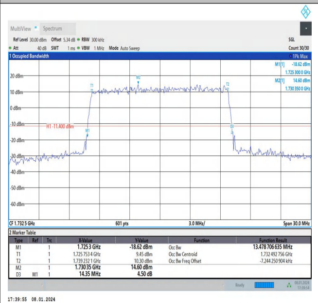
Band4-15MHz-16QAM-20175-75RB#0-PASS
