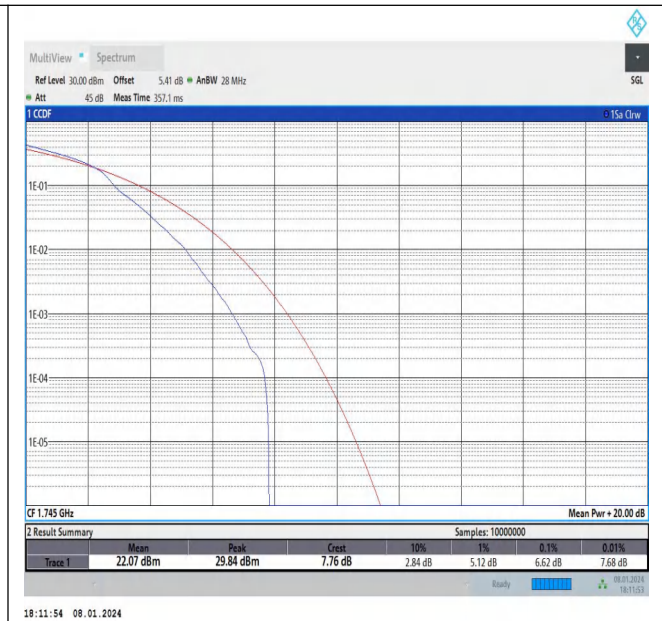
Band4-20MHz-16QAM-20300-1RB#0-PASS
