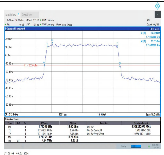
Band4-5MHz-16QAM-19975-25RB#0-PASS
