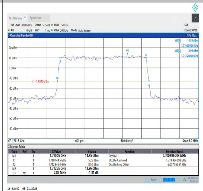
Band4-3MHz-16QAM-19965-15RB#0-PASS
