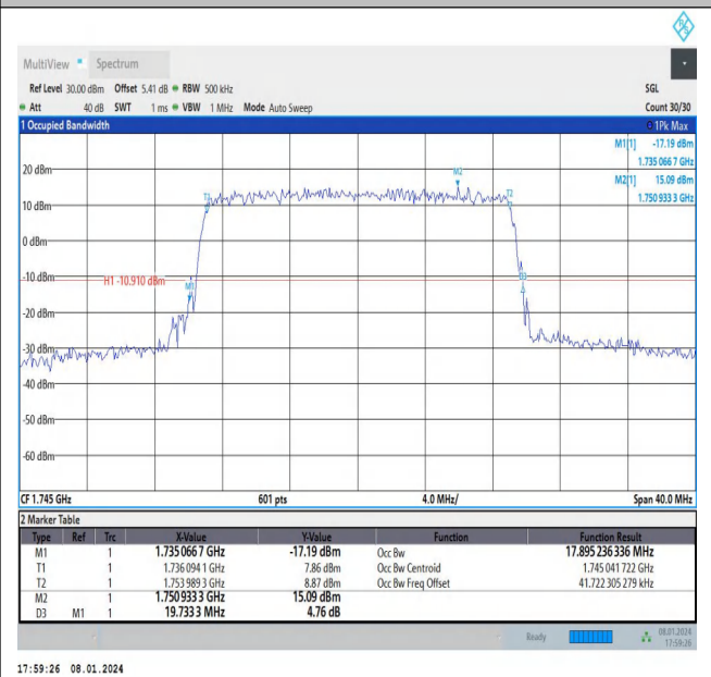
Band4-20MHz-16QAM-20300-100RB#0-PASS
