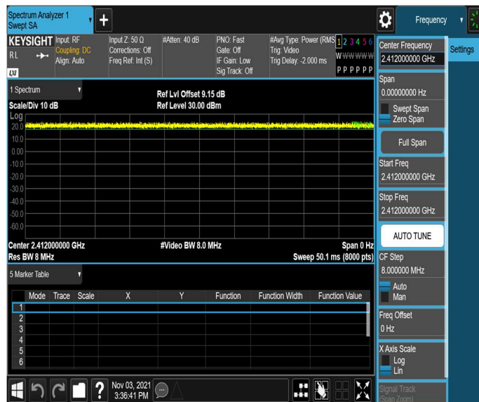
11N20SISO_Ant1_2412
