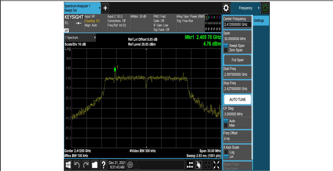
11G_Ant1_2412_0~Reference
