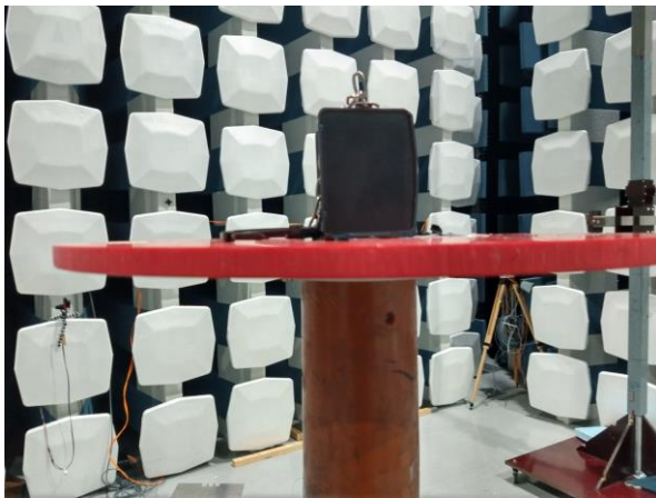
Radiated Emissions above 1 GHz, XZ plane
