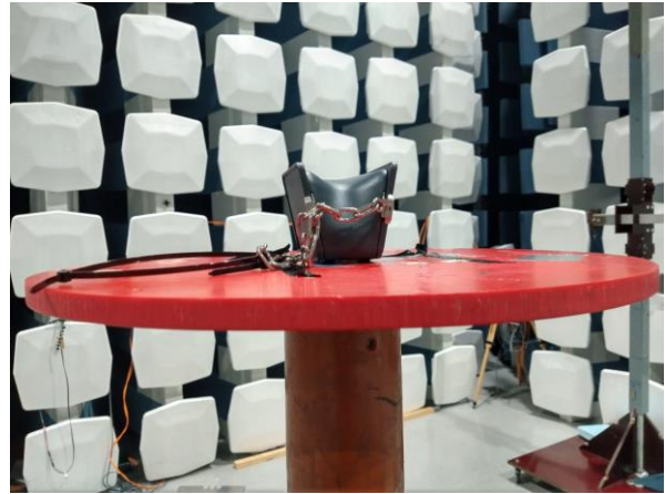
Radiated Emissions above 1GHz, XY plane
