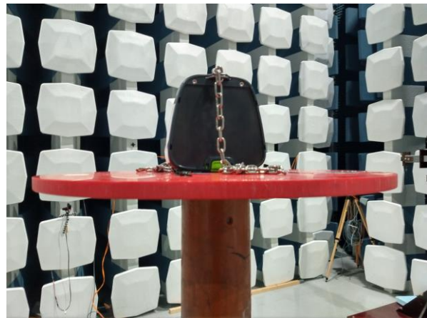
Radiated Emissions above 1 GHz, YZ plane
