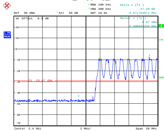
DH1_Hopping_Lower
