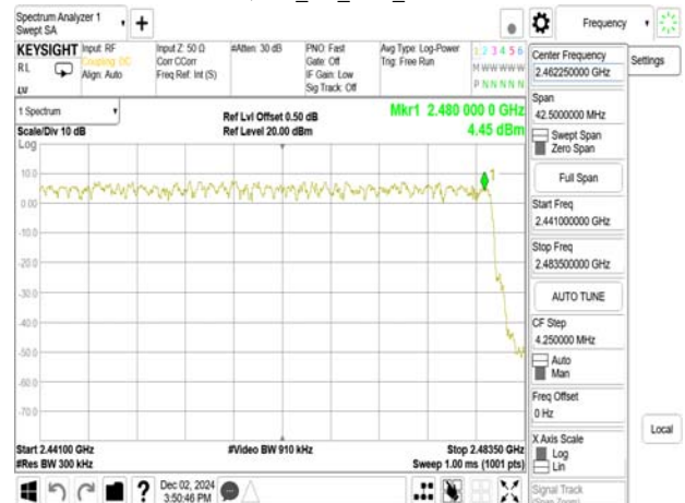
\pi/4 DQPSK_2M_DH5_2441-2480
