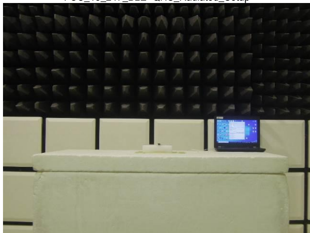
FCC_15_247_BLE+QHS_Radiated_Setup
