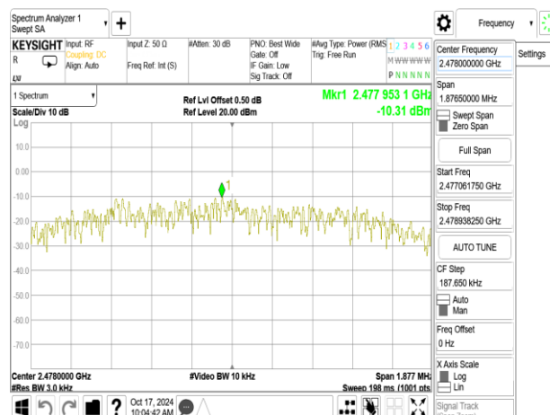
PSD_BLE 2M_HighCH38-2478MHz
