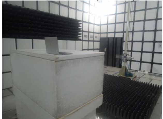
FCC_15_247_BT_Radiated_Spot Check_Setup
