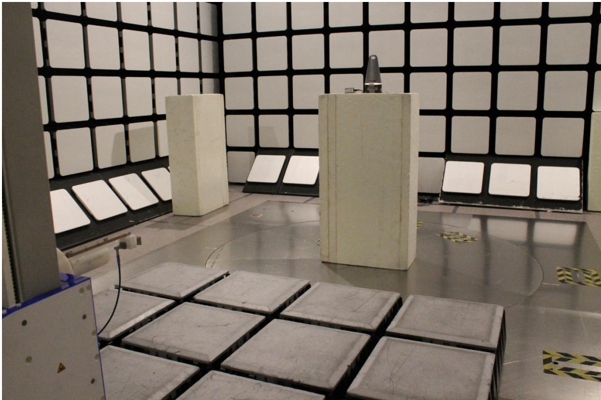
Photograph 3: Radiated spurious emissions setup 18 – 26.5 GHz
