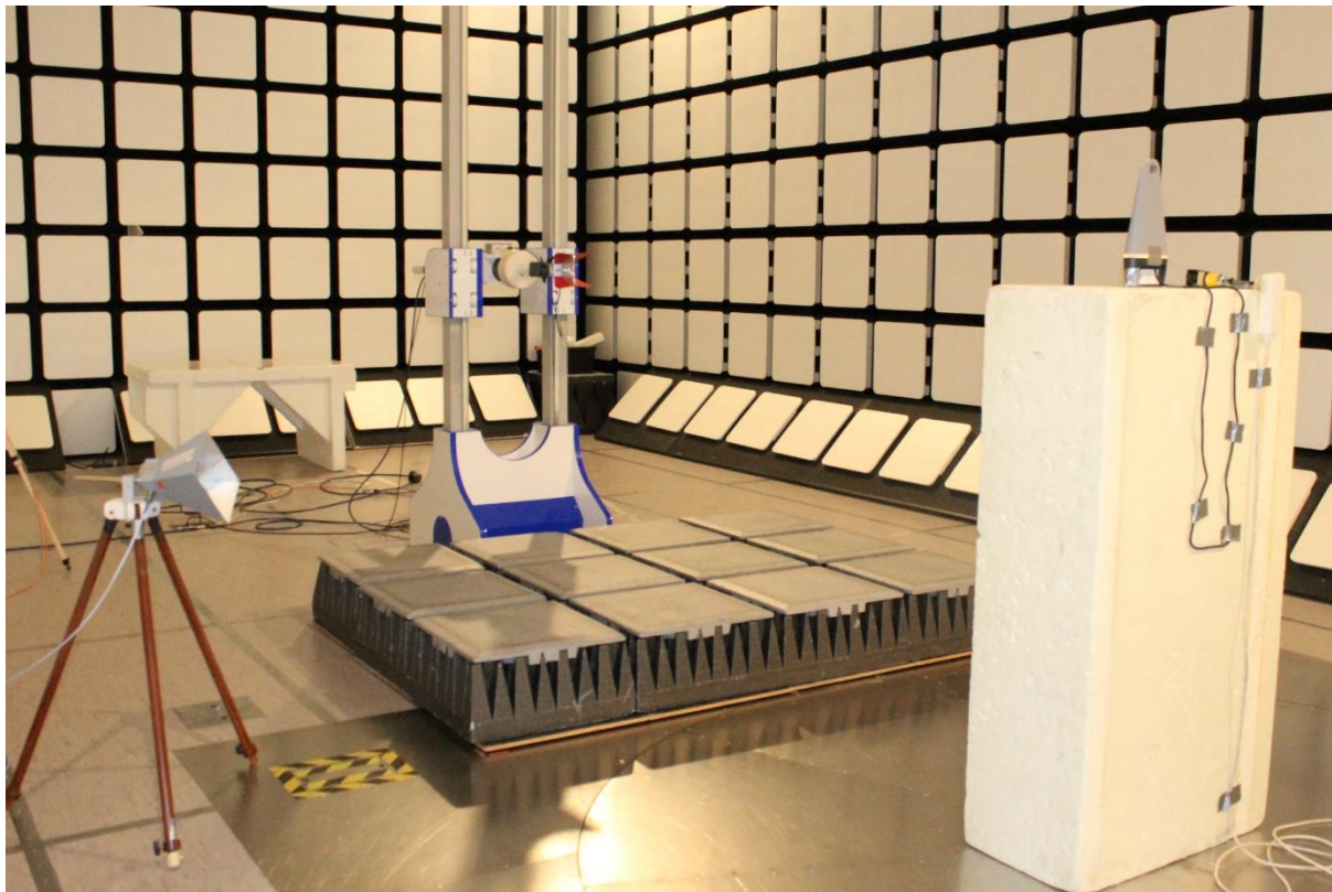
Photograph 2: Radiated spurious emissions setup 1 – 18GHz
