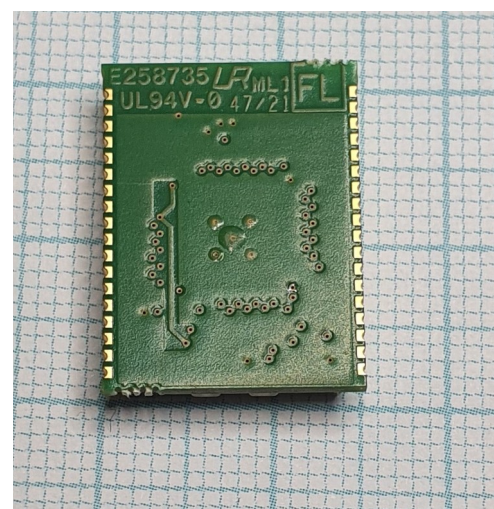
Figure 4: Bottom View
