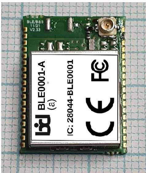
Figure 1: Top View U.F.L. Connector
