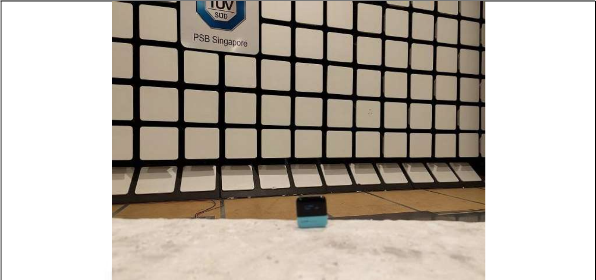
Radiated Emissions (Spurious Emissions Inclusive Restricted Bands Requirement) Test Setup (Front View)
