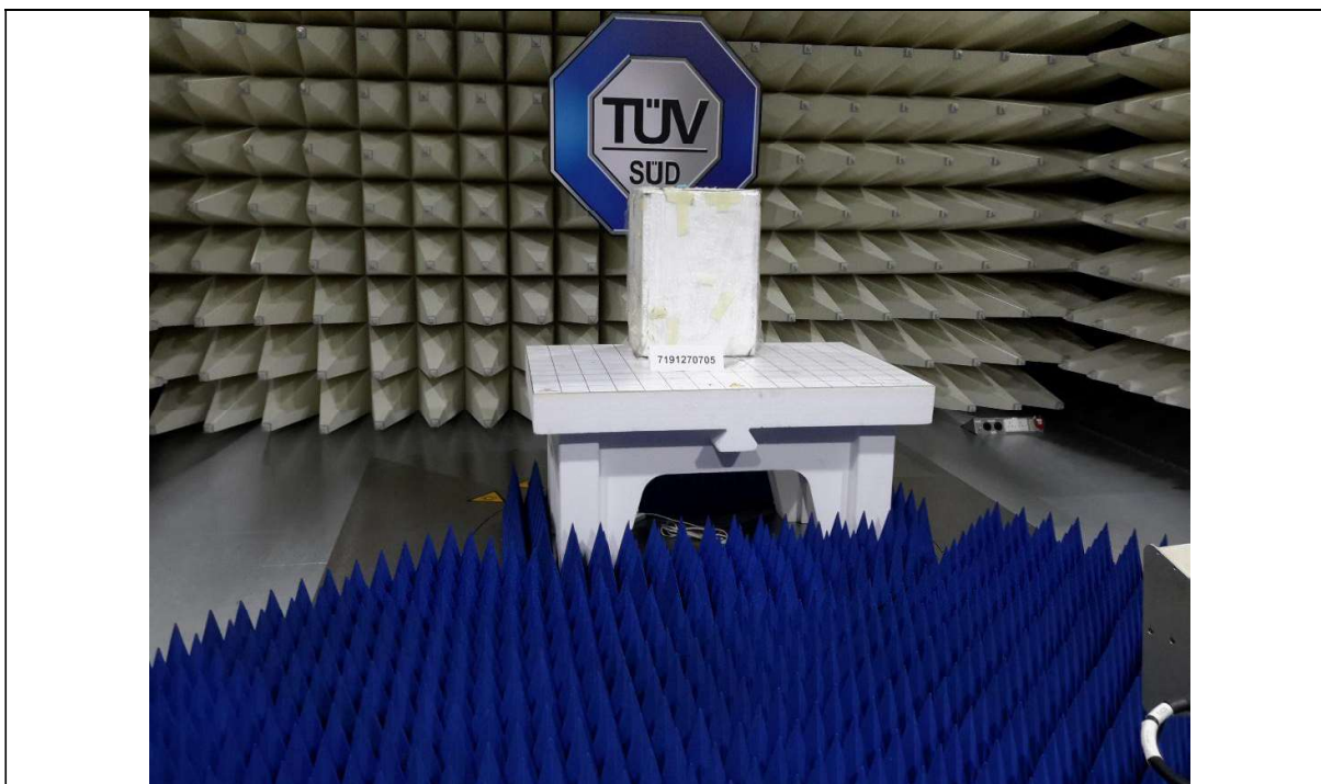
Radiated Emissions (Spurious Emissions Inclusive Restricted Bands Requirement) Test Setup (Front View)
