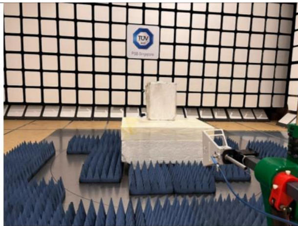
Radiated Emissions Test Setup (Front View)
