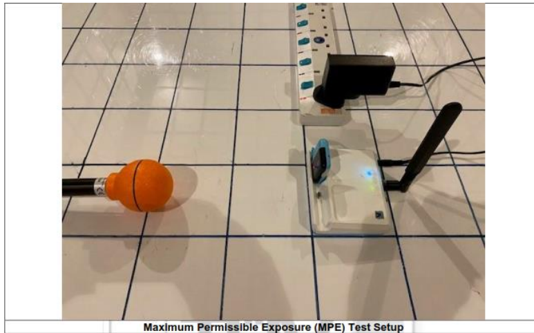
Maximum Permissible Exposure (MPE) Test Setup
