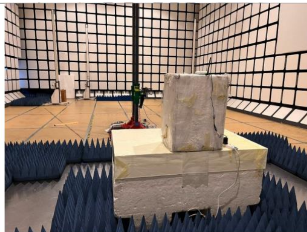
Radiated Emissions Test Setup (Rear View)
