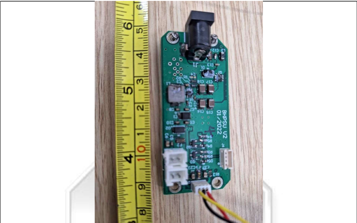
PCB View 4
