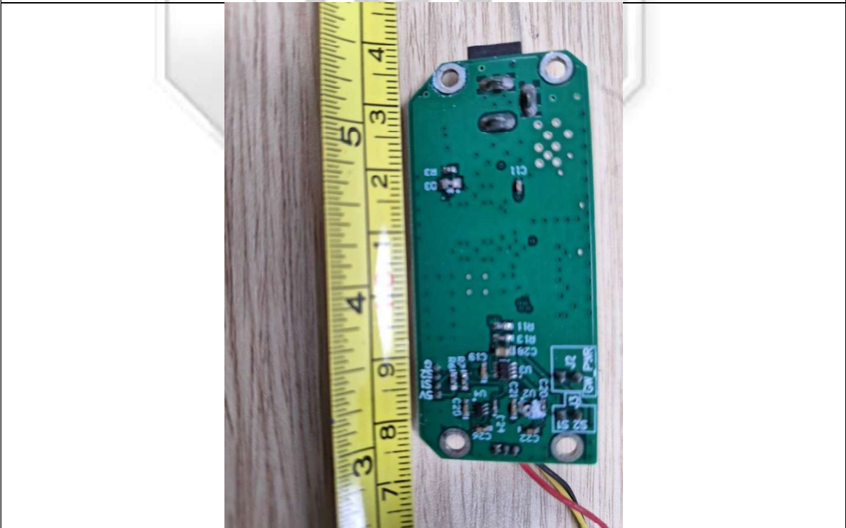
PCB View 5
