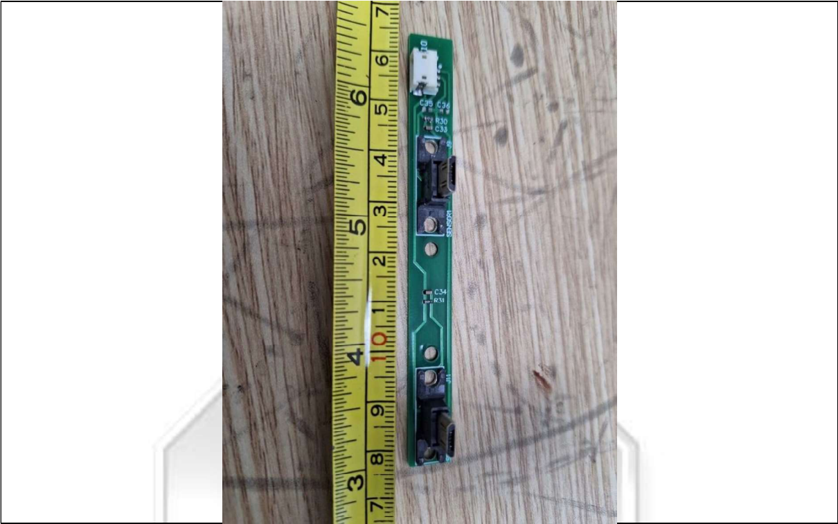
EUT PCB View 8
