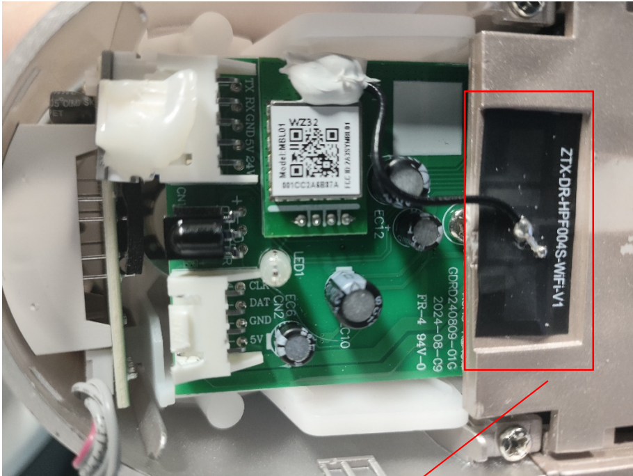
WiFi/BLE Antenna
