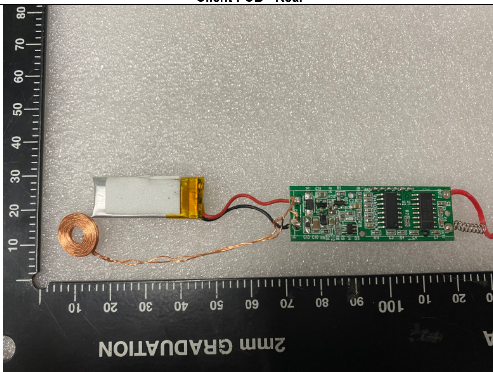
Client PCB - Rear
