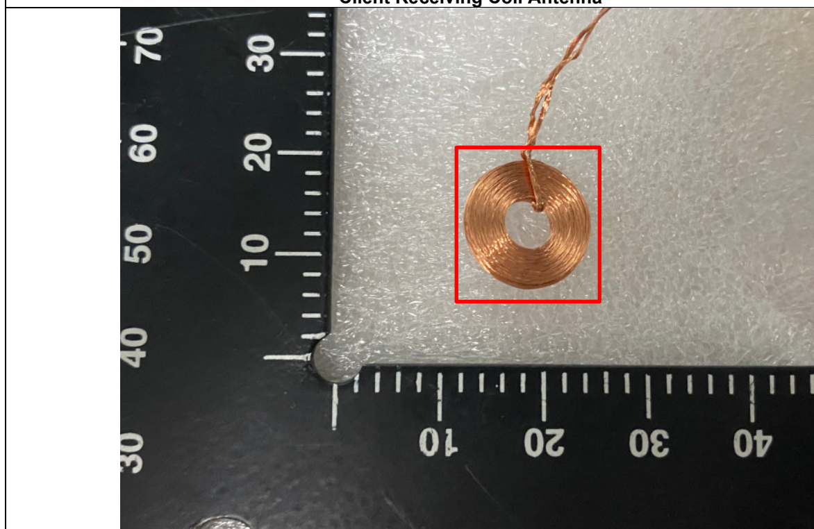
Client Receiving Coil Antenna
