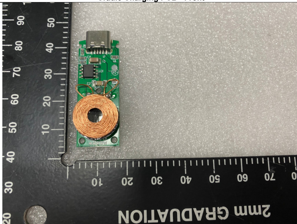
Cradle Charging PCB - Front
