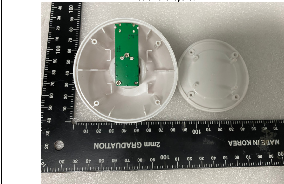
Cradle Cover opened
