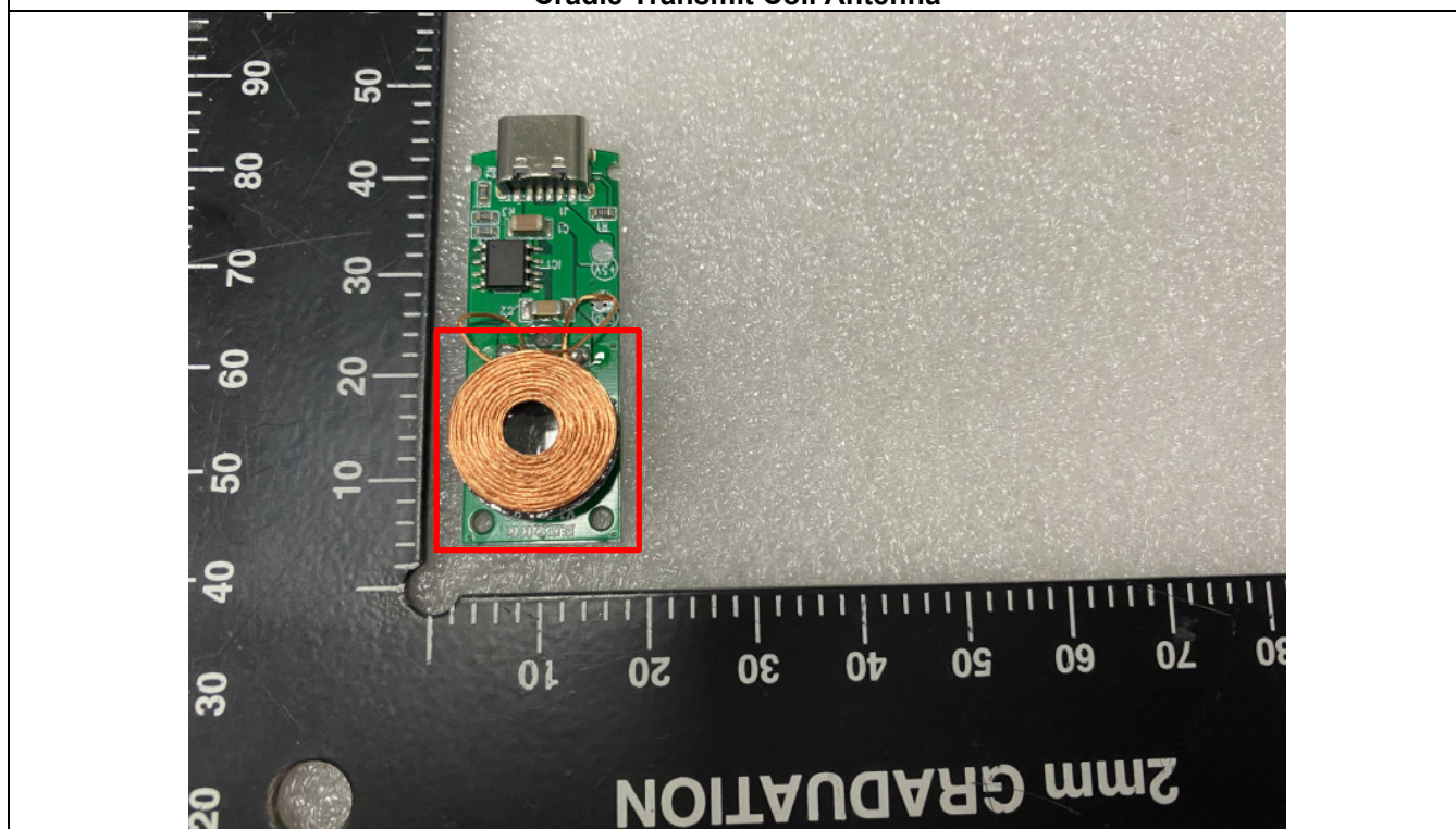
Cradle Transmit Coil Antenna
