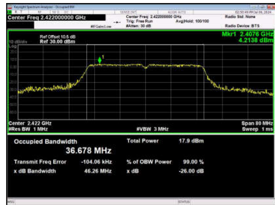
11N40SISO-Ant1-2422
