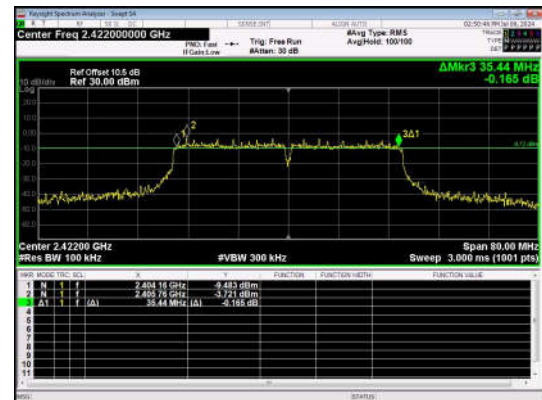
11N40SISO-Ant1-2422-PASS
