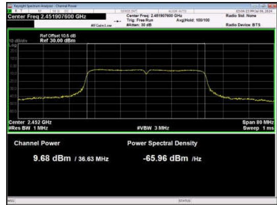
11N40SISO-Ant1-2452-PASS
