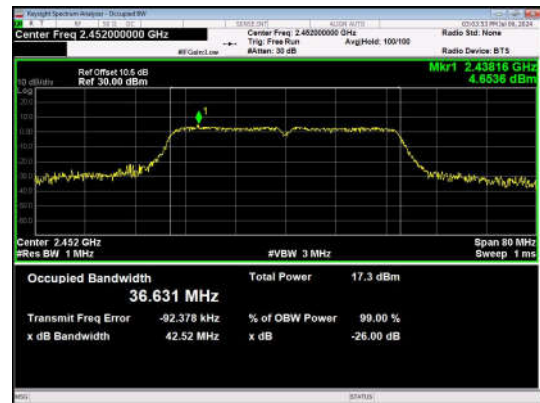
11N40SISO-Ant1-2452
