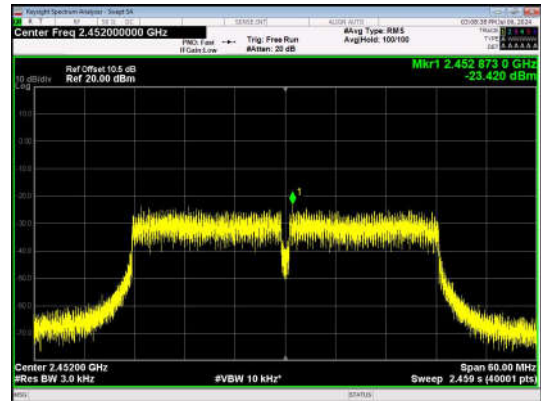
11N40SISO-Ant1-2452-PASS
