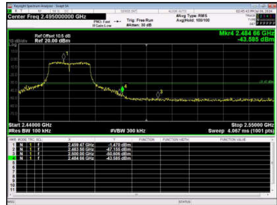
11N20SISO-Ant1-2462-PASS
