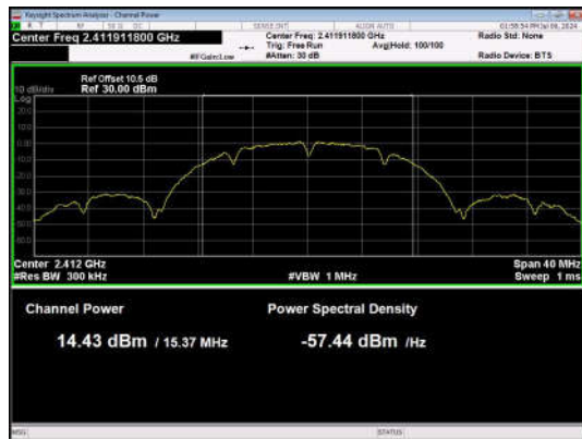
11B-Ant1-2412-PASS
