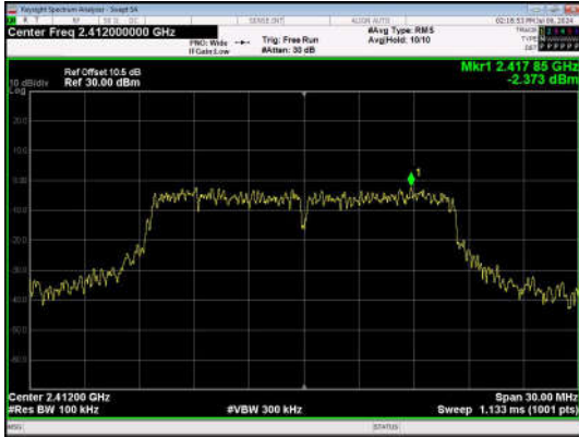
11G-Ant1-2412-0~Reference-PASS
