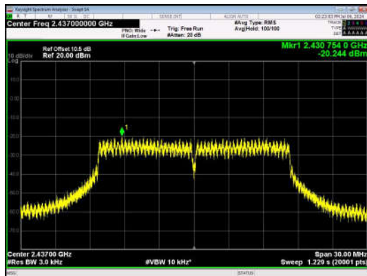
11G-Ant1-2437-PASS
