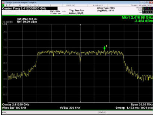
11N20SISO-Ant1-2412-0~Reference-PASS
