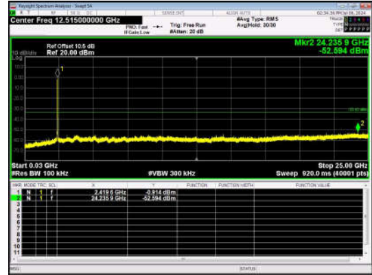
11N20SISO-Ant1-2412-30~25000-PASS
