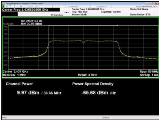
11N40SISO-Ant1-2437-PASS
