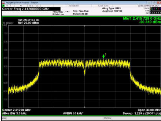
11N20SISO-Ant1-2412-PASS
