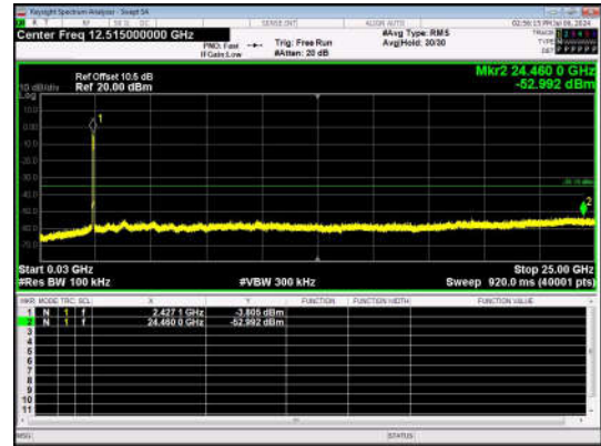
11N40SISO-Ant1-2422-30~25000-PASS
