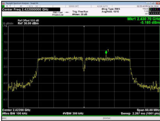
11N40SISO-Ant1-2422-0~Reference-PASS
