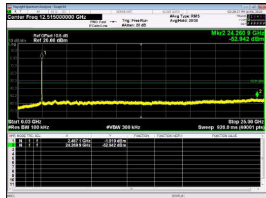
11G-Ant1-2462-30~25000-PASS
