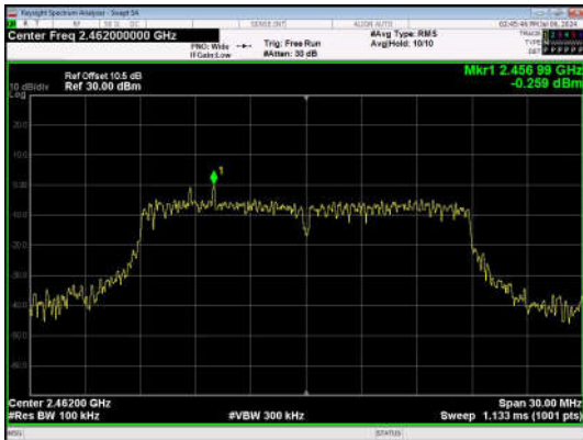
11N20SISO-Ant1-2462-0~Reference-PASS
