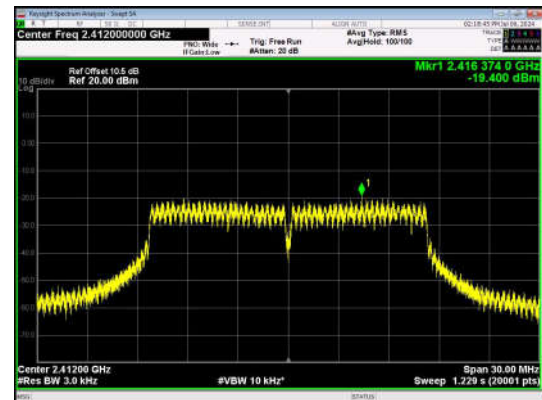
11G-Ant1-2412-PASS
