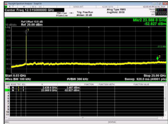
11B-Ant1-2437-30~25000-PASS
