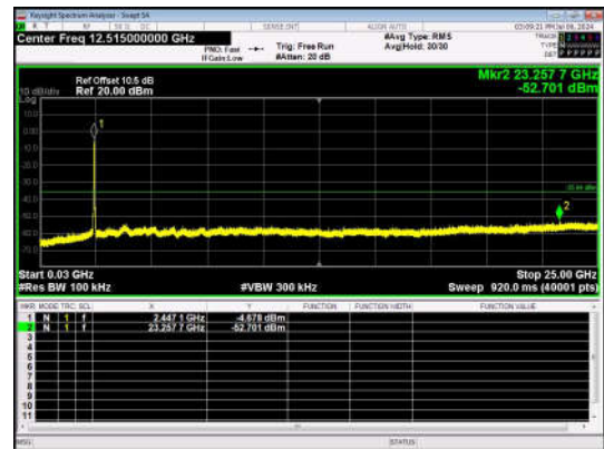
11N40SISO-Ant1-2452-30~25000-PASS
