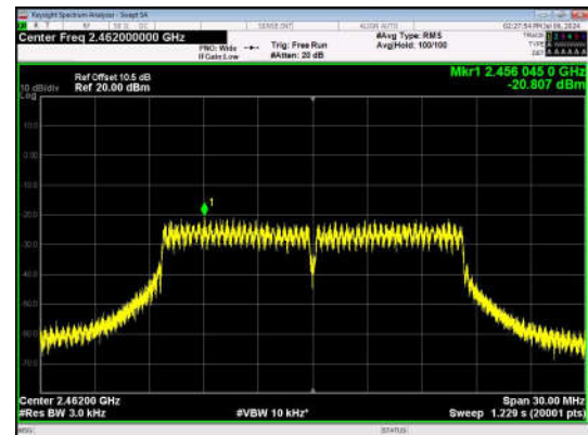
11G-Ant1-2462-PASS
