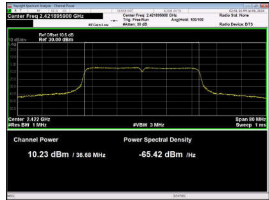
11N40SISO-Ant1-2422-PASS
