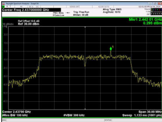
11N20SISO-Ant1-2437-0~Reference-PASS
