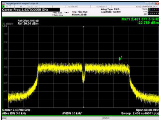
11N40SISO-Ant1-2437-PASS
