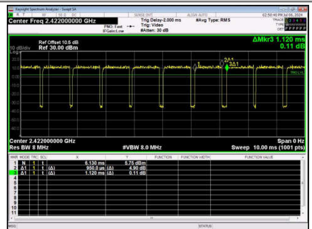
NTNV-11N40SISO-Ant1-2422
