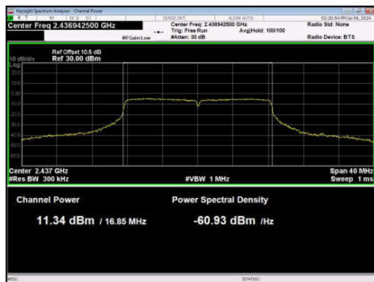
11G-Ant1-2437-PASS
