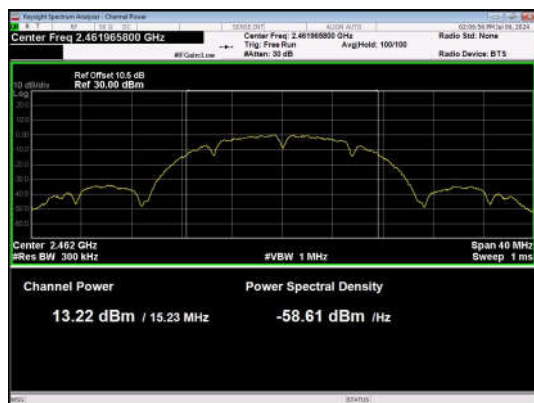
11B-Ant1-2462-PASS
