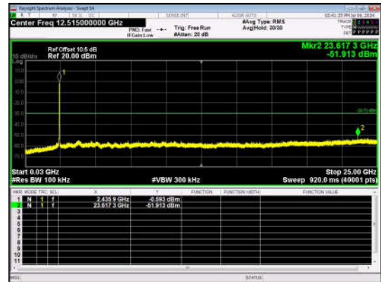
11N20SISO-Ant1-2437-30~25000-PASS
