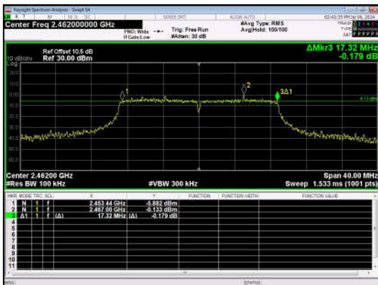
11N20SISO-Ant1-2462-PASS
