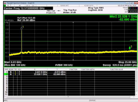
11G-Ant1-2437-30~25000-PASS
