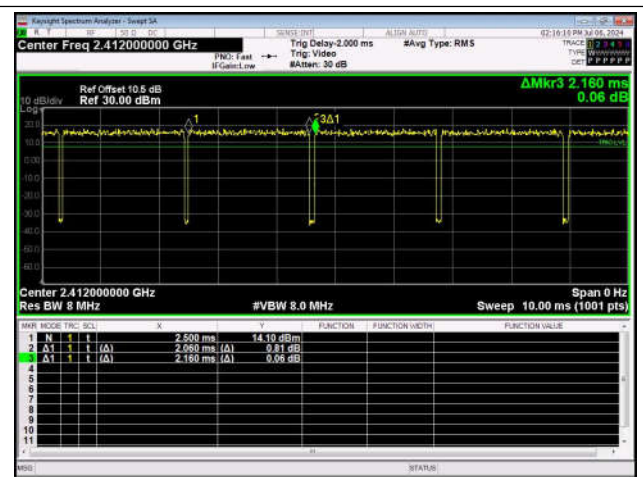
NTNV-11G-Ant1-2412
