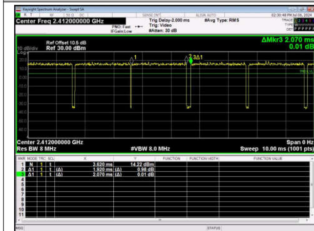
NTNV-11N20SISO-Ant1-2412
