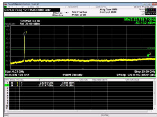
11N40SISO-Ant1-2437-30~25000-PASS
