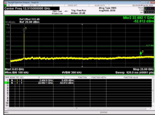
11G-Ant1-2412-30~25000-PASS
