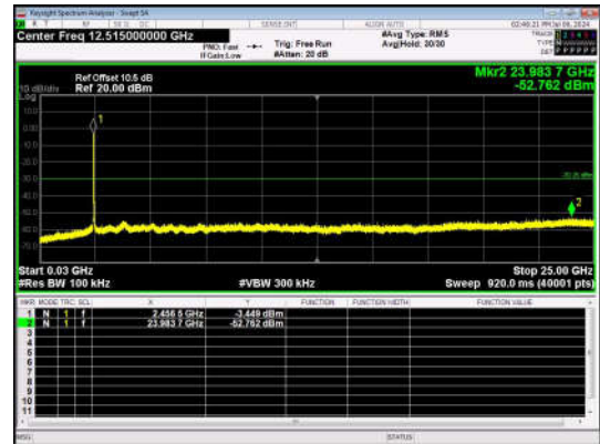
11N20SISO-Ant1-2462-30~25000-PASS
