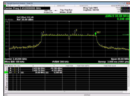
11N40SISO-Ant1-2452-PASS
