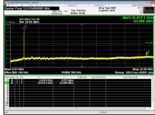
11B-Ant1-2412-30~25000-PASS
