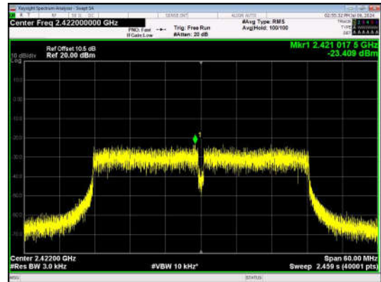
11N40SISO-Ant1-2422-PASS
