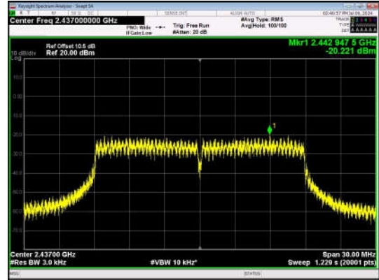
11N20SISO-Ant1-2437-PASS
