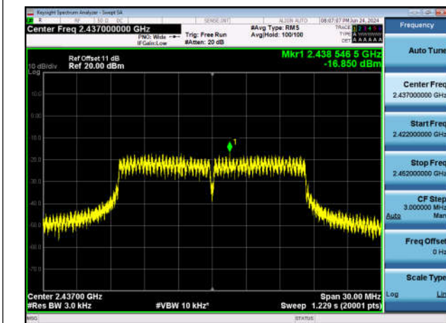
11G-Ant1-2437-PASS
