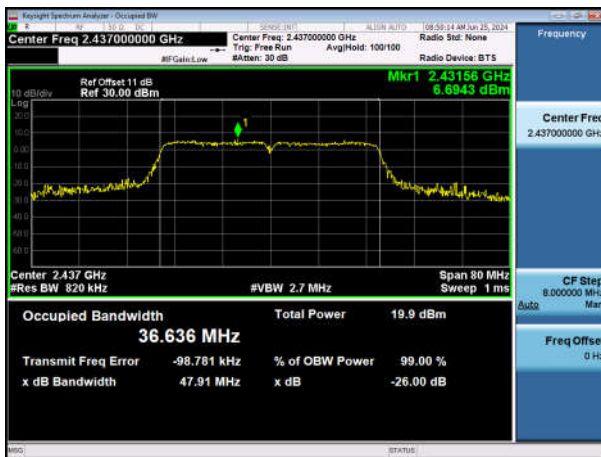
11N40SISO-Ant1-2437
