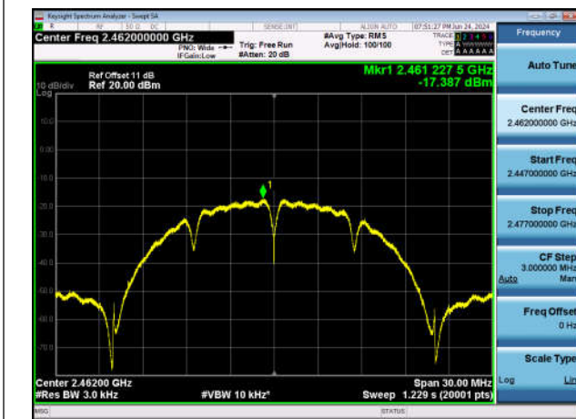
11B-Ant1-2462-PASS
