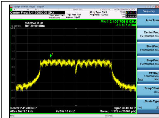
11N20SISO-Ant1-2412-PASS
