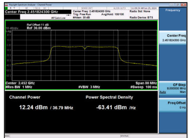
11N40SISO-Ant1-2452-PASS
