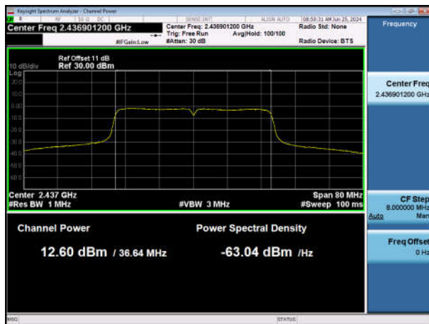
11N40SISO-Ant1-2437-PASS
