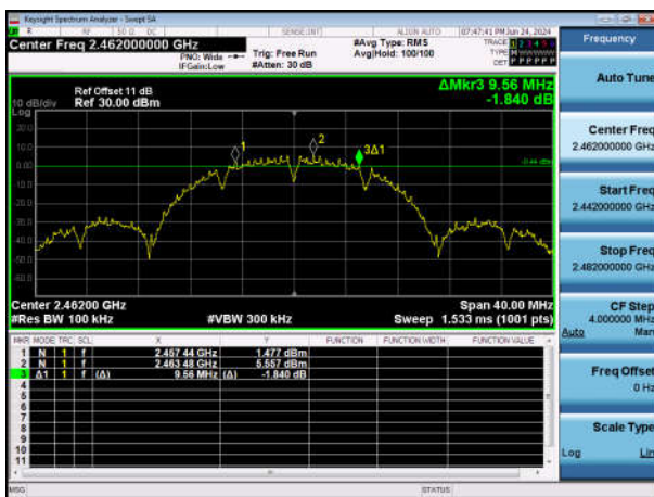
11B-Ant1-2462-PASS
