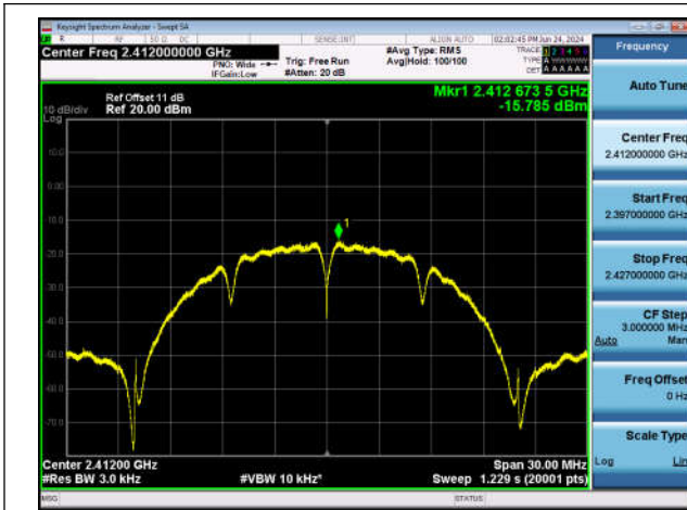
11B-Ant1-2412-PASS
