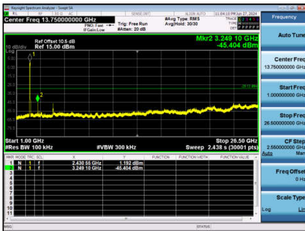
11N40SISO-Ant1-2437-1000~26500-PASS
