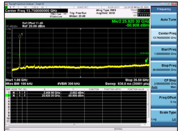
11N40SISO-Ant1-2452-1000~26500-PASS
