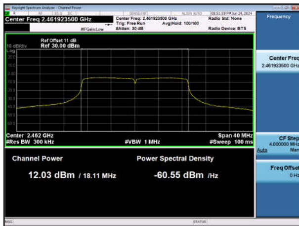
11N20SISO-Ant1-2462-PASS
