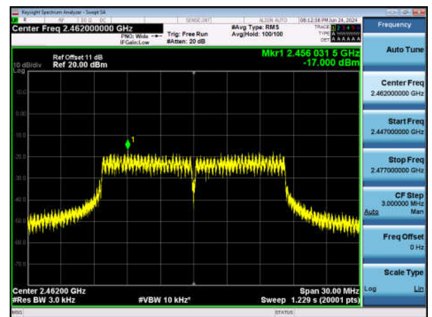
11G-Ant1-2462-PASS
