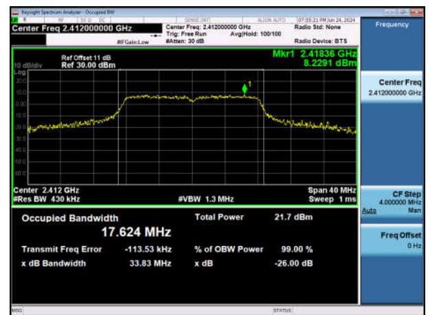
11G-Ant1-2412
