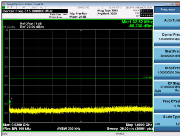
11N40SISO-Ant1-2452-30~1000-PASS
