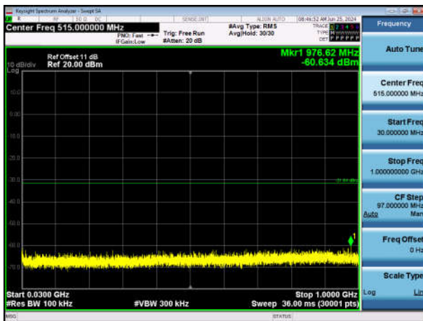
11N40SISO-Ant1-2422-30~1000-PASS
