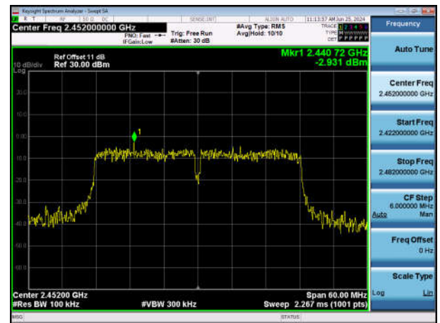
11N40SISO-Ant1-2452-0~Reference-PASS
