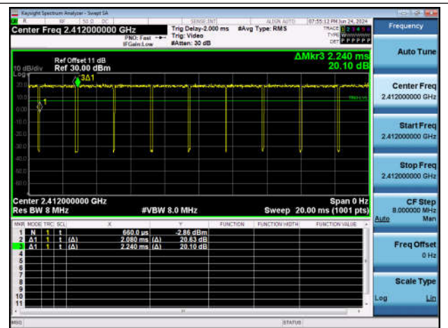
NTNV-11G-Ant1-2412
