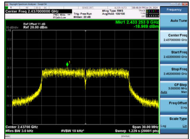
11N20SISO-Ant1-2437-PASS
