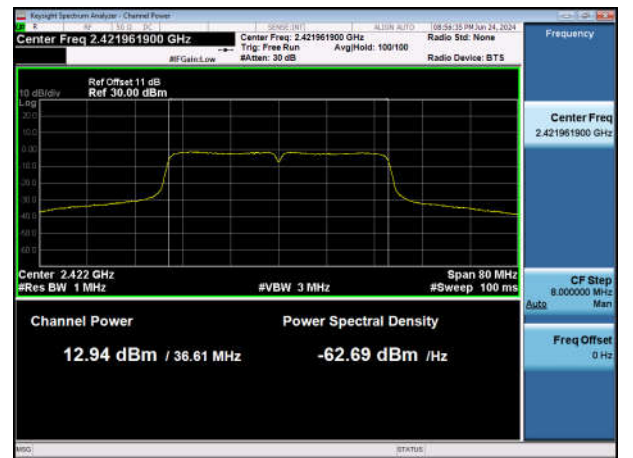
11N40SISO-Ant1-2422-PASS
