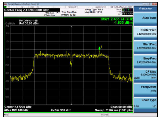
11N40SISO-Ant1-2422-0~Reference-PASS
