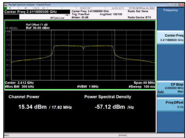
11G-Ant1-2412-PASS
