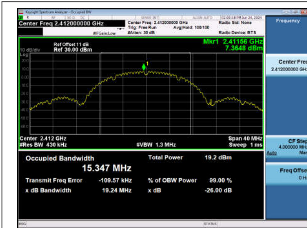
11B-Ant1-2412
