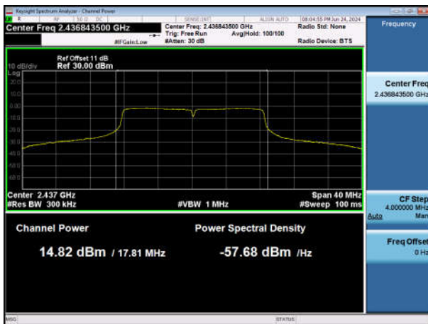
11G-Ant1-2437-PASS
