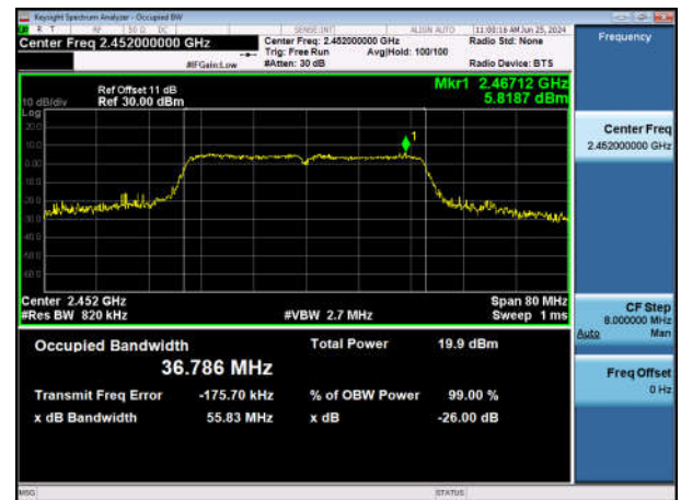
11N40SISO-Ant1-2452
