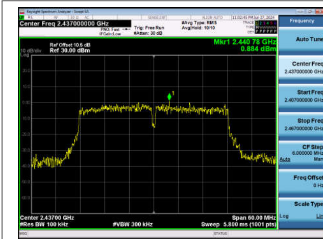
11N40SISO-Ant1-2437-0~Reference-PASS
