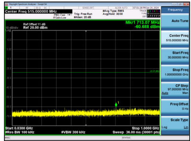
11B-Ant1-2462-30~1000-PASS
