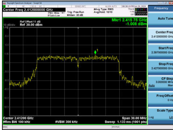
11N20SISO-Ant1-2412-0~Reference-PASS
