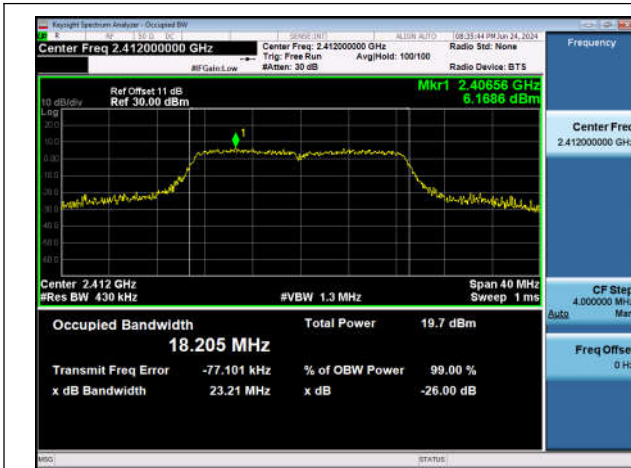
11N20SISO-Ant1-2412
