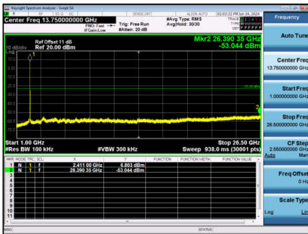
11B-Ant1-2412-1000~26500-PASS
