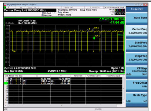
NTNV-11N40SISO-Ant1-2422
