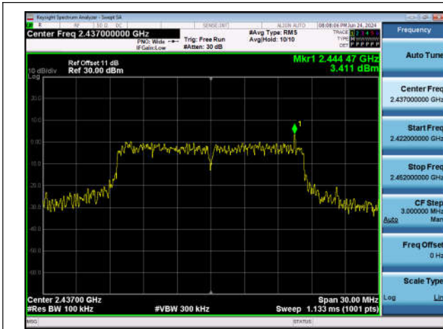
11G-Ant1-2437-0~Reference-PASS
