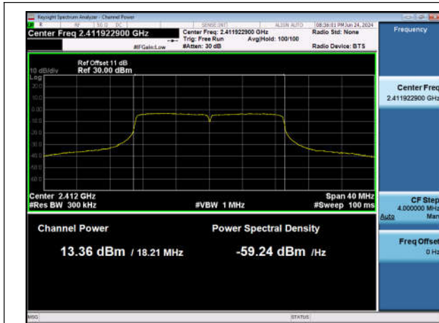
11N20SISO-Ant1-2412-PASS
