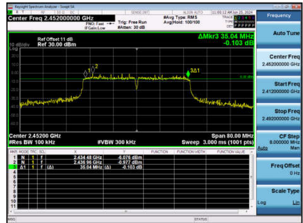
11N40SISO-Ant1-2452-PASS
