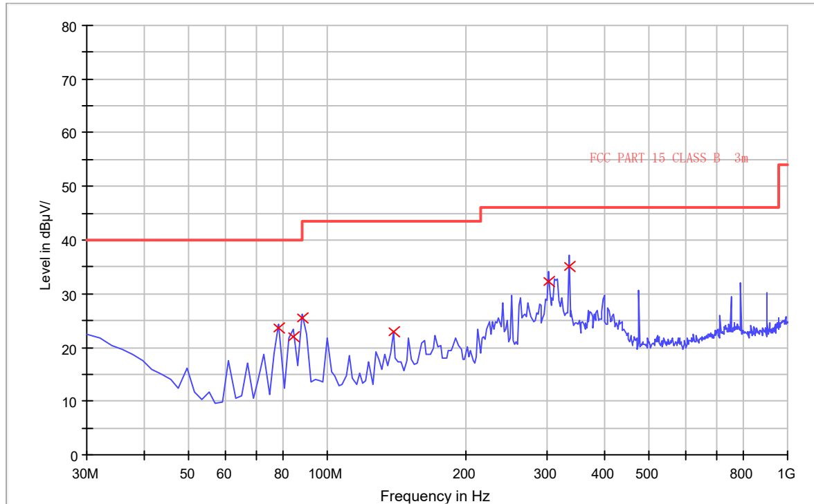
EMI Sweep-3M(30-1G)
