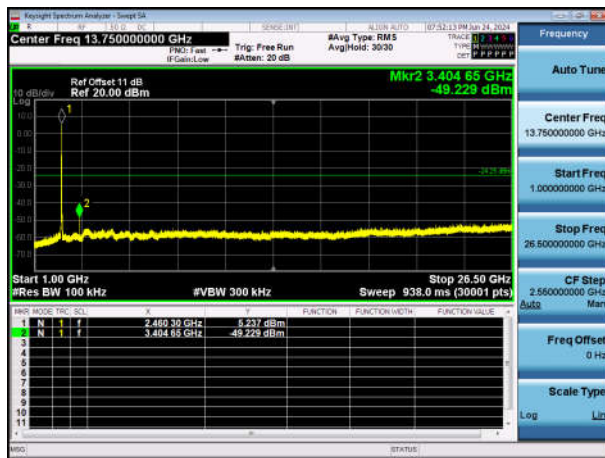
11B-Ant1-2462-1000~26500-PASS
