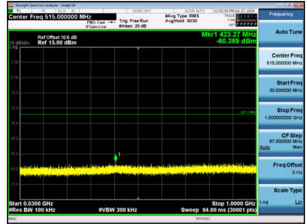
11N40SISO-Ant1-2437-30~1000-PASS
