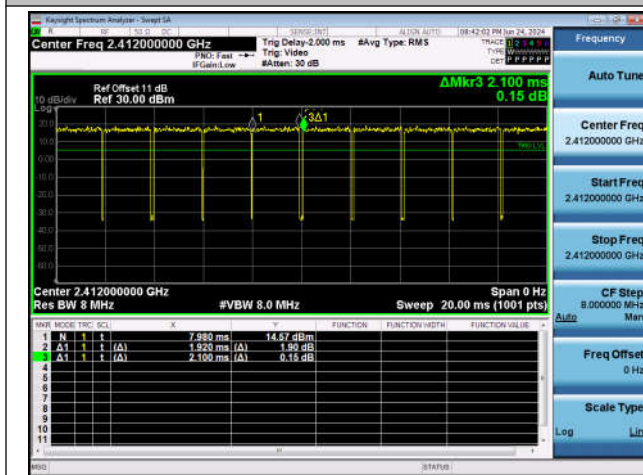
NTNV-11N20SISO-Ant1-2412
