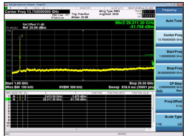
11N40SISO-Ant1-2422-1000~26500-PASS
