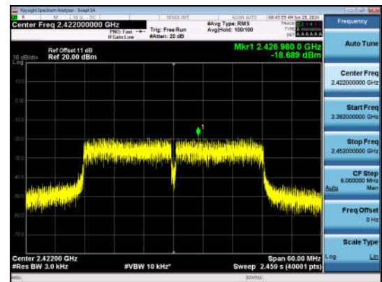
11N40SISO-Ant1-2422-PASS
