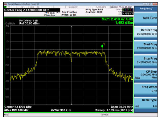
11G-Ant1-2412-0~Reference-PASS
