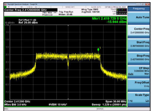
11G-Ant1-2412-PASS
