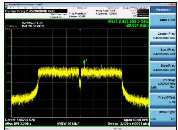
11N40SISO-Ant1-2452-PASS
