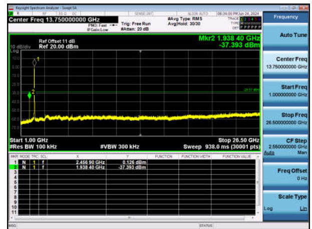
11G-Ant1-2462-1000~26500-PASS
