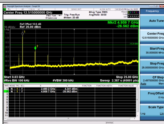
BLE_1M-Ant1-2480-30-25000-PASS
