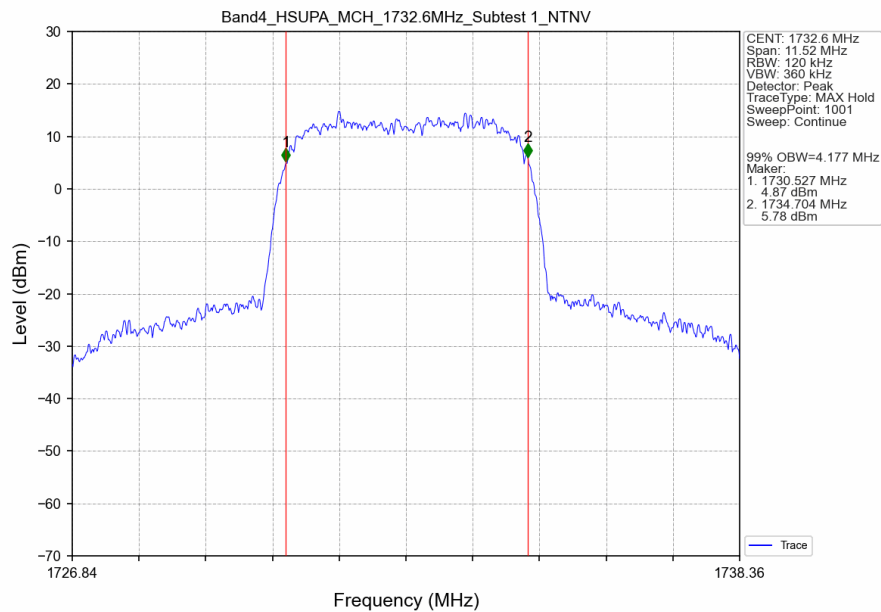
Band4_HSUPA_MCH_1732.6MHz_Subtest 1_NTNV
