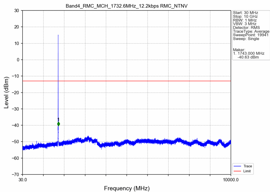
Band4_RMC_MCH_1732.6MHz_12.2kbps RMC_NTNV
