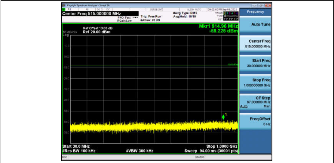
Zigbee_Ant1_2440_30~1000
