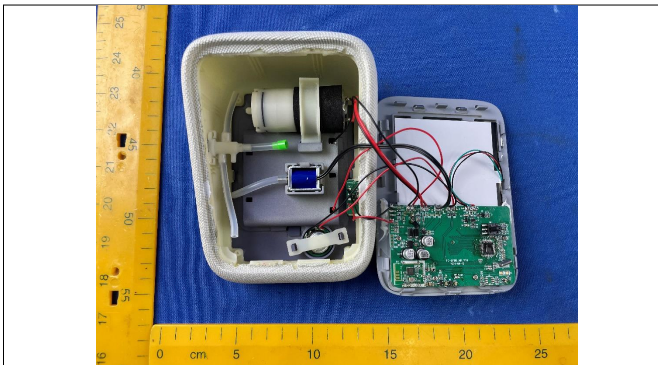
Details of: Internal view 2 of main unit (M/N: FC-BP110)
