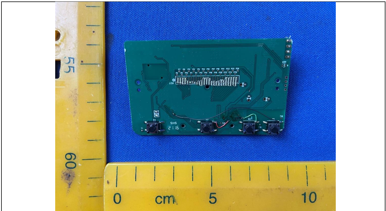
Details of: PCB view 5 of main unit (M/N: FC-BP110)
