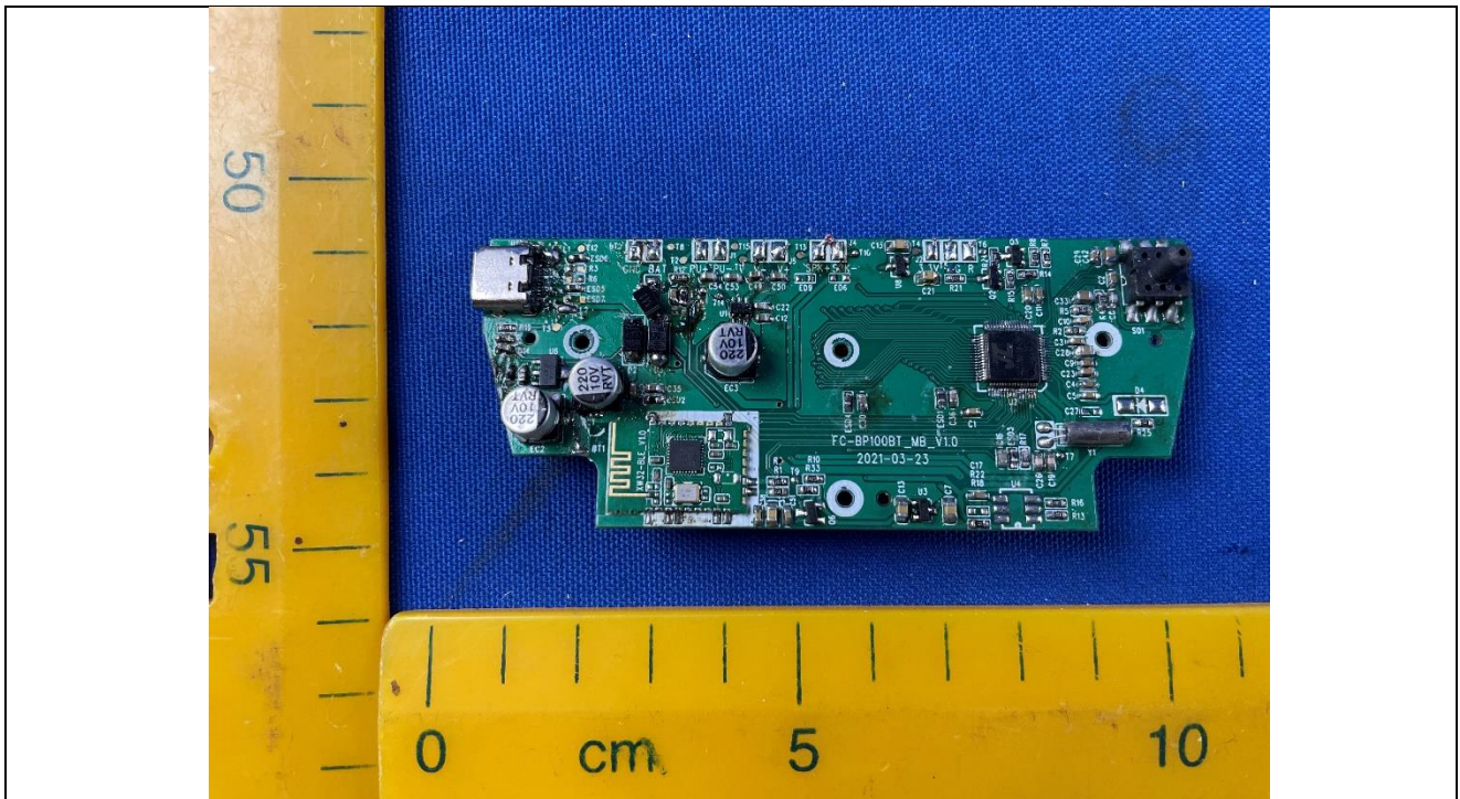
Details of: PCB view 4 of main unit (M/N: FC-BP100)
