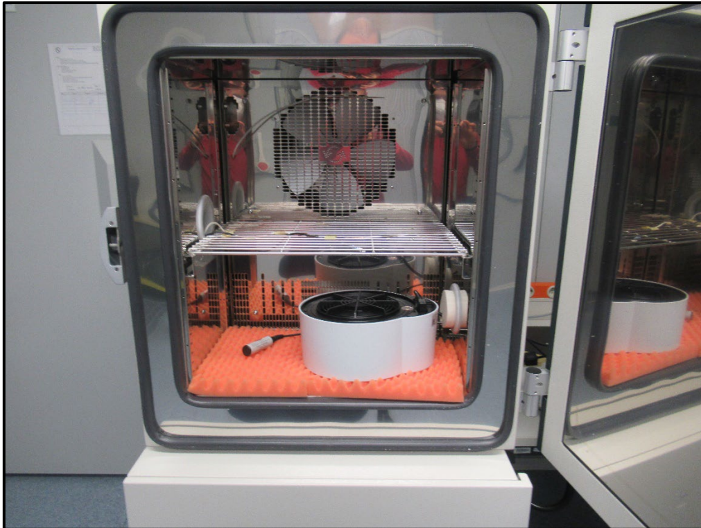
Photo 5: Frequency Stability & Bandwidth Test Setup
