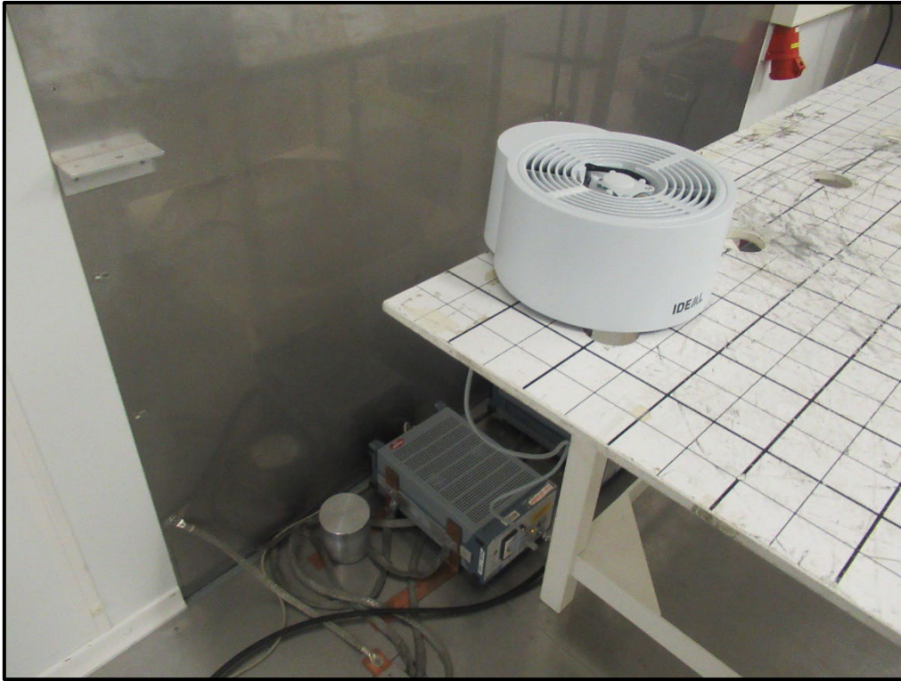
Photo 7: AC Conducted Emissions Test Setup
