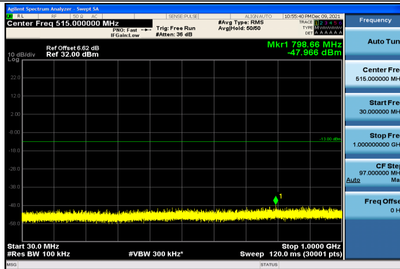
Band25-10MHz-64QAM-26640-1RB#0-30~1000MHz
