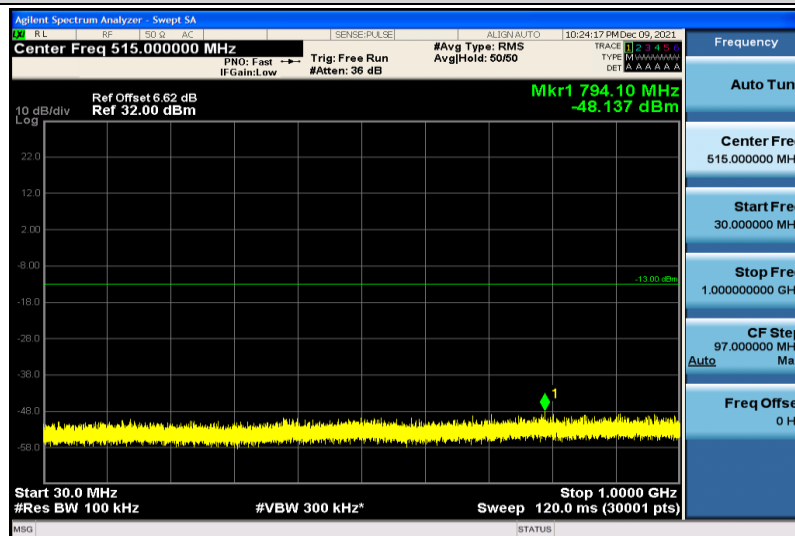
Band25-1.4MHz-64QAM-26365-1RB#0-30~1000MHz
