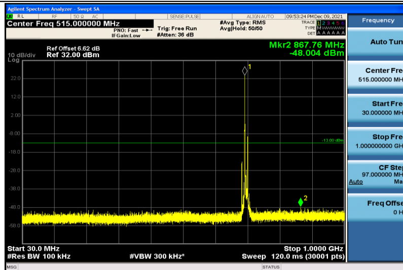
Band12-10MHz-64QAM-23060-1RB#0-30~1000MHz
