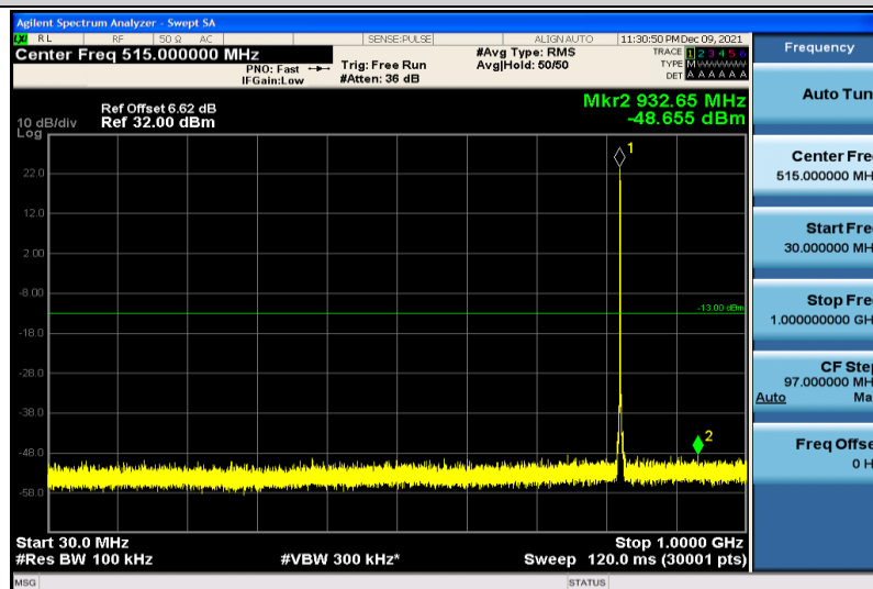
Band26-1.4MHz-64QAM-26797-1RB#0-30~1000MHz
