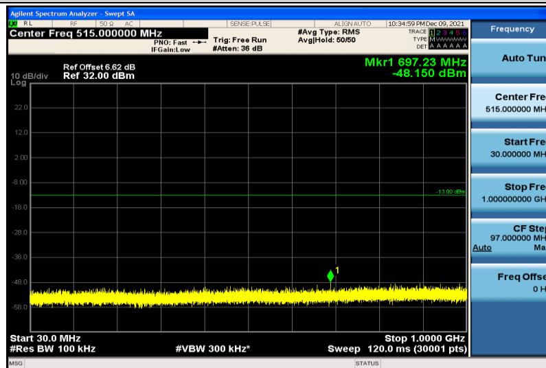
Band25-3MHz-64QAM-26365-1RB#0-30~1000MHz
