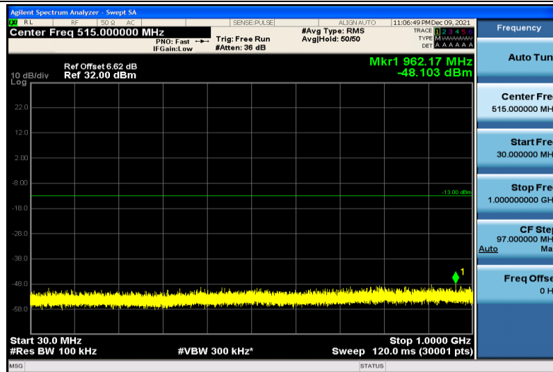
Band25-15MHz-64QAM-26615-1RB#0-30~1000MHz
