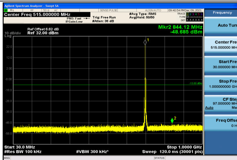
Band12-5MHz-64QAM-23095-1RB#0-30~1000MHz
