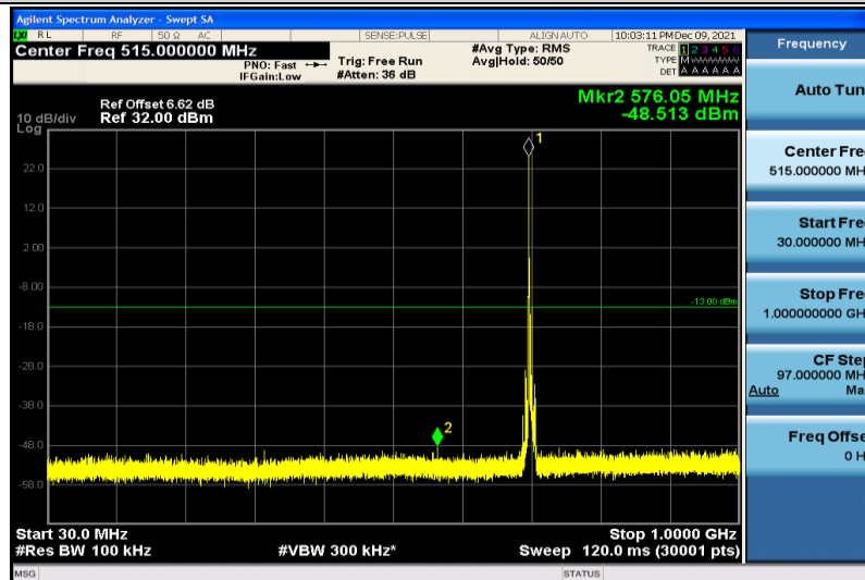
Band17-5MHz-64QAM-23755-1RB#0-30~1000MHz
