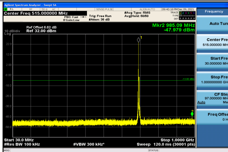
Band12-5MHz-64QAM-23035-1RB#0-30~1000MHz
