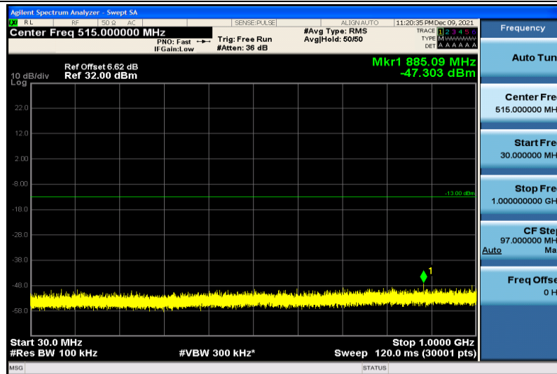
Band25-20MHz-64QAM-26590-1RB#0-30~1000MHz
