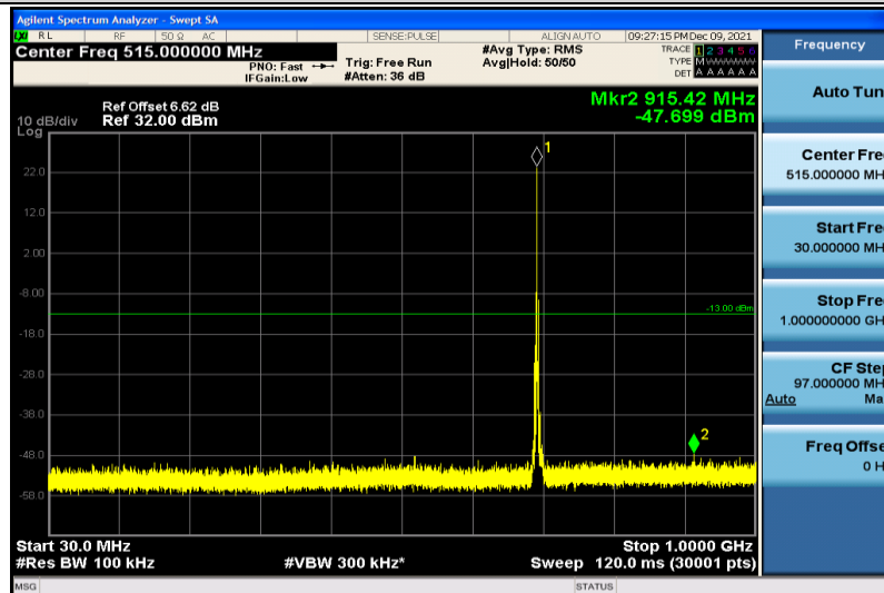
Band12-3MHz-64QAM-23025-1RB#0-30~1000MHz
