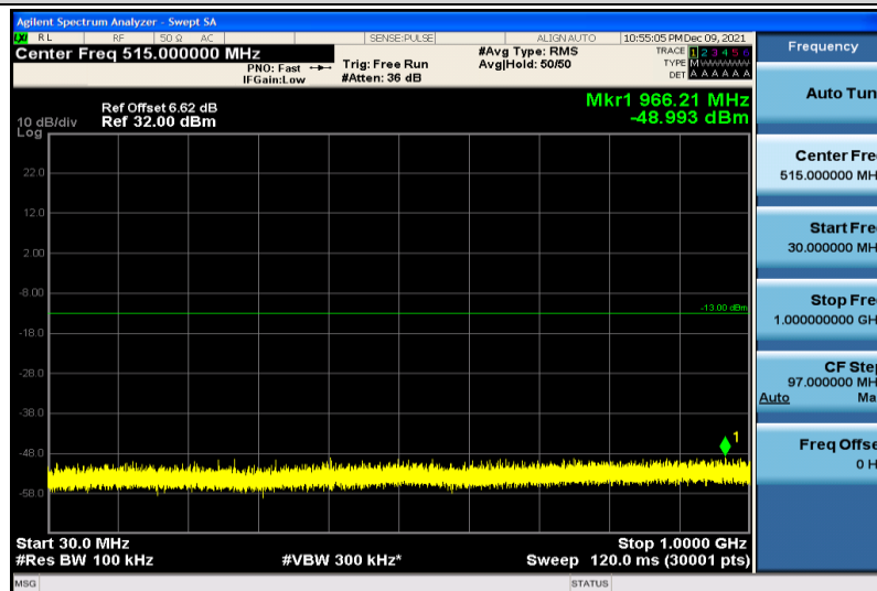
Band25-10MHz-64QAM-26365-1RB#0-30~1000MHz
