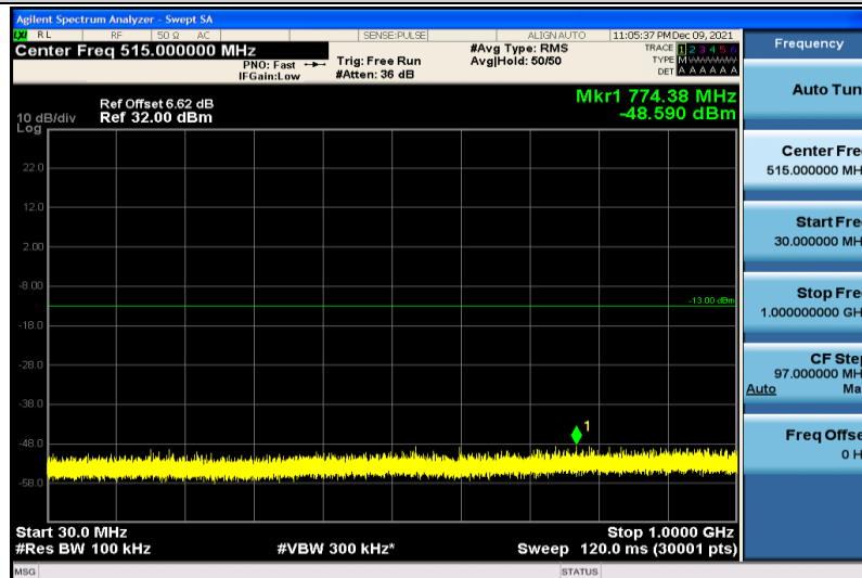
Band25-15MHz-64QAM-26115-1RB#0-30~1000MHz
