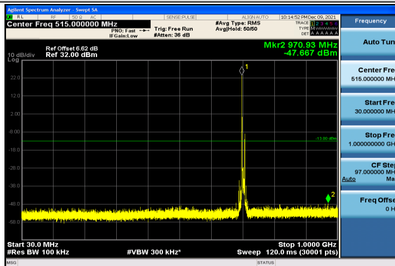
Band17-10MHz-64QAM-23790-1RB#0-30~1000MHz
