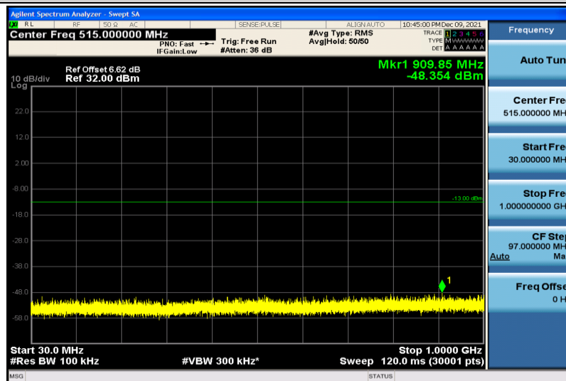
Band25-5MHz-64QAM-26365-1RB#0-30~1000MHz
