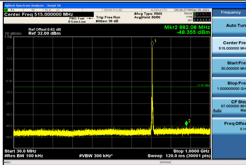
Band12-3MHz-64QAM-23165-1RB#0-30~1000MHz
