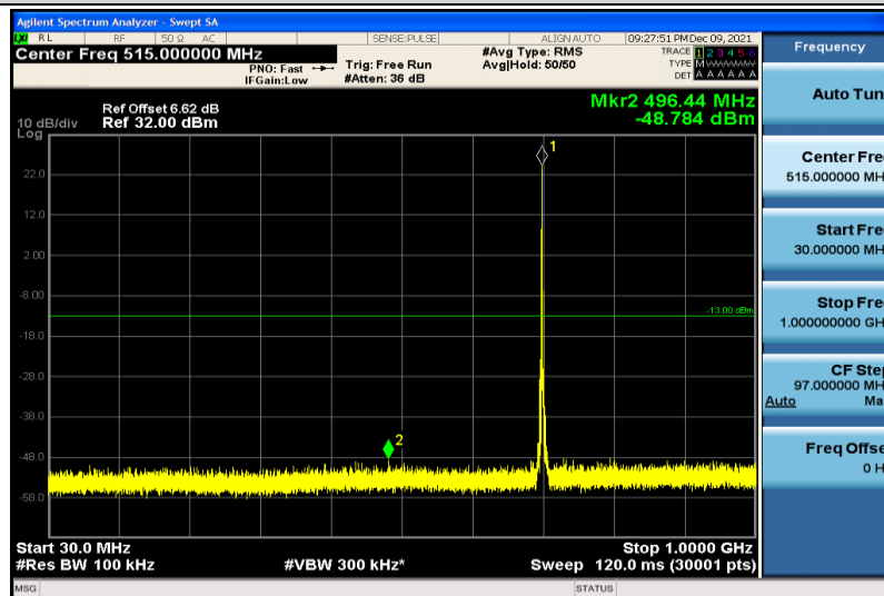
Band12-3MHz-64QAM-23095-1RB#0-30~1000MHz
