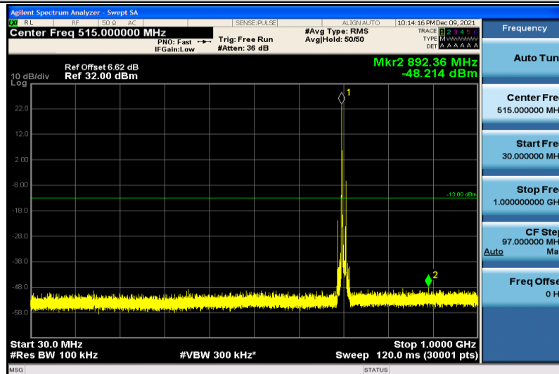
Band17-10MHz-64QAM-23780-1RB#0-30~1000MHz
