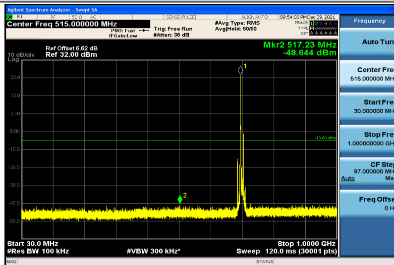
Band12-10MHz-64QAM-23095-1RB#0-30~1000MHz
