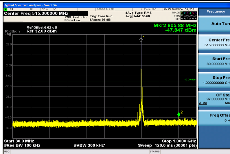
Band17-10MHz-64QAM-23800-1RB#0-30~1000MHz
