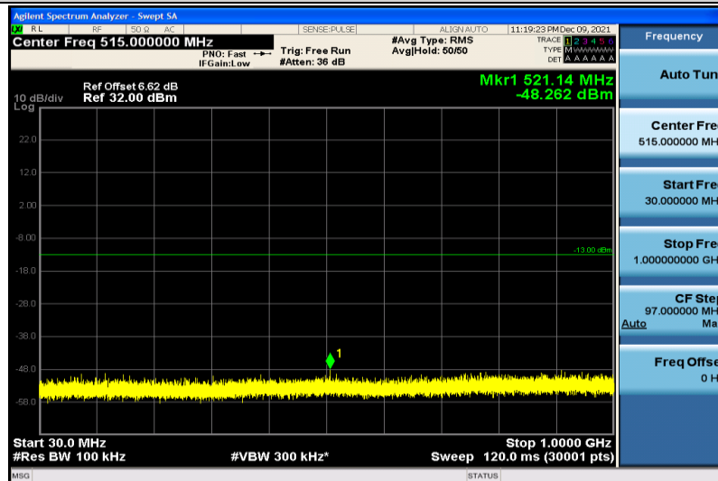
Band25-20MHz-64QAM-26140-1RB#0-30~1000MHz
