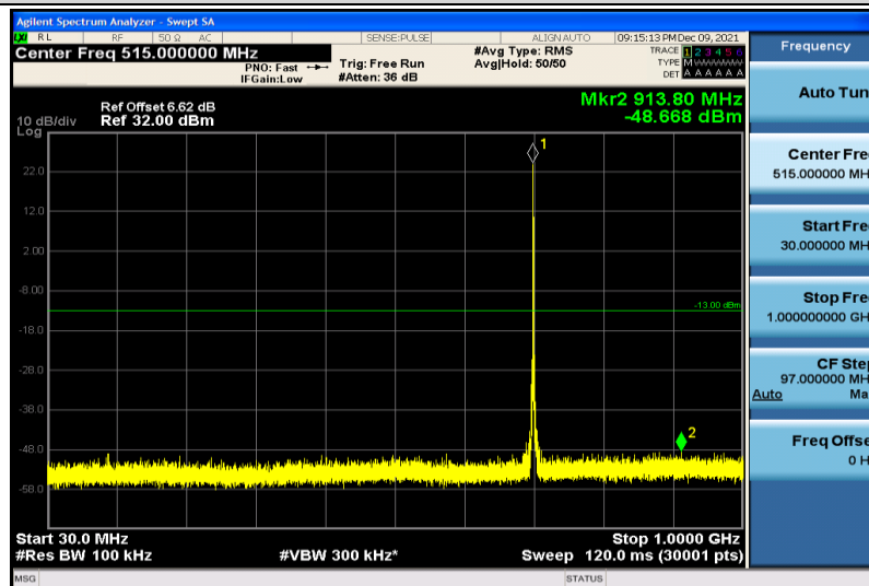
Band12-1.4MHz-64QAM-23095-1RB#0-30~1000MHz
