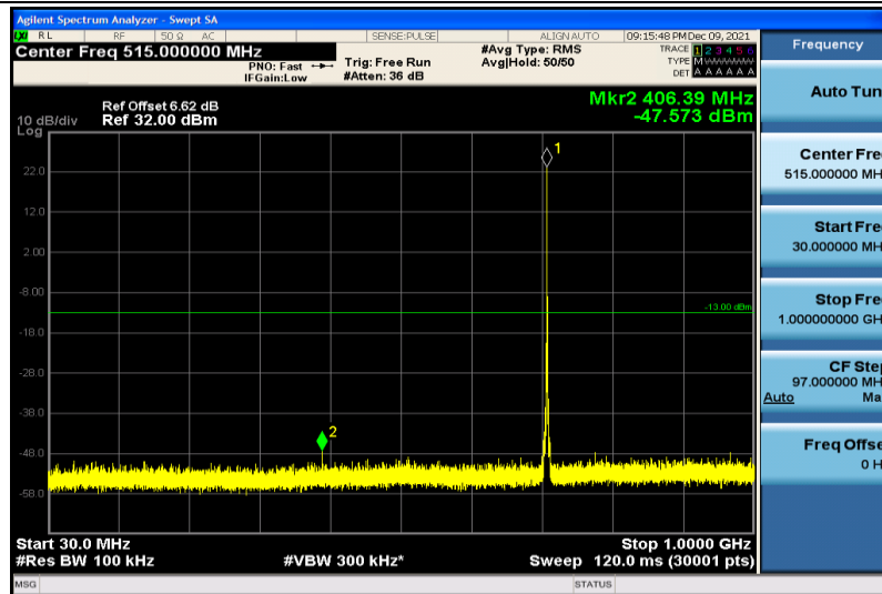
Band12-1.4MHz-64QAM-23173-1RB#0-30~1000MHz
