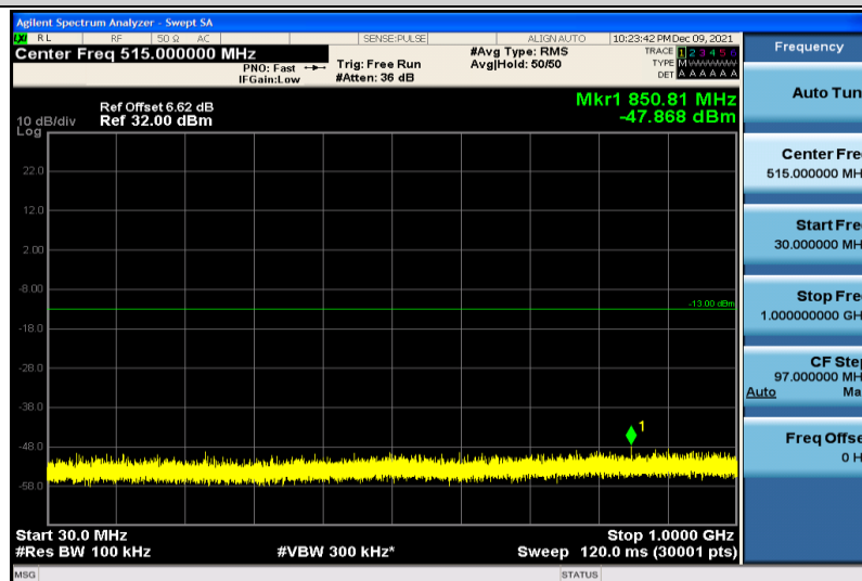
Band25-1.4MHz-64QAM-26047-1RB#0-30~1000MHz
