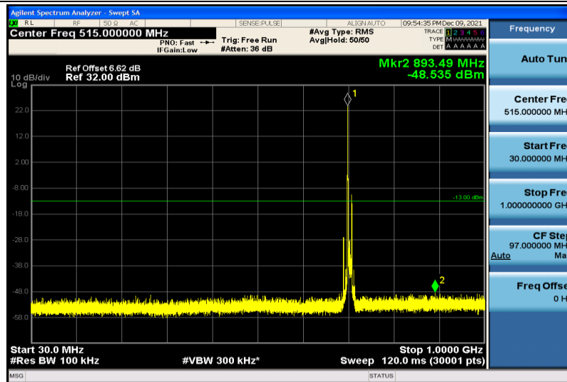
Band12-10MHz-64QAM-23130-1RB#0-30~1000MHz
