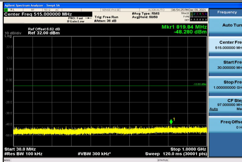
Band4-5MHz-64QAM-19975-1RB#0-30~1000MHz
