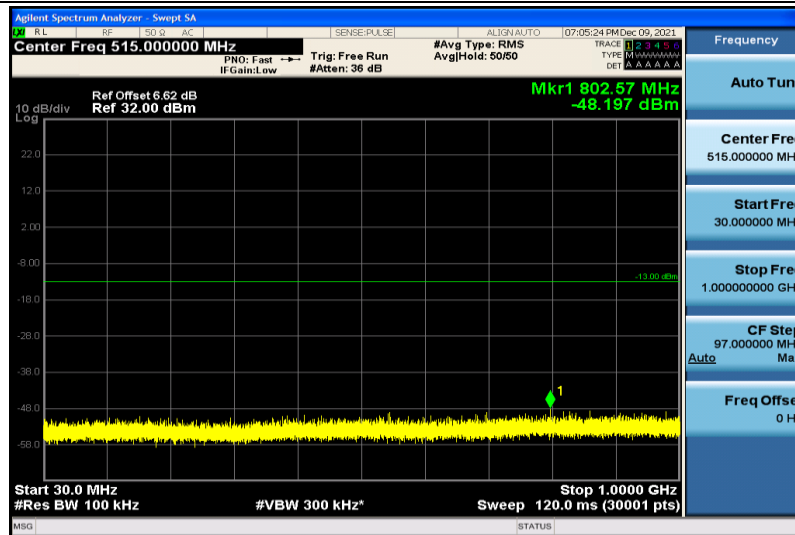
Band4-10MHz-64QAM-20350-1RB#0-30~1000MHz
