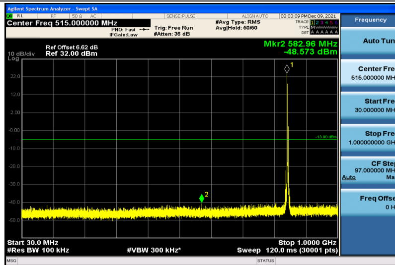
Band5-5MHz-64QAM-20625-1RB#0-30~1000MHz
