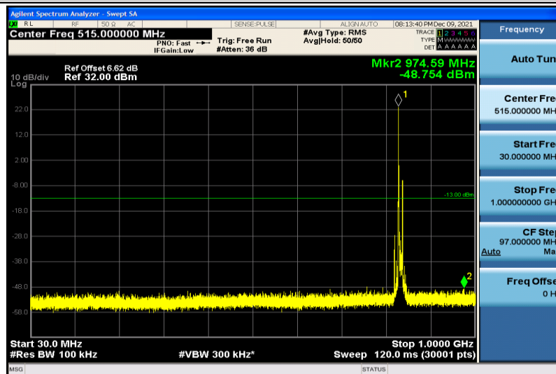
Band5-10MHz-64QAM-20525-1RB#0-30~1000MHz
