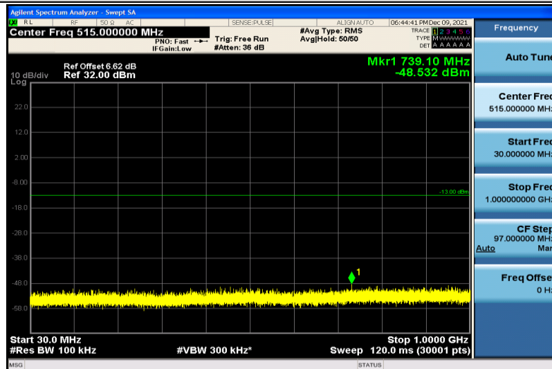
Band4-3MHz-64QAM-19965-1RB#0-30~1000MHz
