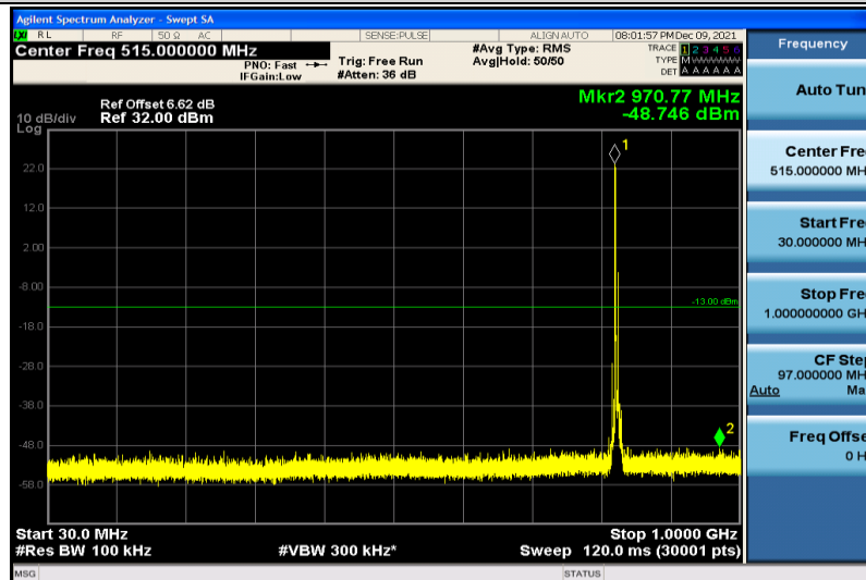
Band5-5MHz-64QAM-20425-1RB#0-30~1000MHz
