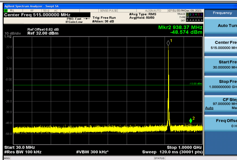
Band5-3MHz-64QAM-20415-1RB#0-30~1000MHz
