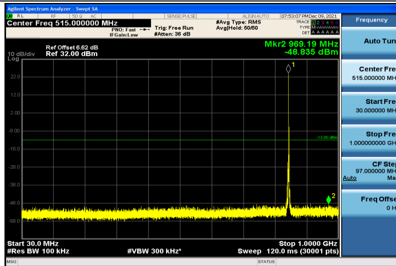
Band5-3MHz-64QAM-20635-1RB#0-30~1000MHz
