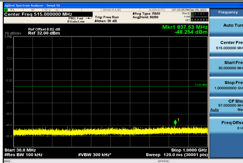
Band4-15MHz-64QAM-20025-1RB#0-30~1000MHz
