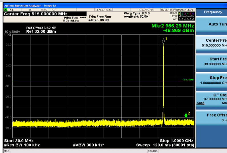
Band5-1.4MHz-64QAM-20525-1RB#0-30~1000MHz
