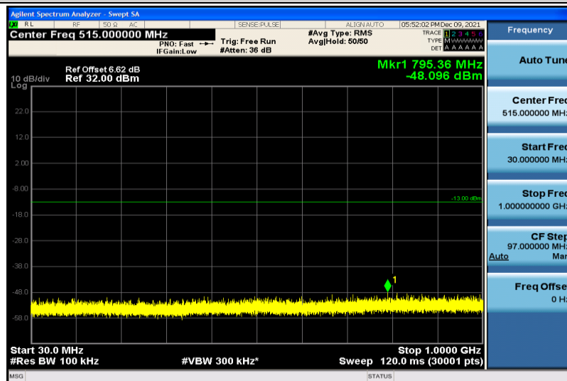
Band2-5MHz-64QAM-18900-1RB#0-30~1000MHz
