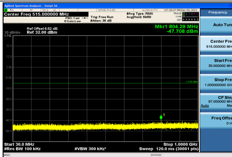
Band4-20MHz-64QAM-20175-1RB#0-30~1000MHz
