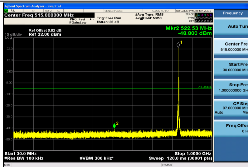
Band5-5MHz-64QAM-20525-1RB#0-30~1000MHz
