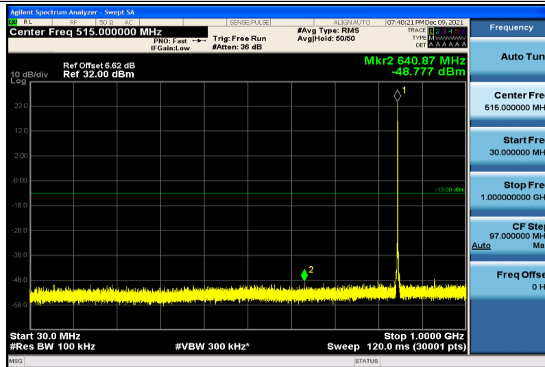
Band5-1.4MHz-64QAM-20643-1RB#0-30~1000MHz
