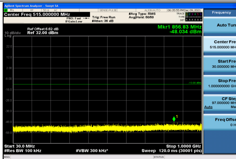
Band4-1.4MHz-64QAM-20175-1RB#0-30~1000MHz
