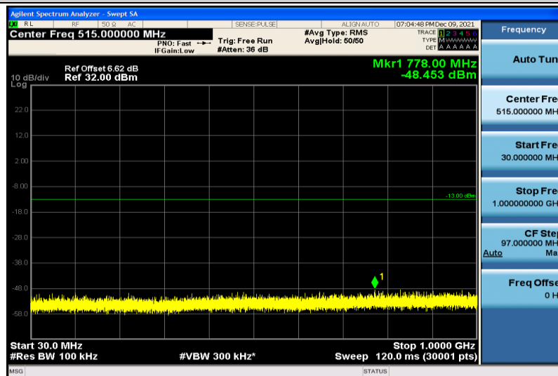
Band4-10MHz-64QAM-20175-1RB#0-30~1000MHz
