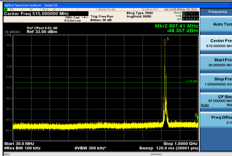
Band5-10MHz-64QAM-20450-1RB#0-30~1000MHz
