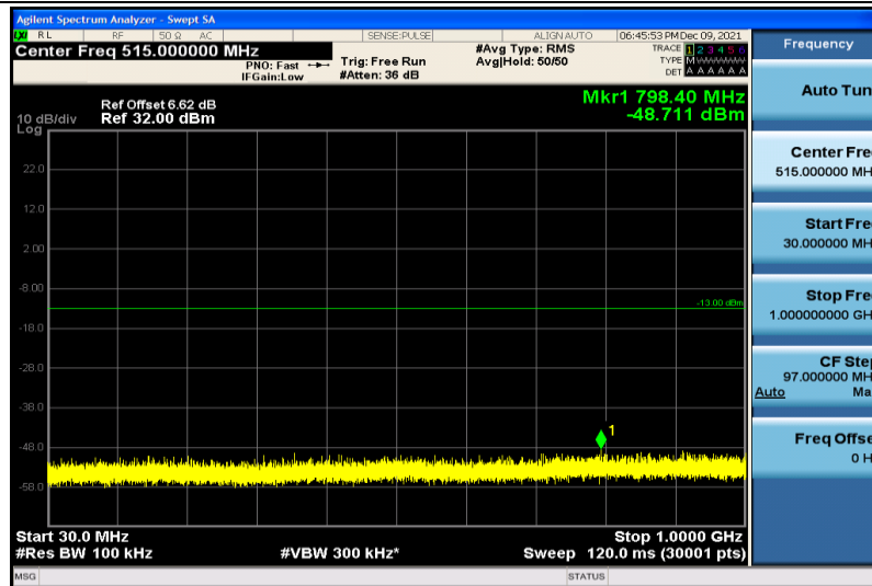
Band4-3MHz-64QAM-20385-1RB#0-30~1000MHz
