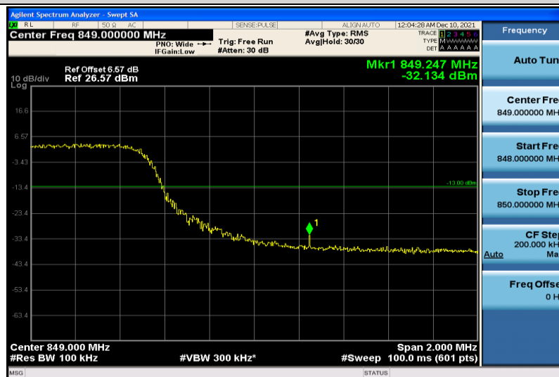
Band26-10MHz-64QAM-26990-50RB#0
