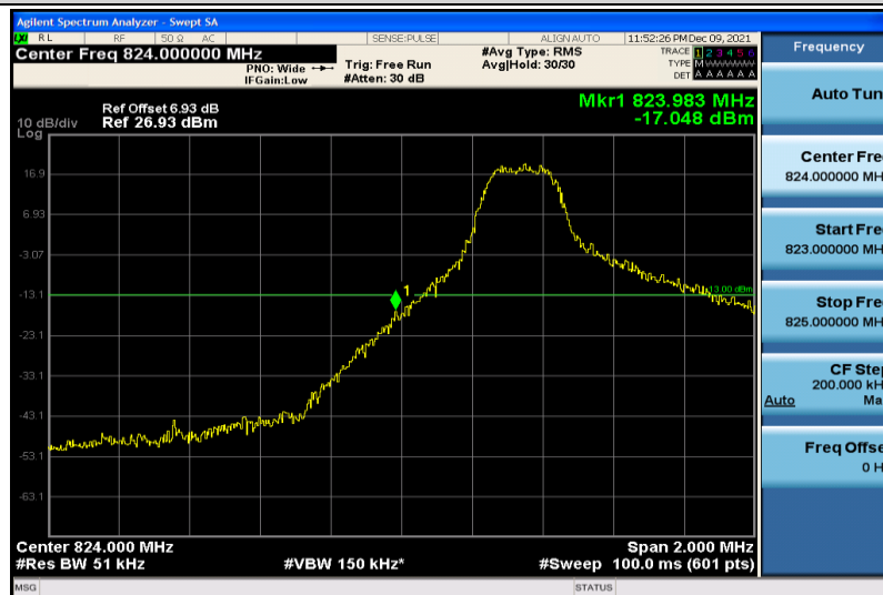
Band26-5MHz-64QAM-26815-1RB#0
