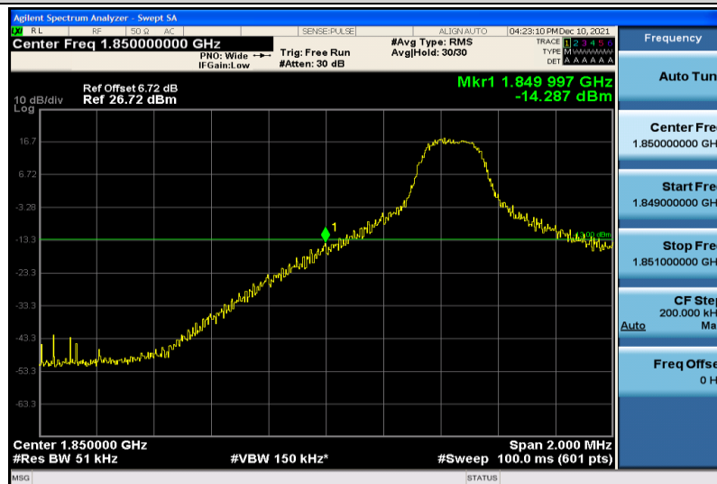
Band25-5MHz-64QAM-26065-1RB#0
