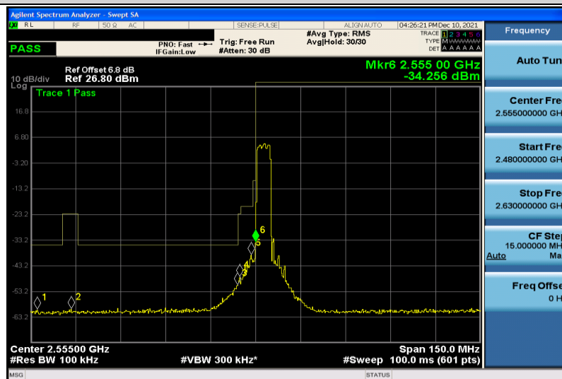
Band41-5MHz-64QAM-40265-25RB#0
