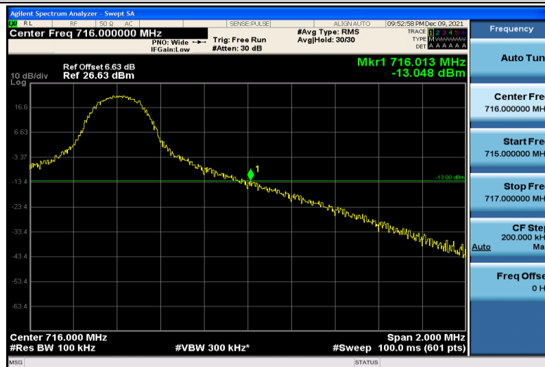
Band12-10MHz-64QAM-23130-1RB#49
