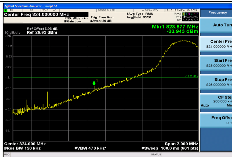
Band26-15MHz-64QAM-26865-1RB#0
