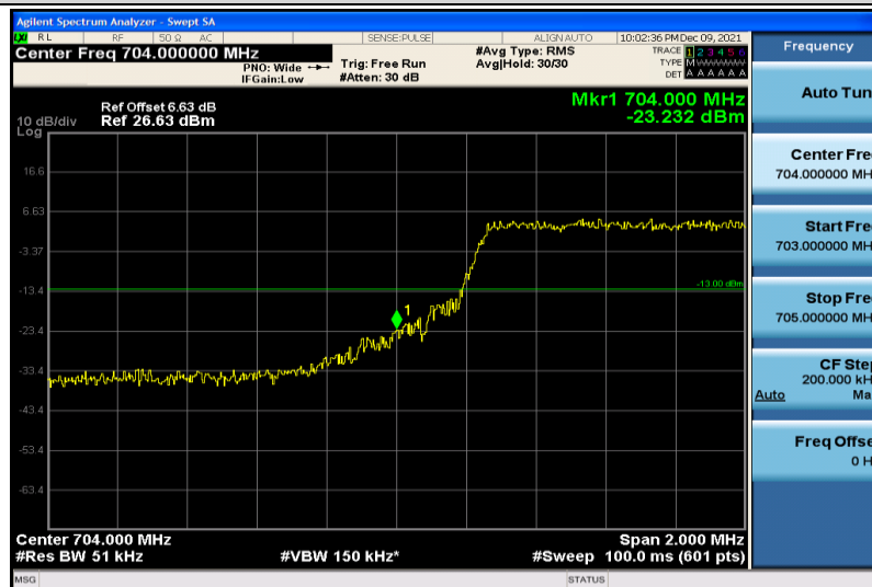
Band17-5MHz-64QAM-23755-25RB#0
