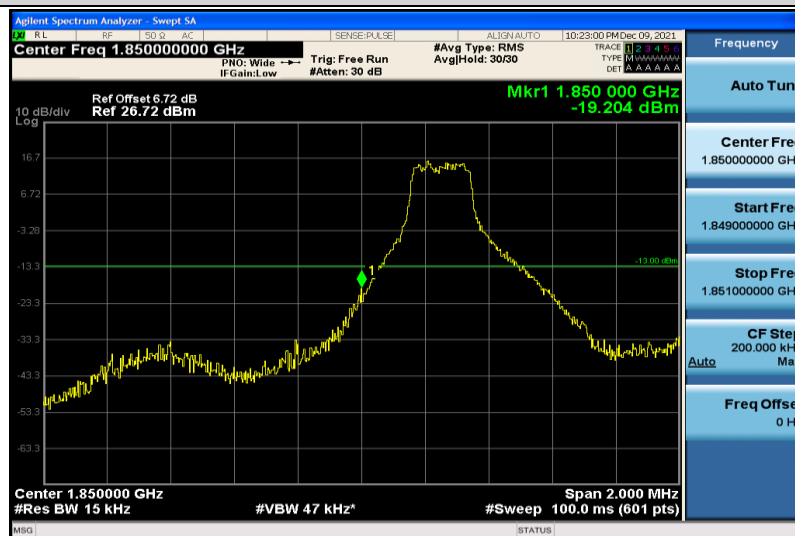
Band25-1.4MHz-64QAM-26047-1RB#0
