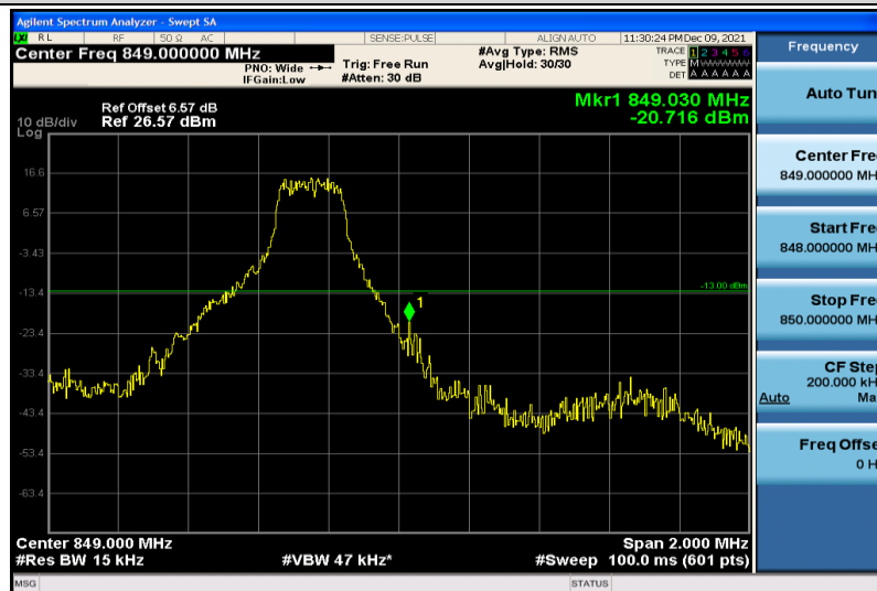
Band26-1.4MHz-64QAM-27033-1RB#5
