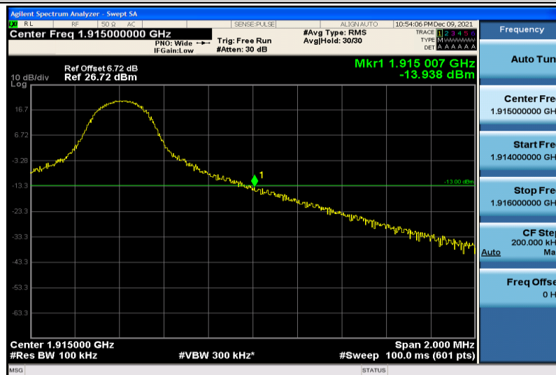
Band25-10MHz-64QAM-26640-1RB#49
