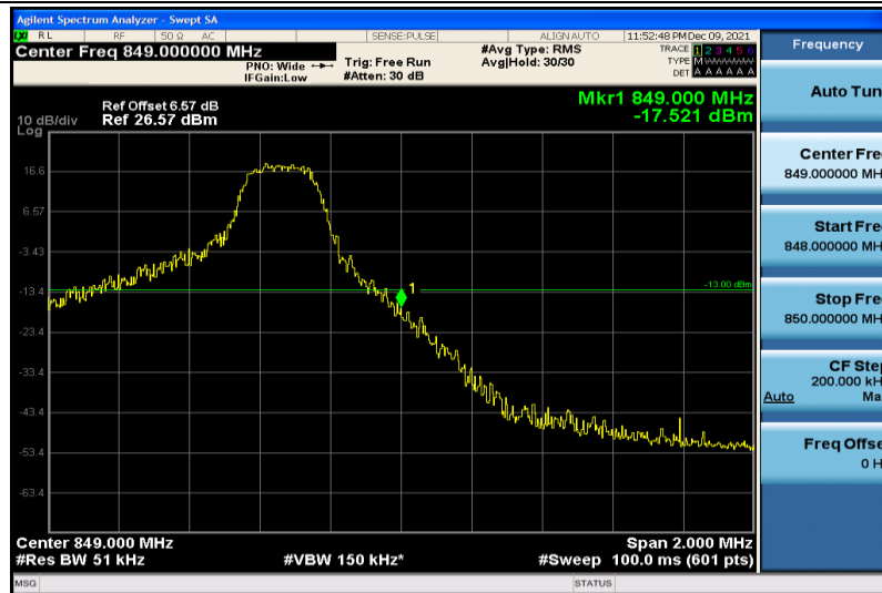
Band26-5MHz-64QAM-27015-1RB#24
