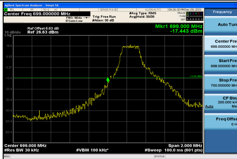
Band12-3MHz-64QAM-23025-1RB#0
