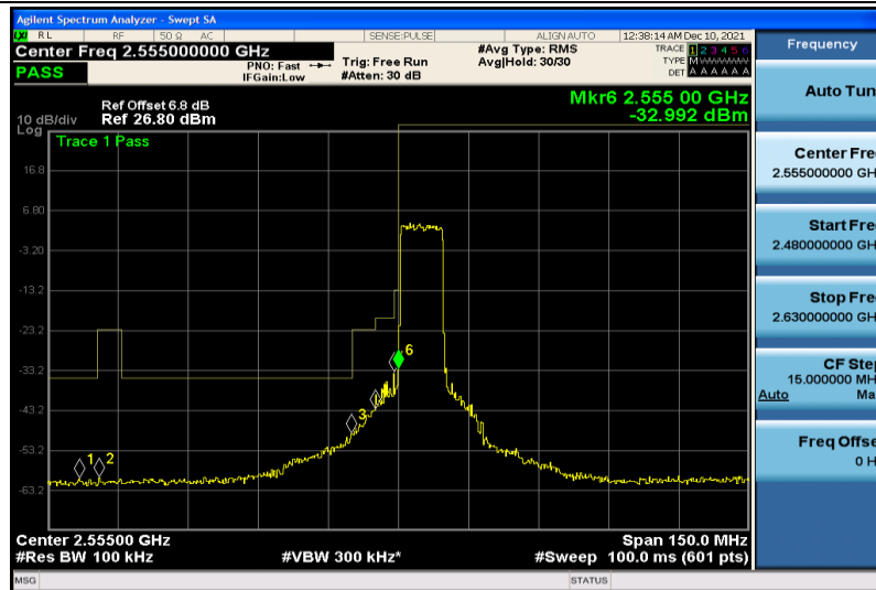
Band41-10MHz-64QAM-40290-50RB#0
