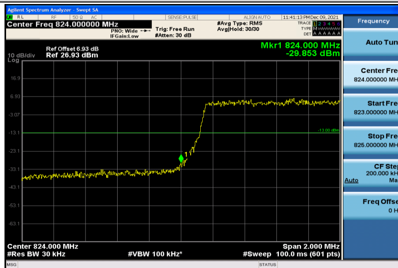
Band26-3MHz-64QAM-26805-15RB#0
