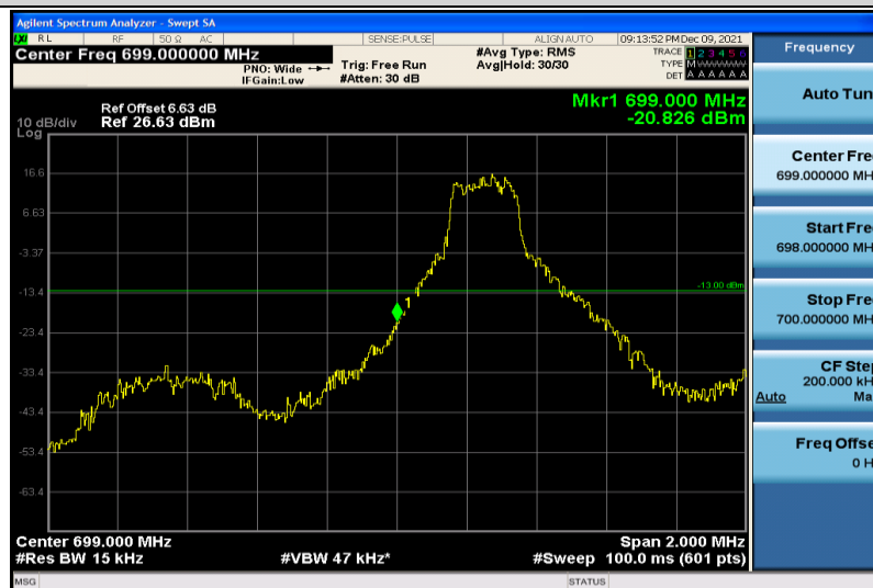
Band12-1.4MHz-64QAM-23017-1RB#0
