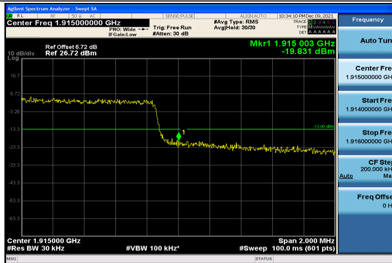
Band25-3MHz-64QAM-26675-15RB#0
