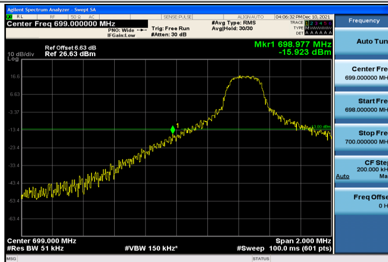
Band12-5MHz-64QAM-23035-1RB#0
