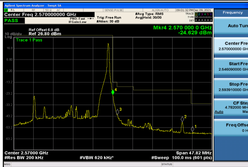
Band7-20MHz-64QAM-21350-1RB#99
