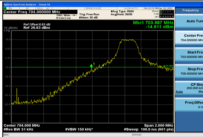
Band17-5MHz-64QAM-23755-1RB#0
