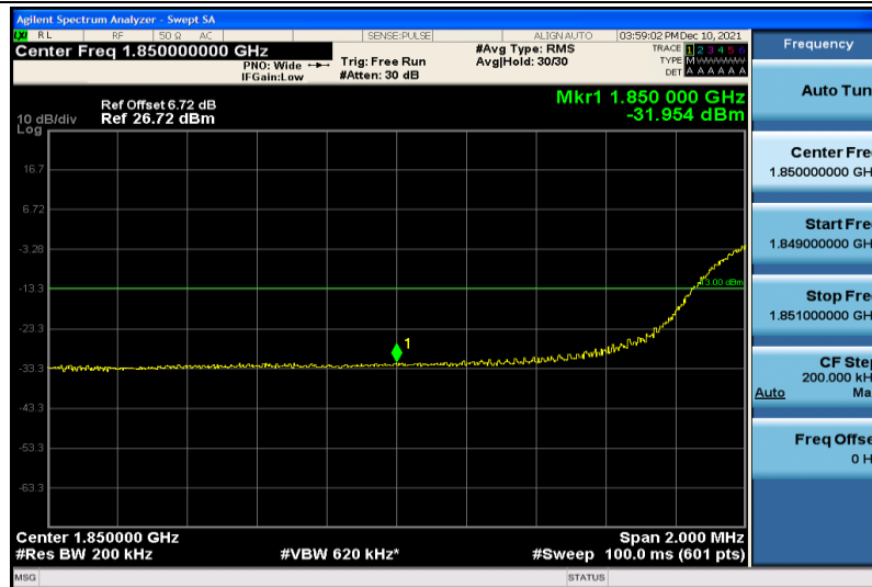
Band2-20MHz-64QAM-18700-100RB#0
