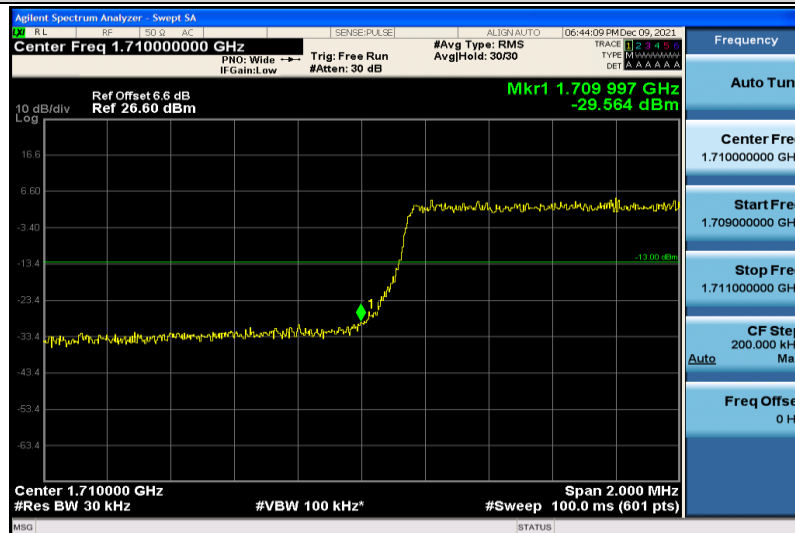
Band4-3MHz-64QAM-19965-15RB#0
