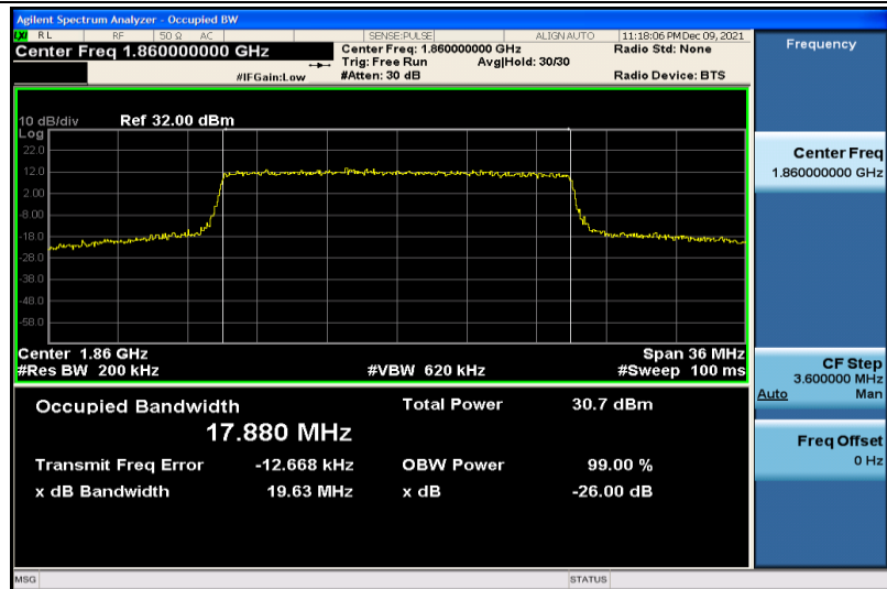
Band25-20MHz-64QAM-26140-100RB#0-17.880
