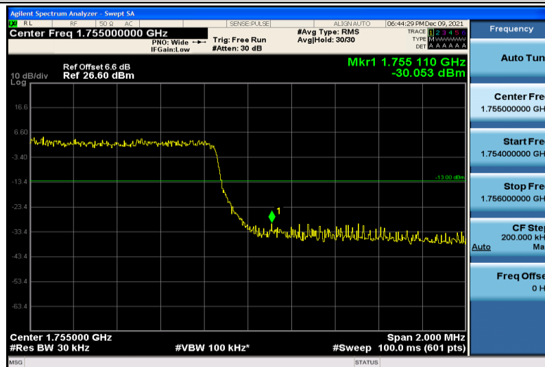
Band4-3MHz-64QAM-20385-15RB#0
