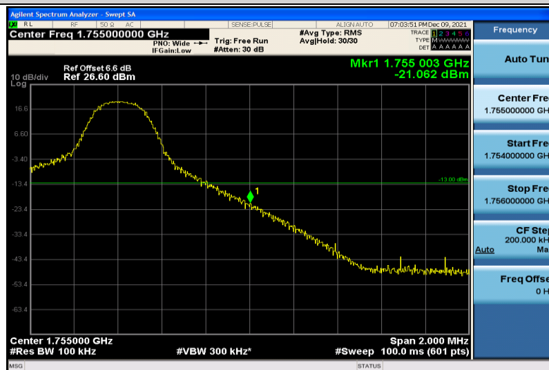
Band4-10MHz-64QAM-20350-1RB#49
