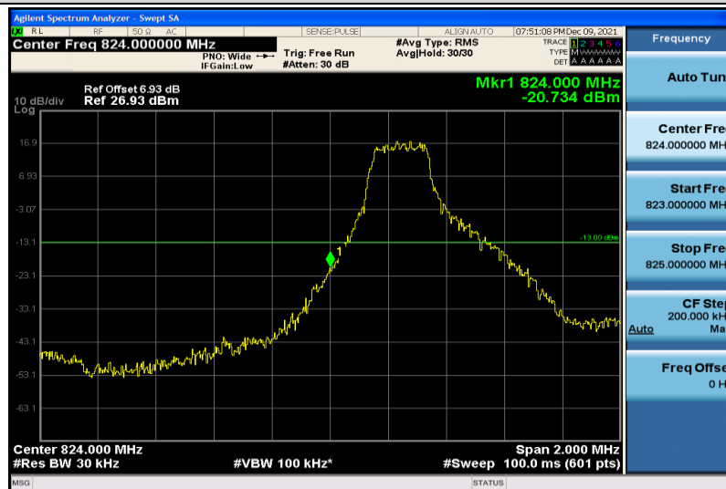
Band5-3MHz-64QAM-20415-1RB#0
