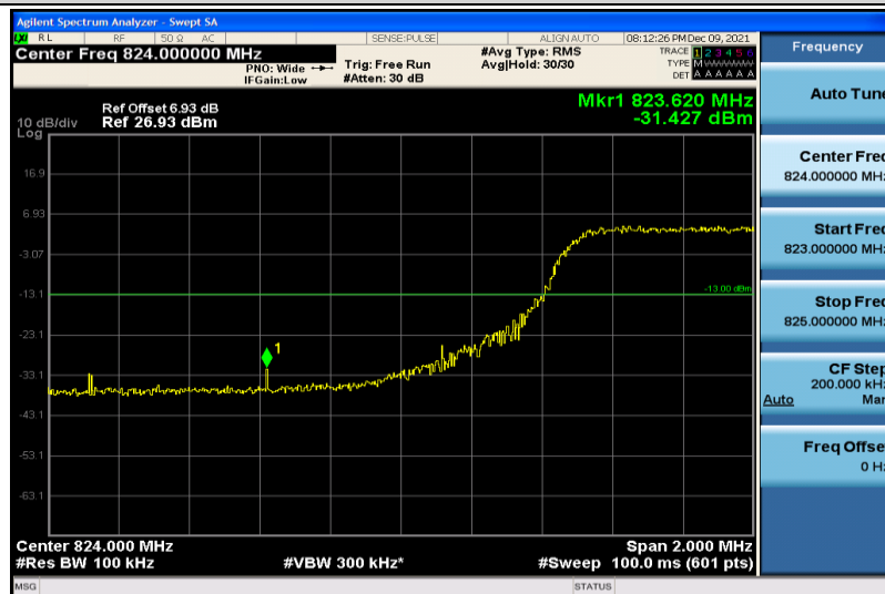
Band5-10MHz-64QAM-20450-50RB#0
