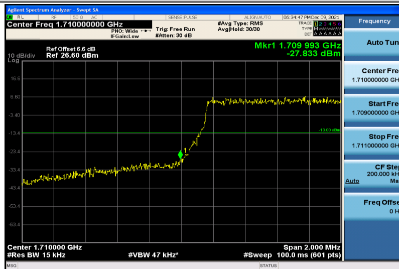
Band4-1.4MHz-64QAM-19957-6RB#0
