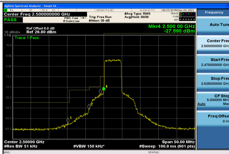
Band7-5MHz-64QAM-20775-25RB#0
