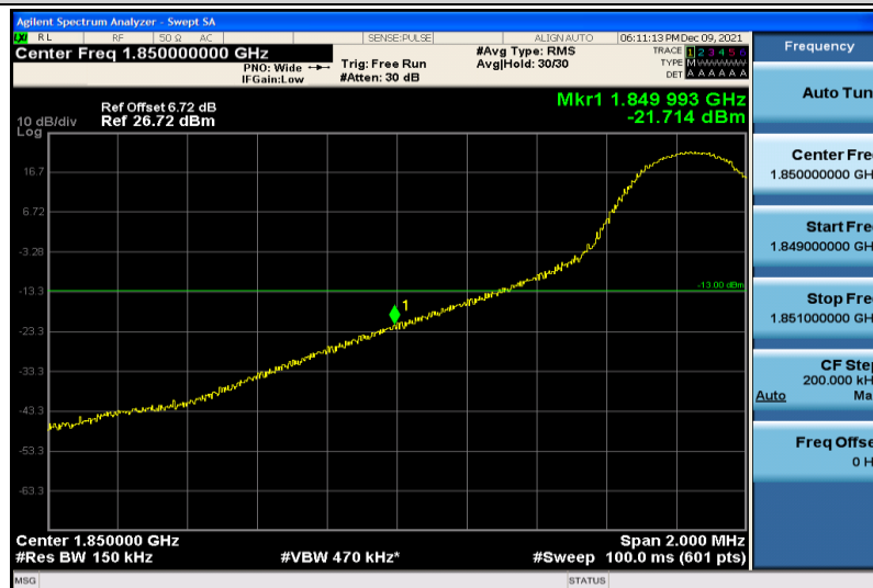
Band2-15MHz-64QAM-18675-1RB#0
