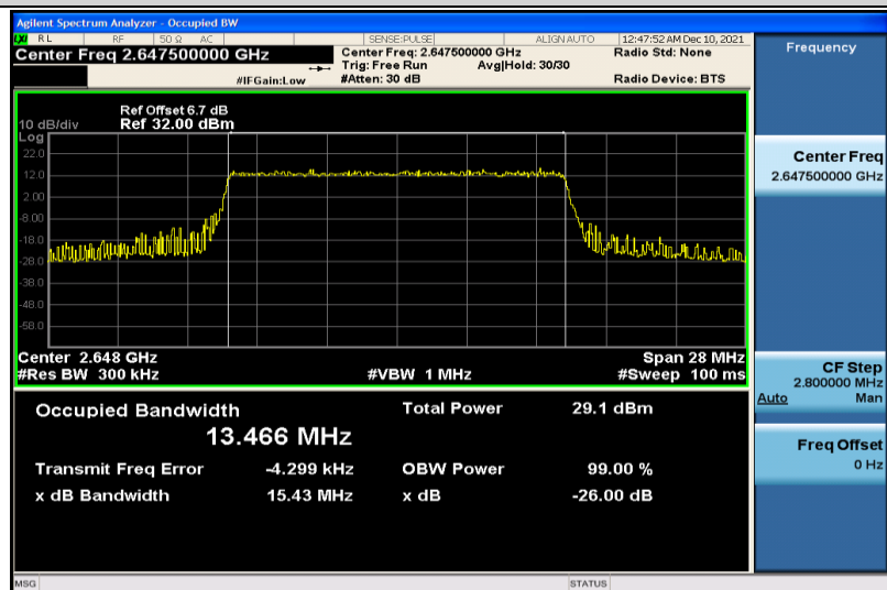
Band41-15MHz-64QAM-41165-75RB#0-13.466
