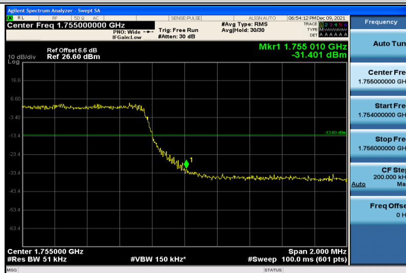
Band4-5MHz-64QAM-20375-25RB#0
