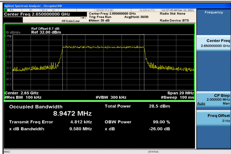
Band41-10MHz-64QAM-41190-50RB#0-8.9472
