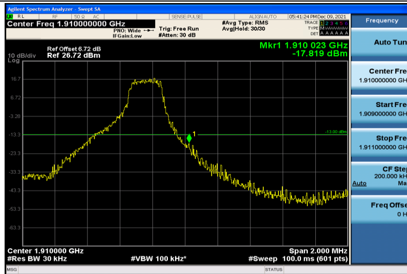
Band2-3MHz-64QAM-19185-1RB#14
