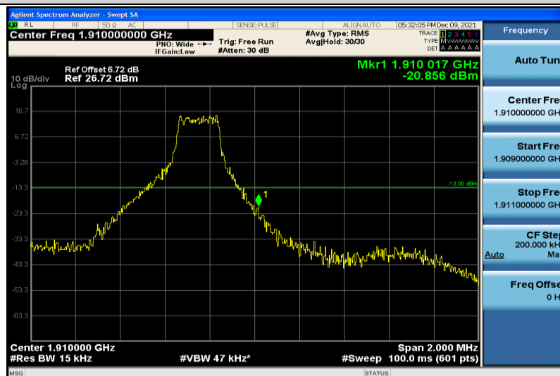
Band2-1.4MHz-64QAM-19193-1RB#5
