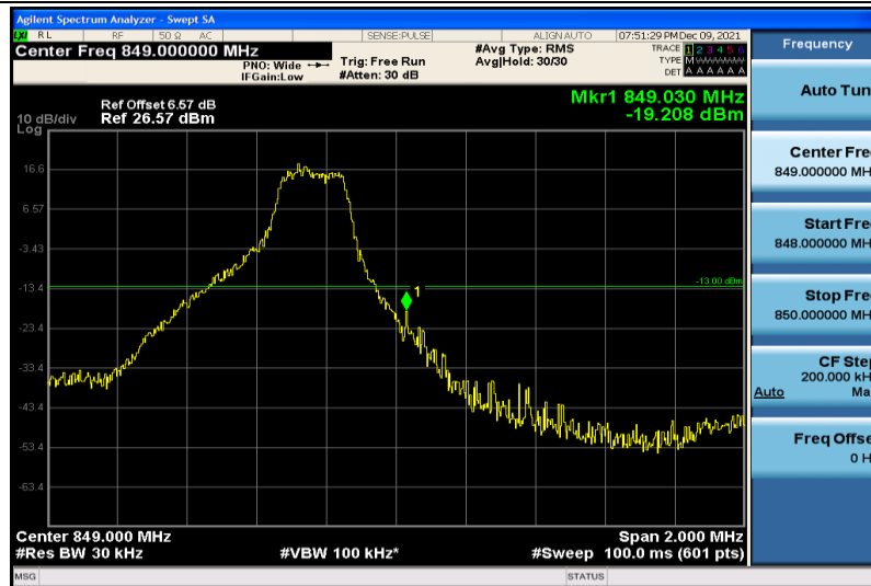
Band5-3MHz-64QAM-20635-1RB#14
