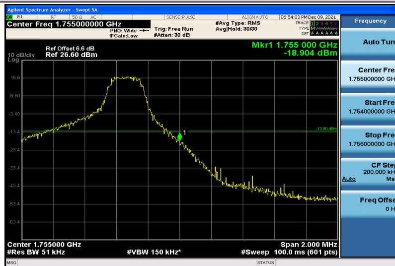
Band4-5MHz-64QAM-20375-1RB#24
