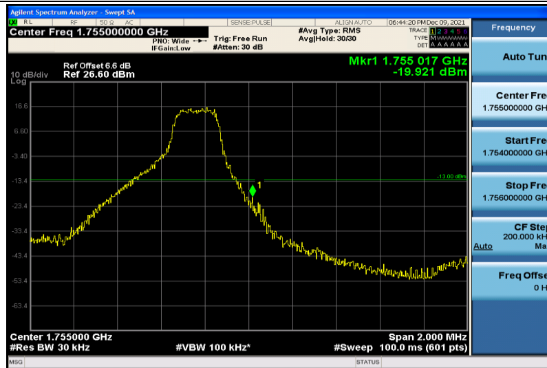
Band4-3MHz-64QAM-20385-1RB#14
