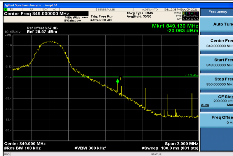
Band5-10MHz-64QAM-20600-1RB#49
