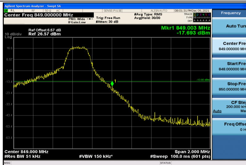
Band5-5MHz-64QAM-20625-1RB#24
