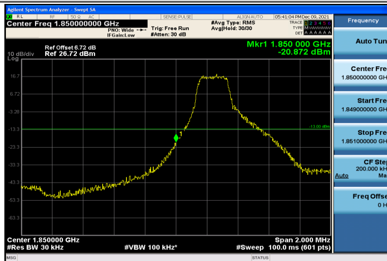
Band2-3MHz-64QAM-18615-1RB#0
