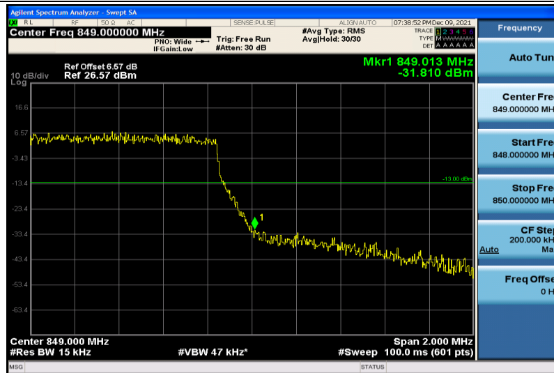
Band5-1.4MHz-64QAM-20643-6RB#0
