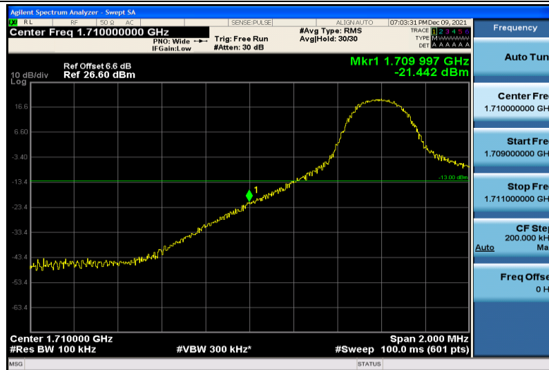
Band4-10MHz-64QAM-20000-1RB#0
