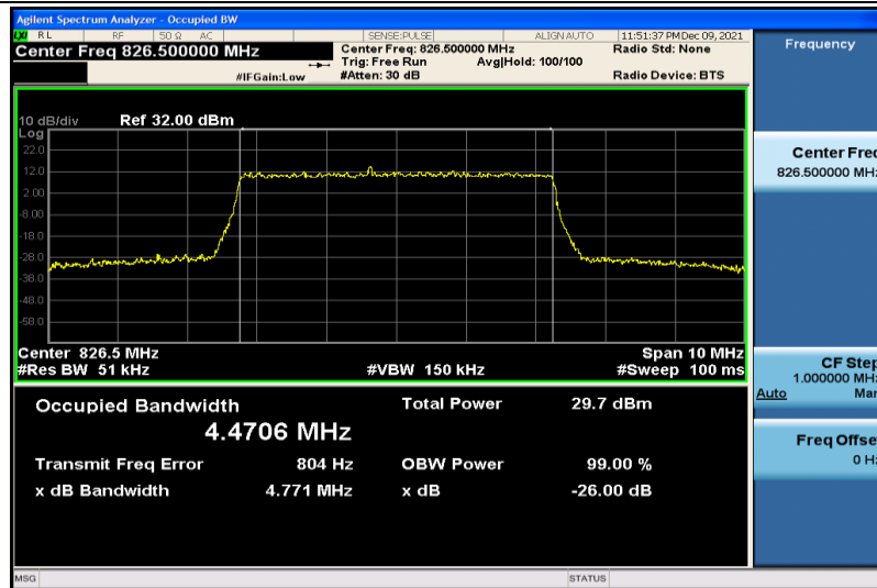
Band26-5MHz-64QAM-26815-25RB#0-4.4706
