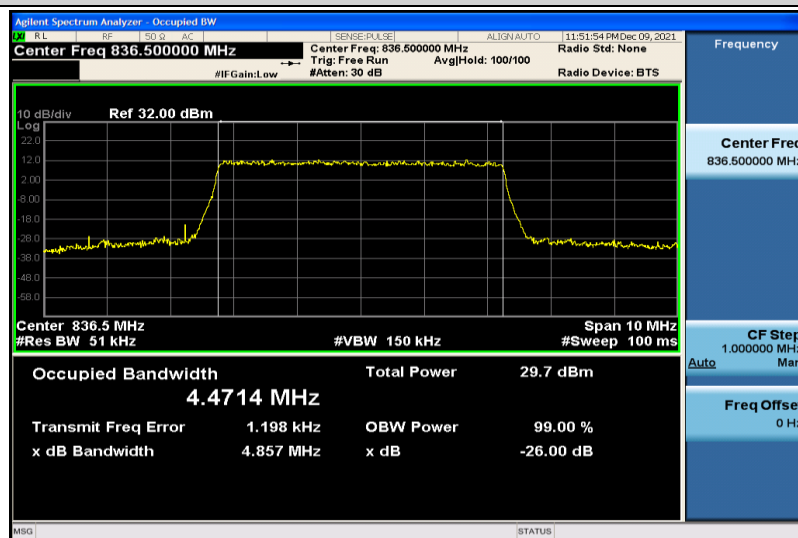
Band26-5MHz-64QAM-26915-25RB#0-4.4714
