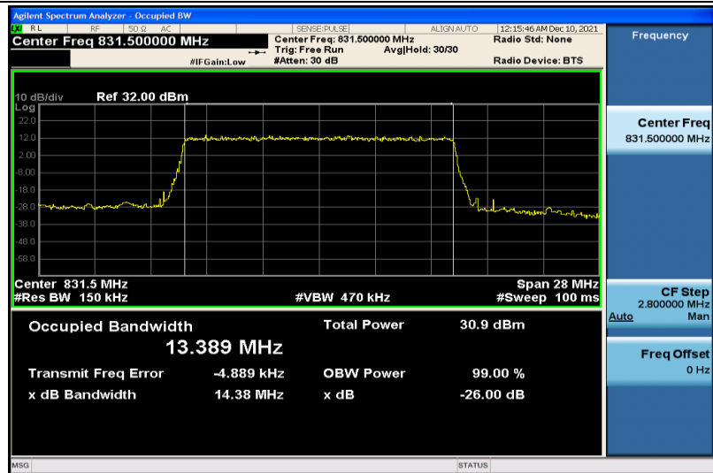
Band26-15MHz-64QAM-26865-75RB#0-13.389
