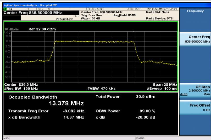
Band26-15MHz-64QAM-26915-75RB#0-13.378
