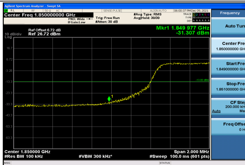
Band2-10MHz-64QAM-18650-50RB#0
