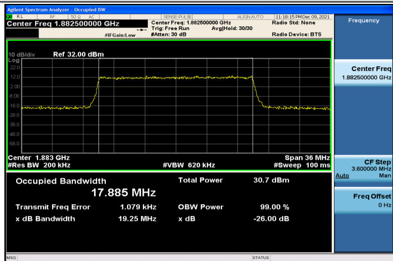
Band25-20MHz-64QAM-26365-100RB#0-17.885
