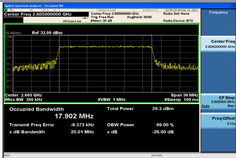
Band41-20MHz-64QAM-40740-100RB#0-17.902
