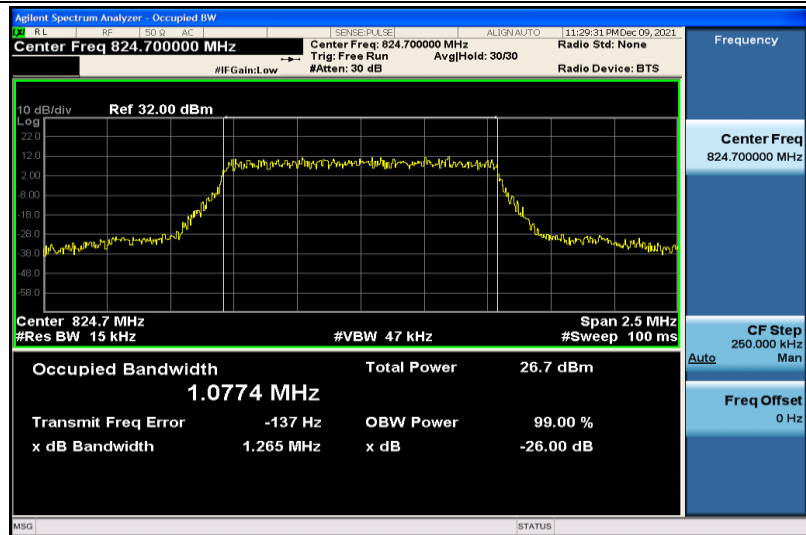
Band26-1.4MHz-64QAM-26797-6RB#0-1.0774
