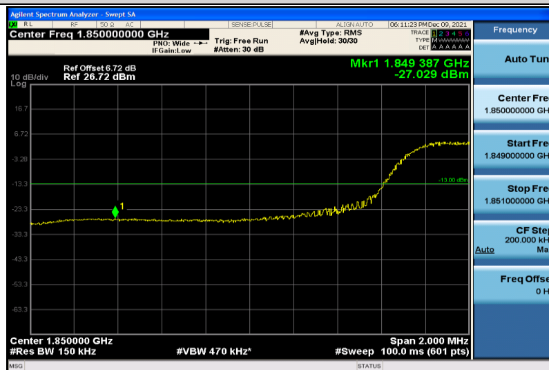
Band2-15MHz-64QAM-18675-75RB#0
