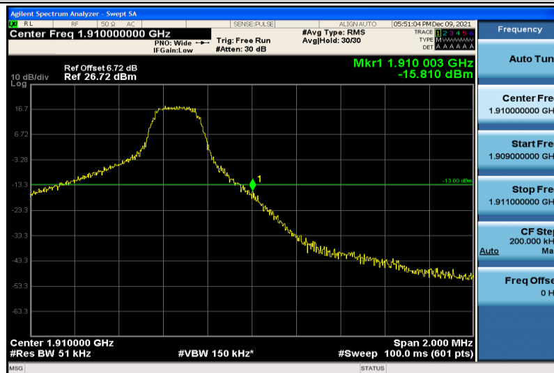
Band2-5MHz-64QAM-19175-1RB#24
