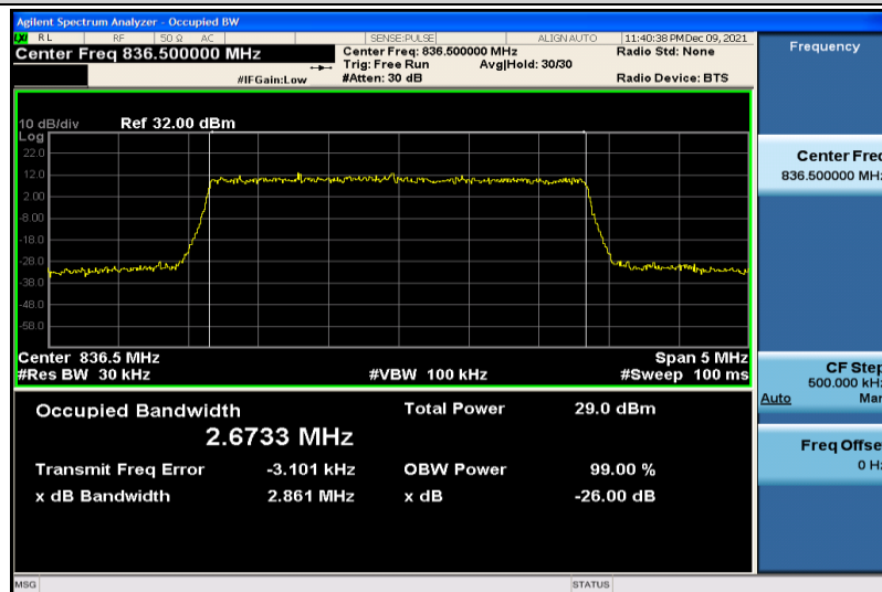
Band26-3MHz-64QAM-26915-15RB#0-2.6733
