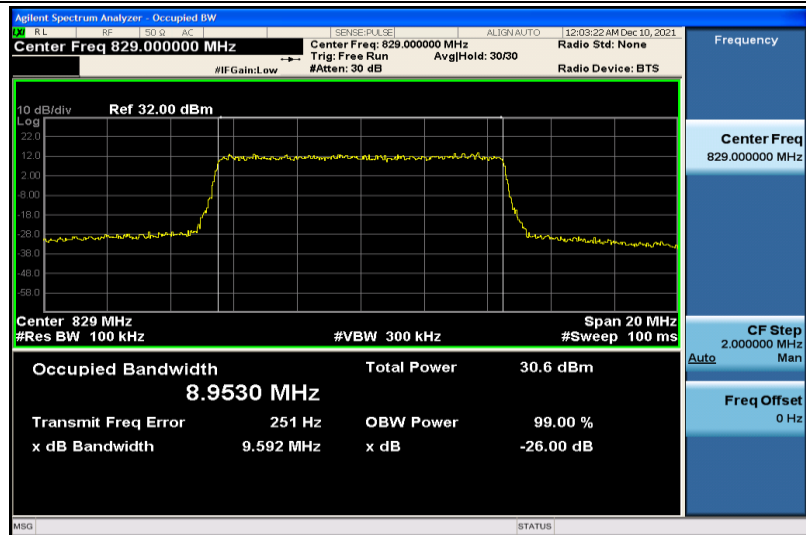
Band26-10MHz-64QAM-26840-50RB#0-8.9530
