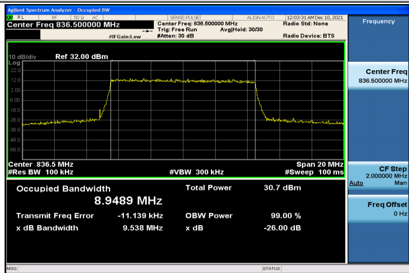
Band26-10MHz-64QAM-26915-50RB#0-8.9489
