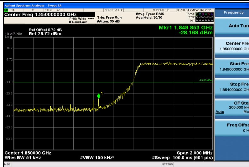
Band2-5MHz-64QAM-18625-25RB#0
