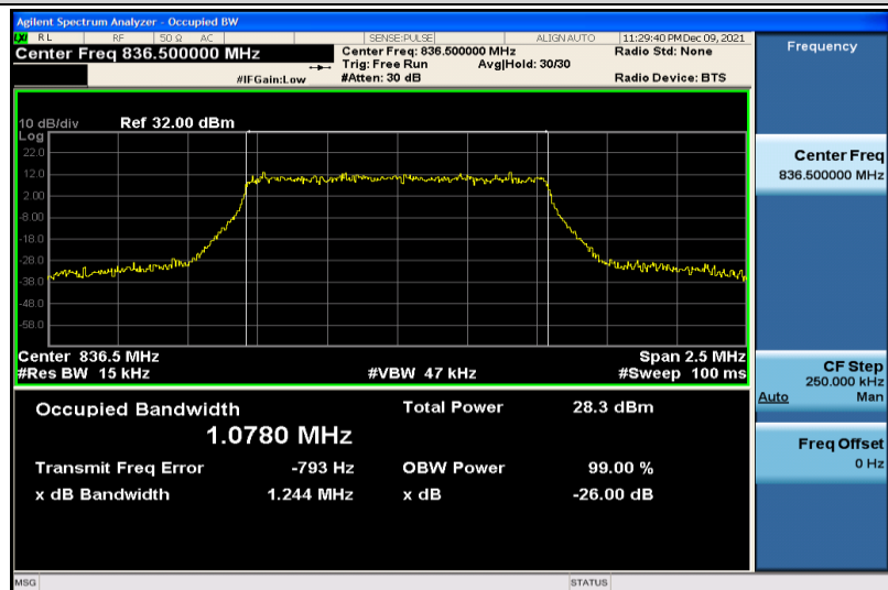
Band26-1.4MHz-64QAM-26915-6RB#0-1.0780
