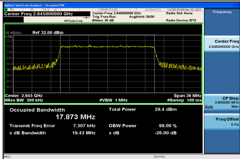
Band41-20MHz-64QAM-41140-100RB#0-17.873
