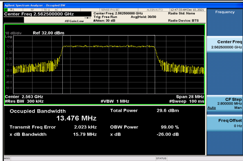
Band41-15MHz-64QAM-40315-75RB#0-13.476
