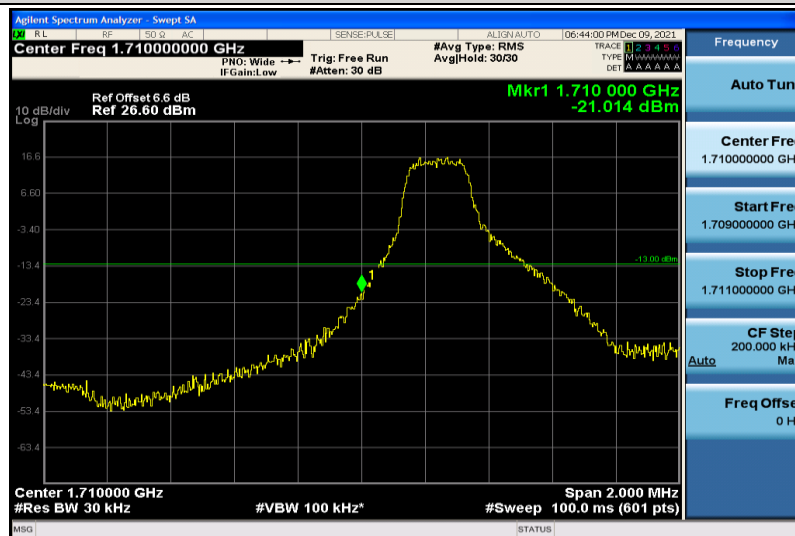
Band4-3MHz-64QAM-19965-1RB#0
