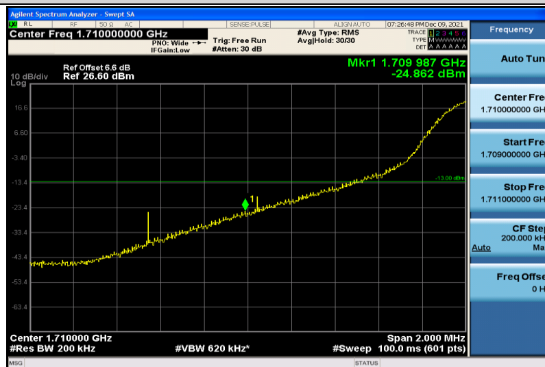
Band4-20MHz-64QAM-20050-1RB#0
