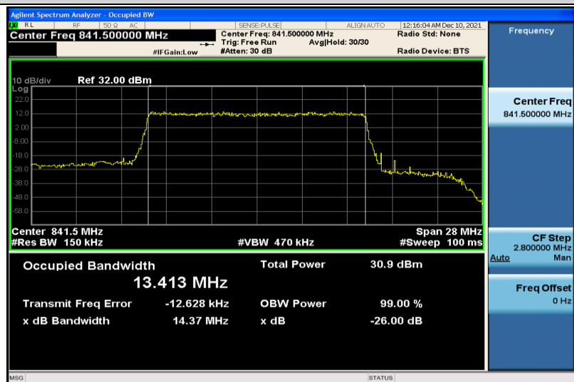
Band26-15MHz-64QAM-26965-75RB#0-13.413
