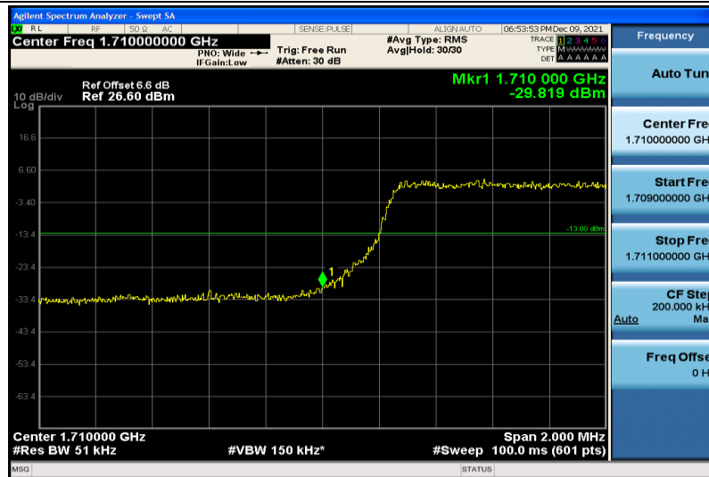
Band4-5MHz-64QAM-19975-25RB#0
