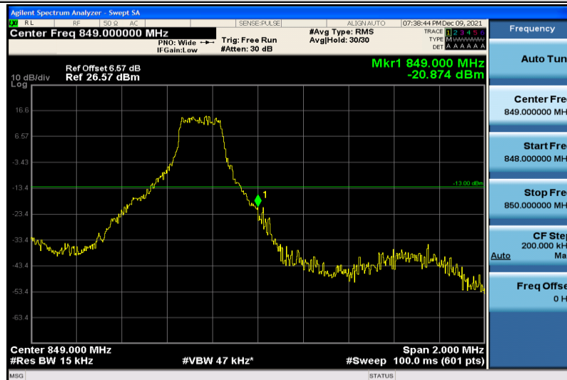
Band5-1.4MHz-64QAM-20643-1RB#5
