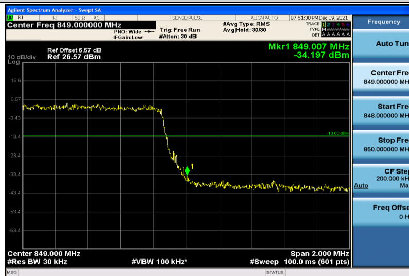
Band5-3MHz-64QAM-20635-15RB#0
