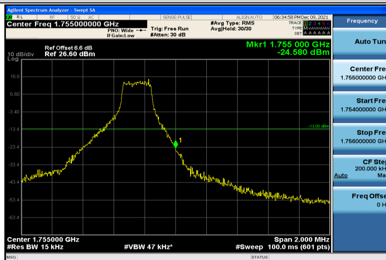
Band4-1.4MHz-64QAM-20393-1RB#5
