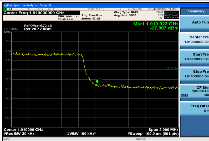
Band2-3MHz-64QAM-19185-15RB#0
