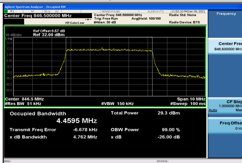
Band26-5MHz-64QAM-27015-25RB#0-4.4595
