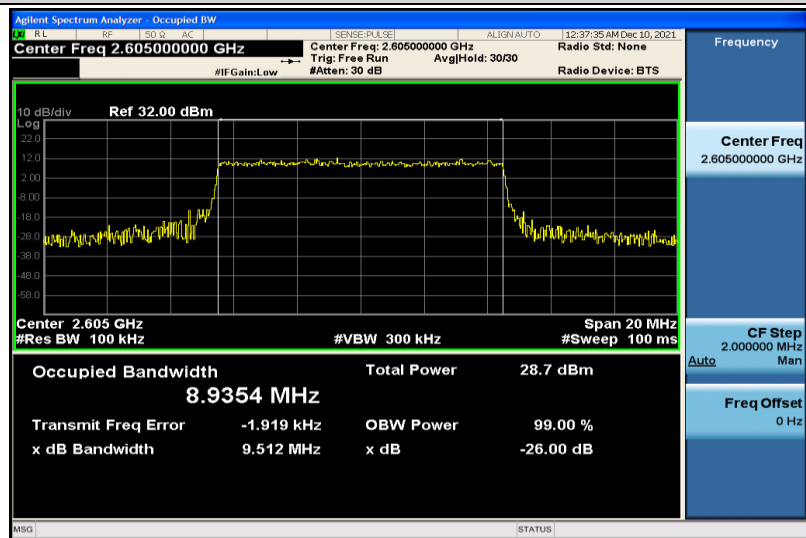
Band41-10MHz-64QAM-40740-50RB#0-8.9354
