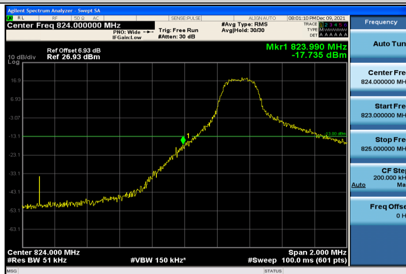
Band5-5MHz-64QAM-20425-1RB#0
