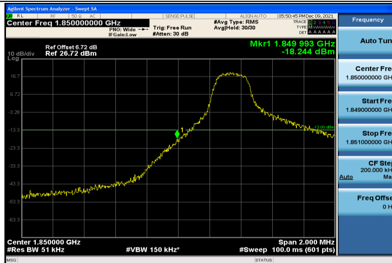
Band2-5MHz-64QAM-18625-1RB#0
