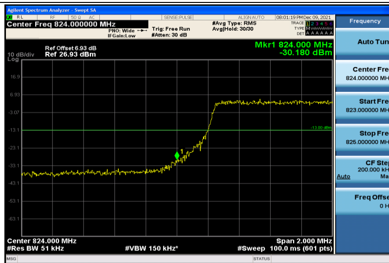
Band5-5MHz-64QAM-20425-25RB#0
