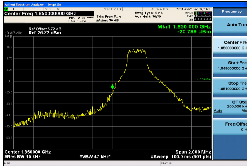
Band2-1.4MHz-64QAM-18607-1RB#0
