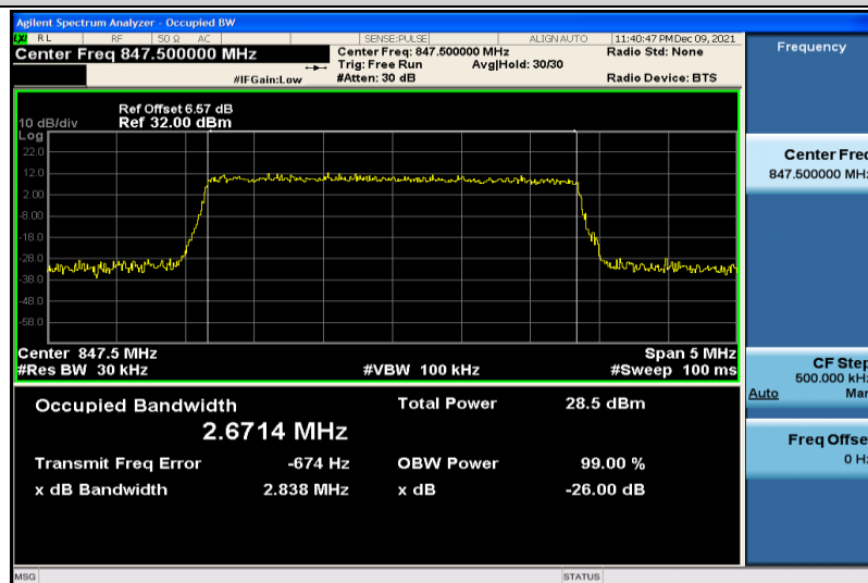
Band26-3MHz-64QAM-27025-15RB#0-2.6714
