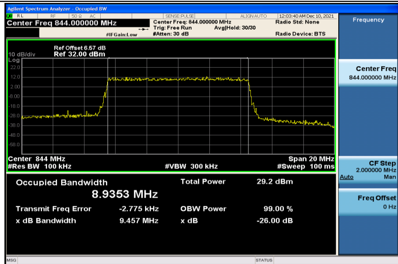
Band26-10MHz-64QAM-26990-50RB#0-8.9353
