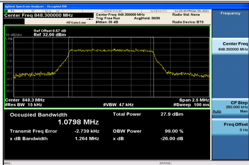
Band26-1.4MHz-64QAM-27033-6RB#0-1.0798
