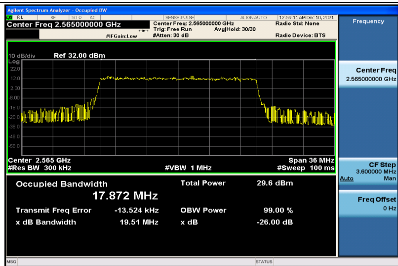
Band41-20MHz-64QAM-40340-100RB#0-17.872
