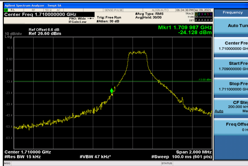
Band4-1.4MHz-64QAM-19957-1RB#0
