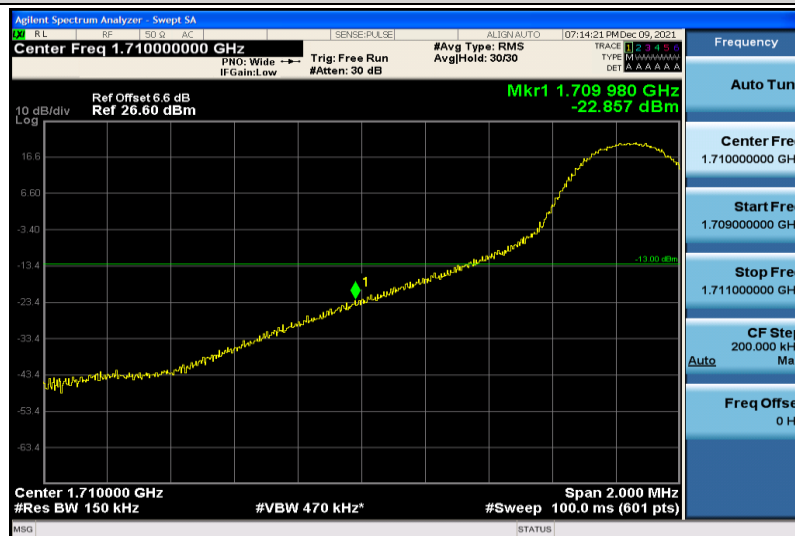
Band4-15MHz-64QAM-20025-1RB#0
