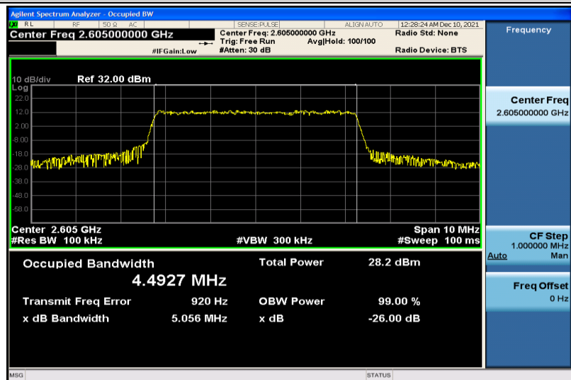
Band41-5MHz-64QAM-40740-25RB#0-4.4927
