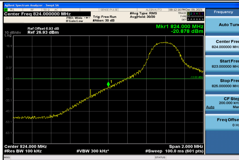
Band5-10MHz-64QAM-20450-1RB#0
