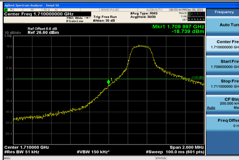
Band4-5MHz-64QAM-19975-1RB#0
