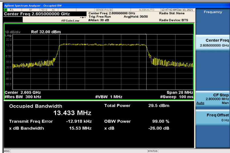
Band41-15MHz-64QAM-40740-75RB#0-13.433
