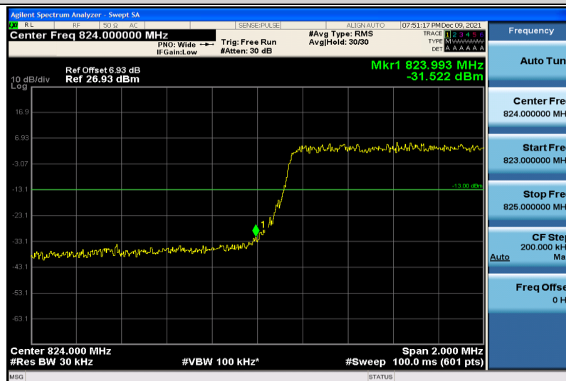
Band5-3MHz-64QAM-20415-15RB#0
