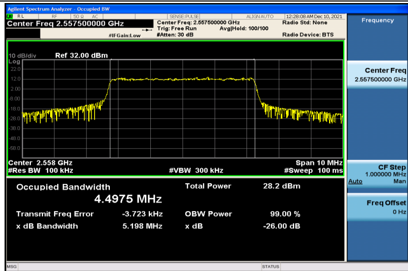
Band41-5MHz-64QAM-40265-25RB#0-4.4975
