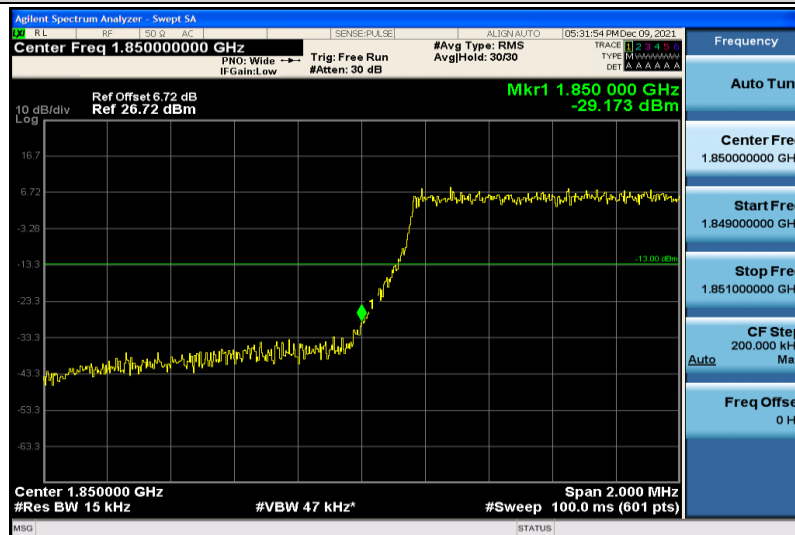
Band2-1.4MHz-64QAM-18607-6RB#0
