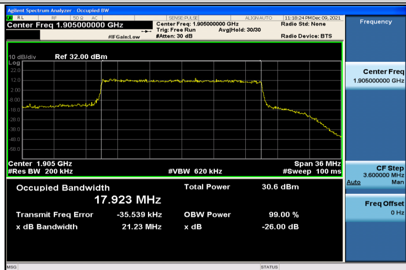
Band25-20MHz-64QAM-26590-100RB#0-17.923
