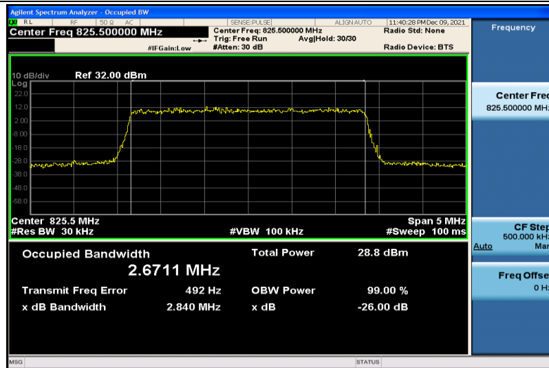
Band26-3MHz-64QAM-26805-15RB#0-2.6711
