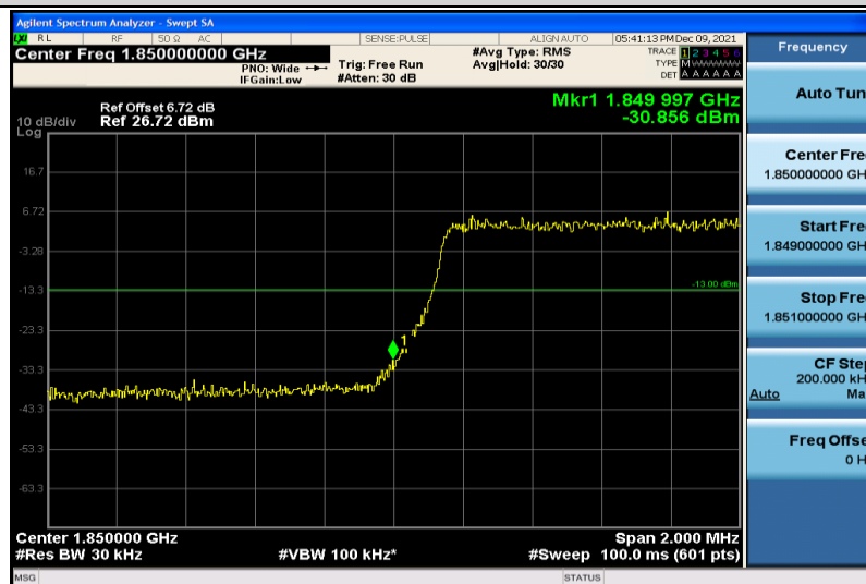
Band2-3MHz-64QAM-18615-15RB#0
