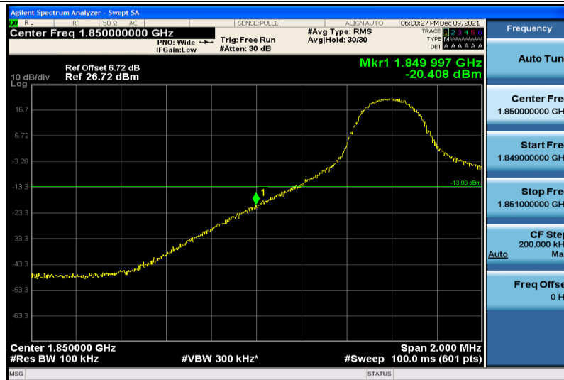
Band2-10MHz-64QAM-18650-1RB#0
