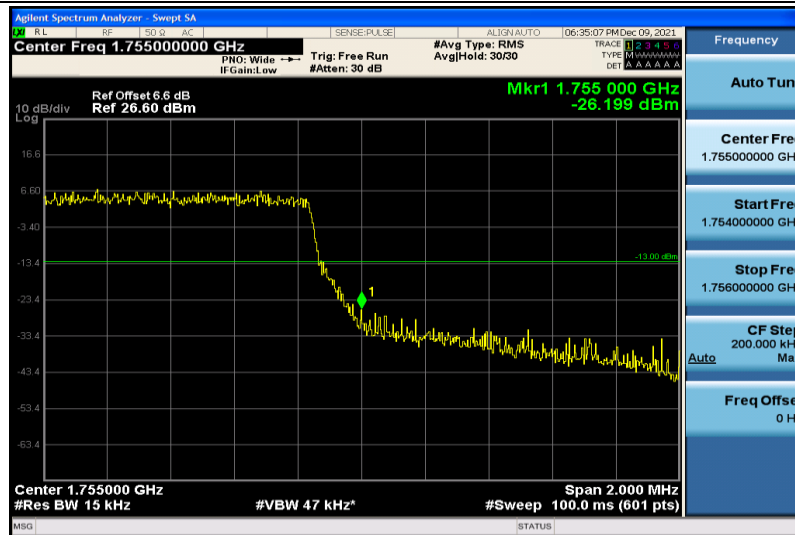
Band4-1.4MHz-64QAM-20393-6RB#0
