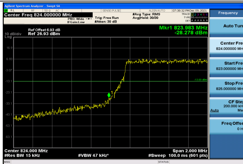
Band5-1.4MHz-64QAM-20407-6RB#0
