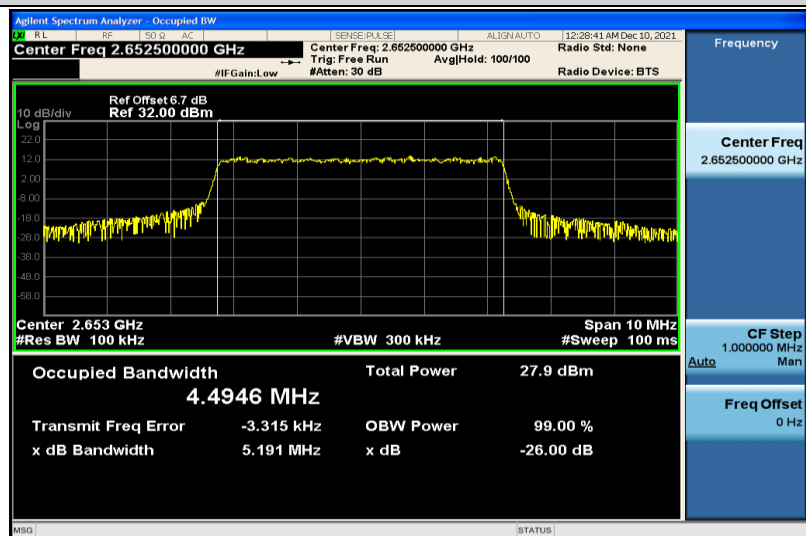
Band41-5MHz-64QAM-41215-25RB#0-4.4946
