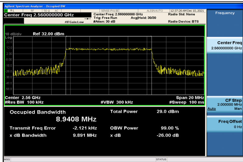
Band41-10MHz-64QAM-40290-50RB#0-8.9408
