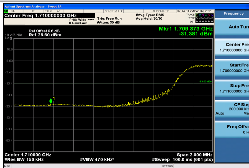
Band4-15MHz-64QAM-20025-75RB#0
