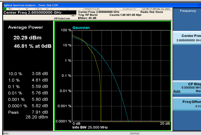
Band41-5MHz-64QAM-40740-1RB#0
