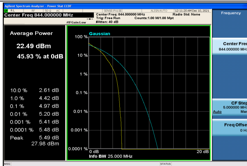
Band26-10MHz-64QAM-26990-1RB#0
