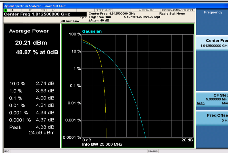
Band25-5MHz-64QAM-26665-25RB#0
