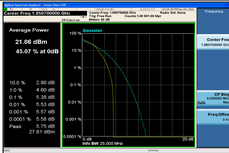
Band25-1.4MHz-64QAM-26047-1RB#0
