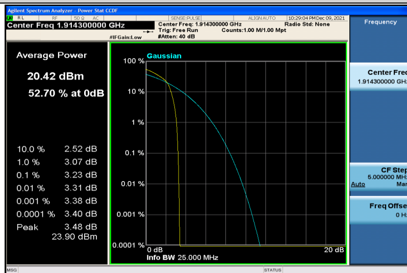
Band25-1.4MHz-64QAM-26683-6RB#0
