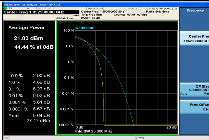
Band25-5MHz-64QAM-26065-1RB#0
