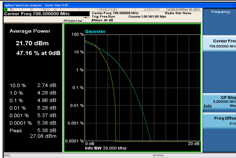
Band17-5MHz-64QAM-23755-1RB#0
