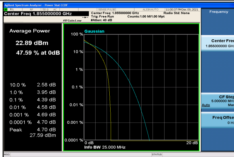
Band25-10MHz-64QAM-26090-1RB#0
