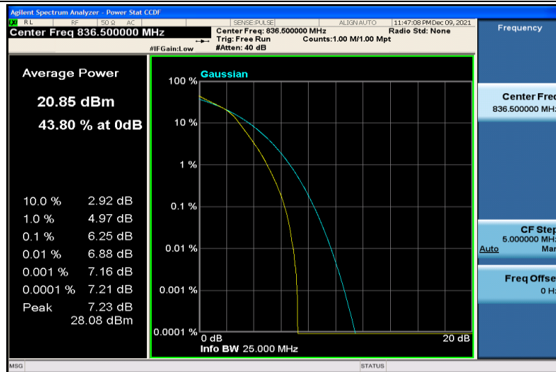
Band26-3MHz-64QAM-26915-15RB#0
