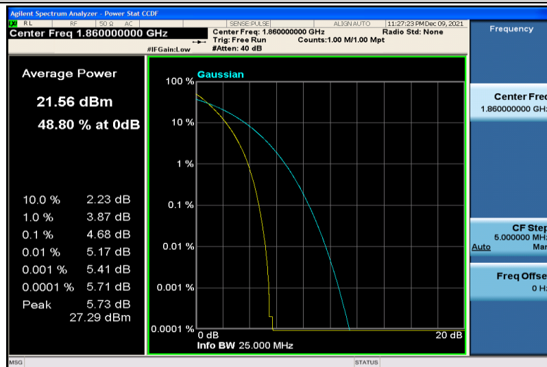
Band25-20MHz-64QAM-26140-100RB#0
