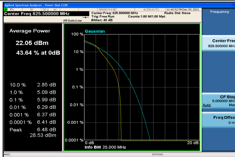
Band26-3MHz-64QAM-26805-1RB#0
