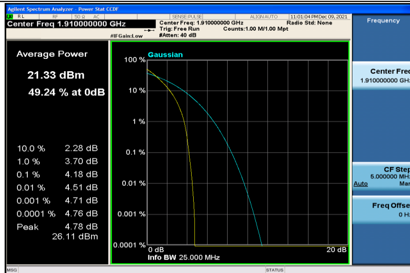
Band25-10MHz-64QAM-26640-50RB#0
