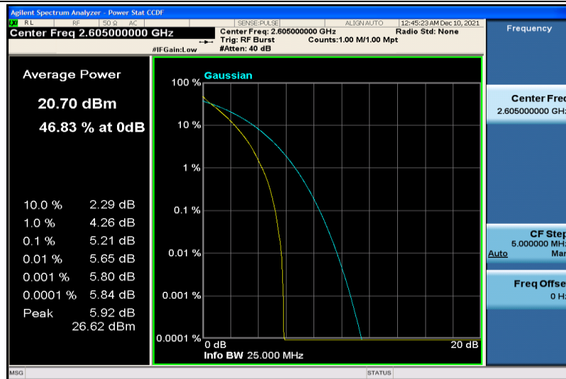
Band41-10MHz-64QAM-40740-50RB#0
