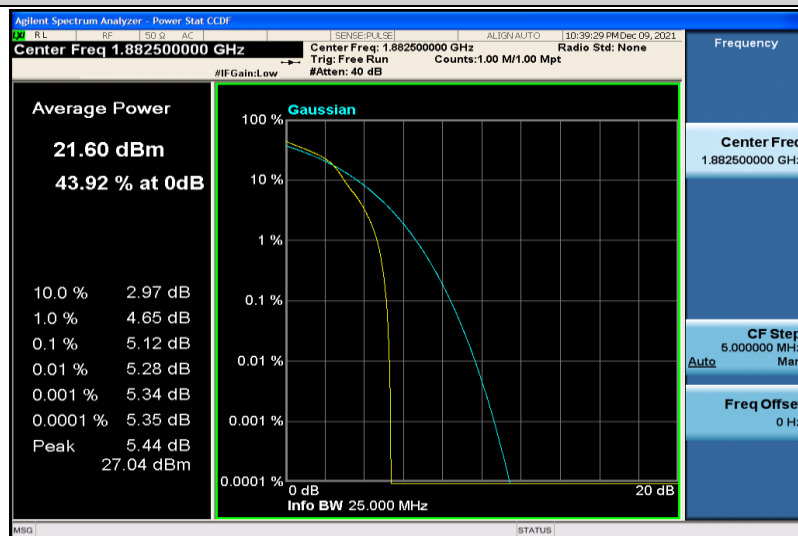
Band25-3MHz-64QAM-26365-1RB#0
