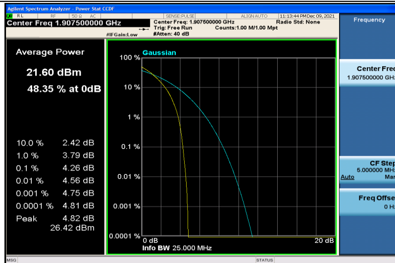
Band25-15MHz-64QAM-26615-75RB#0
