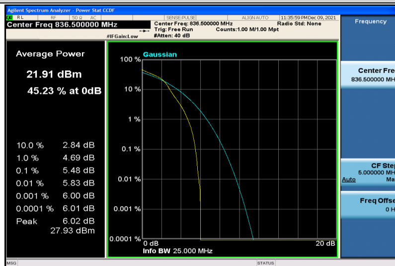
Band26-1.4MHz-64QAM-26915-1RB#0
