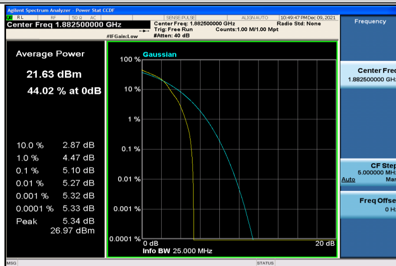
Band25-5MHz-64QAM-26365-1RB#0
