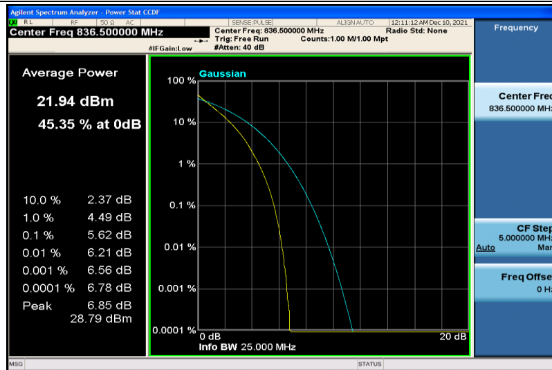
Band26-10MHz-64QAM-26915-50RB#0
