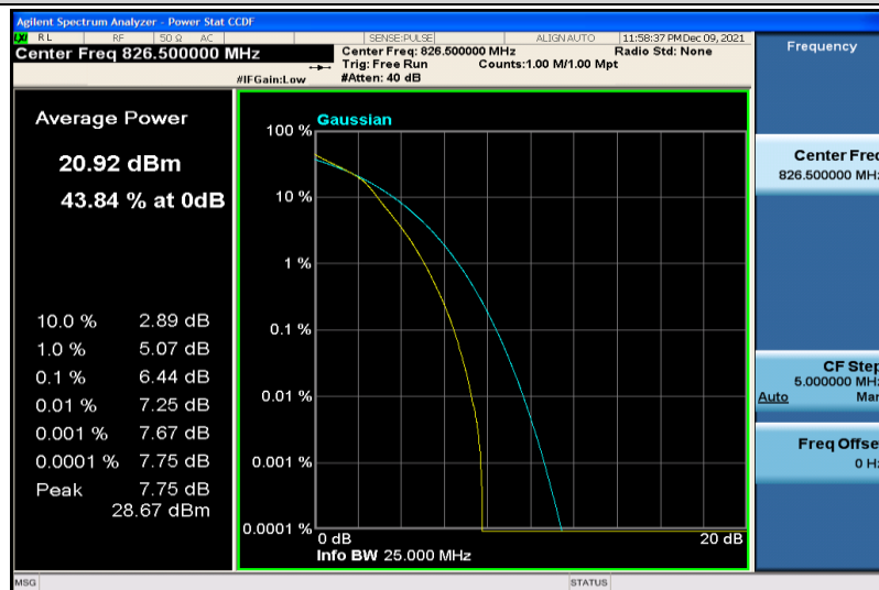
Band26-5MHz-64QAM-26815-25RB#0
