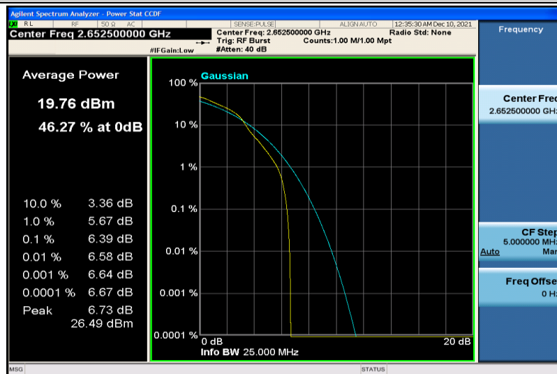
Band41-5MHz-64QAM-41215-1RB#0
