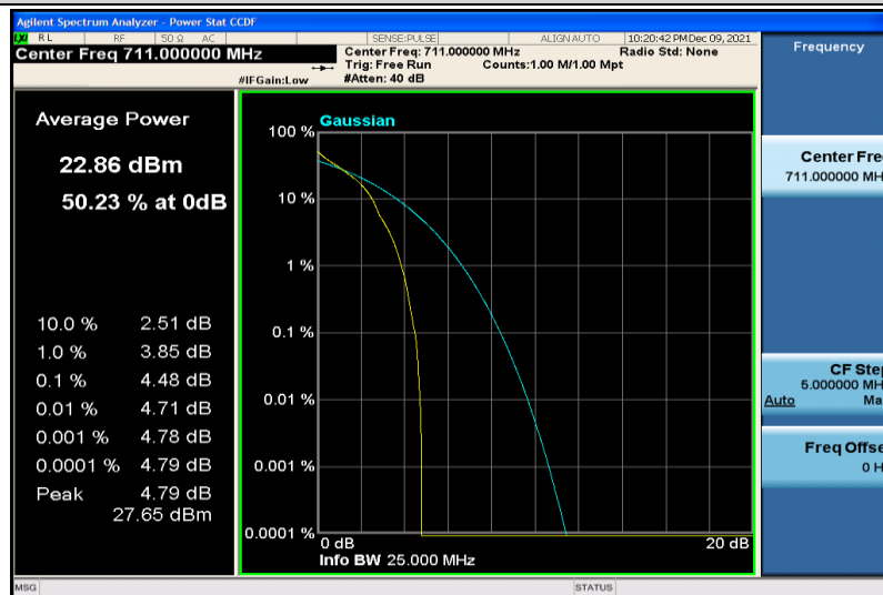
Band17-10MHz-64QAM-23800-1RB#0
