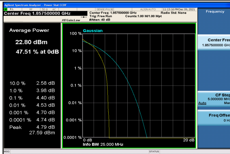
Band25-15MHz-64QAM-26115-1RB#0
