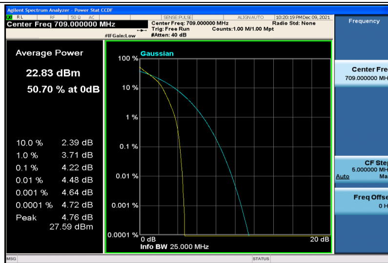
Band17-10MHz-64QAM-23780-1RB#0
