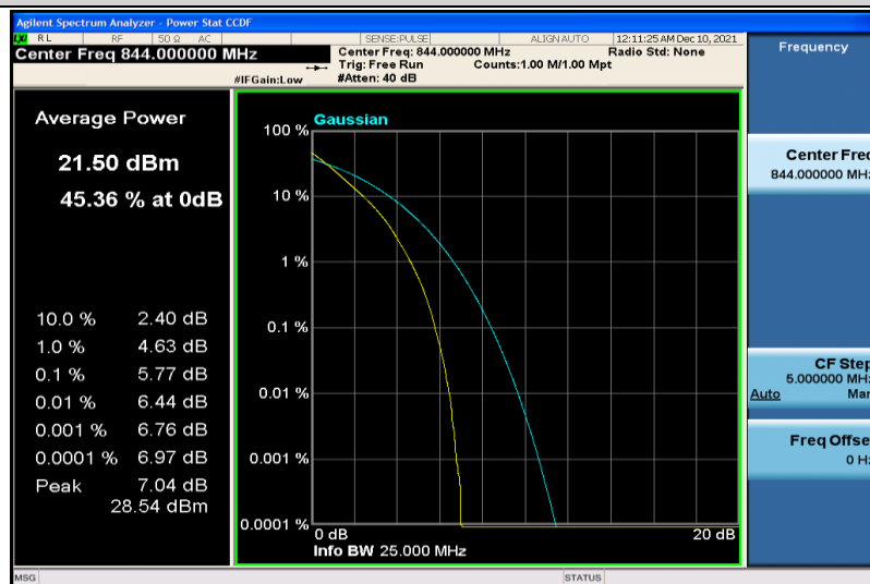
Band26-10MHz-64QAM-26990-50RB#0
