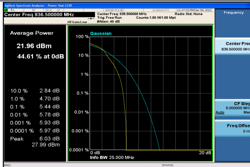
Band26-3MHz-64QAM-26915-1RB#0
