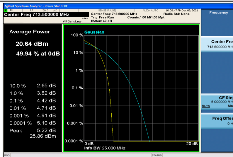
Band17-5MHz-64QAM-23825-25RB#0
