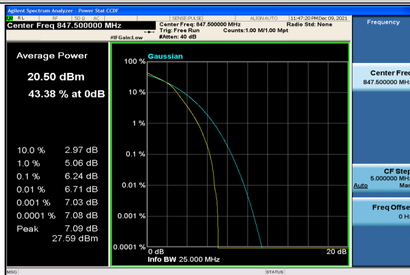
Band26-3MHz-64QAM-27025-15RB#0
