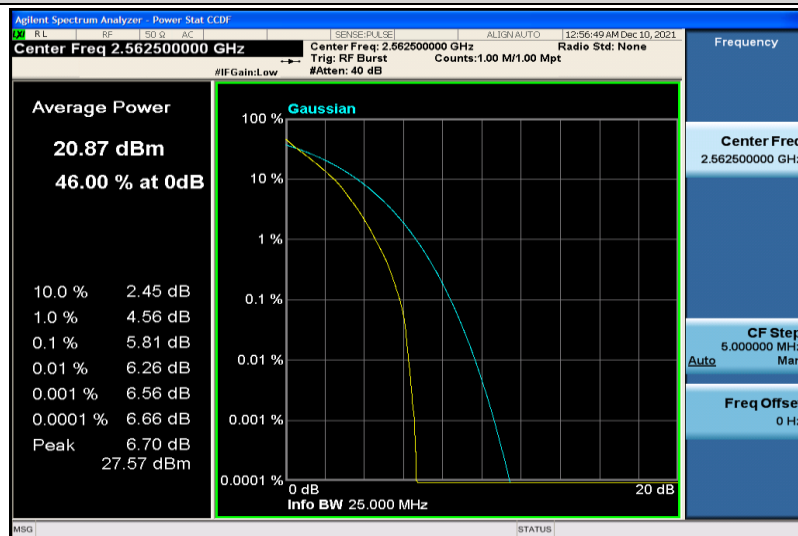
Band41-15MHz-64QAM-40315-75RB#0
