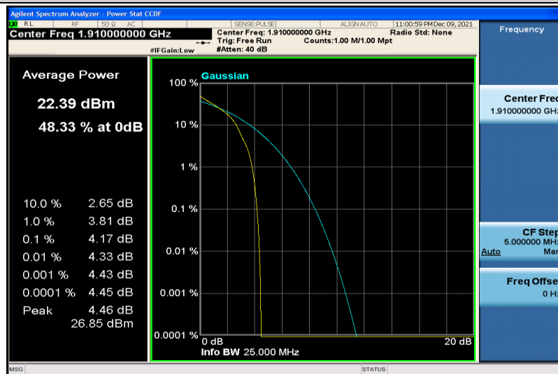
Band25-10MHz-64QAM-26640-1RB#0
