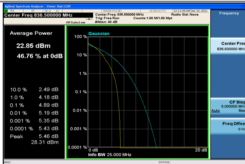
Band26-10MHz-64QAM-26915-1RB#0
