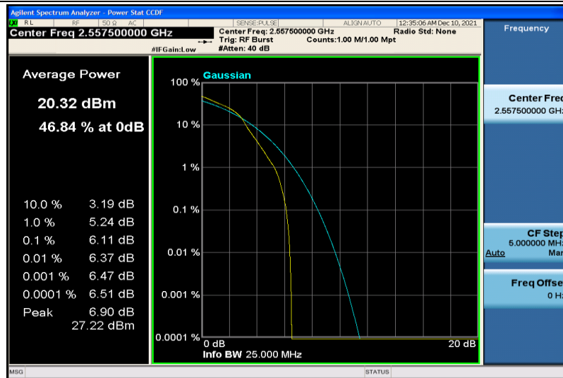
Band41-5MHz-64QAM-40265-1RB#0
