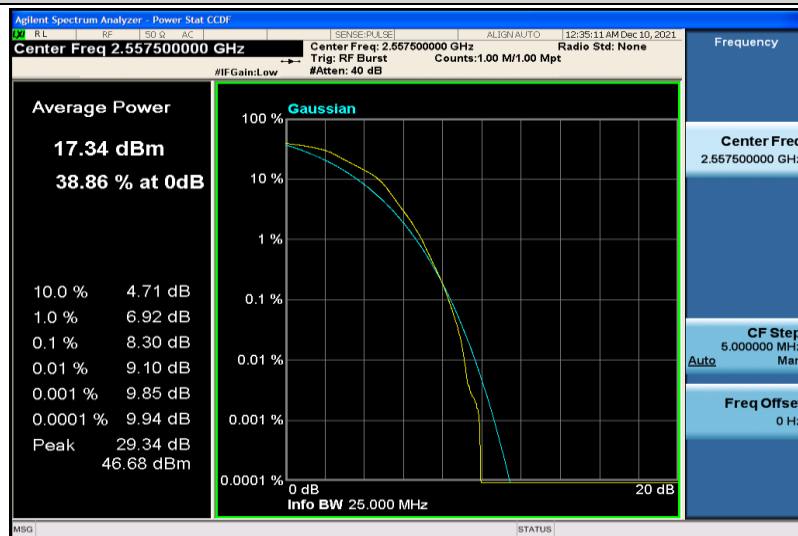
Band41-5MHz-64QAM-40265-25RB#0
