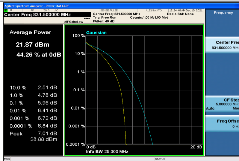
Band26-15MHz-64QAM-26865-75RB#0
