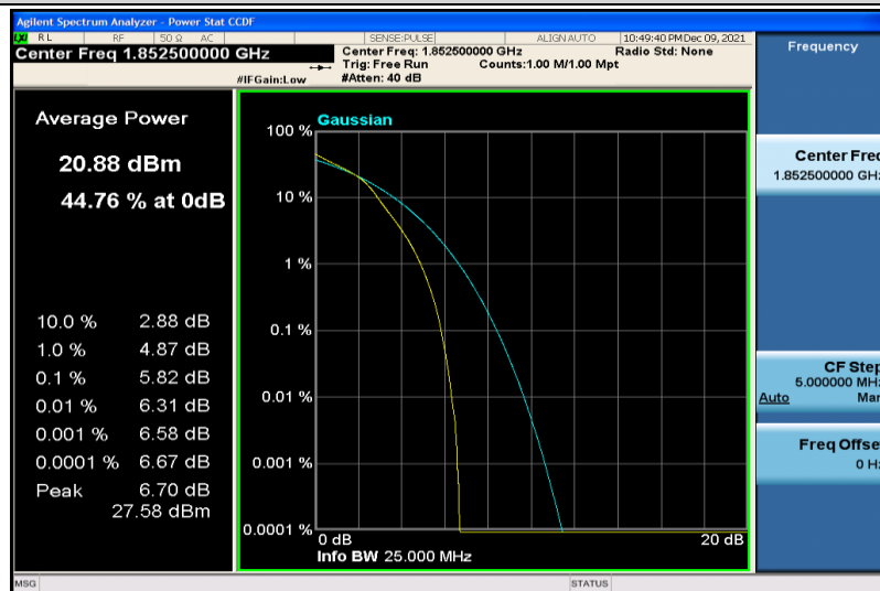
Band25-5MHz-64QAM-26065-25RB#0
