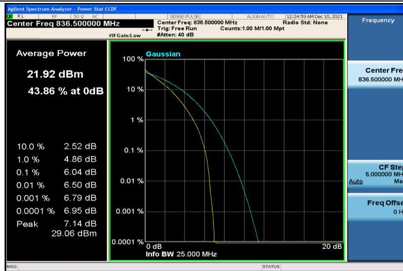
Band26-15MHz-64QAM-26915-75RB#0
