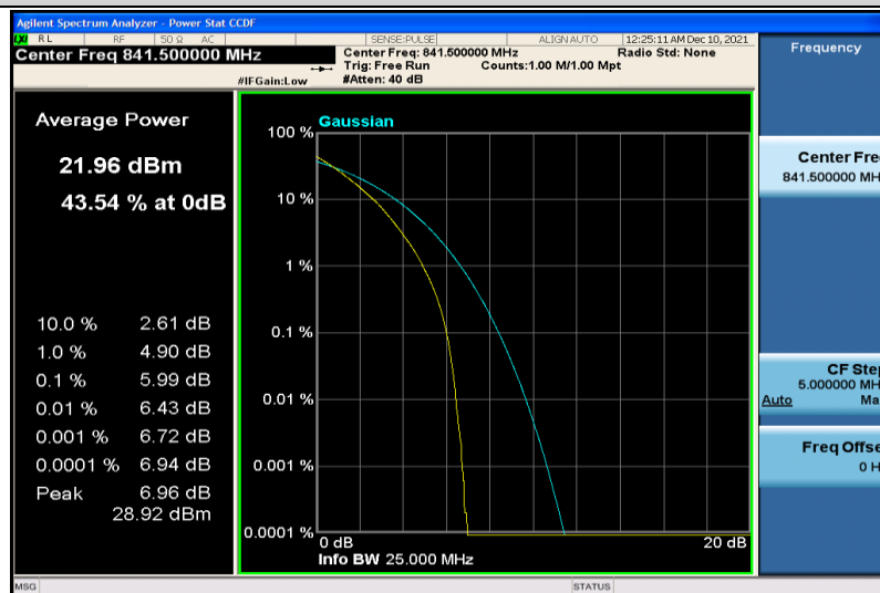
Band26-15MHz-64QAM-26965-75RB#0
