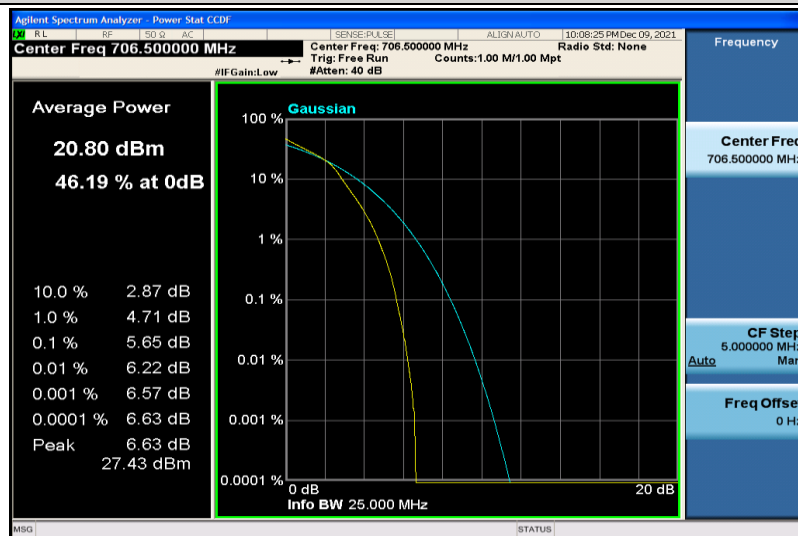
Band17-5MHz-64QAM-23755-25RB#0
