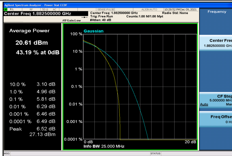
Band25-1.4MHz-64QAM-26365-6RB#0
