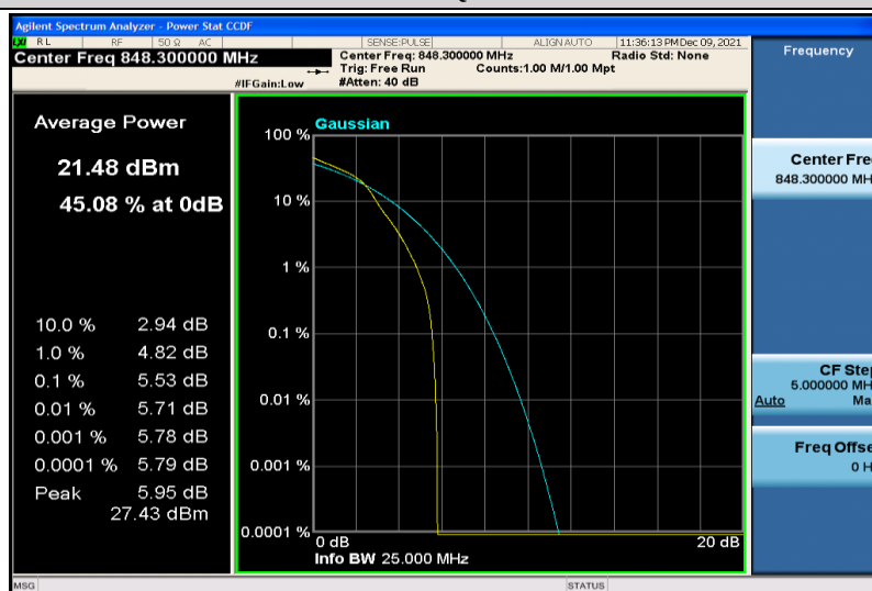
Band26-1.4MHz-64QAM-27033-1RB#0
