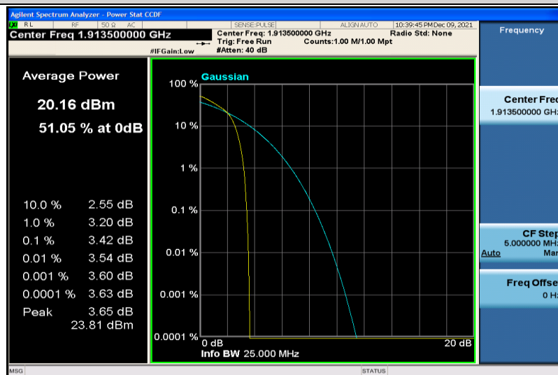
Band25-3MHz-64QAM-26675-15RB#0
