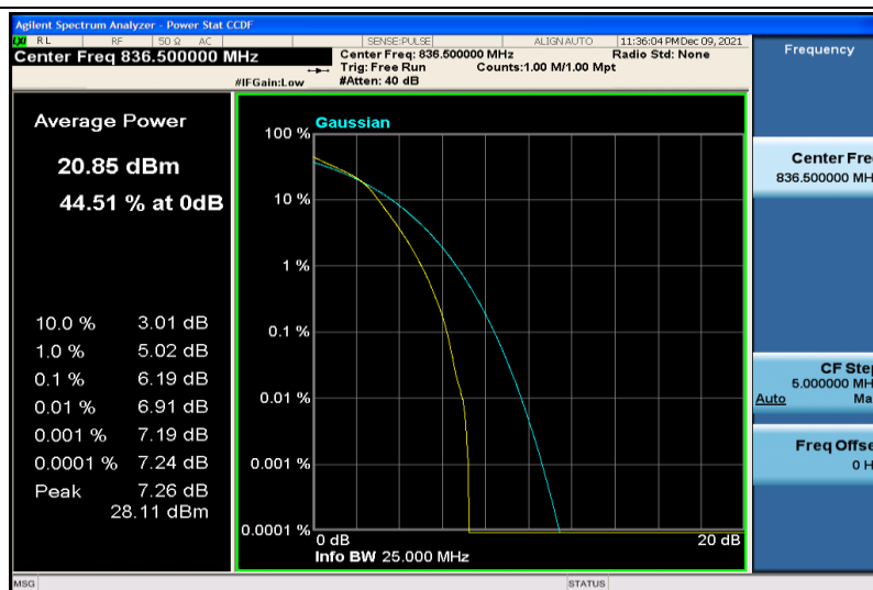
Band26-1.4MHz-64QAM-26915-6RB#0
