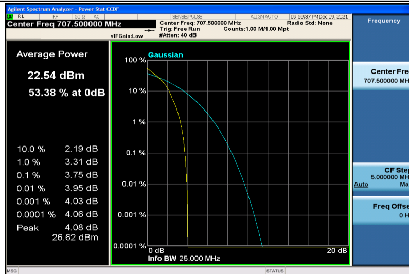
Band12-10MHz-64QAM-23095-1RB#0
