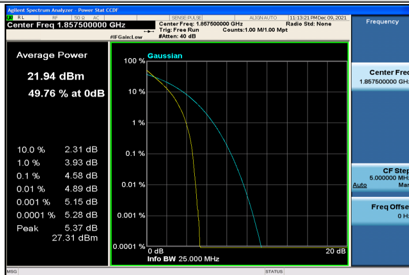
Band25-15MHz-64QAM-26115-75RB#0
