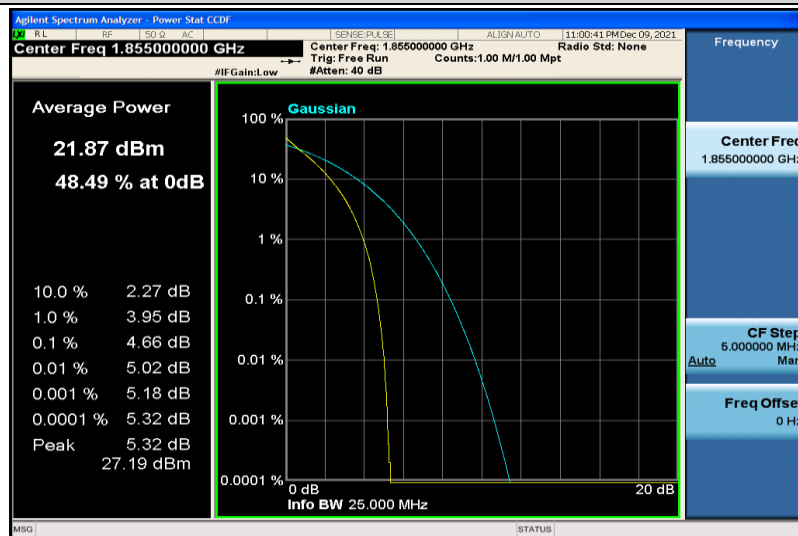
Band25-10MHz-64QAM-26090-50RB#0
