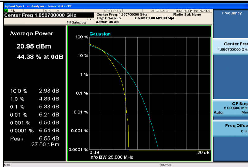
Band25-1.4MHz-64QAM-26047-6RB#0
