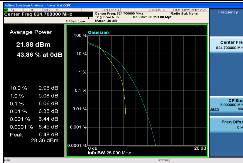
Band26-1.4MHz-64QAM-26797-1RB#0
