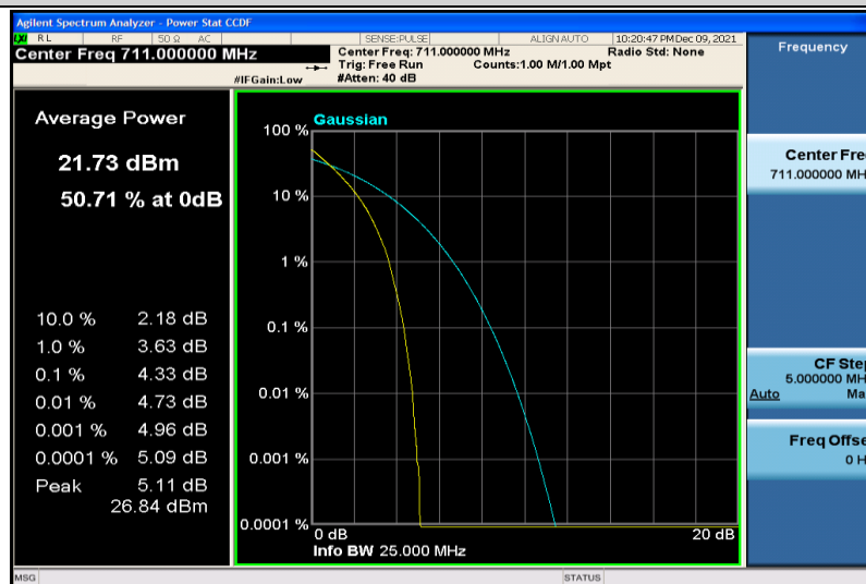
Band17-10MHz-64QAM-23800-50RB#0
