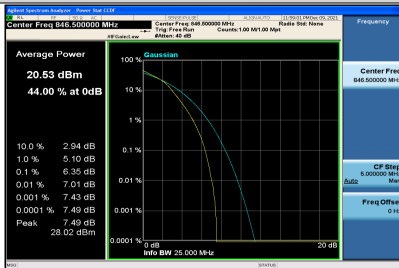
Band26-5MHz-64QAM-27015-25RB#0
