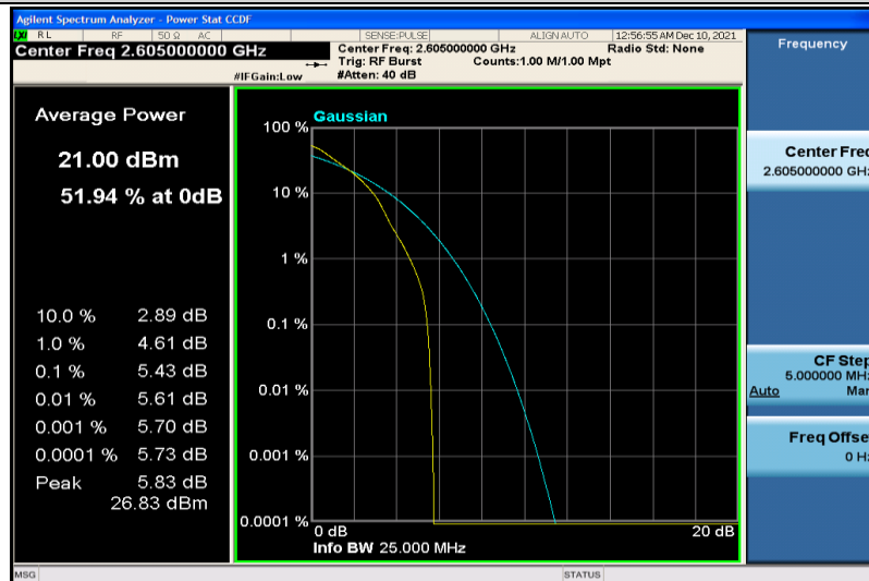
Band41-15MHz-64QAM-40740-1RB#0
