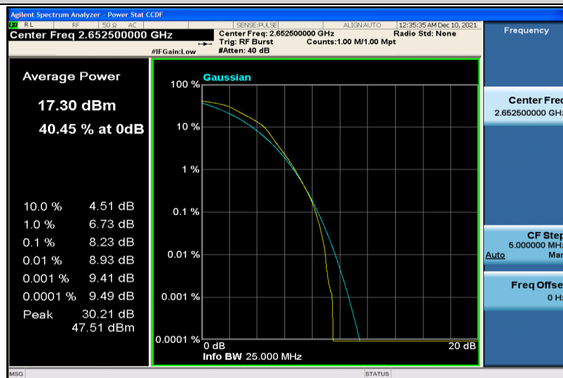
Band41-5MHz-64QAM-41215-25RB#0
