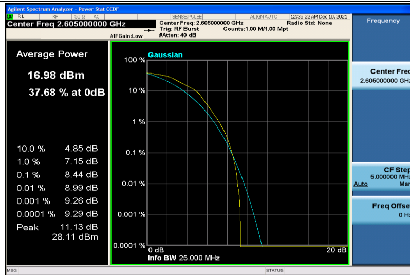
Band41-5MHz-64QAM-40740-25RB#0
