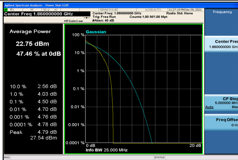
Band25-20MHz-64QAM-26140-1RB#0
