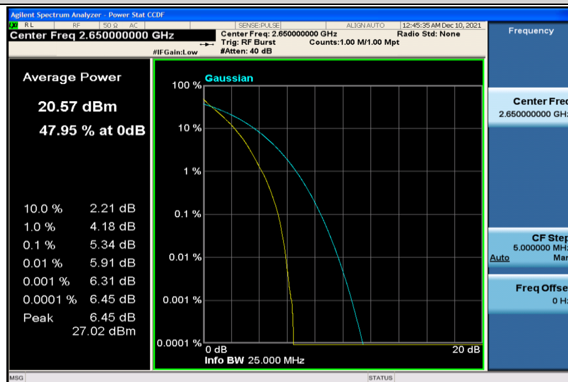
Band41-10MHz-64QAM-41190-50RB#0
