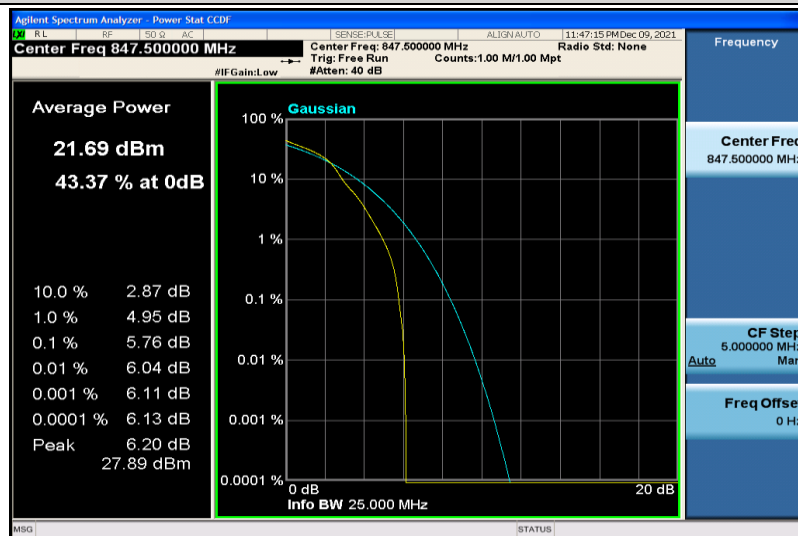
Band26-3MHz-64QAM-27025-1RB#0
