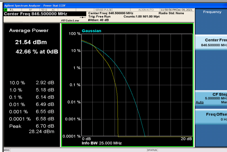
Band26-5MHz-64QAM-27015-1RB#0
