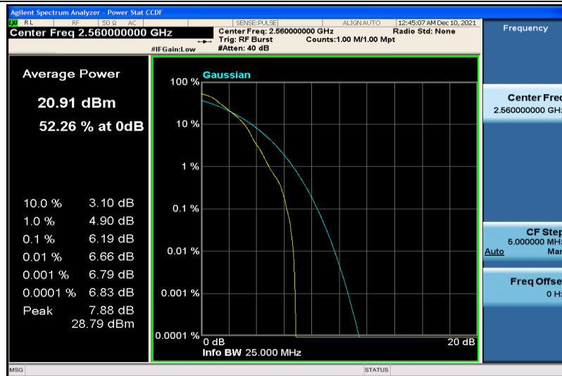
Band41-10MHz-64QAM-40290-1RB#0
