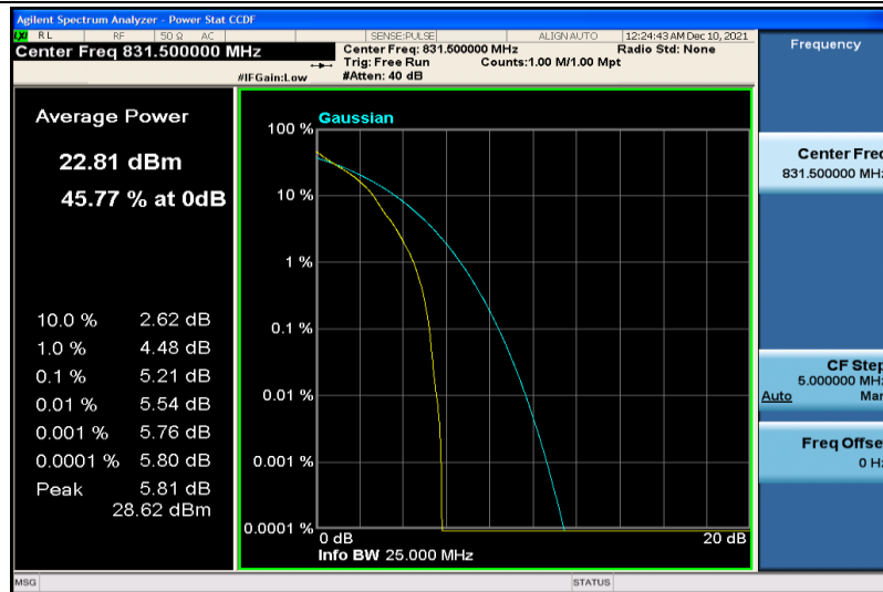
Band26-15MHz-64QAM-26865-1RB#0
