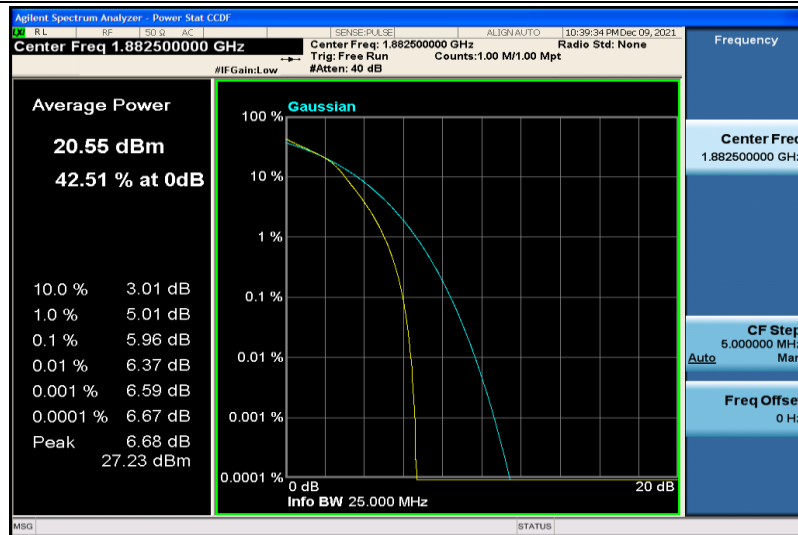
Band25-3MHz-64QAM-26365-15RB#0
