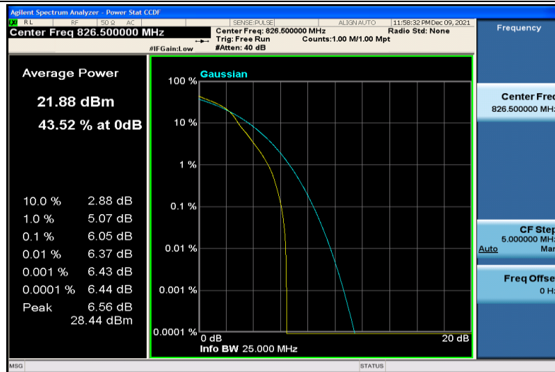
Band26-5MHz-64QAM-26815-1RB#0
