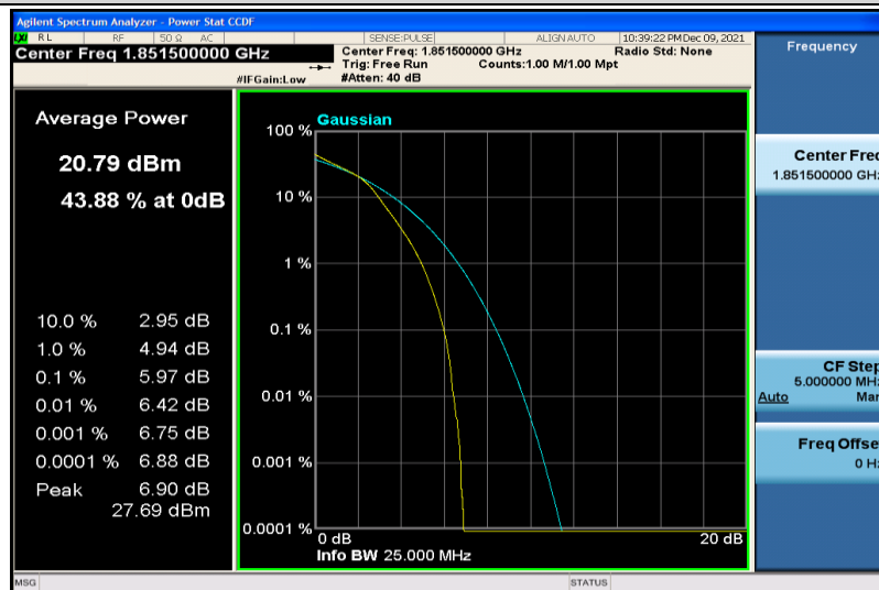
Band25-3MHz-64QAM-26055-15RB#0
