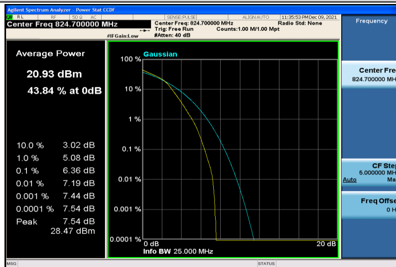
Band26-1.4MHz-64QAM-26797-6RB#0
