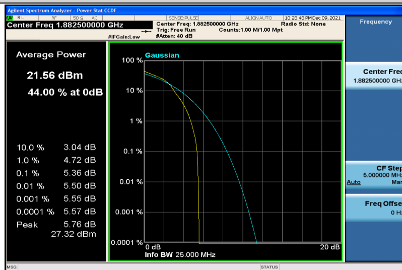
Band25-1.4MHz-64QAM-26365-1RB#0
