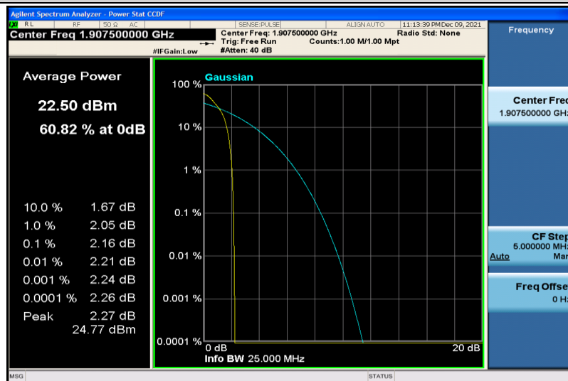
Band25-15MHz-64QAM-26615-1RB#0
