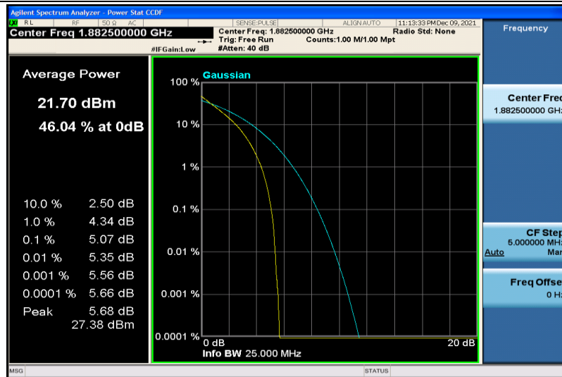
Band25-15MHz-64QAM-26365-75RB#0
