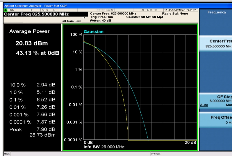
Band26-3MHz-64QAM-26805-15RB#0
