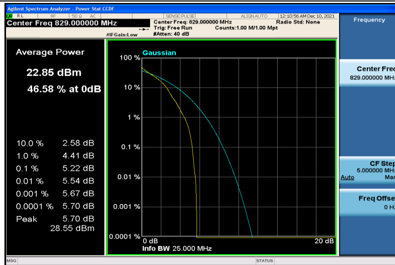
Band26-10MHz-64QAM-26840-1RB#0
