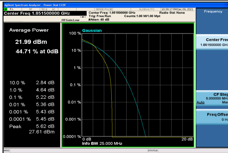
Band25-3MHz-64QAM-26055-1RB#0
