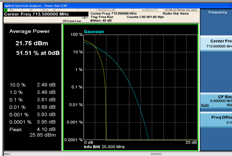
Band17-5MHz-64QAM-23825-1RB#0
