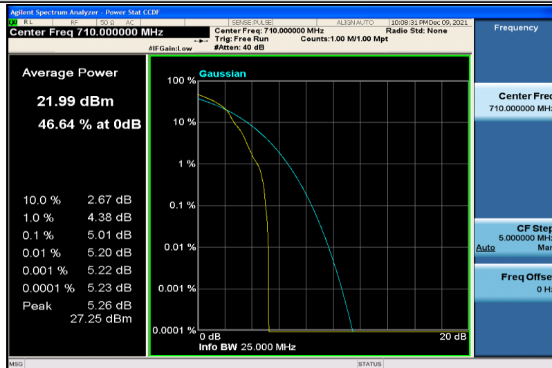
Band17-5MHz-64QAM-23790-1RB#0
