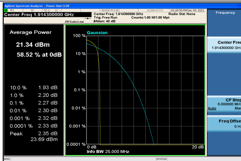
Band25-1.4MHz-64QAM-26683-1RB#0
