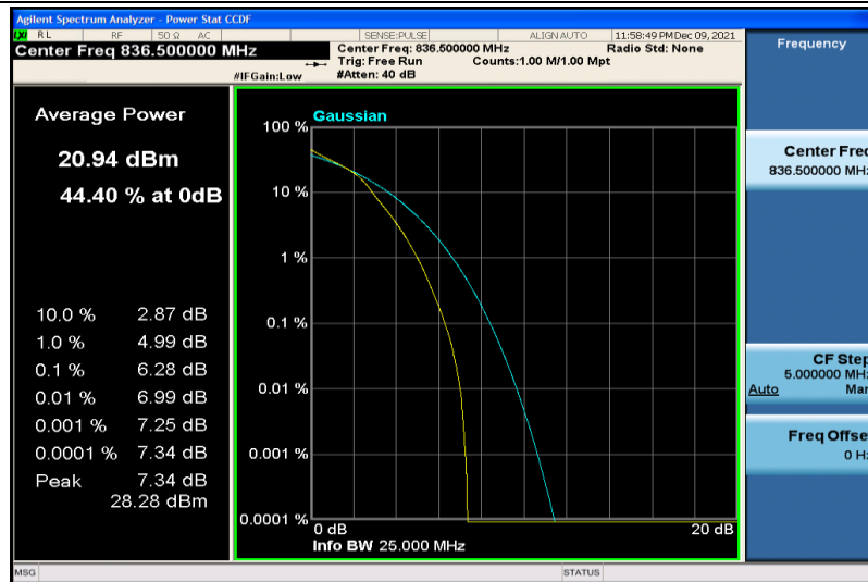
Band26-5MHz-64QAM-26915-25RB#0
