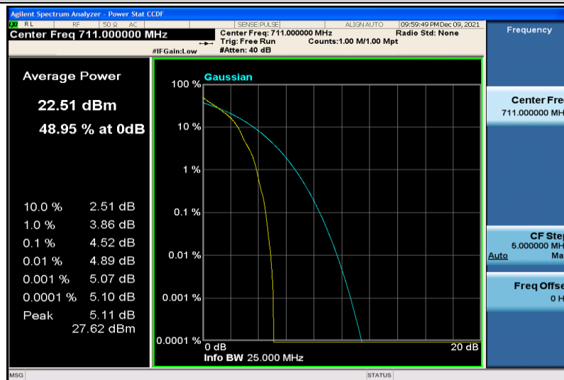
Band12-10MHz-64QAM-23130-1RB#0
