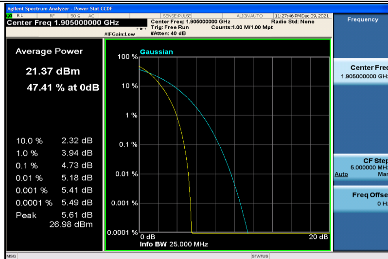
Band25-20MHz-64QAM-26590-100RB#0
