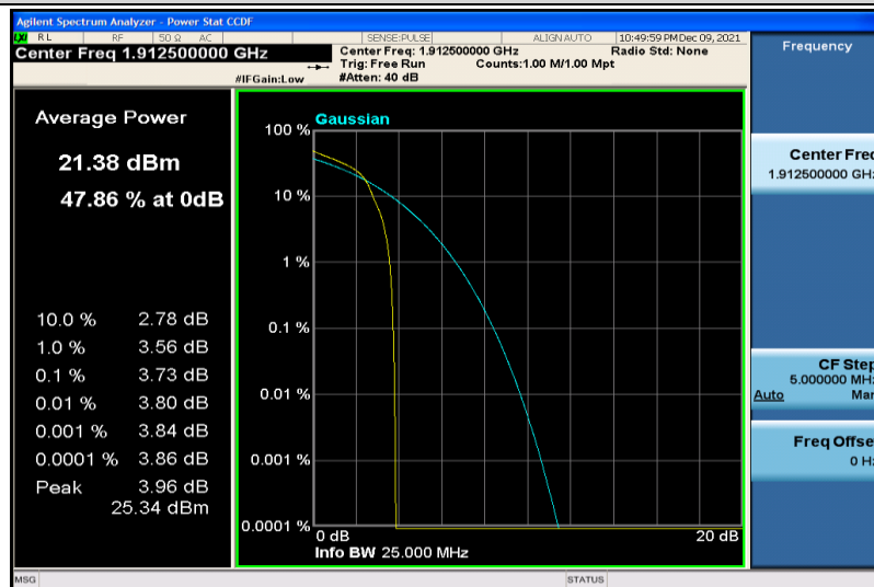
Band25-5MHz-64QAM-26665-1RB#0
