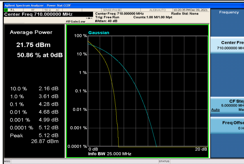
Band17-10MHz-64QAM-23790-50RB#0
