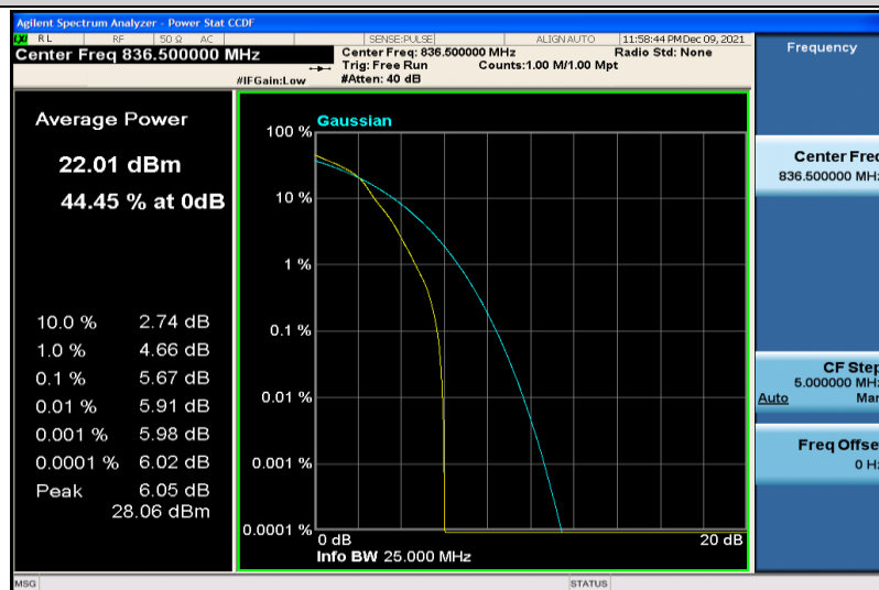
Band26-5MHz-64QAM-26915-1RB#0
