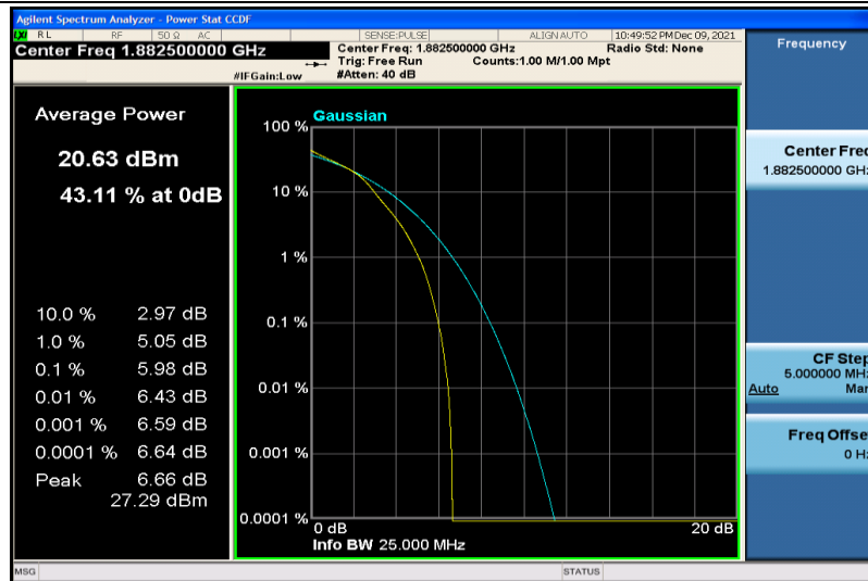
Band25-5MHz-64QAM-26365-25RB#0
