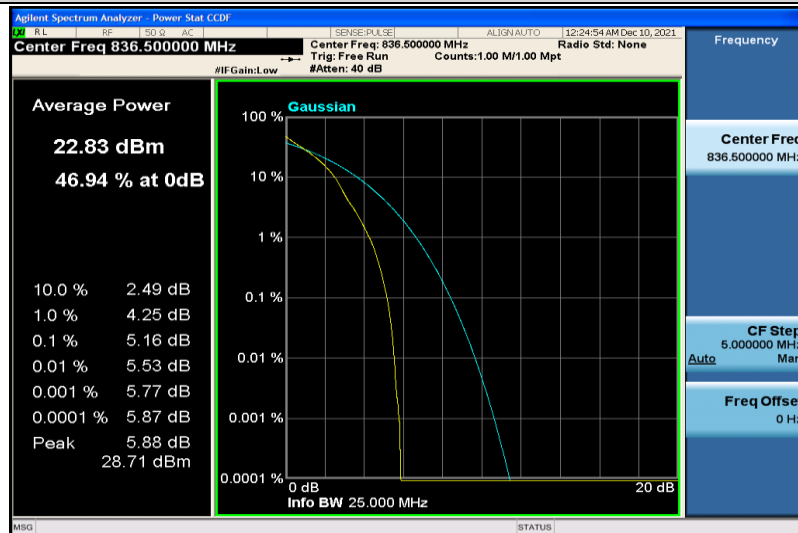
Band26-15MHz-64QAM-26915-1RB#0
