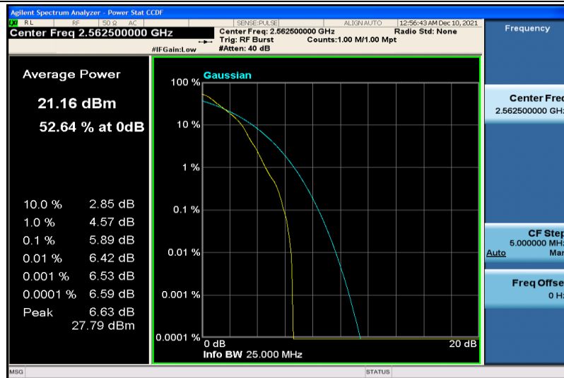
Band41-15MHz-64QAM-40315-1RB#0
