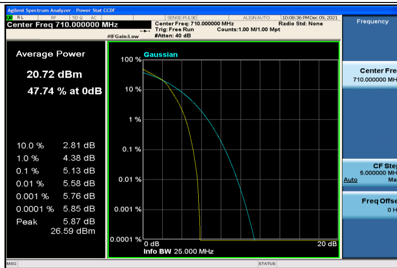
Band17-5MHz-64QAM-23790-25RB#0
