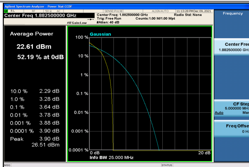
Band25-15MHz-64QAM-26365-1RB#0
