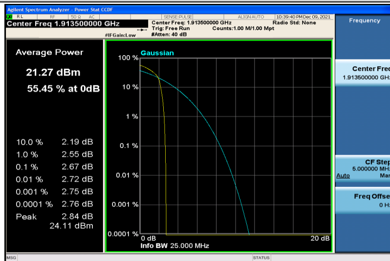
Band25-3MHz-64QAM-26675-1RB#0
