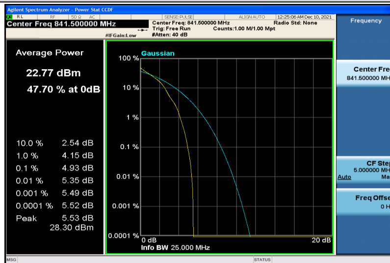
Band26-15MHz-64QAM-26965-1RB#0
