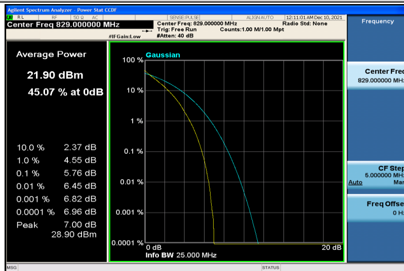
Band26-10MHz-64QAM-26840-50RB#0
