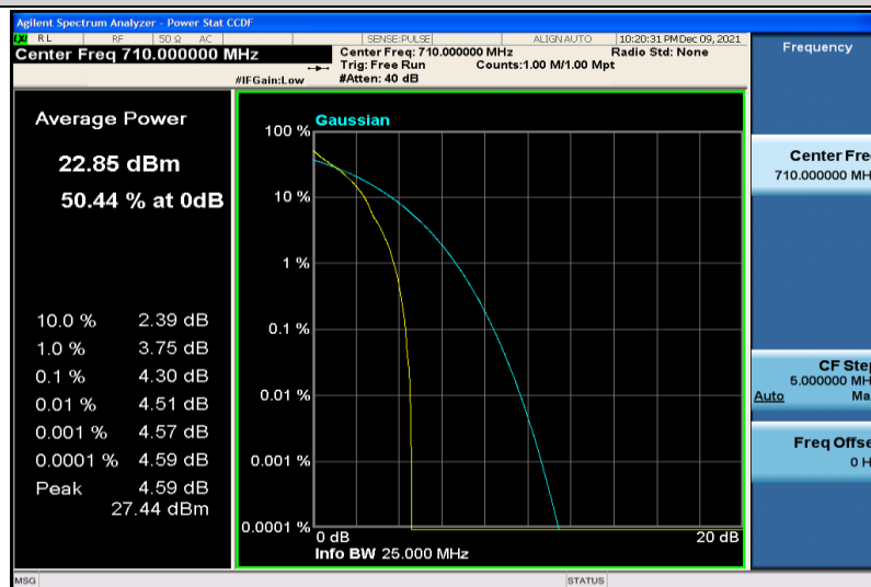
Band17-10MHz-64QAM-23790-1RB#0
