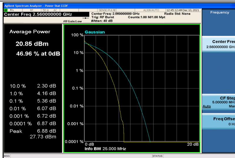
Band41-10MHz-64QAM-40290-50RB#0
