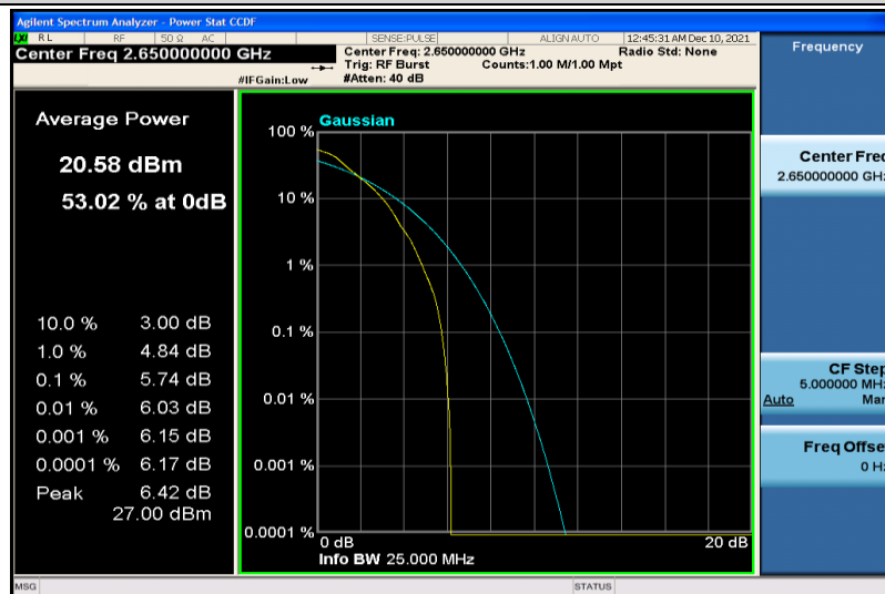
Band41-10MHz-64QAM-41190-1RB#0
