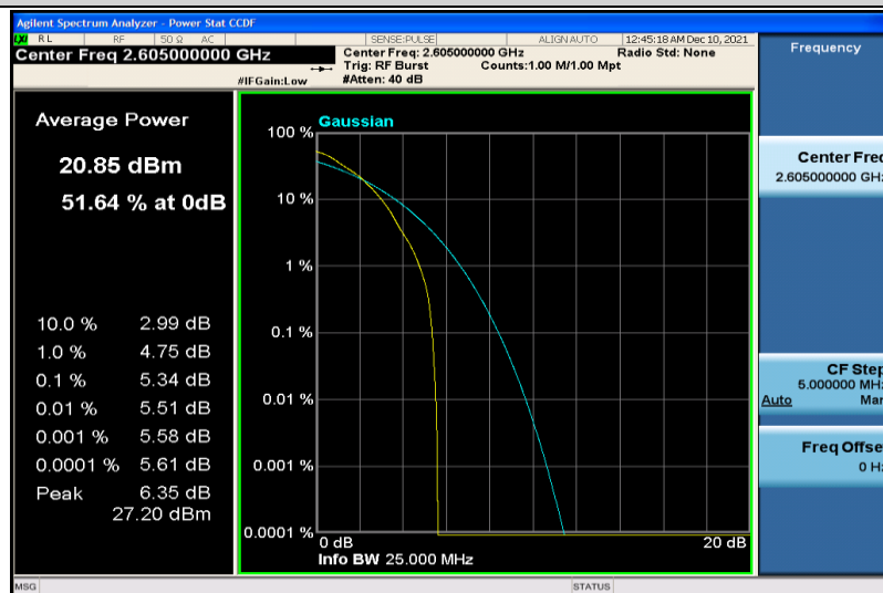
Band41-10MHz-64QAM-40740-1RB#0
