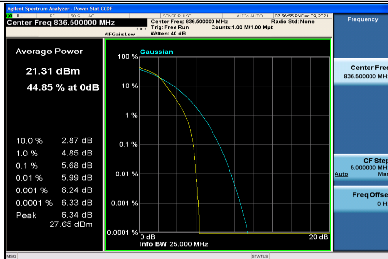
Band5-3MHz-64QAM-20525-1RB#0
