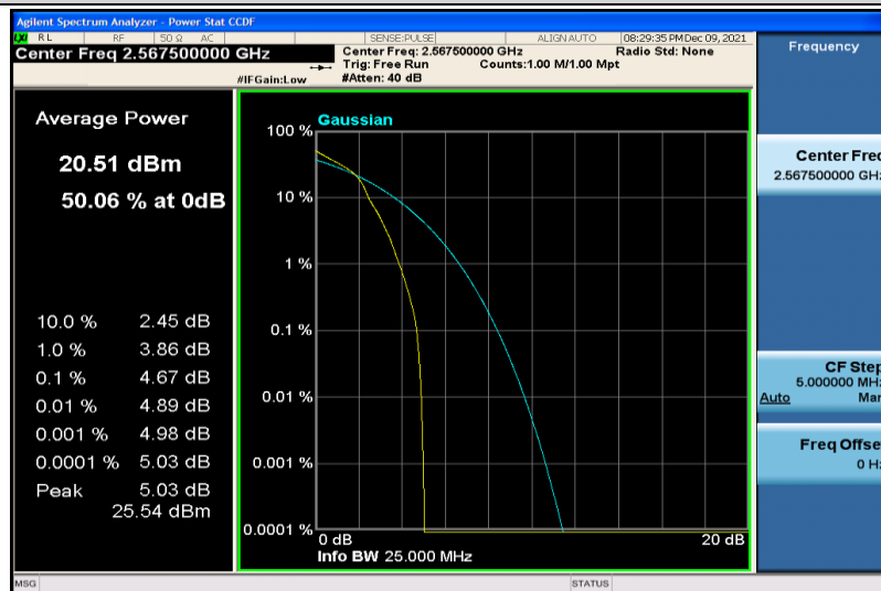
Band7-5MHz-64QAM-21425-1RB#0
