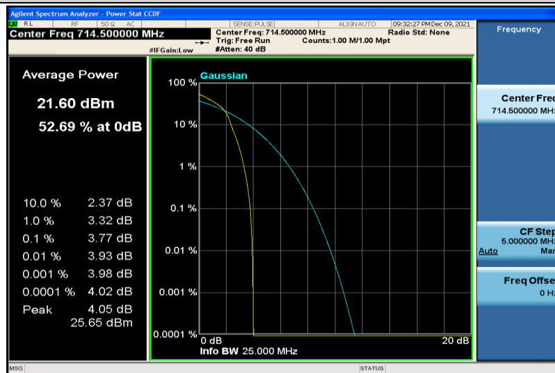
Band12-3MHz-64QAM-23165-1RB#0
