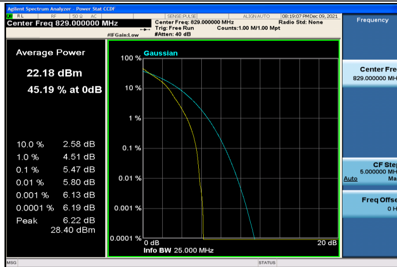
Band5-10MHz-64QAM-20450-1RB#0
