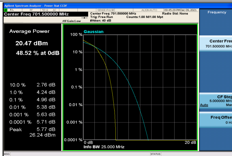
Band12-5MHz-64QAM-23035-25RB#0
