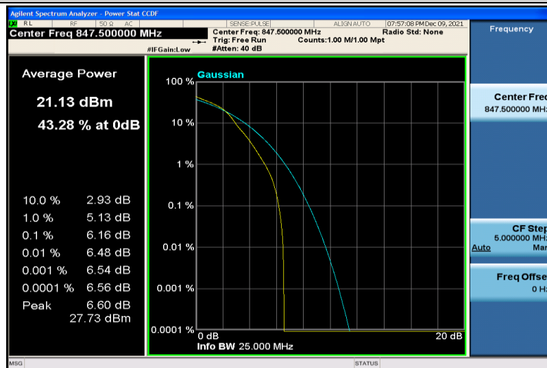
Band5-3MHz-64QAM-20635-1RB#0
