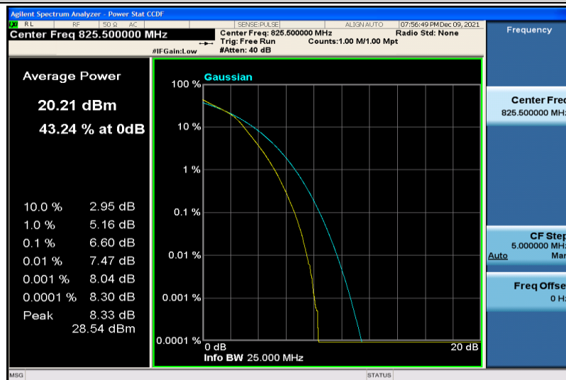
Band5-3MHz-64QAM-20415-15RB#0
