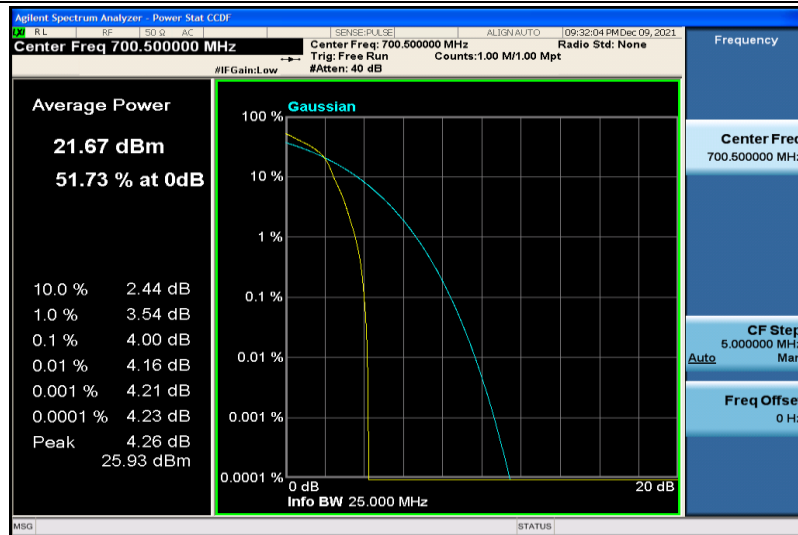
Band12-3MHz-64QAM-23025-1RB#0
