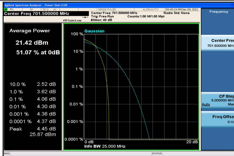
Band12-5MHz-64QAM-23035-1RB#0
