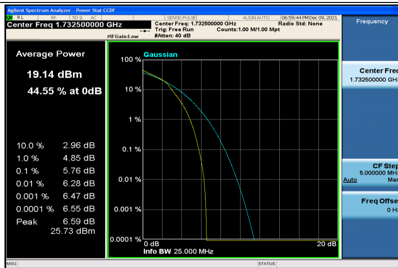
Band4-5MHz-64QAM-20175-25RB#0
