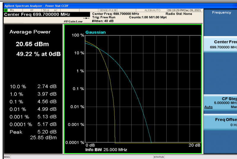
Band12-1.4MHz-64QAM-23017-6RB#0
