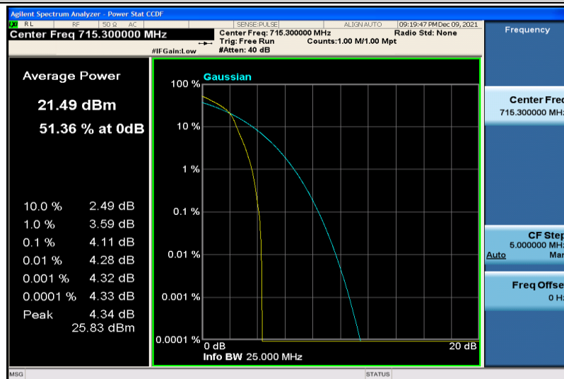
Band12-1.4MHz-64QAM-23173-1RB#0
