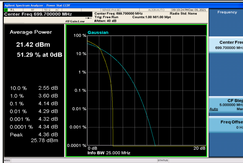
Band12-1.4MHz-64QAM-23017-1RB#0
