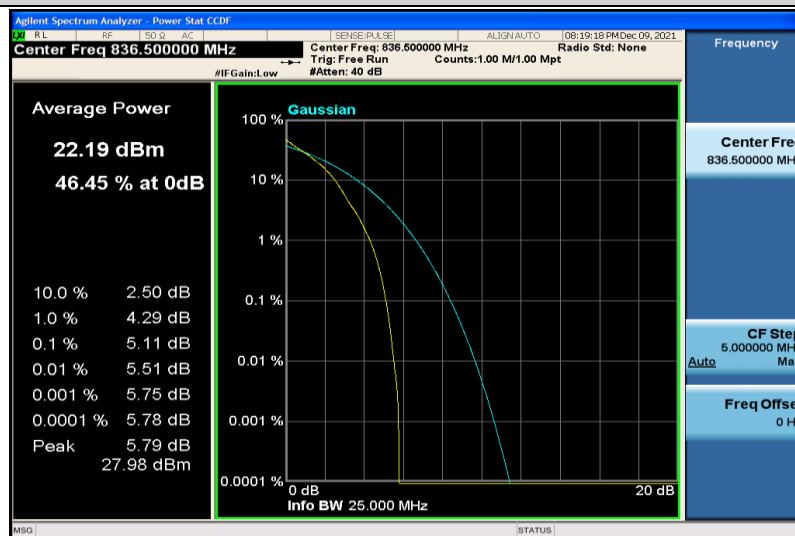
Band5-10MHz-64QAM-20525-1RB#0
