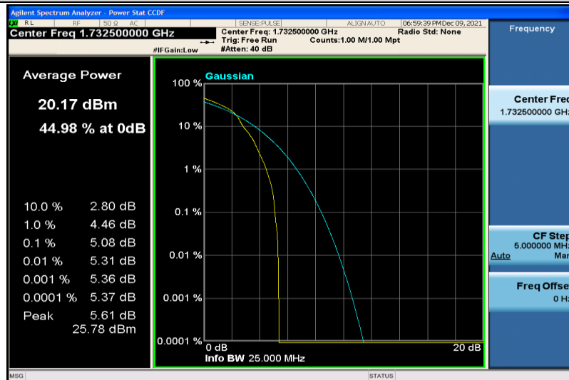
Band4-5MHz-64QAM-20175-1RB#0
