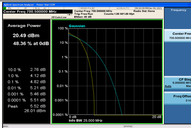
Band12-3MHz-64QAM-23025-15RB#0
