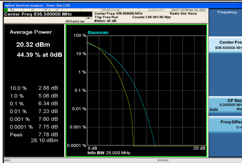
Band5-5MHz-64QAM-20525-25RB#0
