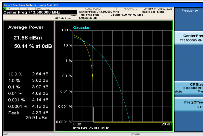
Band12-5MHz-64QAM-23155-1RB#0
