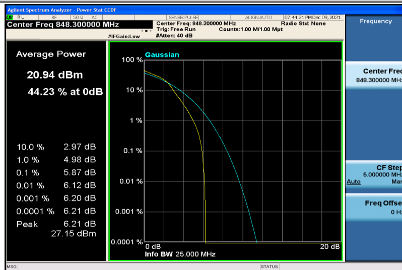
Band5-1.4MHz-64QAM-20643-1RB#0
