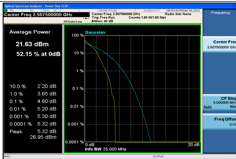
Band7-15MHz-64QAM-20825-1RB#0
