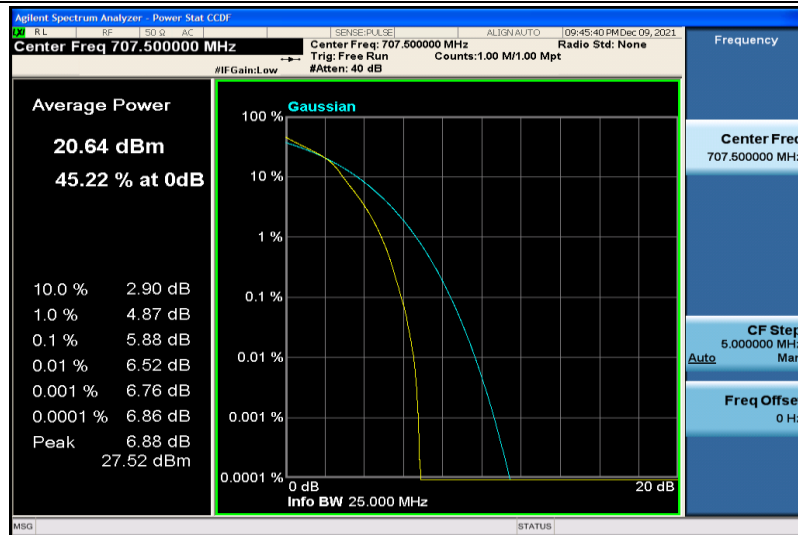
Band12-5MHz-64QAM-23095-25RB#0
