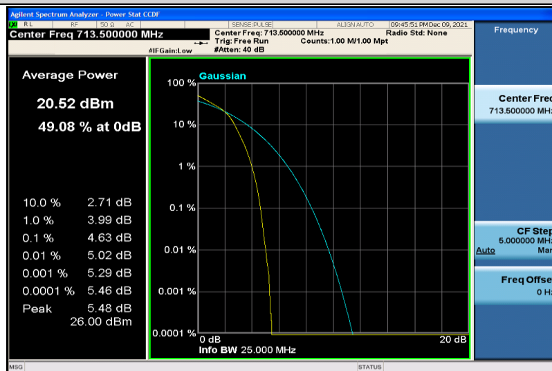
Band12-5MHz-64QAM-23155-25RB#0
