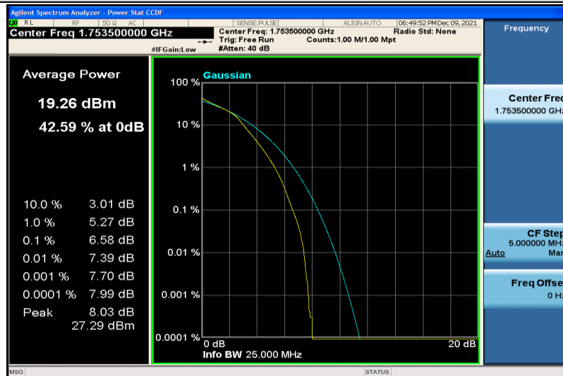
Band4-3MHz-64QAM-20385-15RB#0
