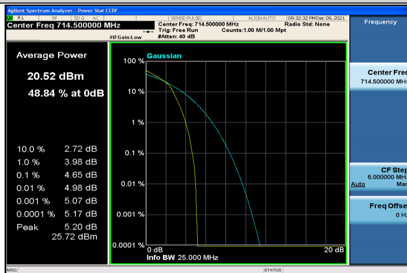
Band12-3MHz-64QAM-23165-15RB#0
