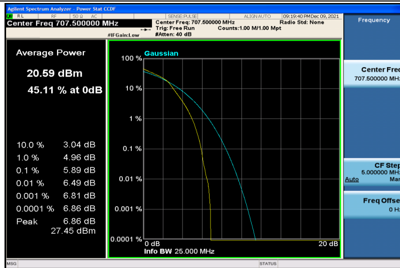
Band12-1.4MHz-64QAM-23095-6RB#0
