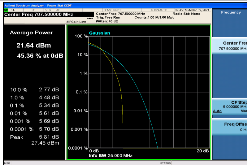
Band12-5MHz-64QAM-23095-1RB#0
