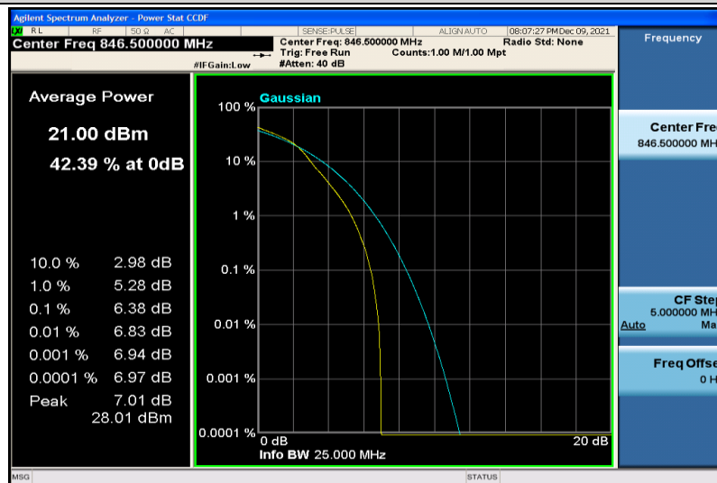
Band5-5MHz-64QAM-20625-1RB#0
