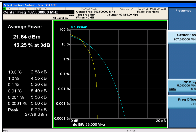
Band12-1.4MHz-64QAM-23095-1RB#0
