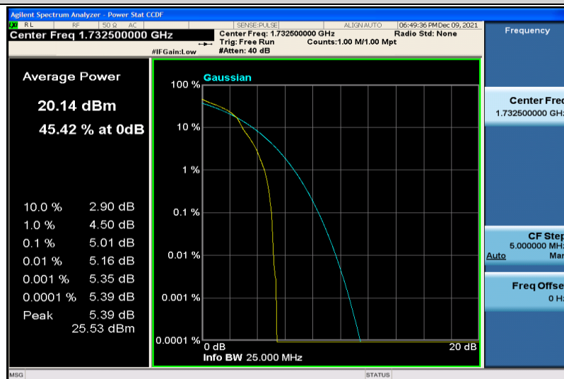
Band4-3MHz-64QAM-20175-1RB#0
