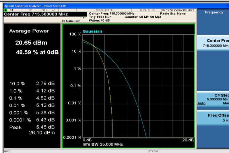
Band12-1.4MHz-64QAM-23173-6RB#0
