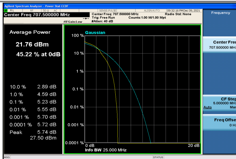
Band12-3MHz-64QAM-23095-1RB#0
