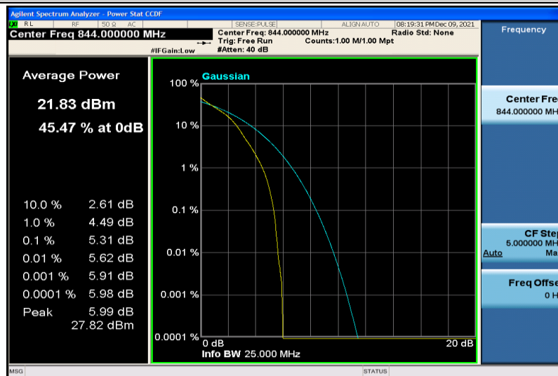
Band5-10MHz-64QAM-20600-1RB#0
