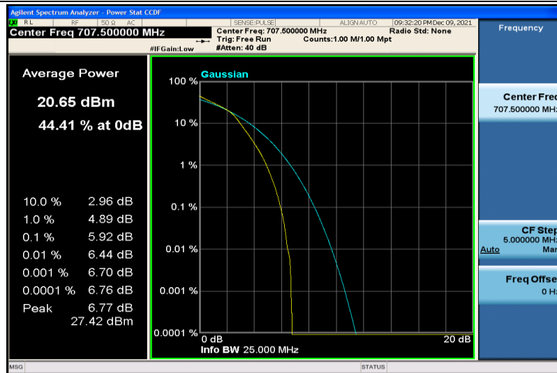
Band12-3MHz-64QAM-23095-15RB#0
