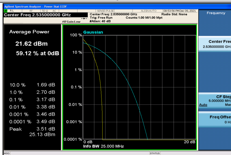
Band7-15MHz-64QAM-21100-1RB#0
