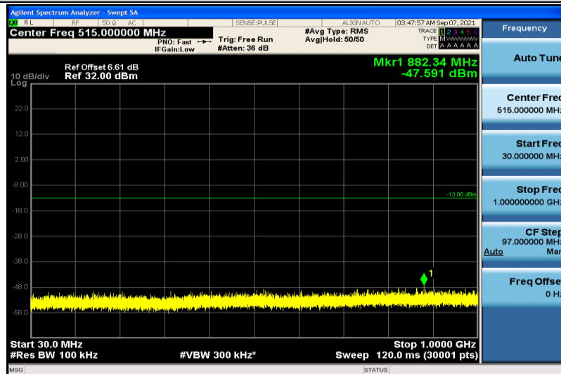
Band25-3MHz-QPSK-26675-1RB#0-30~1000MHz
