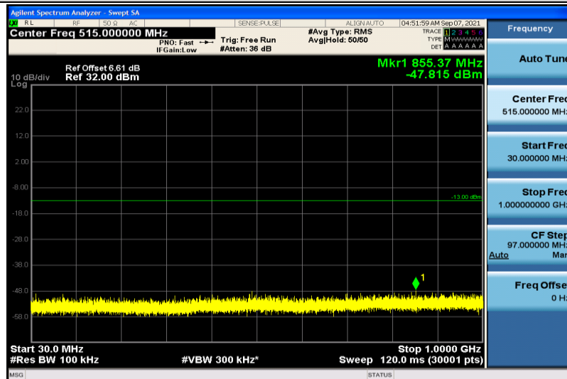
Band25-15MHz-16QAM-26615-1RB#0-30~1000MHz
