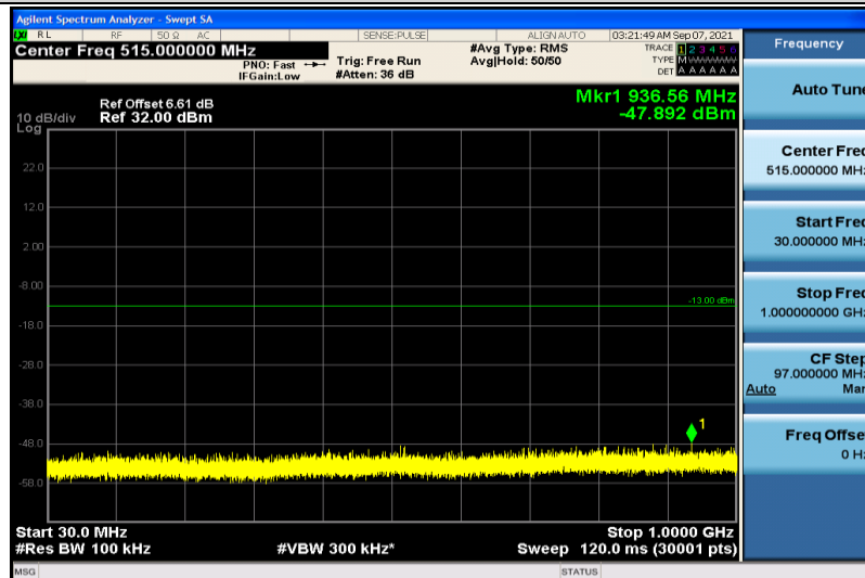
Band25-1.4MHz-QPSK-26683-1RB#0-30~1000MHz
