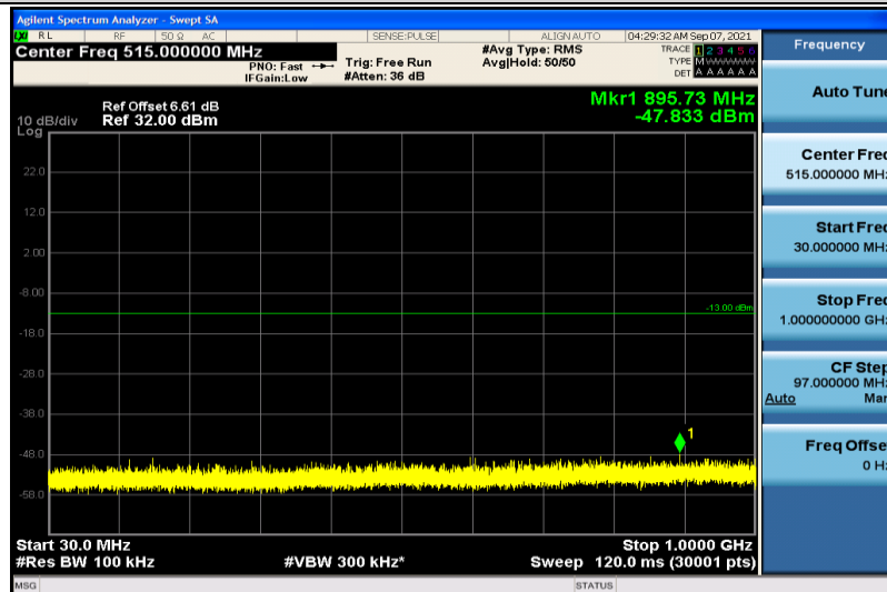
Band25-10MHz-16QAM-26640-1RB#0-30~1000MHz
