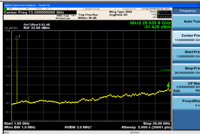
Band2-20MHz-16QAM-18700-1RB#0-1000~26000MHz
