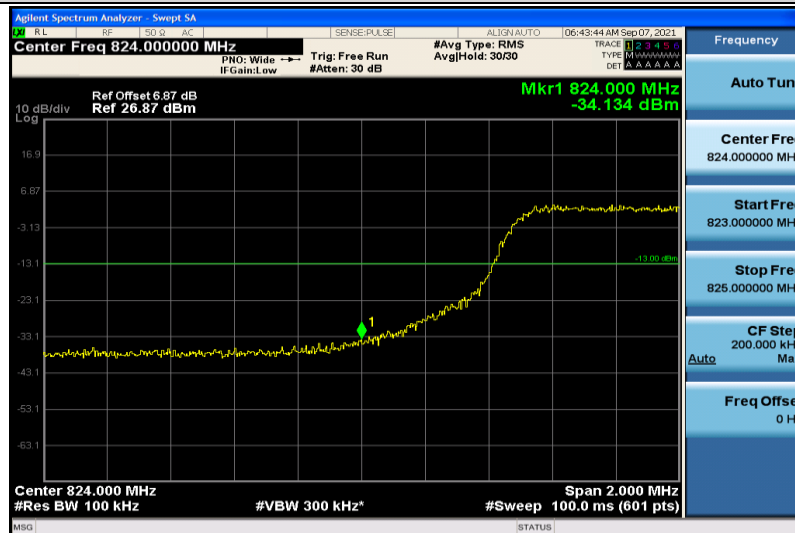
Band26-10MHz-16QAM-26840-50RB#0
