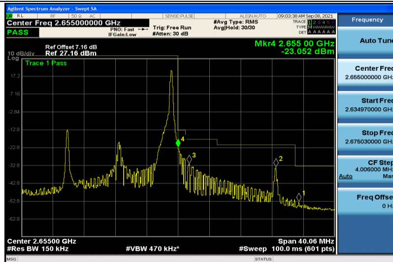
Band41-15MHz-16QAM-41165-1RB#74
