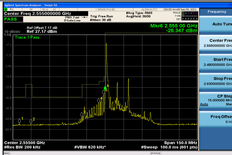
Band41-20MHz-16QAM-40340-1RB#0
