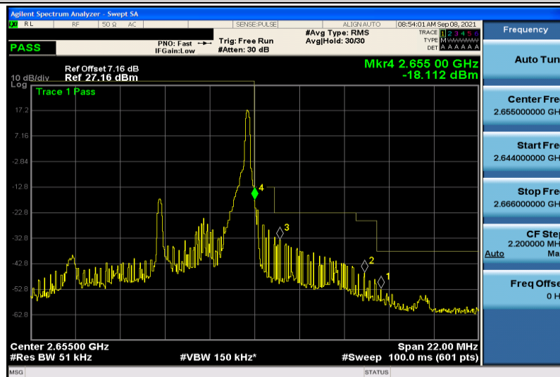
Band41-5MHz-16QAM-41215-1RB#24
