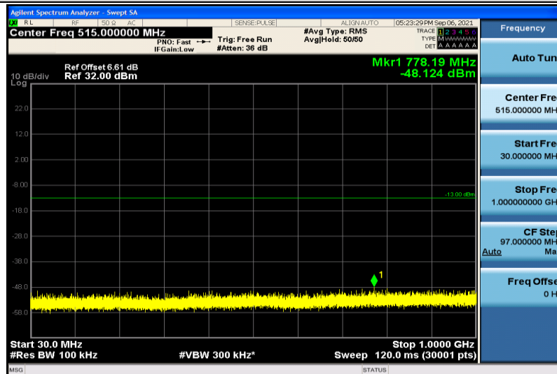
Band2-1.4MHz-16QAM-19193-1RB#0-30~1000MHz
