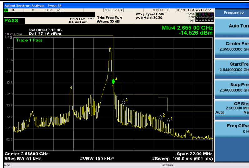
Band41-5MHz-QPSK-41215-1RB#24
