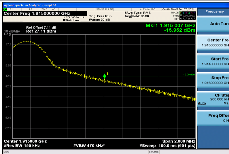
Band25-15MHz-16QAM-26615-1RB#74
