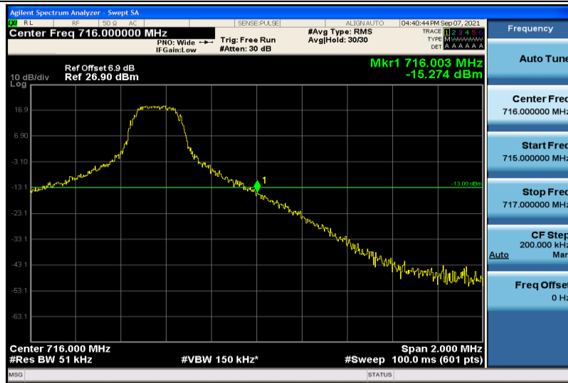
Band12-5MHz-16QAM-23155-1RB#24
