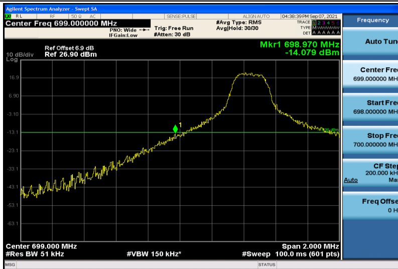
Band12-5MHz-QPSK-23035-1RB#0
