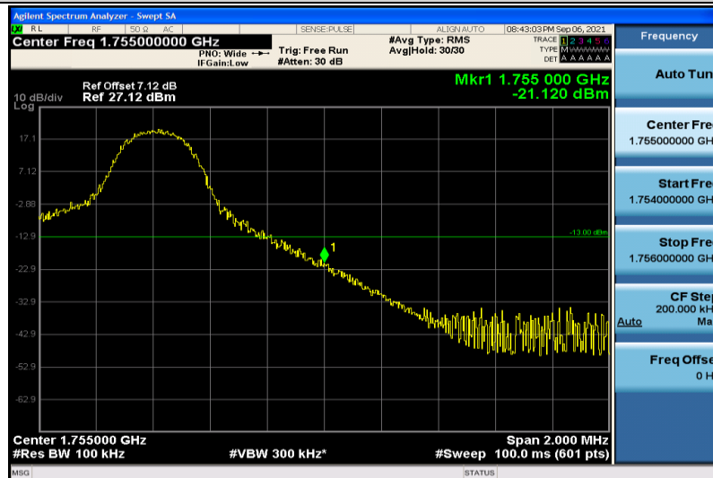
Band4-10MHz-16QAM-20350-1RB#49
