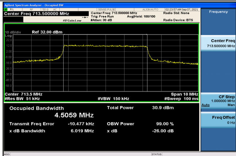
Band17-5MHz-QPSK-23825-25RB#0-4.5059
