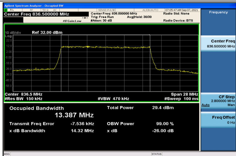
Band26-15MHz-16QAM-26915-75RB#0-13.387
