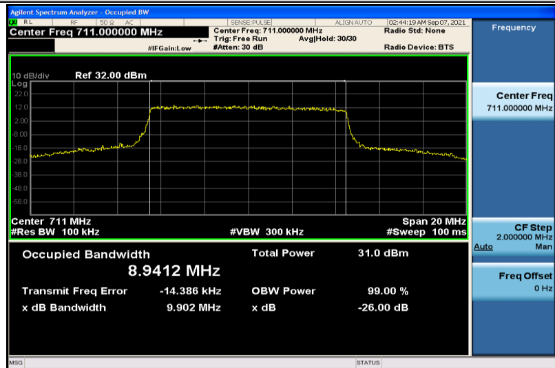
Band17-10MHz-QPSK-23800-50RB#0-8.9412
