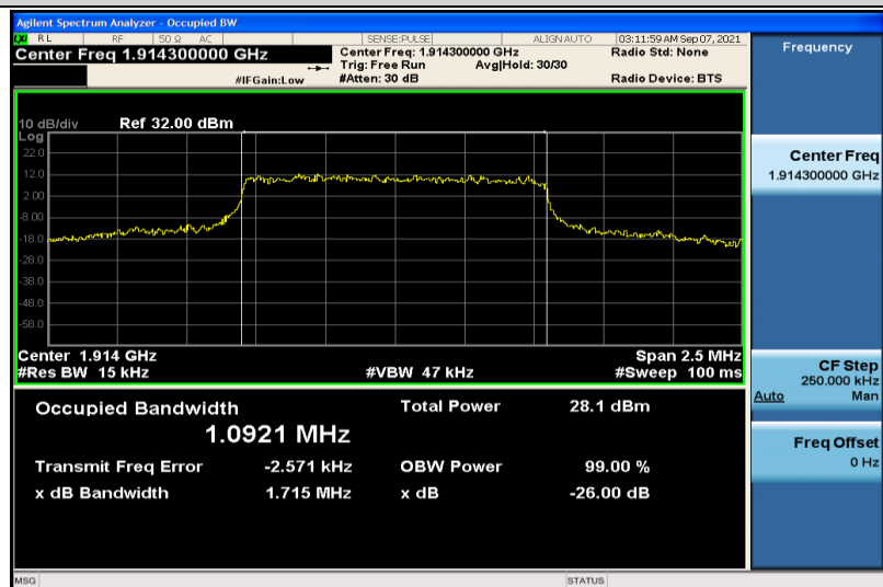
Band25-1.4MHz-QPSK-26683-6RB#0-1.0921
