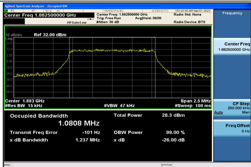
Band25-1.4MHz-16QAM-26365-6RB#0-1.0808
