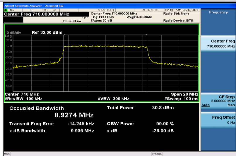
Band17-10MHz-QPSK-23790-50RB#0-8.9274
