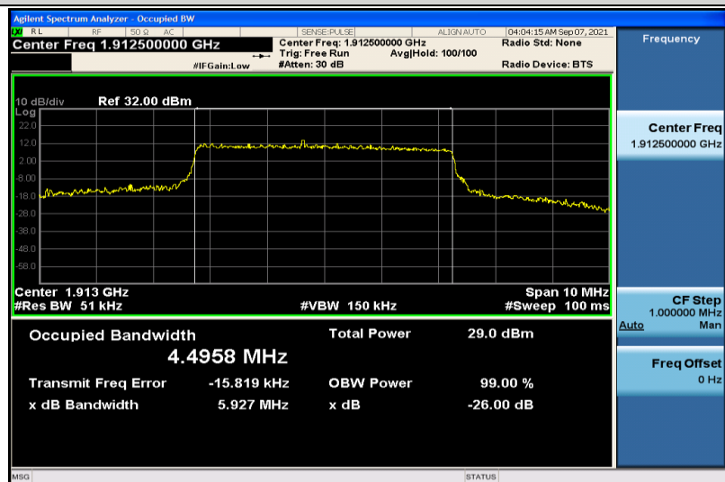
Band25-5MHz-16QAM-26665-25RB#0-4.4958
