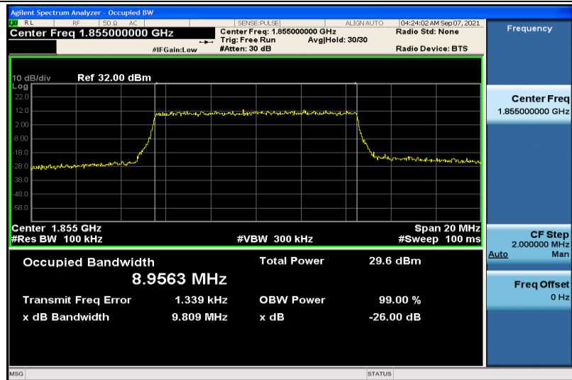
Band25-10MHz-16QAM-26090-50RB#0-8.9563
