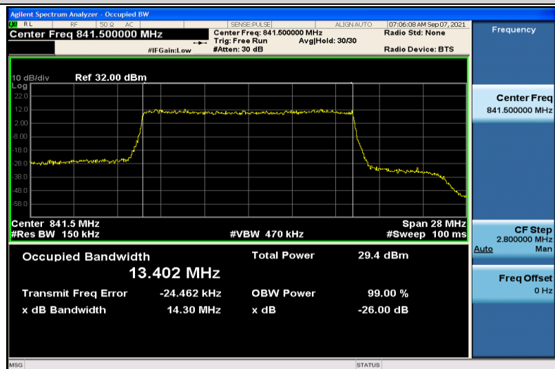
Band26-15MHz-16QAM-26965-75RB#0-13.402
