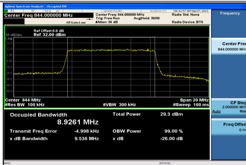
Band26-10MHz-16QAM-26990-50RB#0-8.9261
