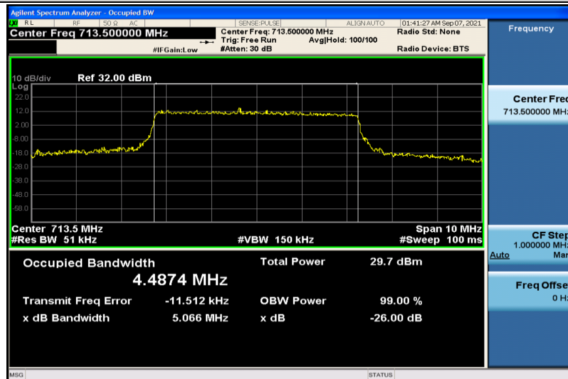
Band12-5MHz-16QAM-23155-25RB#0-4.4874
