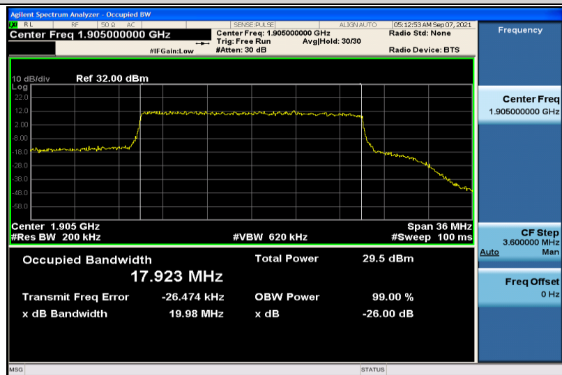
Band25-20MHz-16QAM-26590-100RB#0-17.923
