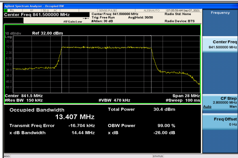
Band26-15MHz-QPSK-26965-75RB#0-13.407
