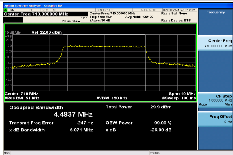
Band17-5MHz-16QAM-23790-25RB#0-4.4837
