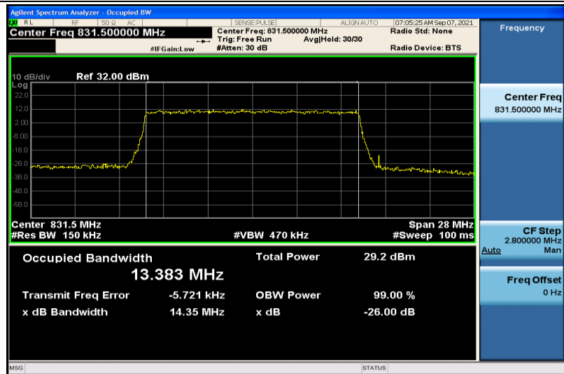
Band26-15MHz-16QAM-26865-75RB#0-13.383
