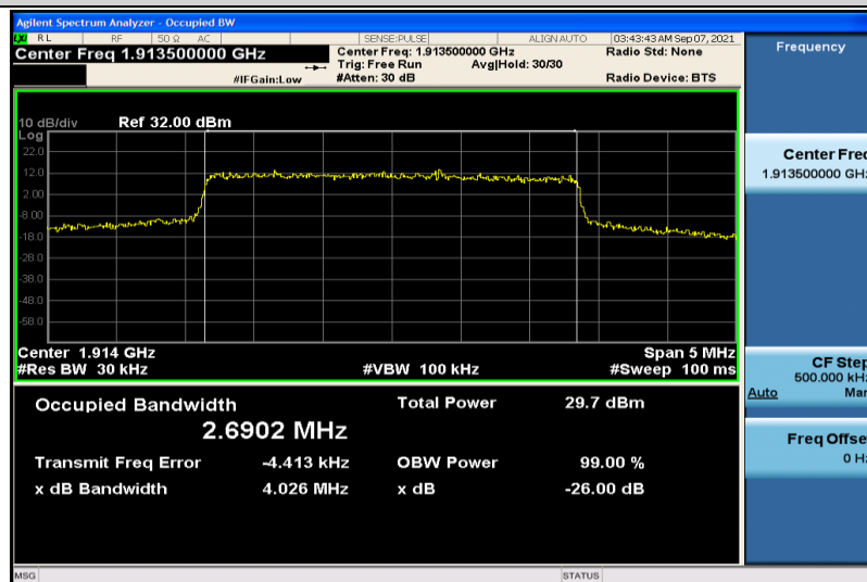
Band25-3MHz-QPSK-26675-15RB#0-2.6902
