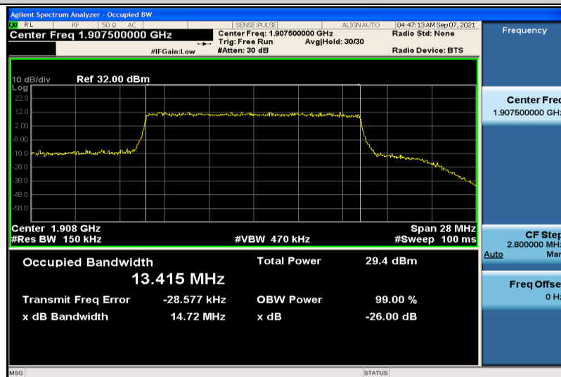
Band25-15MHz-16QAM-26615-75RB#0-13.415
