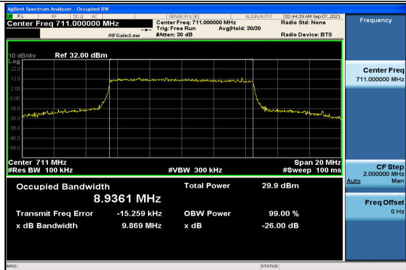
Band17-10MHz-16QAM-23800-50RB#0-8.9361
