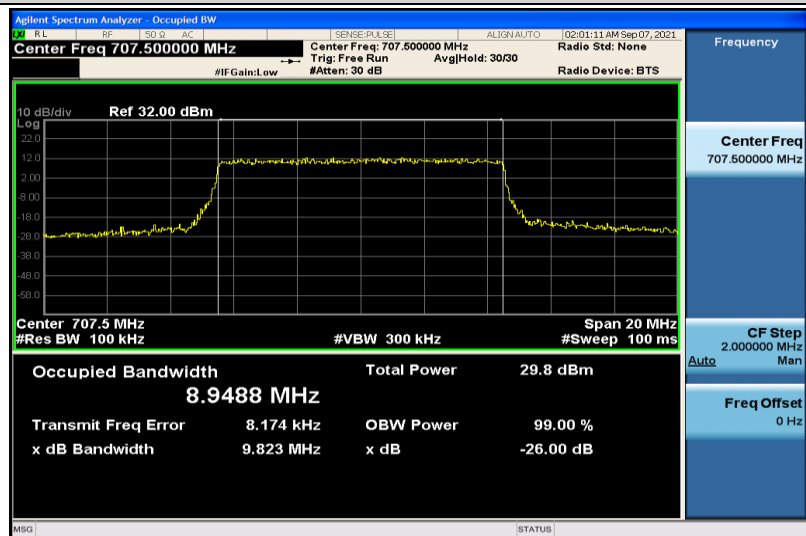
Band12-10MHz-16QAM-23095-50RB#0-8.9488
