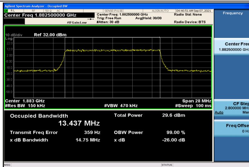
Band25-15MHz-16QAM-26365-75RB#0-13.437
