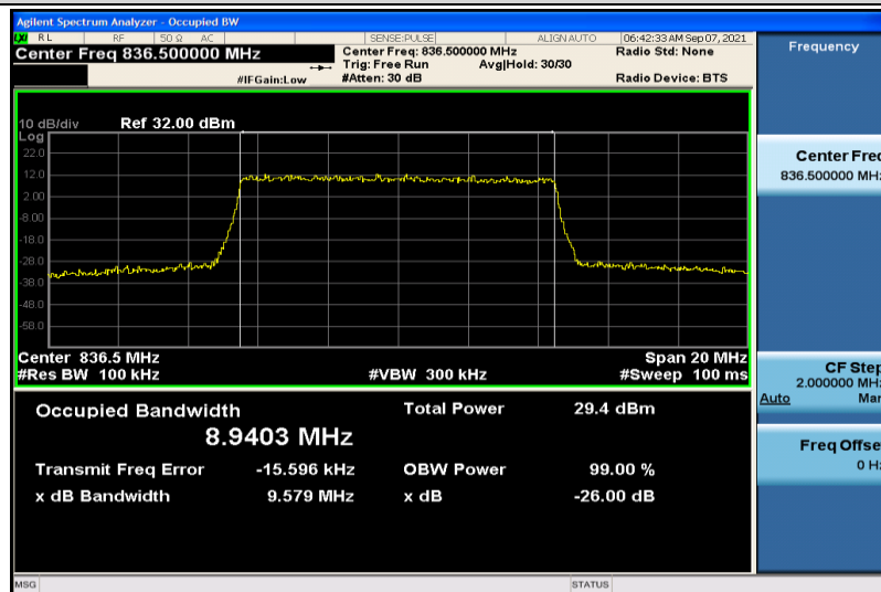
Band26-10MHz-16QAM-26915-50RB#0-8.9403
