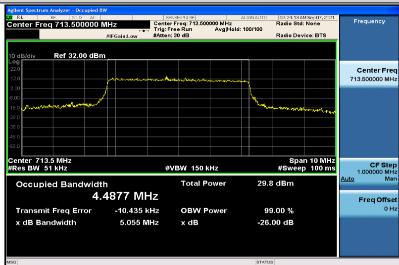
Band17-5MHz-16QAM-23825-25RB#0-4.4877
