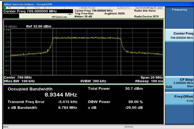
Band17-10MHz-QPSK-23780-50RB#0-8.9344
