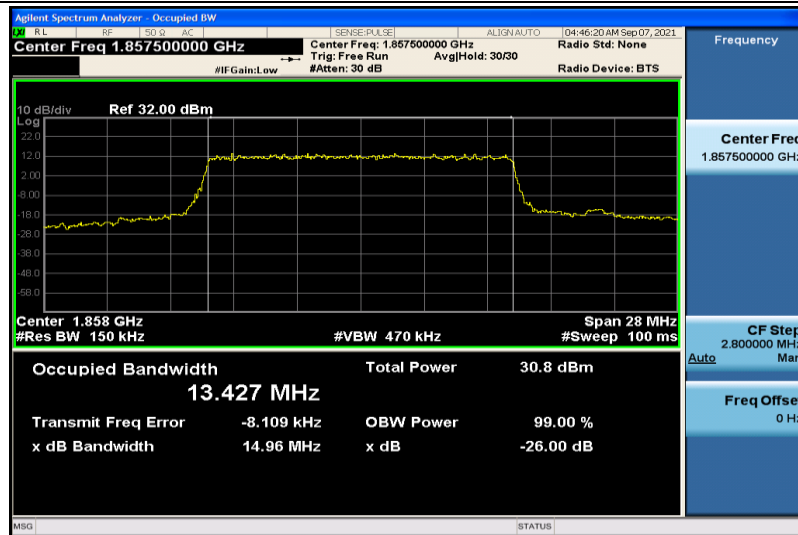
Band25-15MHz-QPSK-26115-75RB#0-13.427
