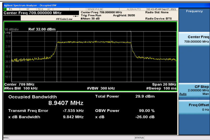
Band17-10MHz-16QAM-23780-50RB#0-8.9407
