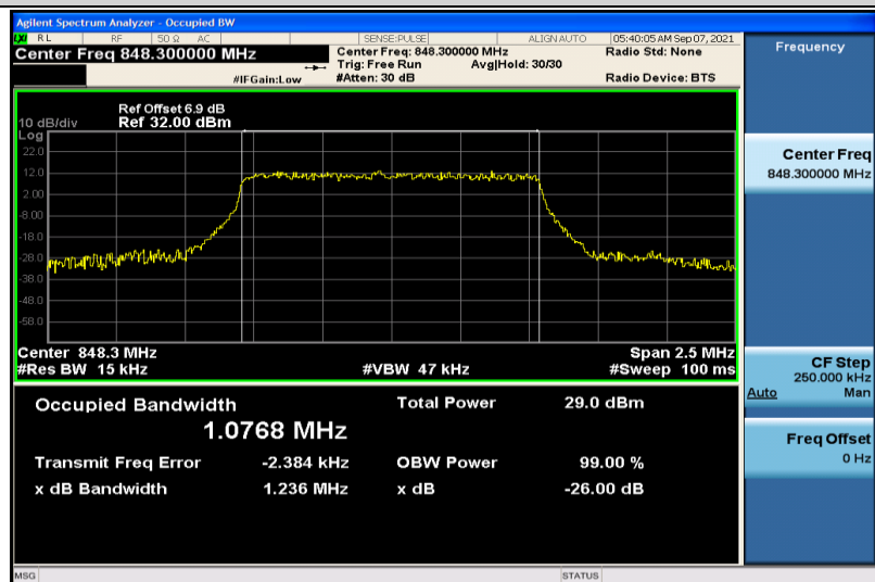
Band26-1.4MHz-QPSK-27033-6RB#0-1.0768
