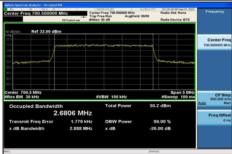
Band12-3MHz-QPSK-23025-15RB#0-2.6806
