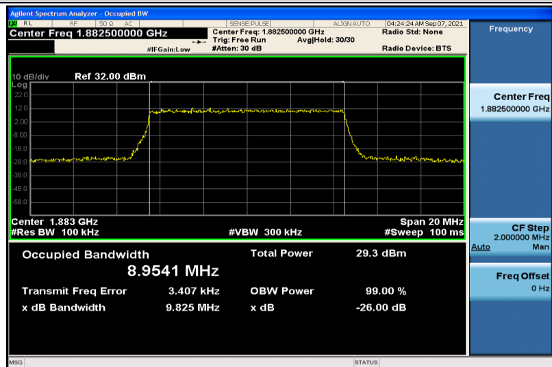
Band25-10MHz-16QAM-26365-50RB#0-8.9541
