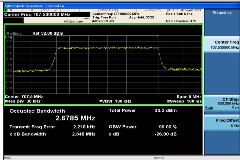
Band12-3MHz-QPSK-23095-15RB#0-2.6785
