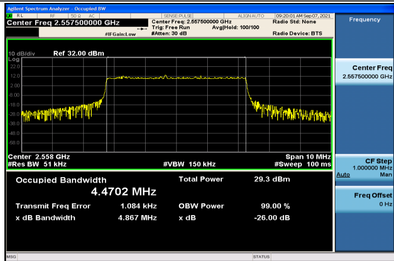
Band41-5MHz-QPSK-40265-25RB#0-4.4702
