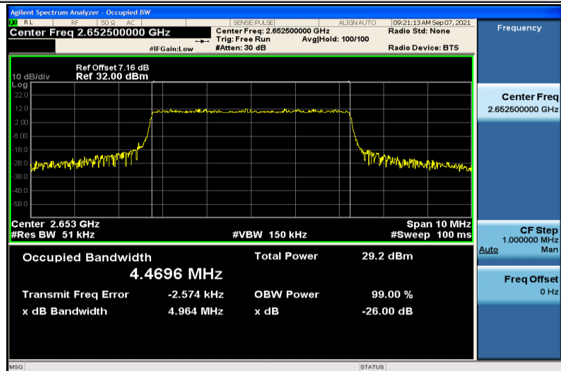
Band41-5MHz-QPSK-41215-25RB#0-4.4696
