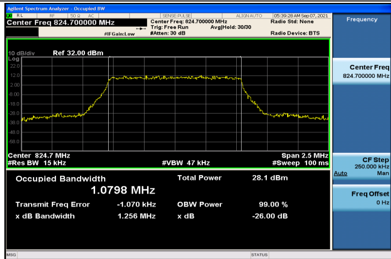
Band26-1.4MHz-16QAM-26797-6RB#0-1.0798
