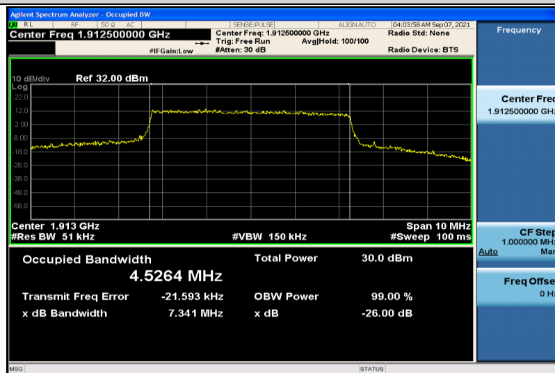
Band25-5MHz-QPSK-26665-25RB#0-4.5264
