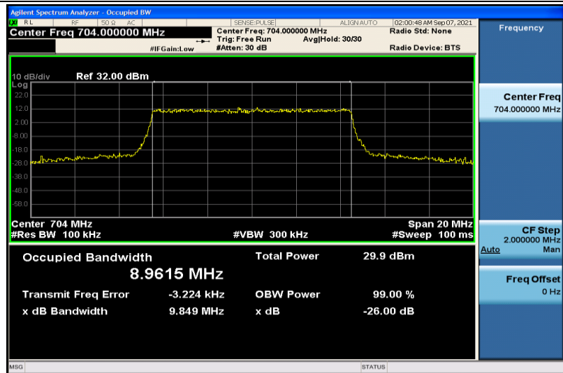
Band12-10MHz-16QAM-23060-50RB#0-8.9615
