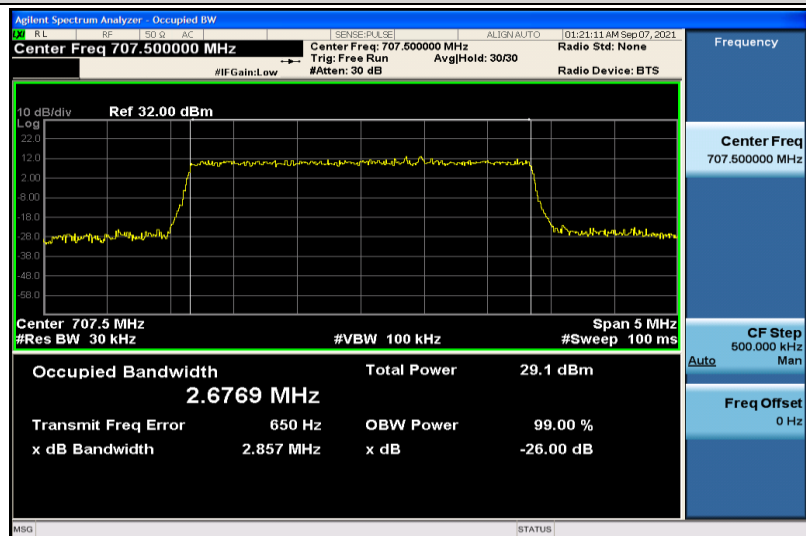
Band12-3MHz-16QAM-23095-15RB#0-2.6769
