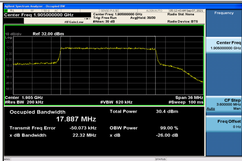
Band25-20MHz-QPSK-26590-100RB#0-17.887
