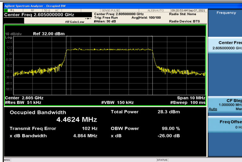
Band41-5MHz-16QAM-40740-25RB#0-4.4624
