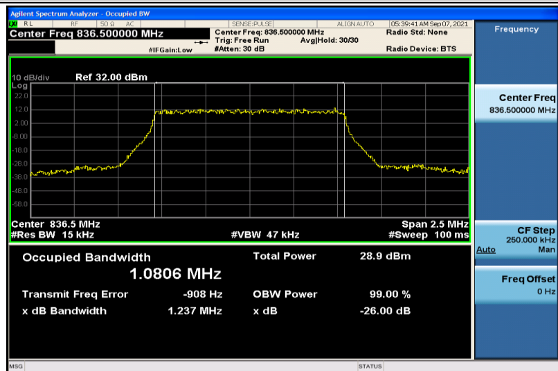
Band26-1.4MHz-QPSK-26915-6RB#0-1.0806
