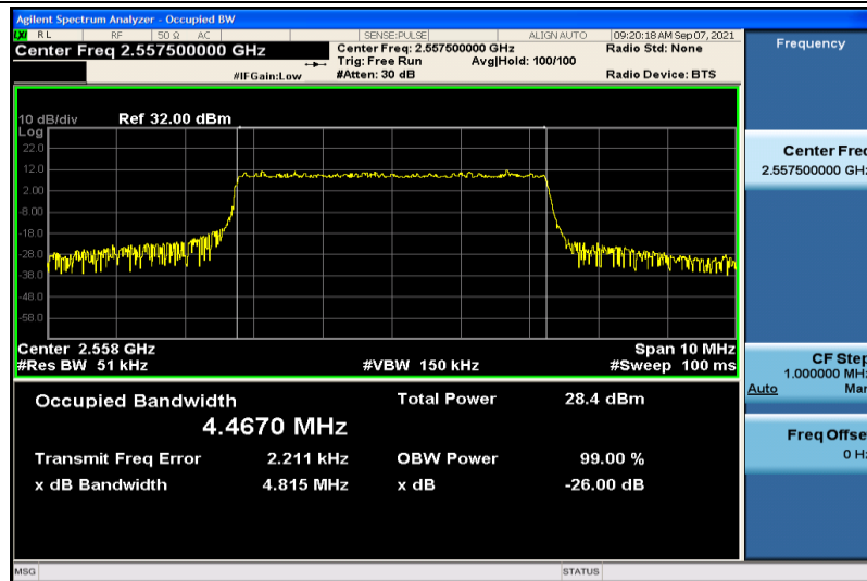
Band41-5MHz-16QAM-40265-25RB#0-4.4670
