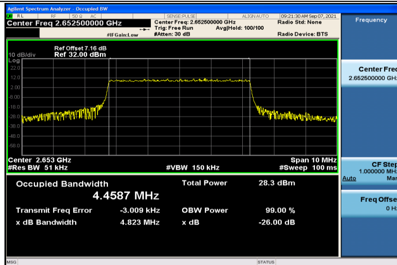
Band41-5MHz-16QAM-41215-25RB#0-4.4587
