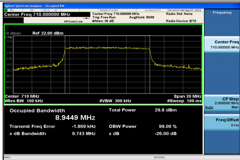
Band17-10MHz-16QAM-23790-50RB#0-8.9449
