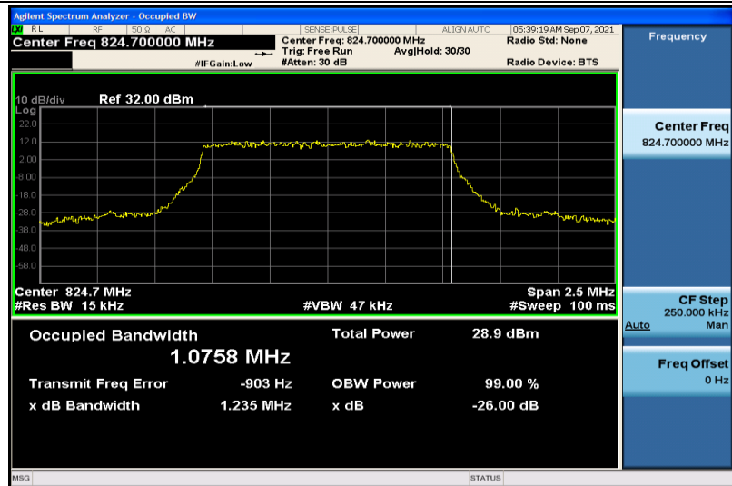
Band26-1.4MHz-QPSK-26797-6RB#0-1.0758
