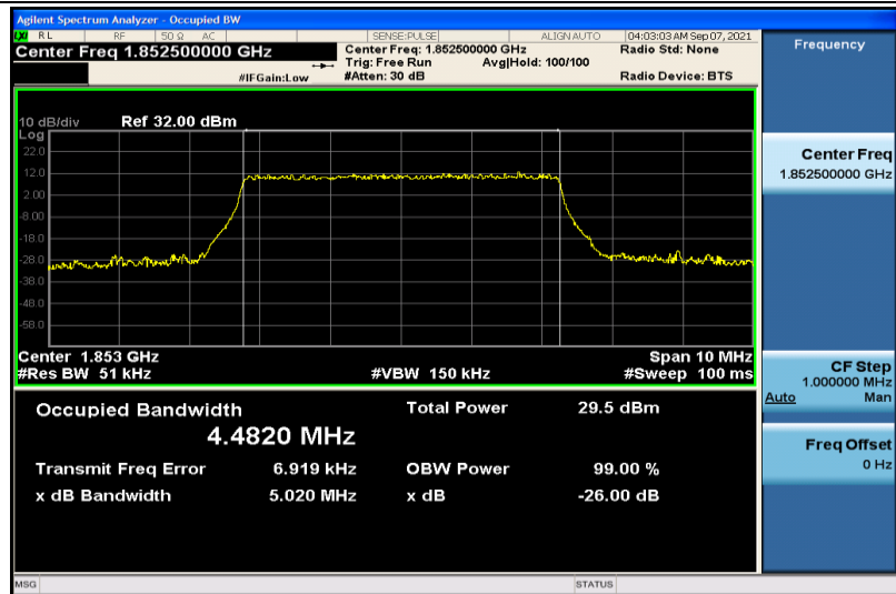
Band25-5MHz-16QAM-26065-25RB#0-4.4820
