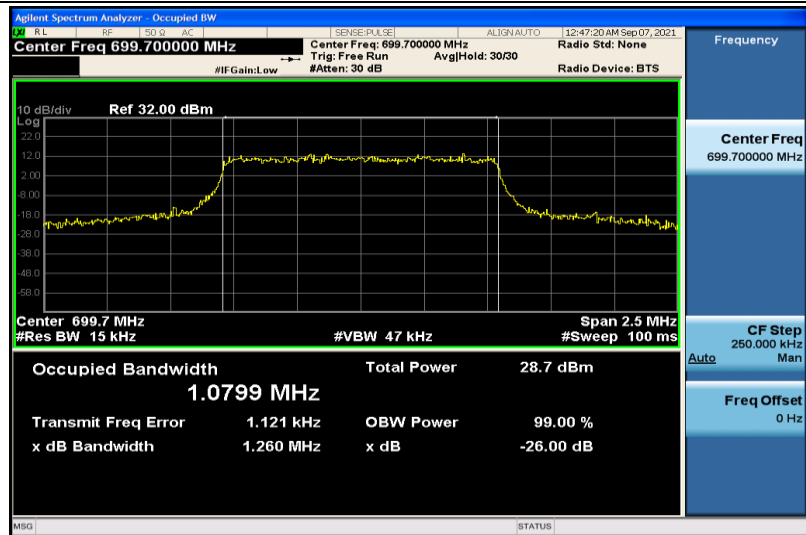
Band12-1.4MHz-16QAM-23017-6RB#0-1.0799
