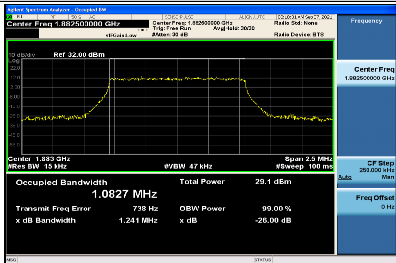
Band25-1.4MHz-QPSK-26365-6RB#0-1.0827
