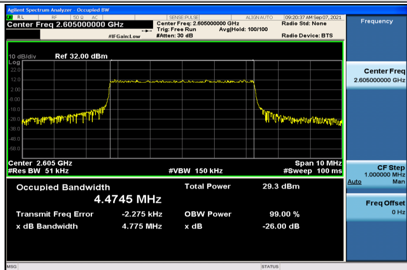
Band41-5MHz-QPSK-40740-25RB#0-4.4745
