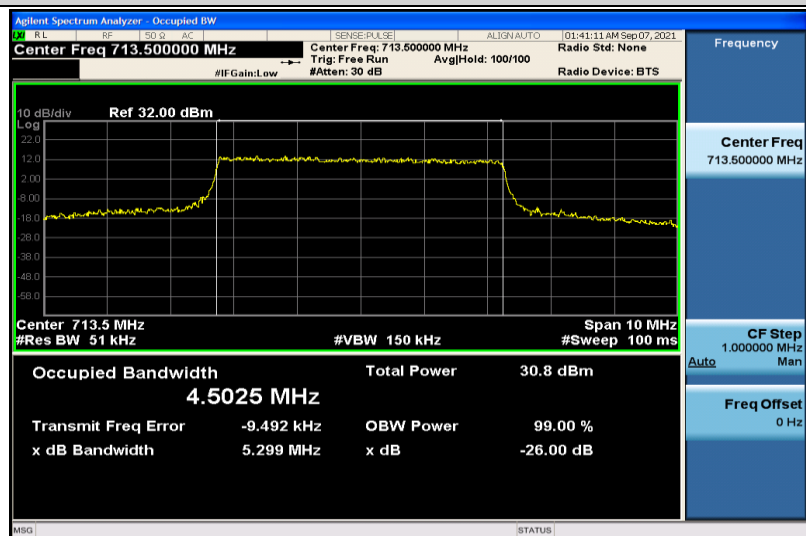
Band12-5MHz-QPSK-23155-25RB#0-4.5025
