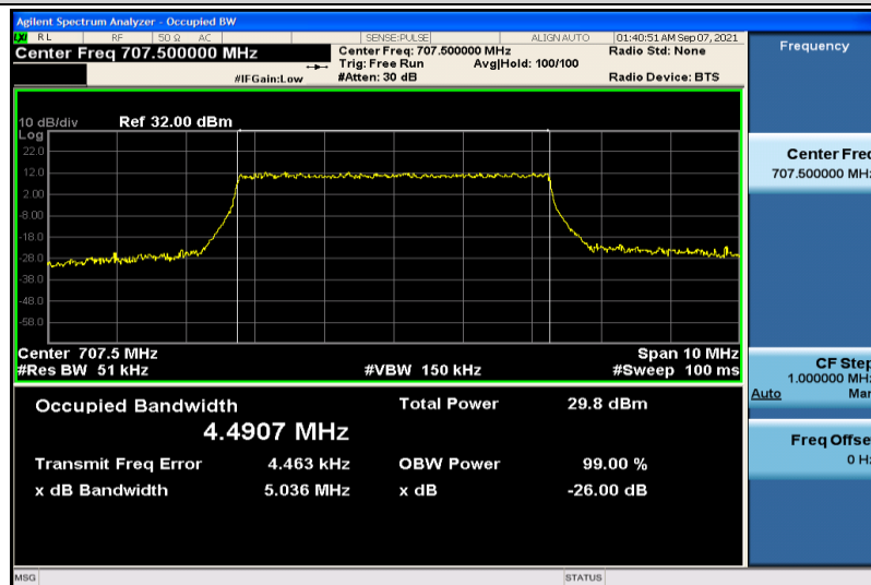
Band12-5MHz-16QAM-23095-25RB#0-4.4907
