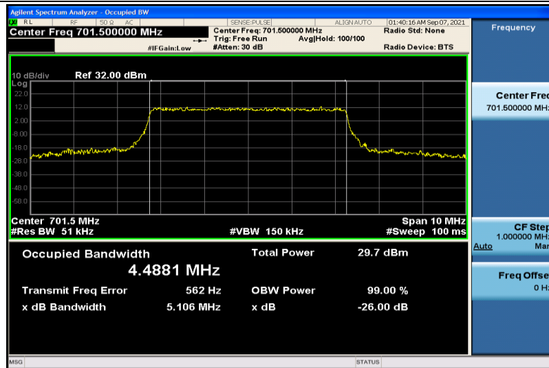
Band12-5MHz-16QAM-23035-25RB#0-4.4881
