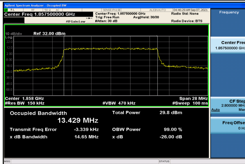
Band25-15MHz-16QAM-26115-75RB#0-13.429
