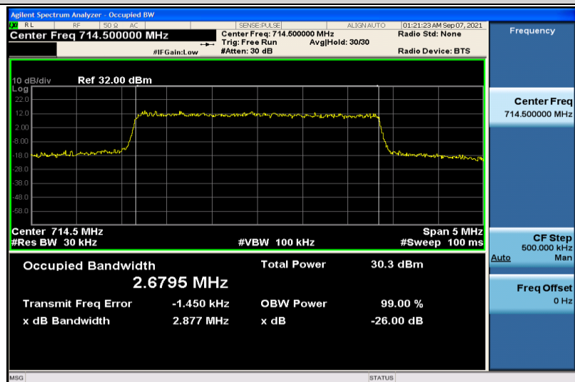
Band12-3MHz-QPSK-23165-15RB#0-2.6795
