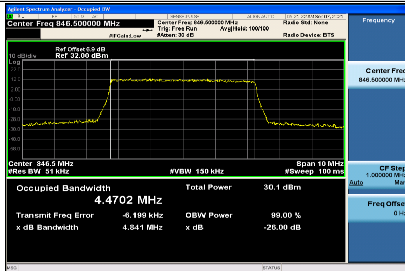
Band26-5MHz-QPSK-27015-25RB#0-4.4702
