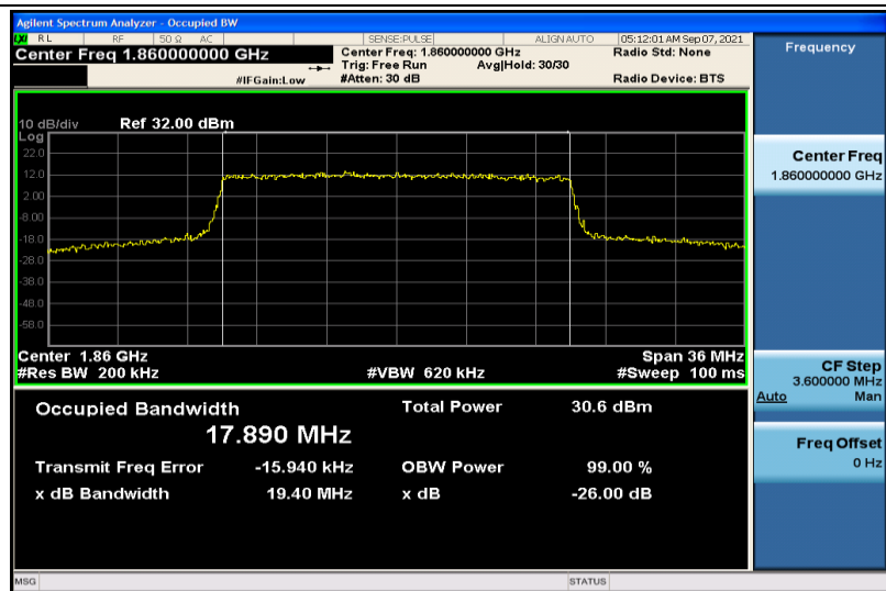
Band25-20MHz-QPSK-26140-100RB#0-17.890
