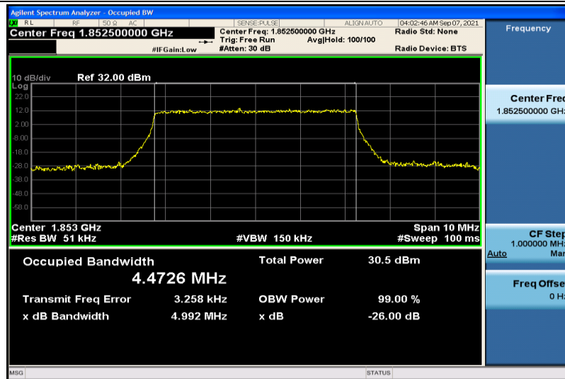
Band25-5MHz-QPSK-26065-25RB#0-4.4726
