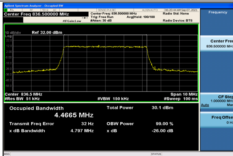
Band26-5MHz-QPSK-26915-25RB#0-4.4665
