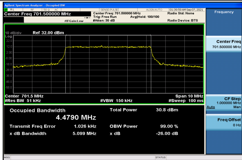
Band12-5MHz-QPSK-23035-25RB#0-4.4790
