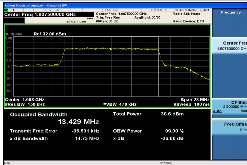
Band25-15MHz-QPSK-26615-75RB#0-13.429
