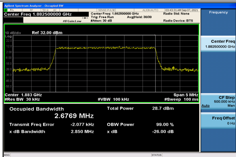
Band25-3MHz-16QAM-26365-15RB#0-2.6769
