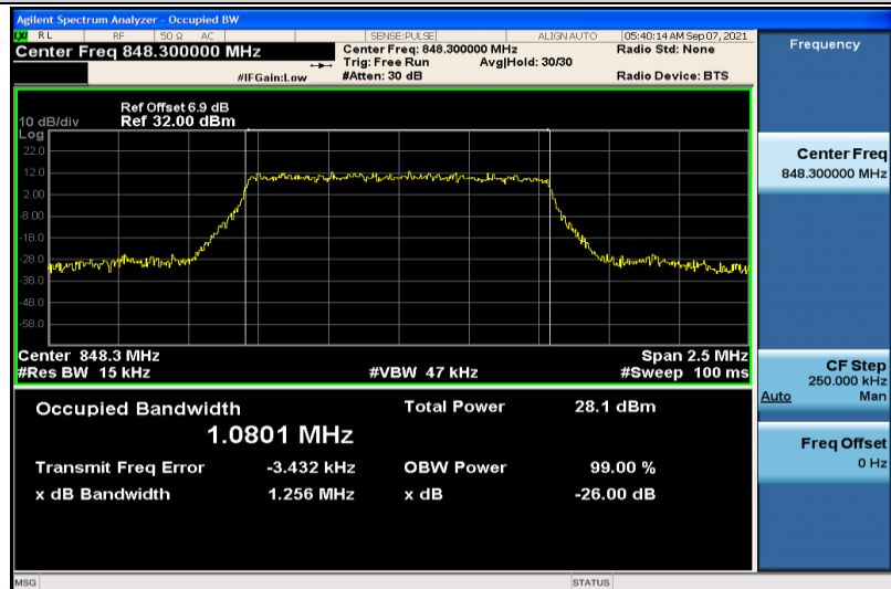
Band26-1.4MHz-16QAM-27033-6RB#0-1.0801
