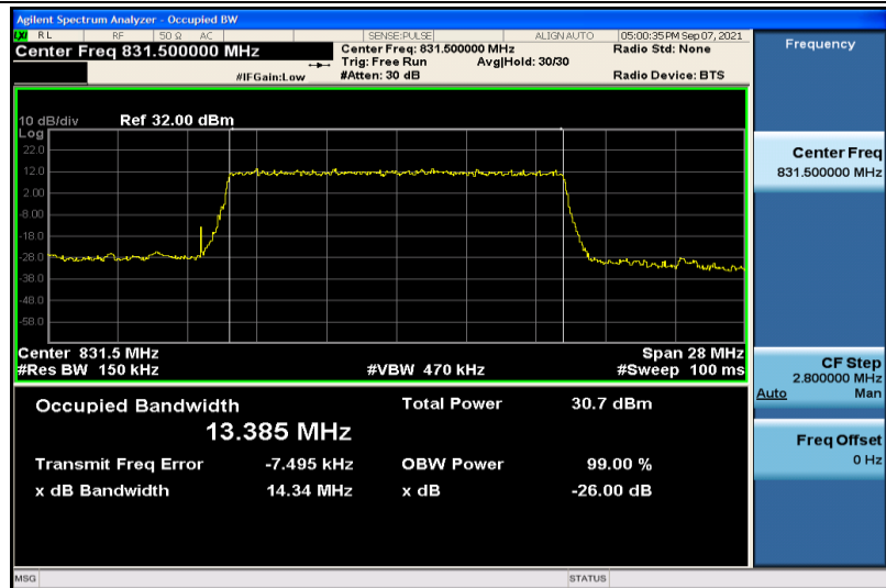
Band26-15MHz-QPSK-26865-75RB#0-13.385
