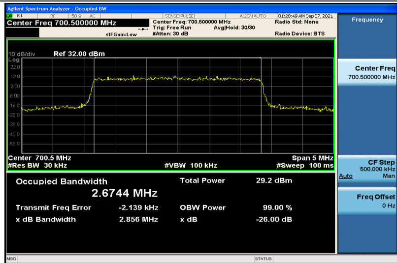
Band12-3MHz-16QAM-23025-15RB#0-2.6744
