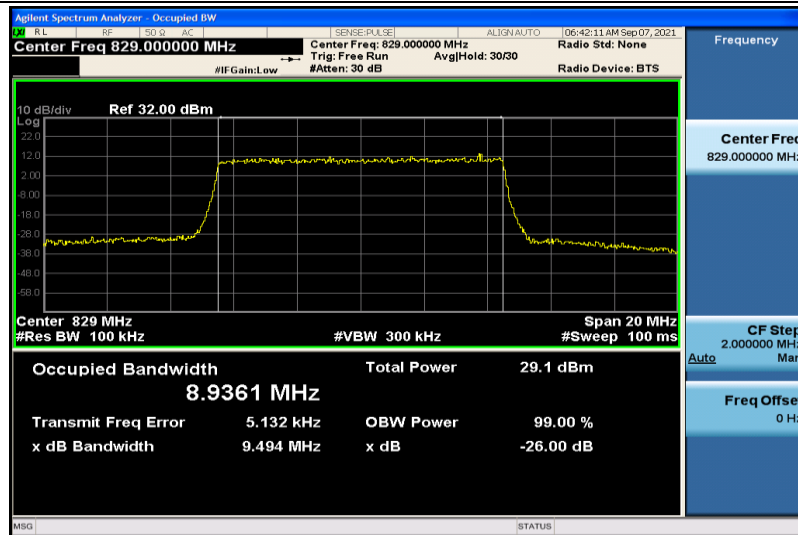
Band26-10MHz-16QAM-26840-50RB#0-8.9361
