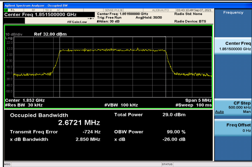
Band25-3MHz-16QAM-26055-15RB#0-2.6721
