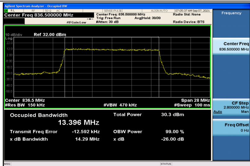
Band26-15MHz-QPSK-26915-75RB#0-13.396
