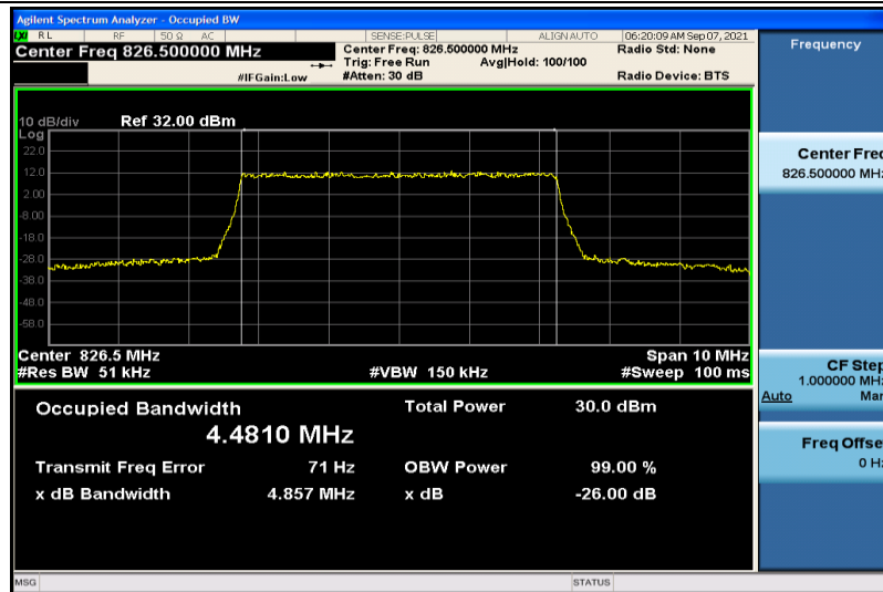
Band26-5MHz-QPSK-26815-25RB#0-4.4810
