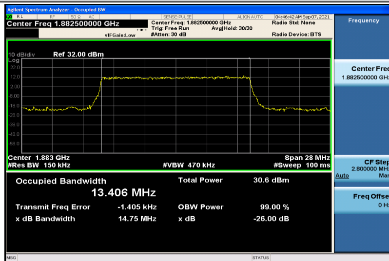
Band25-15MHz-QPSK-26365-75RB#0-13.406
