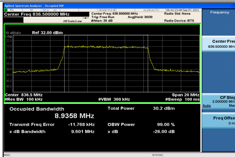
Band26-10MHz-QPSK-26915-50RB#0-8.9358
