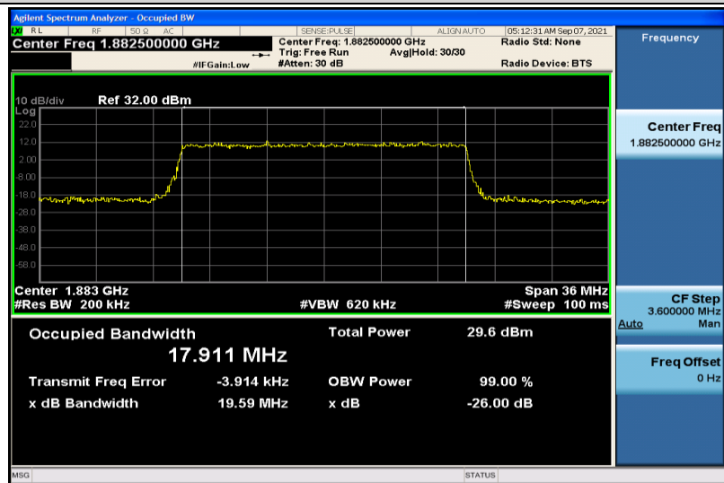
Band25-20MHz-16QAM-26365-100RB#0-17.911
