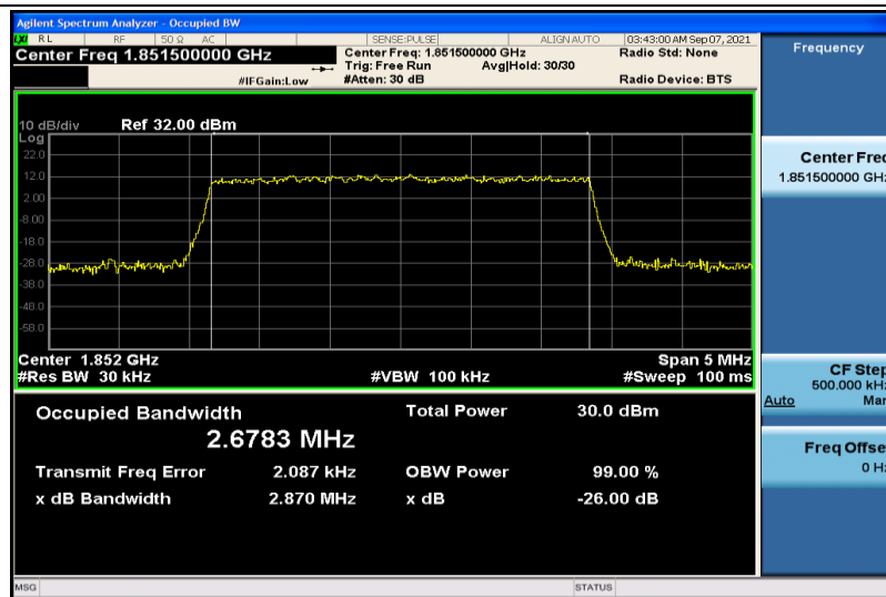
Band25-3MHz-QPSK-26055-15RB#0-2.6783
