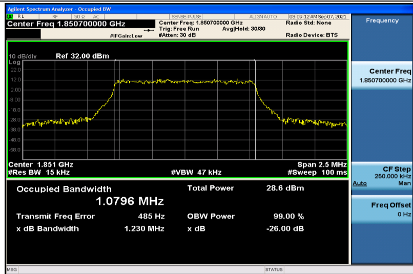
Band25-1.4MHz-16QAM-26047-6RB#0-1.0796
