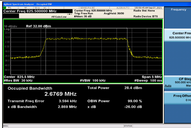
Band26-3MHz-16QAM-26805-15RB#0-2.6769
