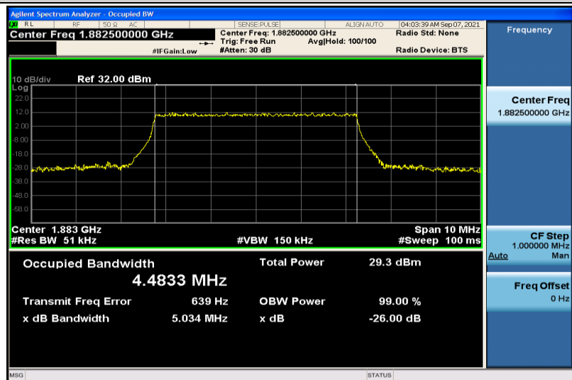
Band25-5MHz-16QAM-26365-25RB#0-4.4833
