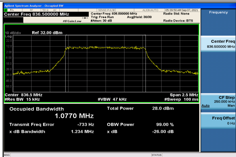
Band26-1.4MHz-16QAM-26915-6RB#0-1.0770
