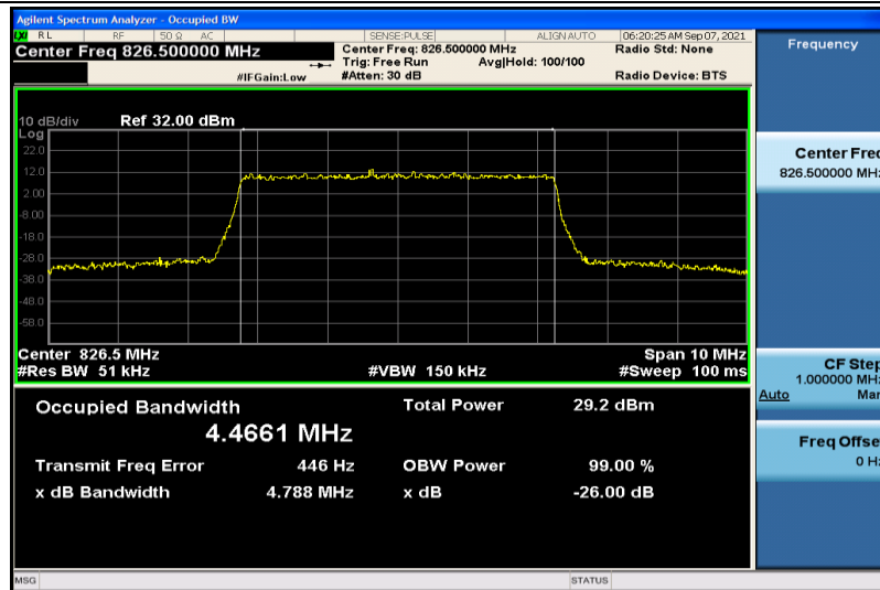
Band26-5MHz-16QAM-26815-25RB#0-4.4661
