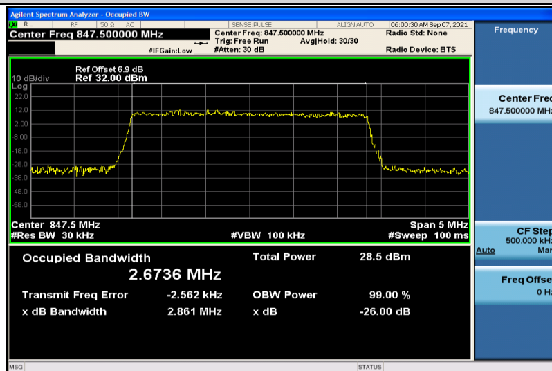
Band26-3MHz-16QAM-27025-15RB#0-2.6736
