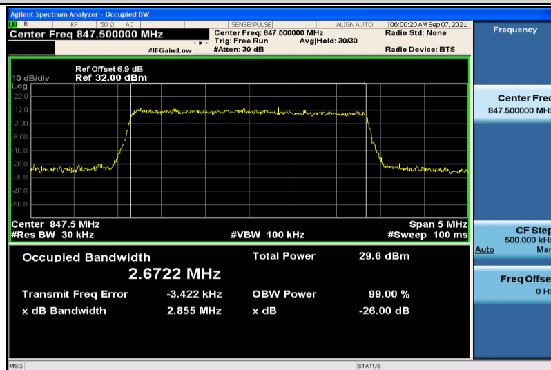
Band26-3MHz-QPSK-27025-15RB#0-2.6722
