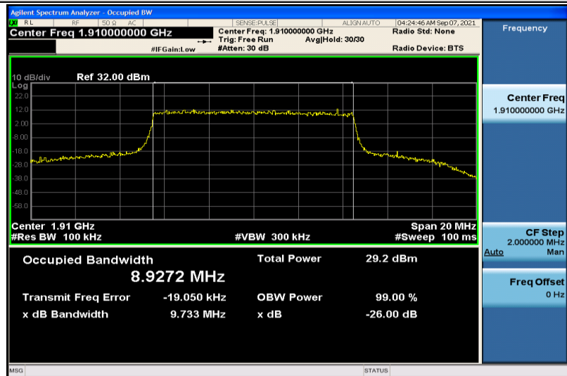
Band25-10MHz-16QAM-26640-50RB#0-8.9272
