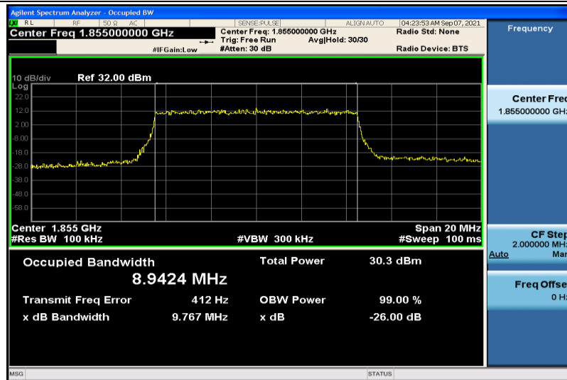
Band25-10MHz-QPSK-26090-50RB#0-8.9424
