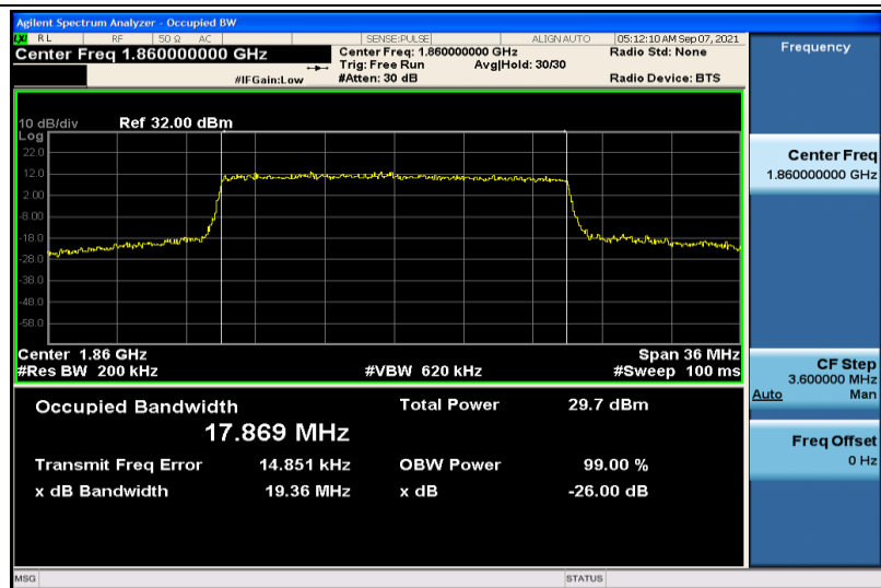
Band25-20MHz-16QAM-26140-100RB#0-17.869
