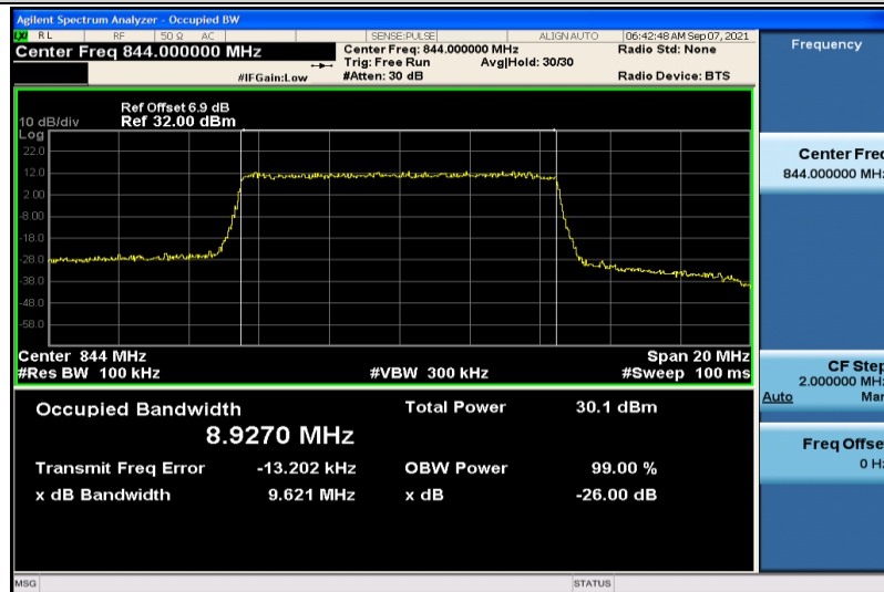
Band26-10MHz-QPSK-26990-50RB#0-8.9270
