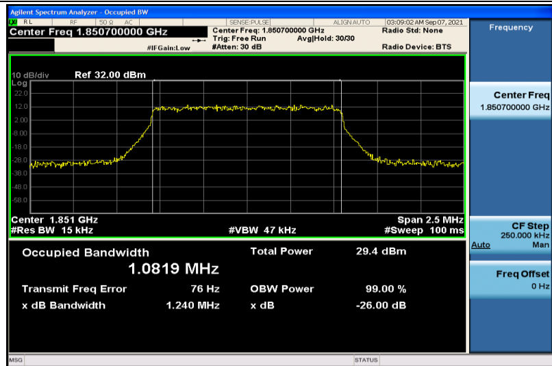
Band25-1.4MHz-QPSK-26047-6RB#0-1.0819
