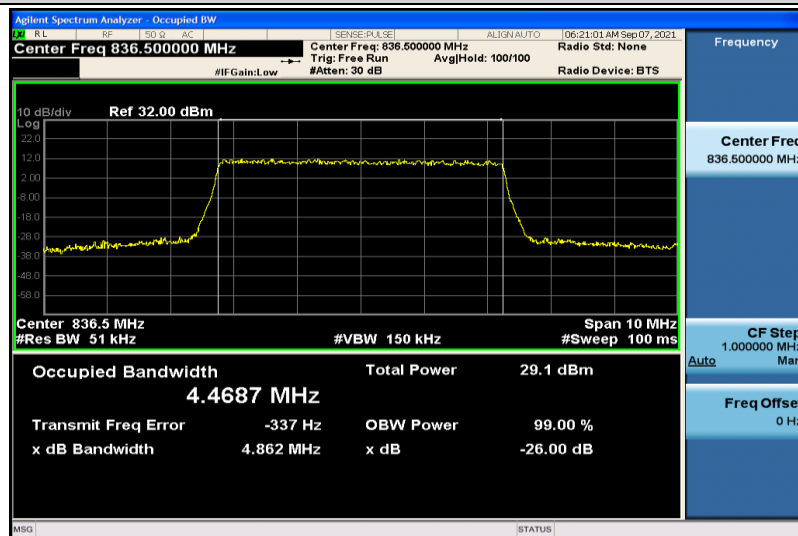
Band26-5MHz-16QAM-26915-25RB#0-4.4687
