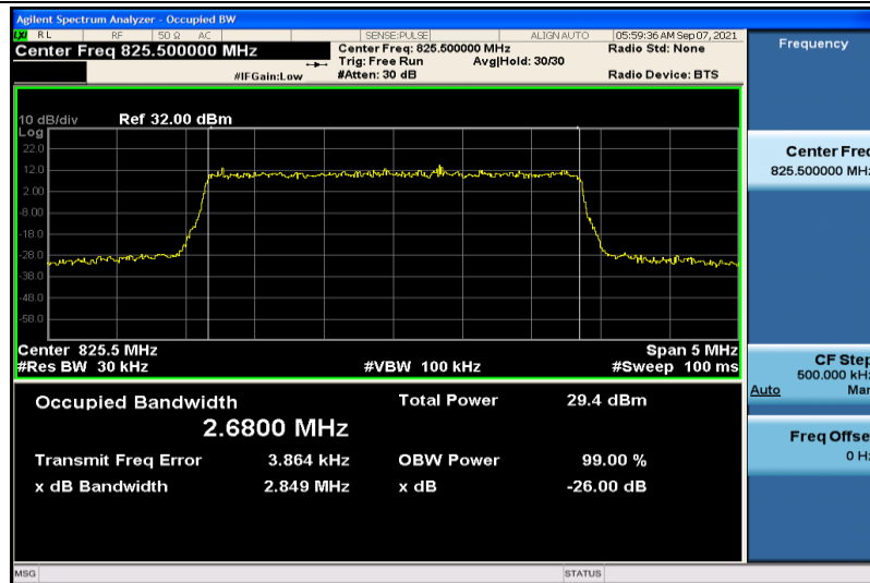
Band26-3MHz-QPSK-26805-15RB#0-2.6800
