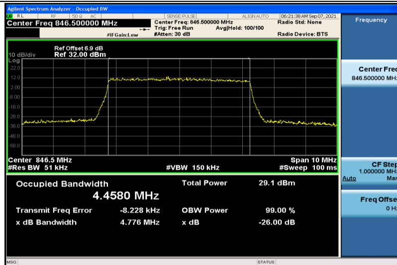
Band26-5MHz-16QAM-27015-25RB#0-4.4580
