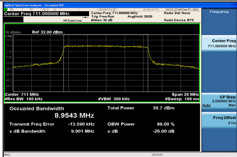
Band12-10MHz-QPSK-23130-50RB#0-8.9543
