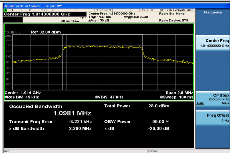
Band25-1.4MHz-16QAM-26683-6RB#0-1.0981
