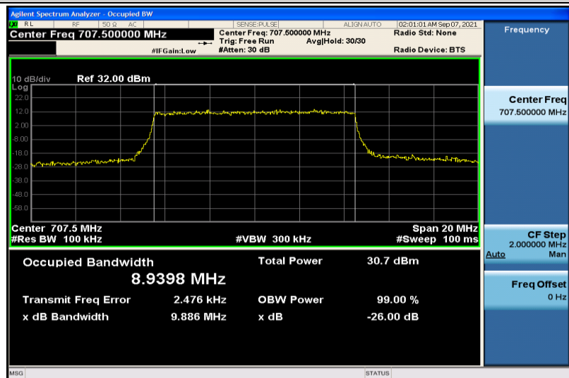
Band12-10MHz-QPSK-23095-50RB#0-8.9398
