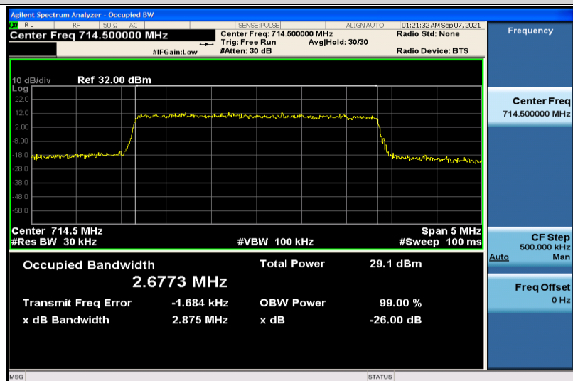
Band12-3MHz-16QAM-23165-15RB#0-2.6773
