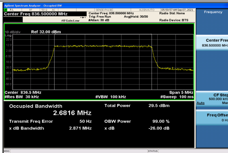
Band26-3MHz-QPSK-26915-15RB#0-2.6816
