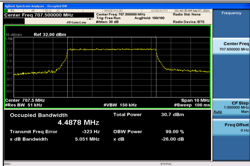
Band12-5MHz-QPSK-23095-25RB#0-4.4878
