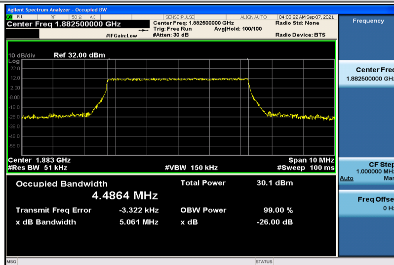
Band25-5MHz-QPSK-26365-25RB#0-4.4864
