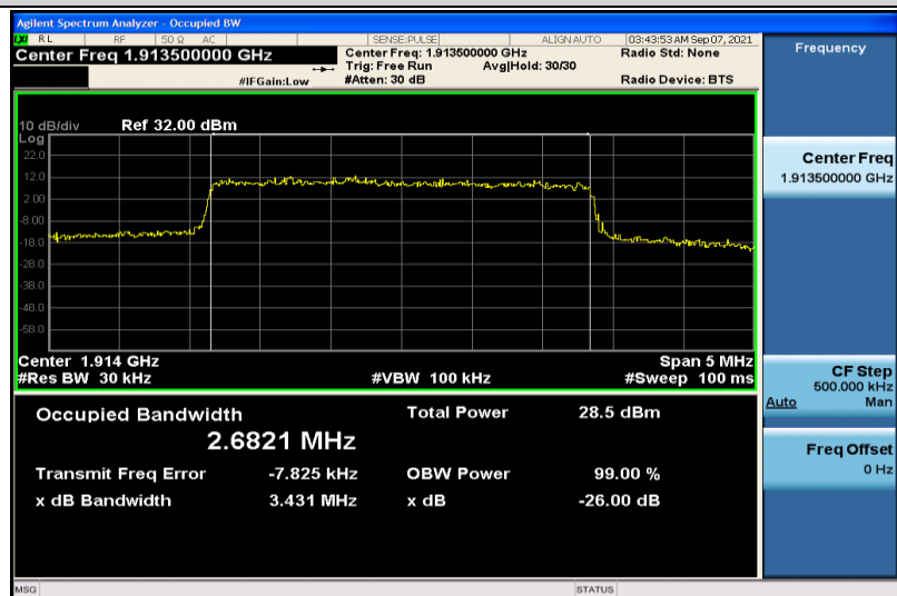
Band25-3MHz-16QAM-26675-15RB#0-2.6821
