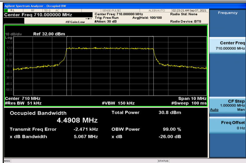
Band17-5MHz-QPSK-23790-25RB#0-4.4908
