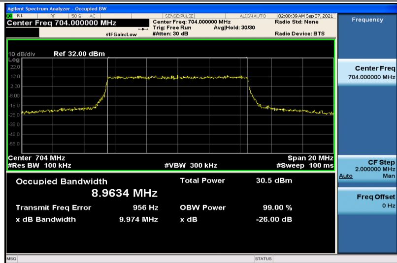
Band12-10MHz-QPSK-23060-50RB#0-8.9634
