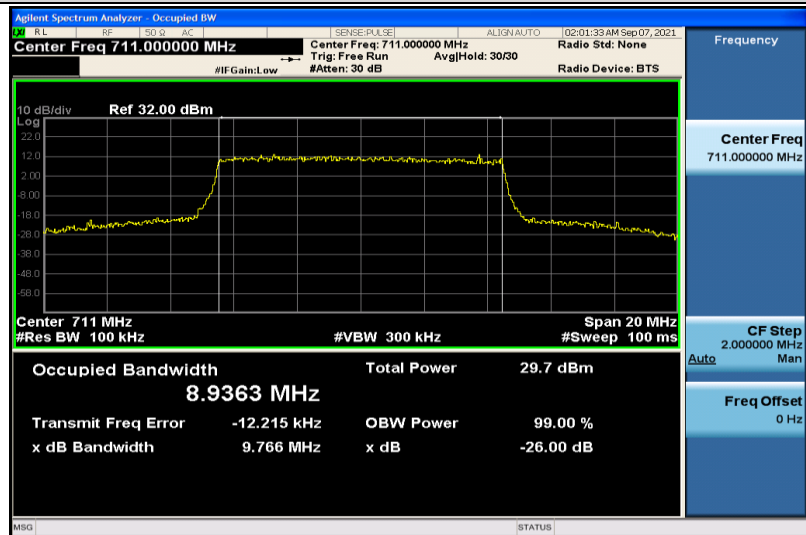
Band12-10MHz-16QAM-23130-50RB#0-8.9363
