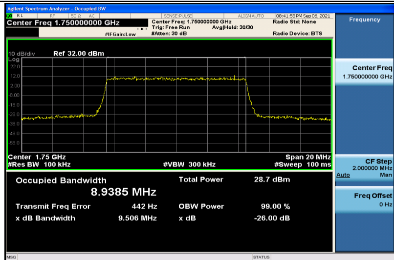
Band4-10MHz-16QAM-20350-50RB#0-8.9385
