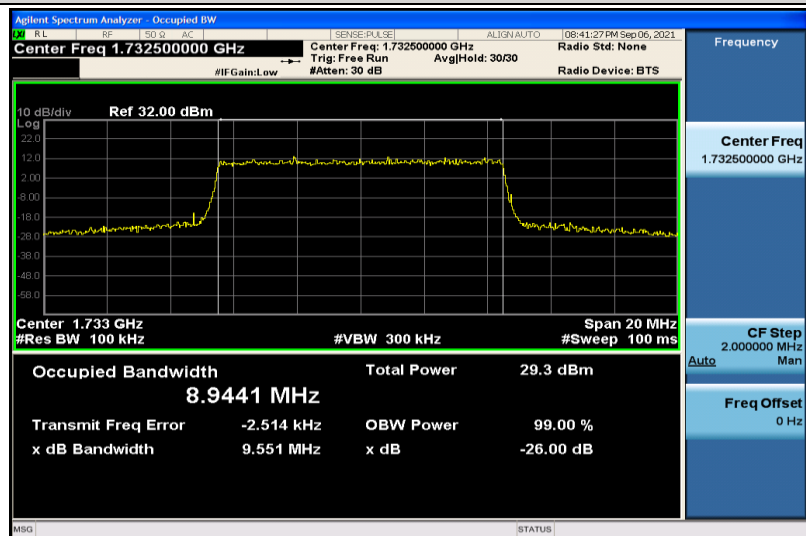
Band4-10MHz-QPSK-20175-50RB#0-8.9441
