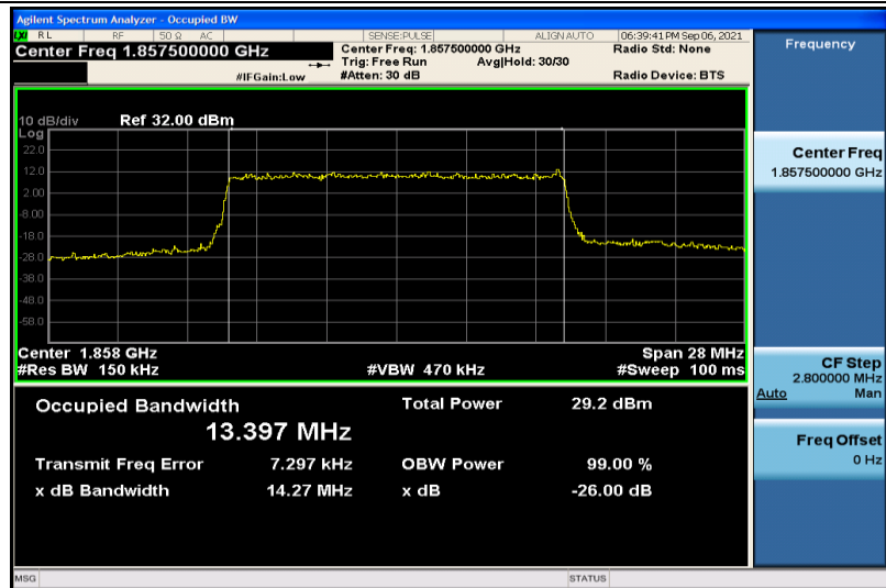
Band2-15MHz-16QAM-18675-75RB#0-13.397
