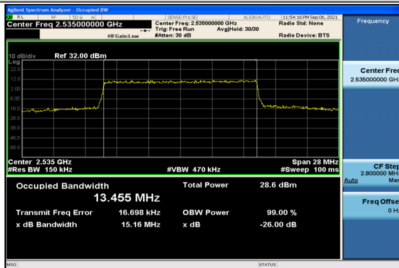
Band7-15MHz-16QAM-21100-75RB#0-13.455
