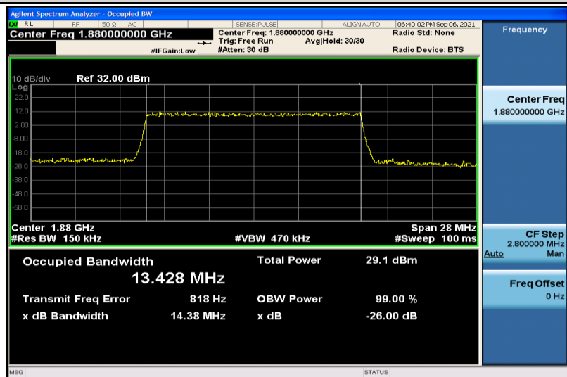
Band2-15MHz-16QAM-18900-75RB#0-13.428
