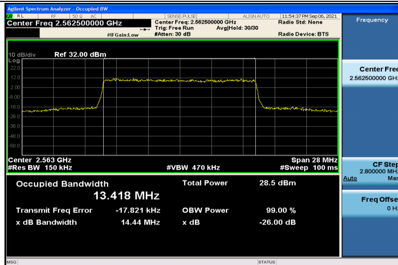
Band7-15MHz-16QAM-21375-75RB#0-13.418
