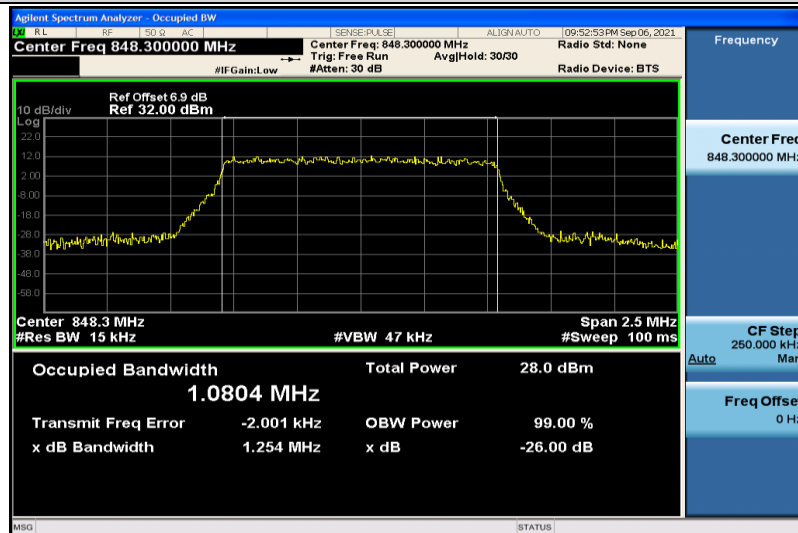
Band5-1.4MHz-16QAM-20643-6RB#0-1.0804
