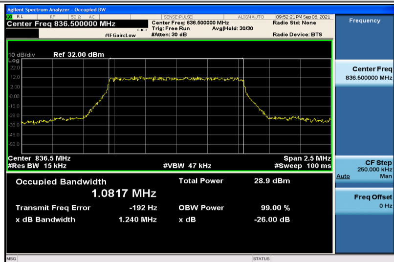
Band5-1.4MHz-QPSK-20525-6RB#0-1.0817
