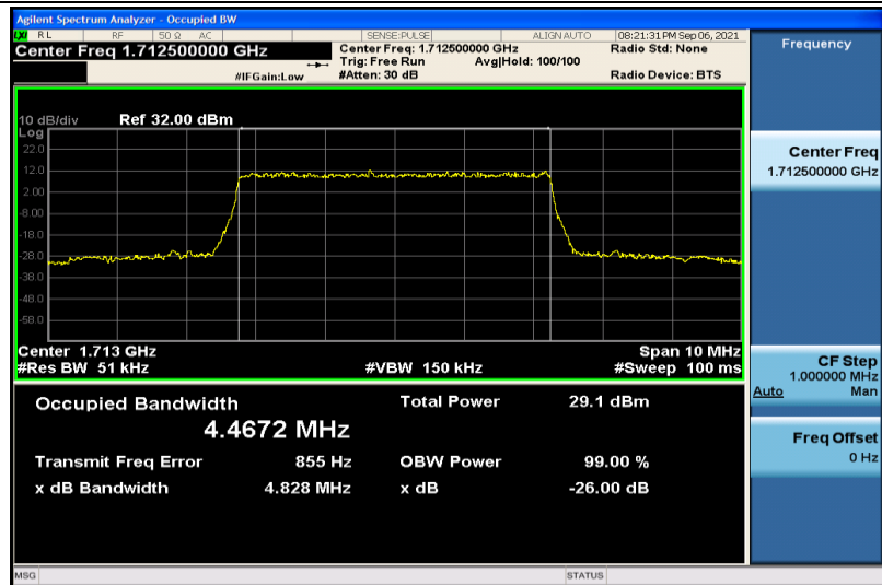
Band4-5MHz-QPSK-19975-25RB#0-4.4672
