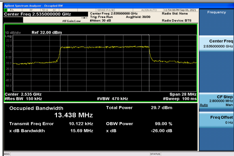
Band7-15MHz-QPSK-21100-75RB#0-13.438
