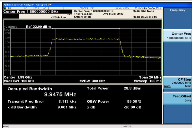
Band2-10MHz-16QAM-18900-50RB#0-8.9475
