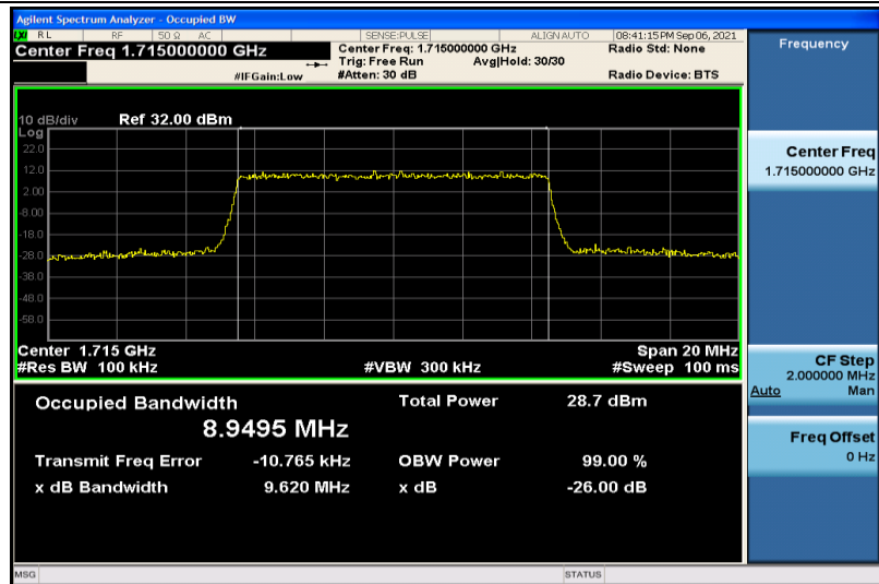
Band4-10MHz-16QAM-20000-50RB#0-8.9495
