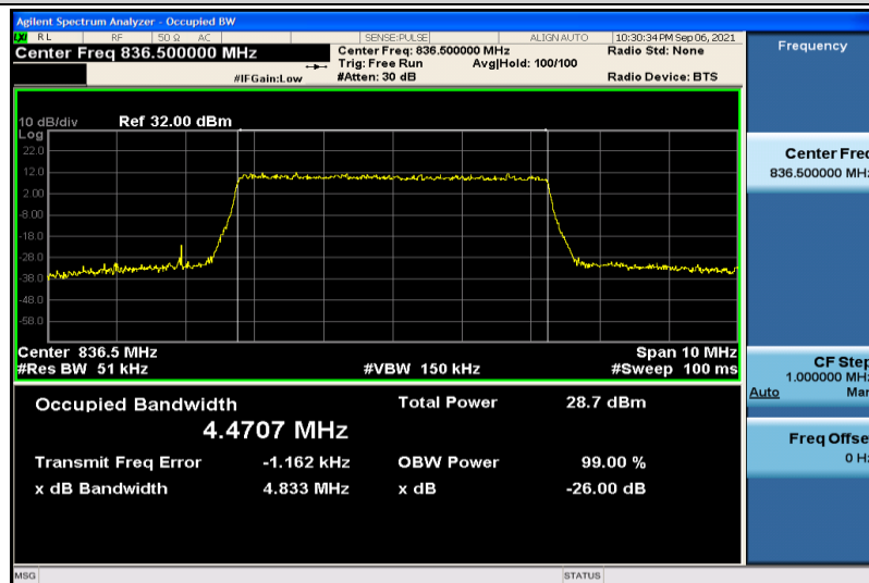
Band5-5MHz-16QAM-20525-25RB#0-4.4707
