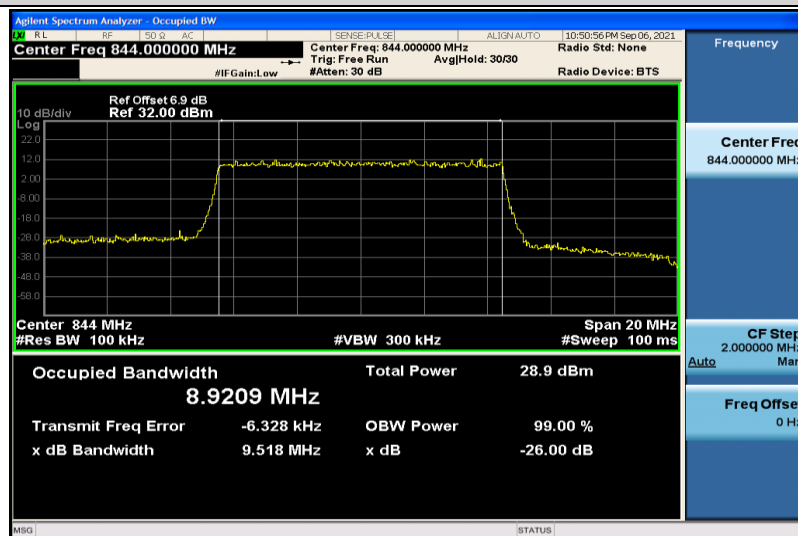
Band5-10MHz-16QAM-20600-50RB#0-8.9209
