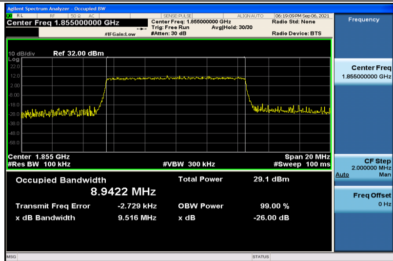
Band2-10MHz-16QAM-18650-50RB#0-8.9422
