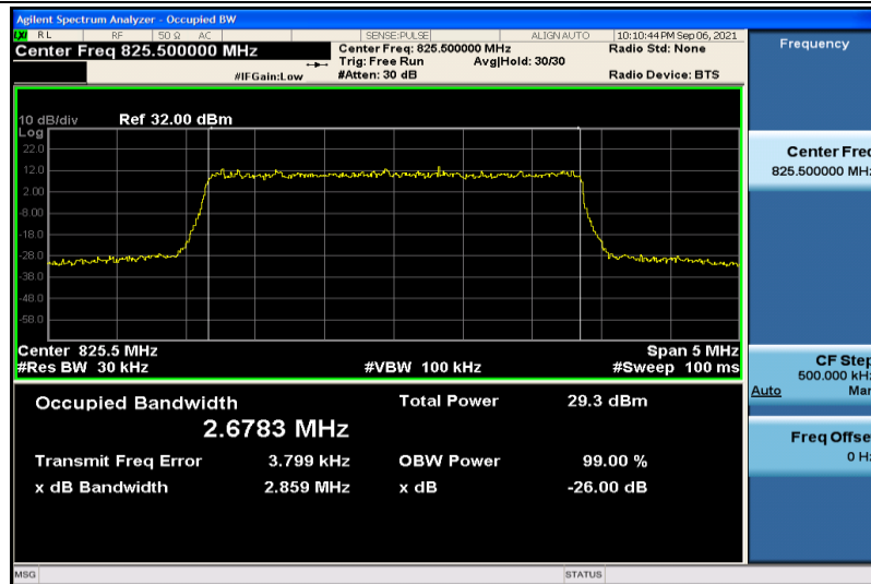
Band5-3MHz-QPSK-20415-15RB#0-2.6783
