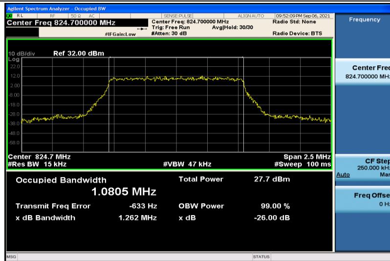
Band5-1.4MHz-16QAM-20407-6RB#0-1.0805
