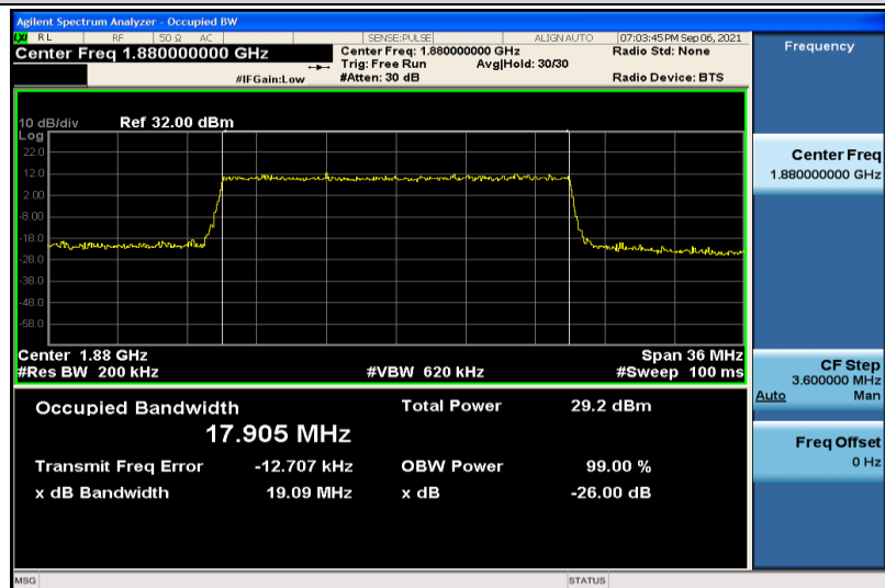
Band2-20MHz-16QAM-18900-100RB#0-17.905
