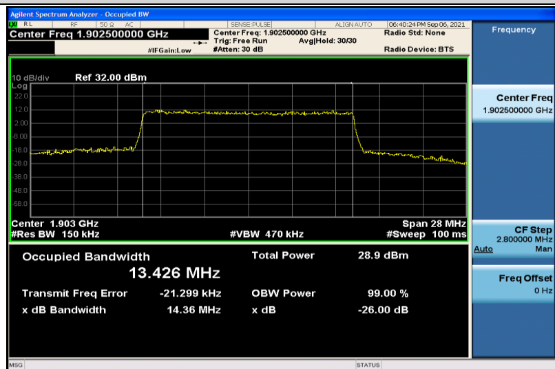
Band2-15MHz-16QAM-19125-75RB#0-13.426
