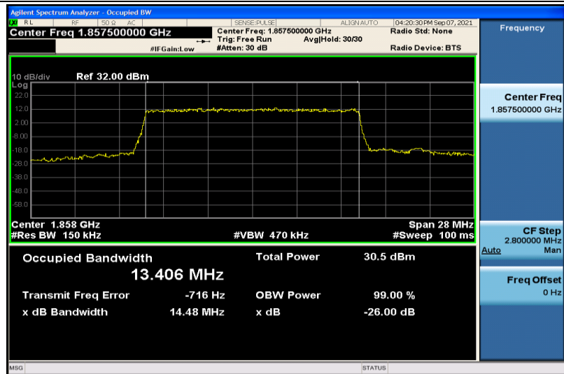
Band2-15MHz-QPSK-18675-75RB#0-13.406
