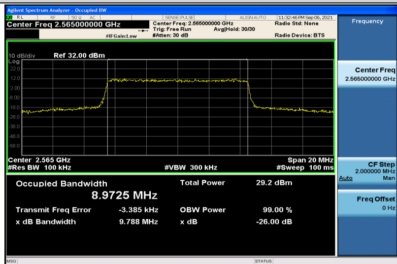
Band7-10MHz-QPSK-21400-50RB#0-8.9725
