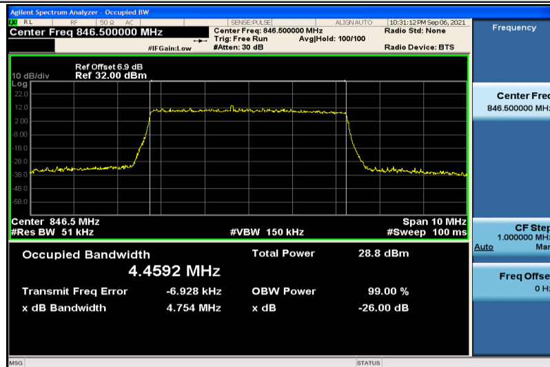
Band5-5MHz-16QAM-20625-25RB#0-4.4592
