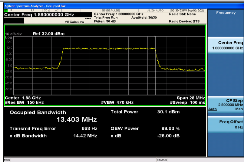
Band2-15MHz-QPSK-18900-75RB#0-13.403
