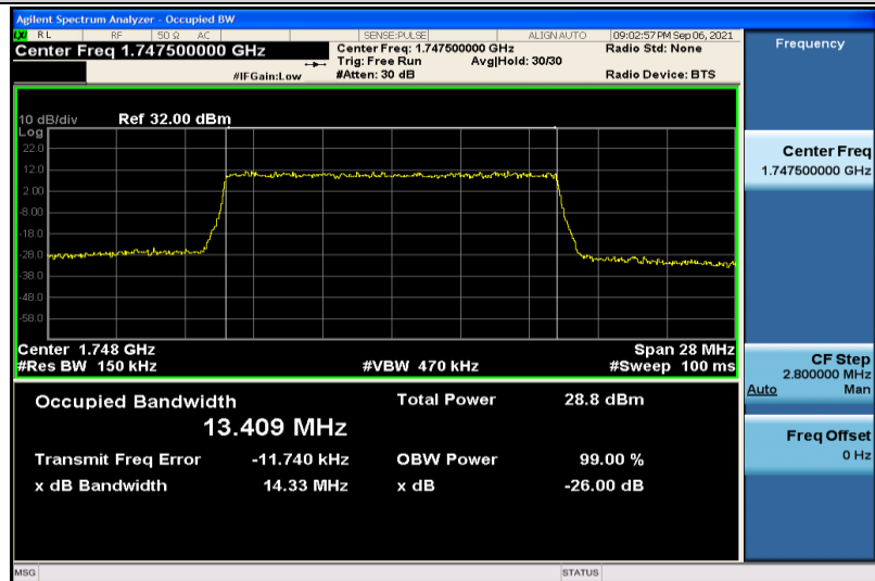
Band4-15MHz-16QAM-20325-75RB#0-13.409
