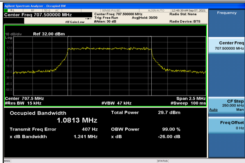
Band12-1.4MHz-QPSK-23095-6RB#0-1.0813
