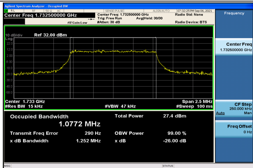
Band4-1.4MHz-16QAM-20175-6RB#0-1.0772
