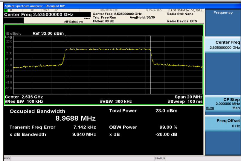
Band7-10MHz-16QAM-21100-50RB#0-8.9688
