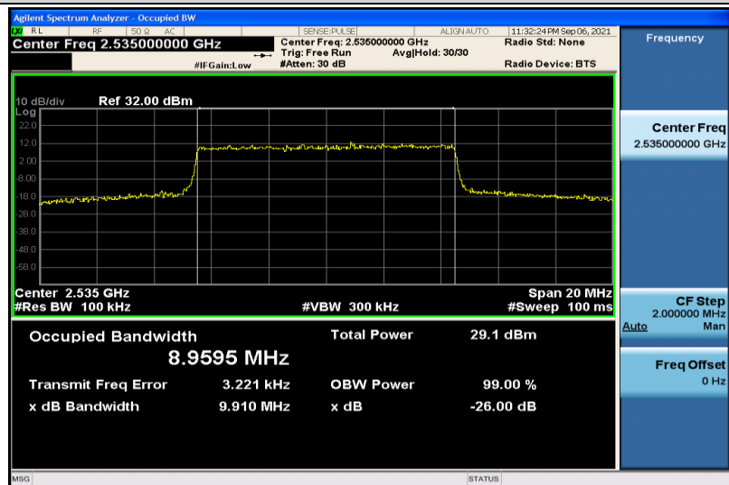
Band7-10MHz-QPSK-21100-50RB#0-8.9595
