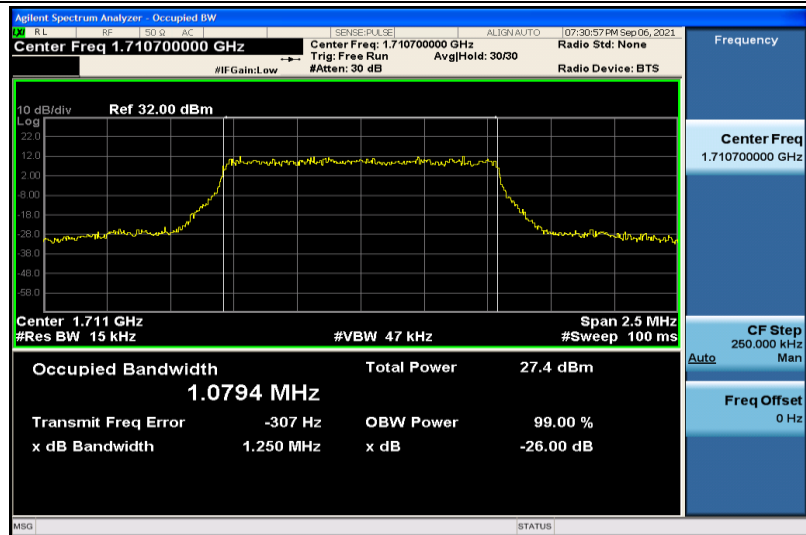
Band4-1.4MHz-16QAM-19957-6RB#0-1.0794
