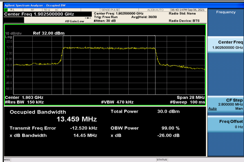
Band2-15MHz-QPSK-19125-75RB#0-13.459
