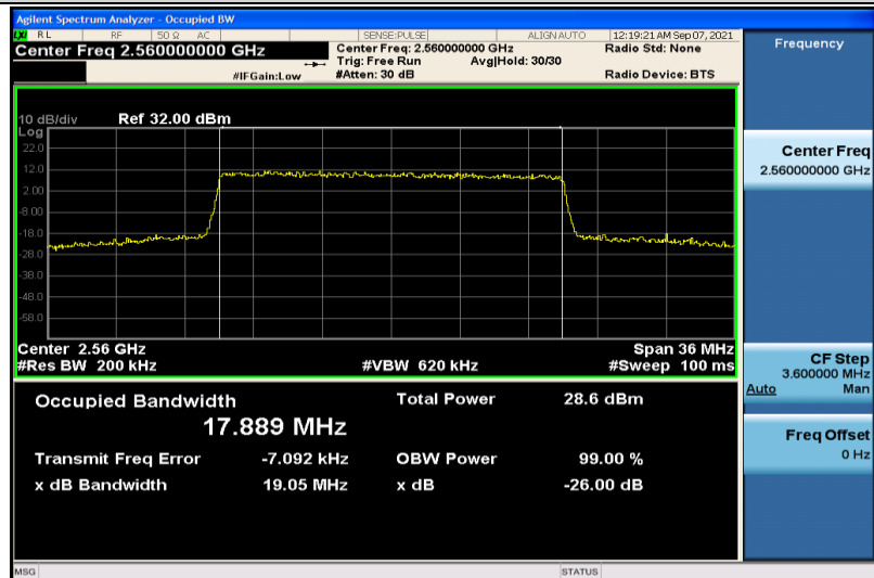
Band7-20MHz-16QAM-21350-100RB#0-17.889
