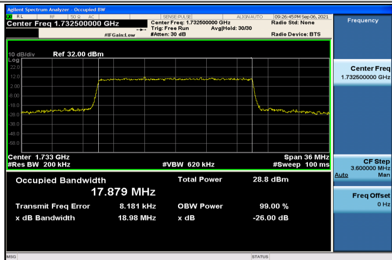
Band4-20MHz-16QAM-20175-100RB#0-17.879
