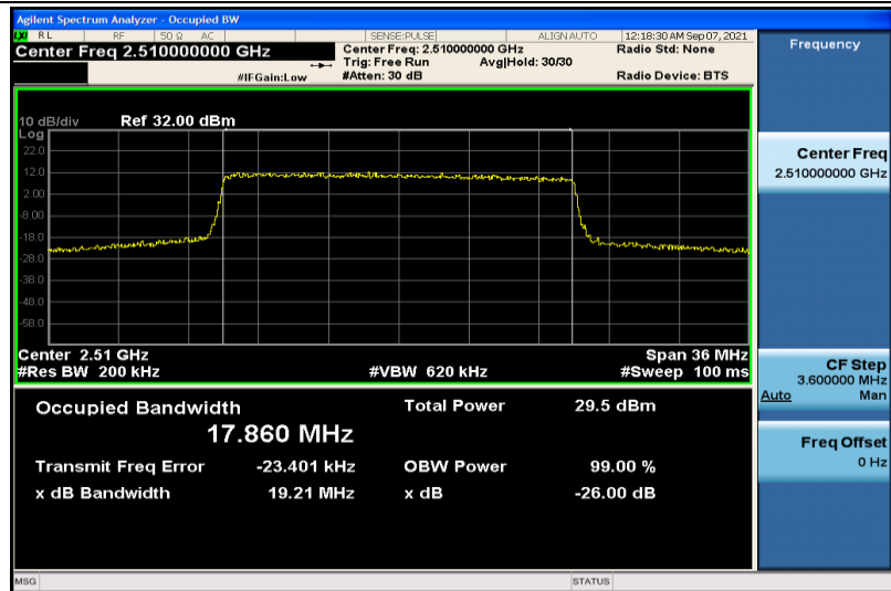
Band7-20MHz-QPSK-20850-100RB#0-17.860
