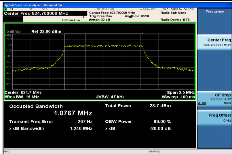
Band5-1.4MHz-QPSK-20407-6RB#0-1.0767
