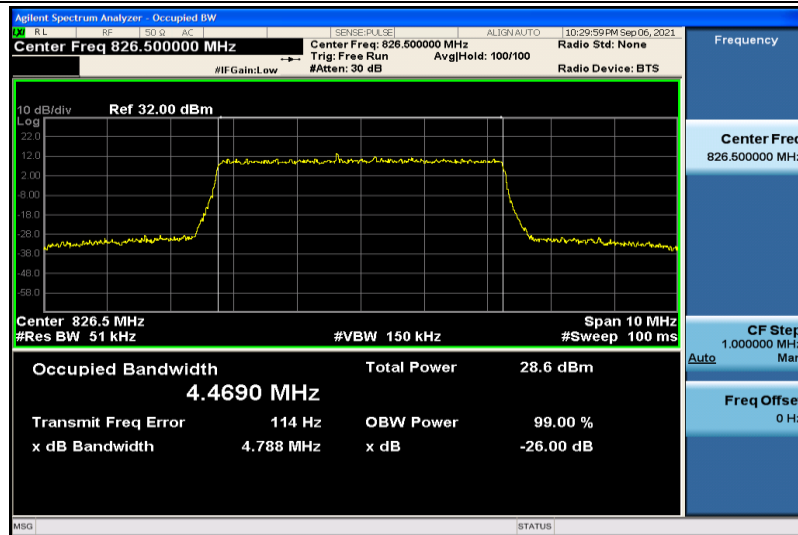
Band5-5MHz-16QAM-20425-25RB#0-4.4690
