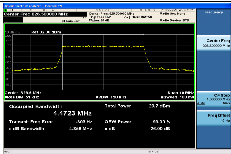
Band5-5MHz-QPSK-20425-25RB#0-4.4723
