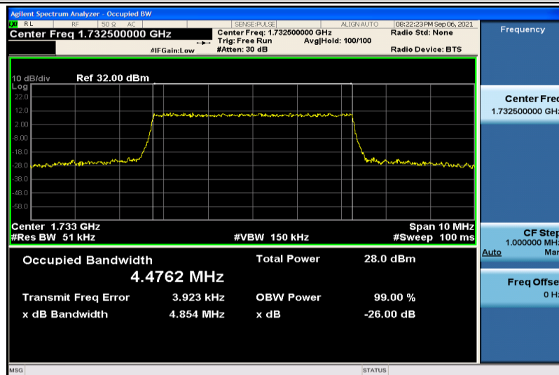
Band4-5MHz-16QAM-20175-25RB#0-4.4762
