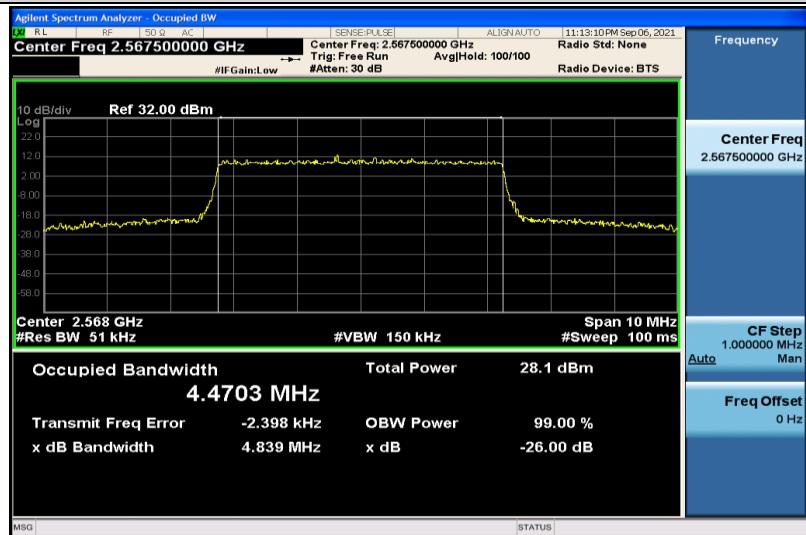
Band7-5MHz-16QAM-21425-25RB#0-4.4703
