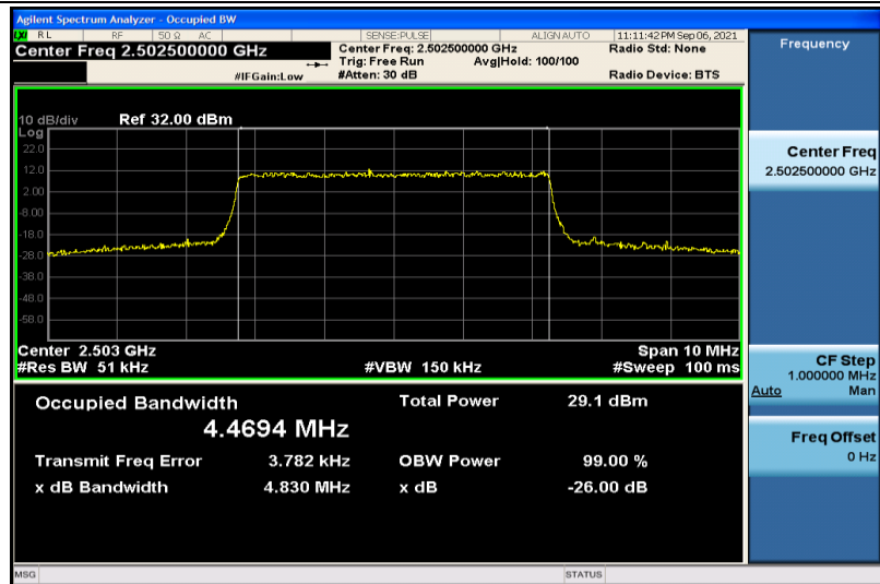
Band7-5MHz-QPSK-20775-25RB#0-4.4694
