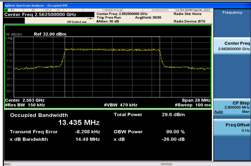
Band7-15MHz-QPSK-21375-75RB#0-13.435
