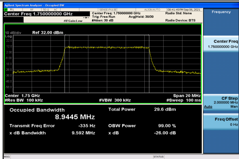
Band4-10MHz-QPSK-20350-50RB#0-8.9445
