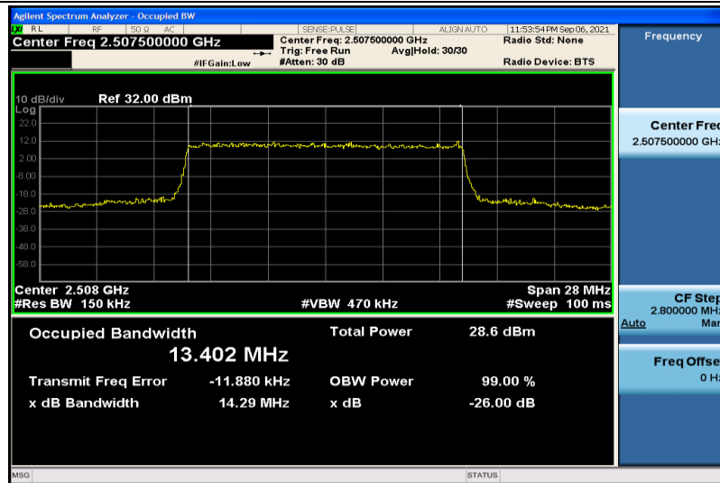
Band7-15MHz-16QAM-20825-75RB#0-13.402
