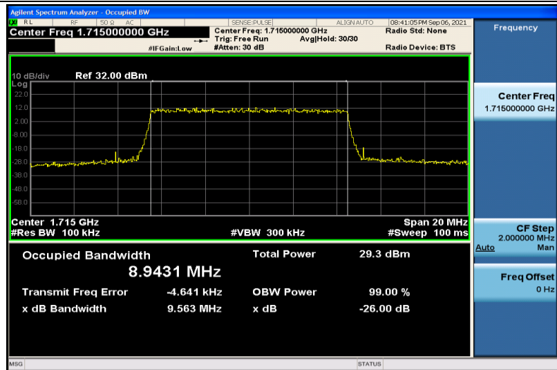
Band4-10MHz-QPSK-20000-50RB#0-8.9431
