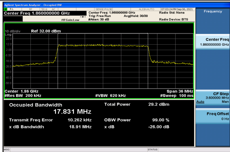
Band2-20MHz-16QAM-18700-100RB#0-17.831
