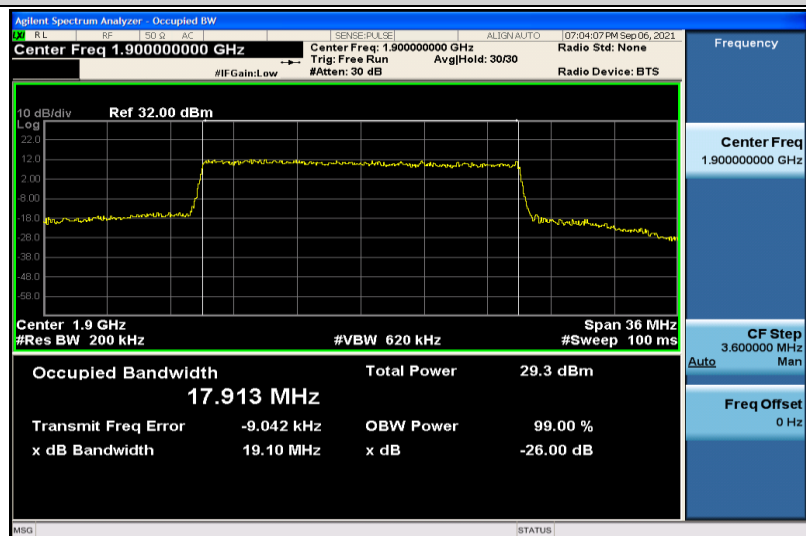
Band2-20MHz-16QAM-19100-100RB#0-17.913
