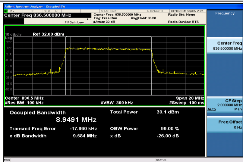
Band5-10MHz-QPSK-20525-50RB#0-8.9491
