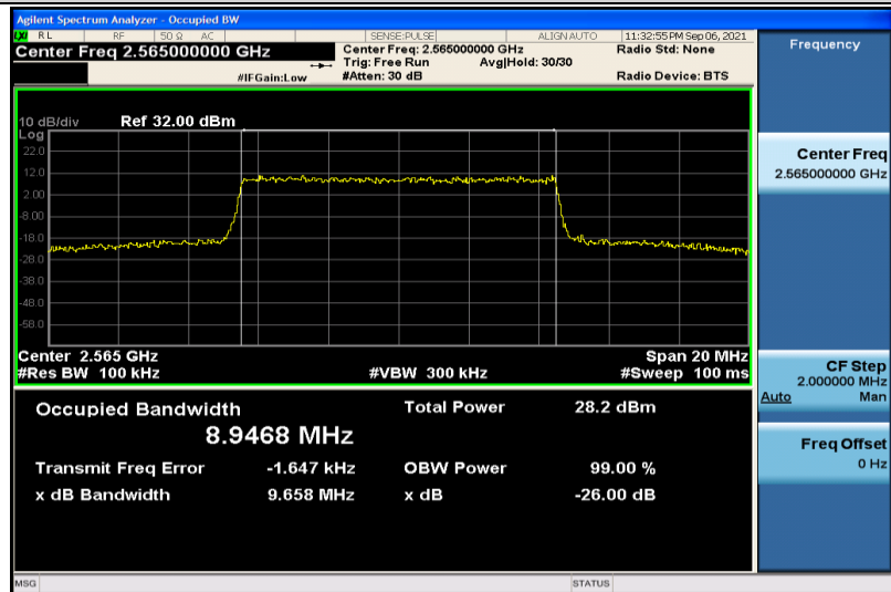
Band7-10MHz-16QAM-21400-50RB#0-8.9468
