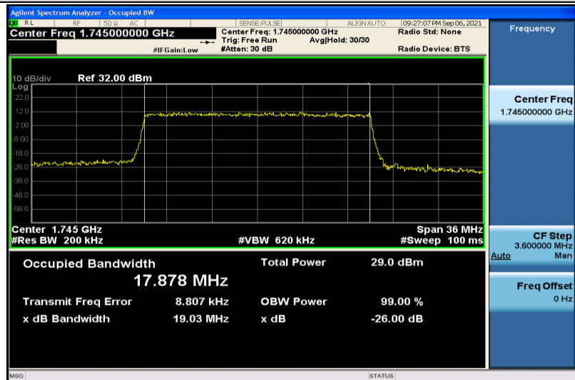
Band4-20MHz-16QAM-20300-100RB#0-17.878
