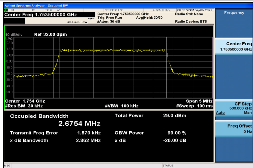
Band4-3MHz-QPSK-20385-15RB#0-2.6754
