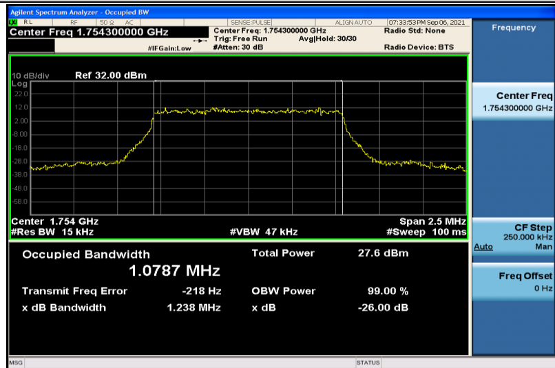
Band4-1.4MHz-16QAM-20393-6RB#0-1.0787
