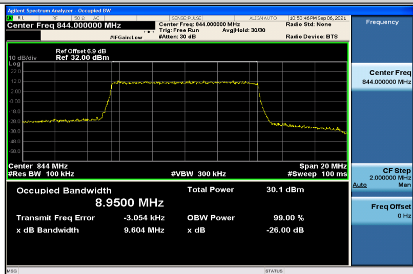
Band5-10MHz-QPSK-20600-50RB#0-8.9500
