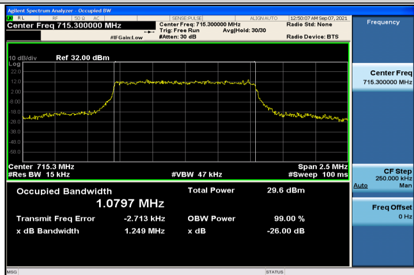
Band12-1.4MHz-QPSK-23173-6RB#0-1.0797
