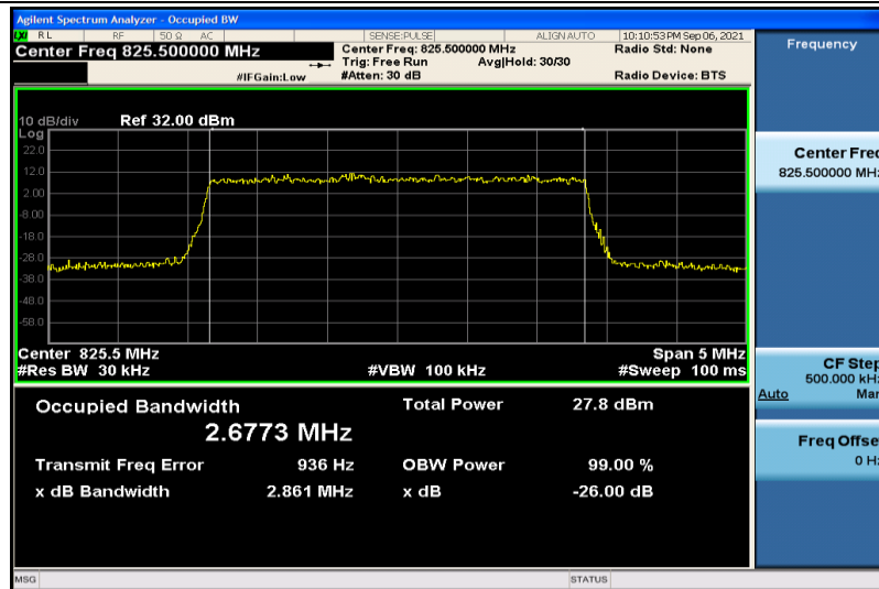
Band5-3MHz-16QAM-20415-15RB#0-2.6773
