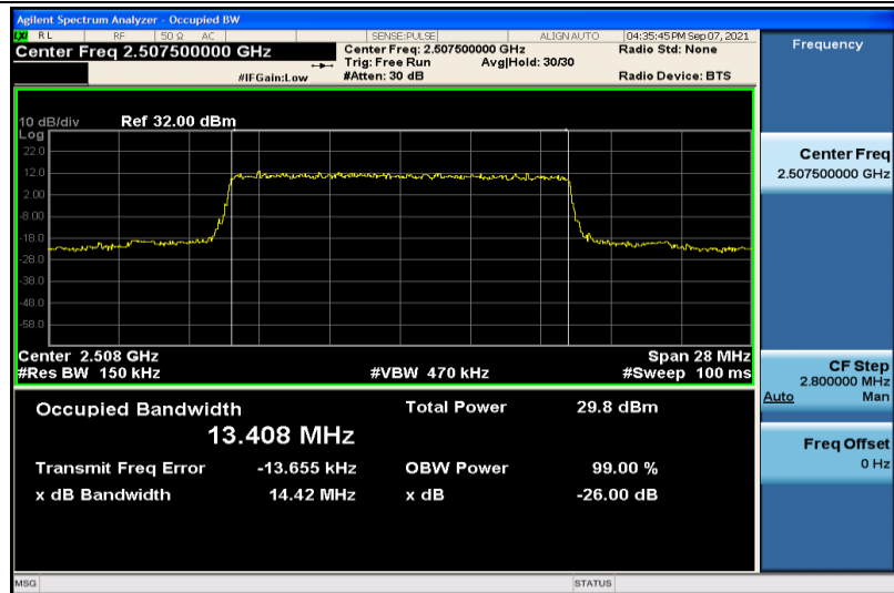
Band7-15MHz-QPSK-20825-75RB#0-13.408
