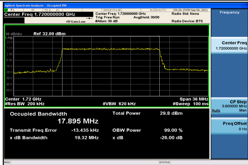
Band4-20MHz-QPSK-20050-100RB#0-17.895
