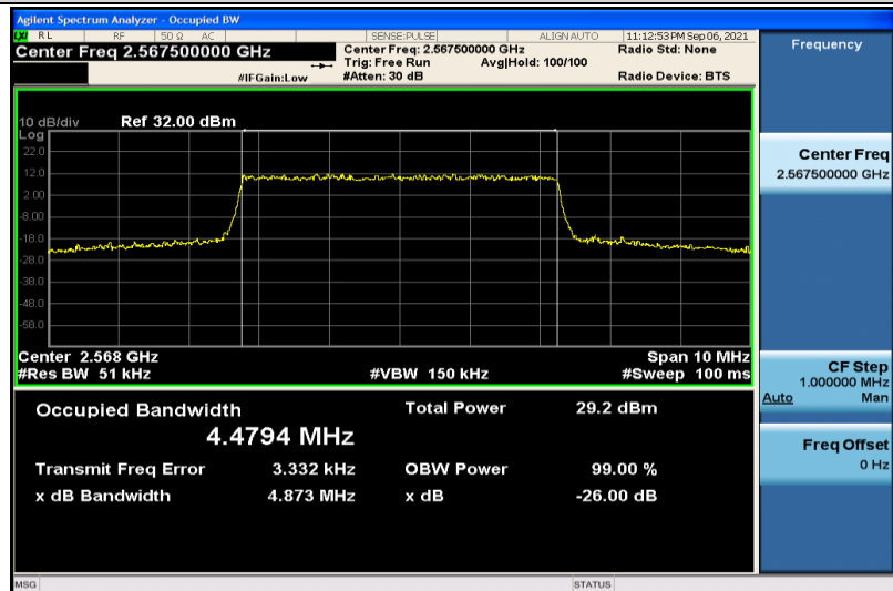
Band7-5MHz-QPSK-21425-25RB#0-4.4794
