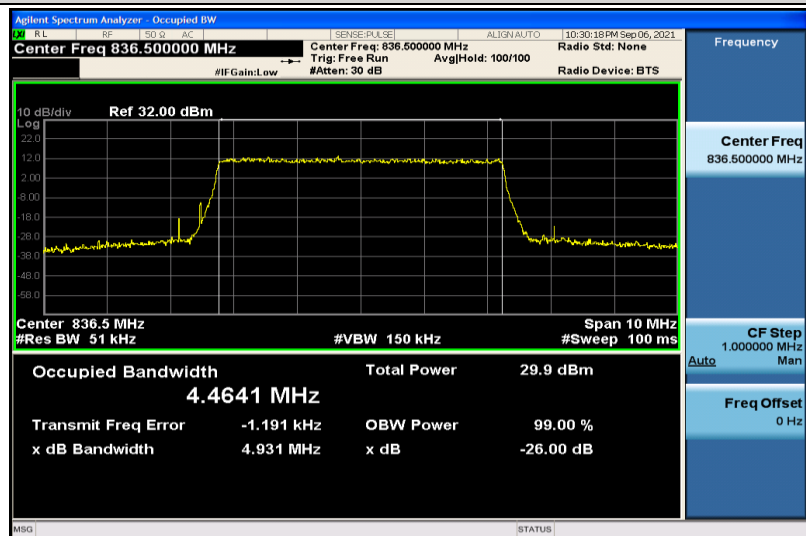
Band5-5MHz-QPSK-20525-25RB#0-4.4641
