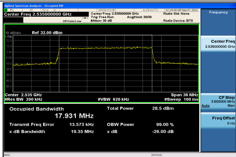
Band7-20MHz-16QAM-21100-100RB#0-17.931
