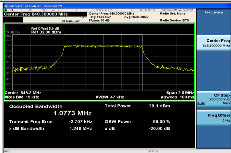
Band5-1.4MHz-QPSK-20643-6RB#0-1.0773
