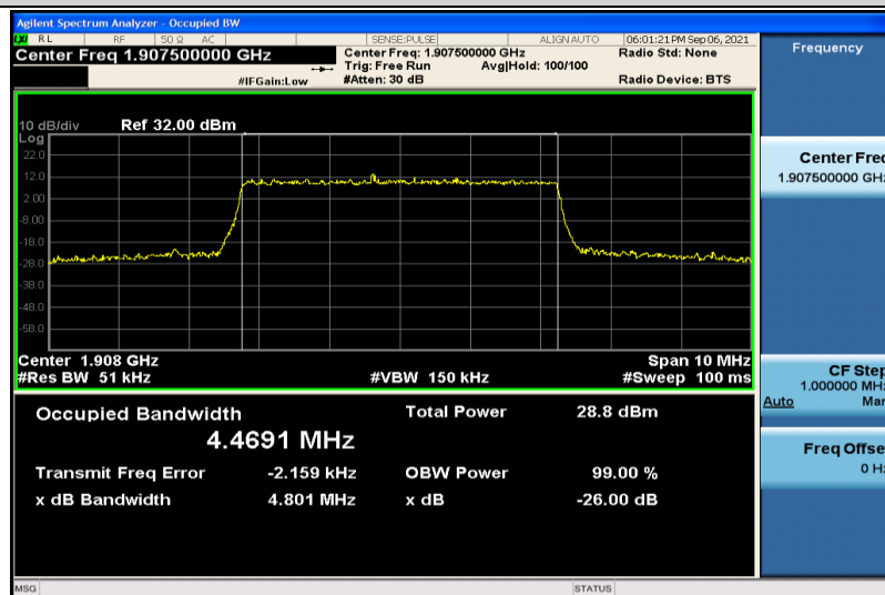
Band2-5MHz-16QAM-19175-25RB#0-4.4691
