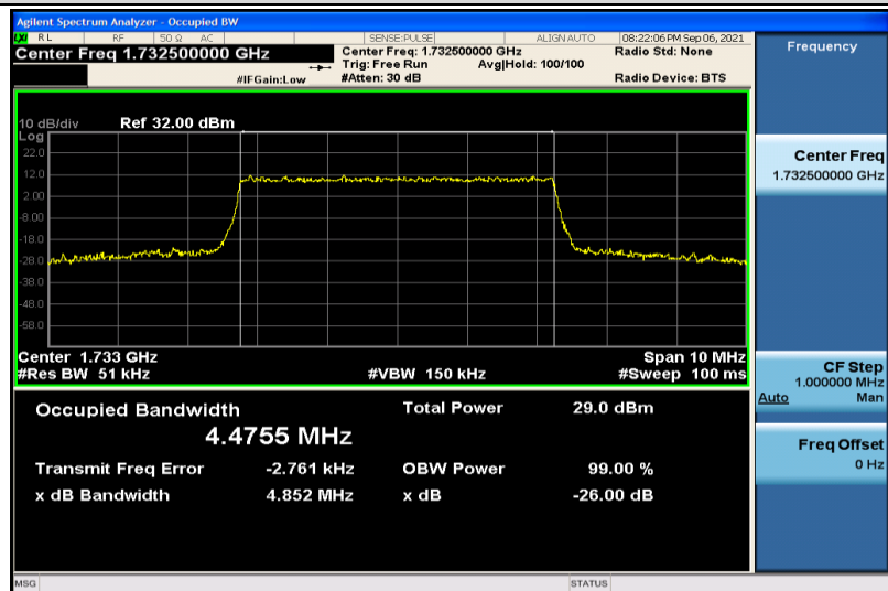
Band4-5MHz-QPSK-20175-25RB#0-4.4755
