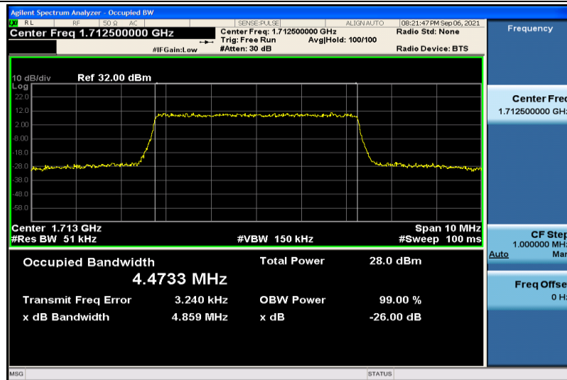
Band4-5MHz-16QAM-19975-25RB#0-4.4733
