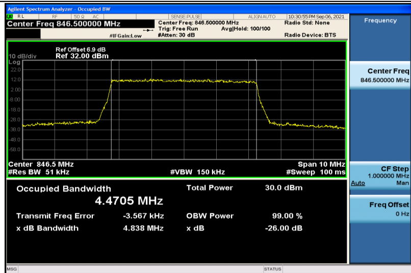
Band5-5MHz-QPSK-20625-25RB#0-4.4705
