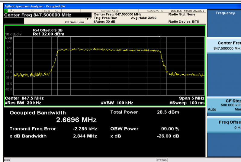
Band5-3MHz-16QAM-20635-15RB#0-2.6696
