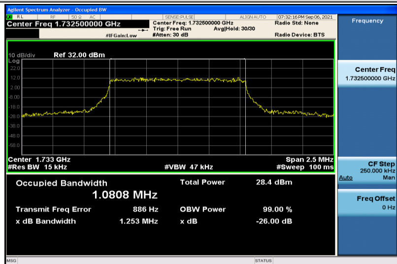
Band4-1.4MHz-QPSK-20175-6RB#0-1.0808
