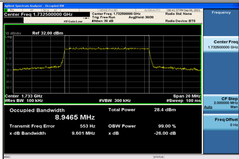
Band4-10MHz-16QAM-20175-50RB#0-8.9465
