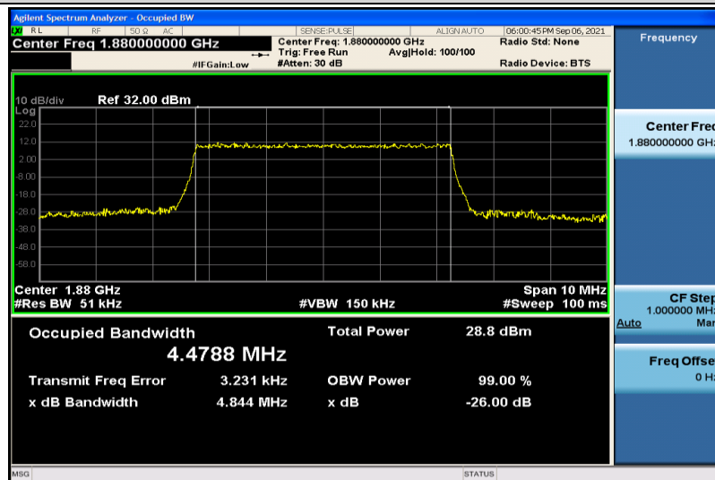
Band2-5MHz-16QAM-18900-25RB#0-4.4788
