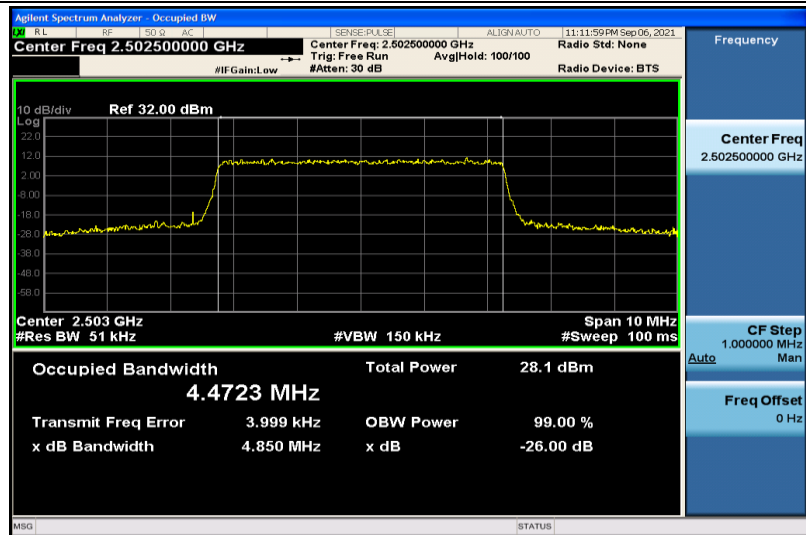
Band7-5MHz-16QAM-20775-25RB#0-4.4723
