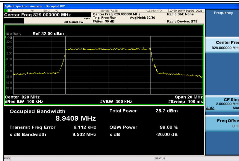
Band5-10MHz-16QAM-20450-50RB#0-8.9409
