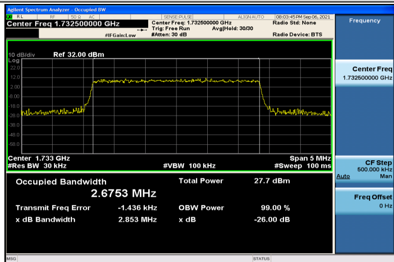
Band4-3MHz-16QAM-20175-15RB#0-2.6753
