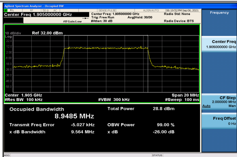
Band2-10MHz-16QAM-19150-50RB#0-8.9485
