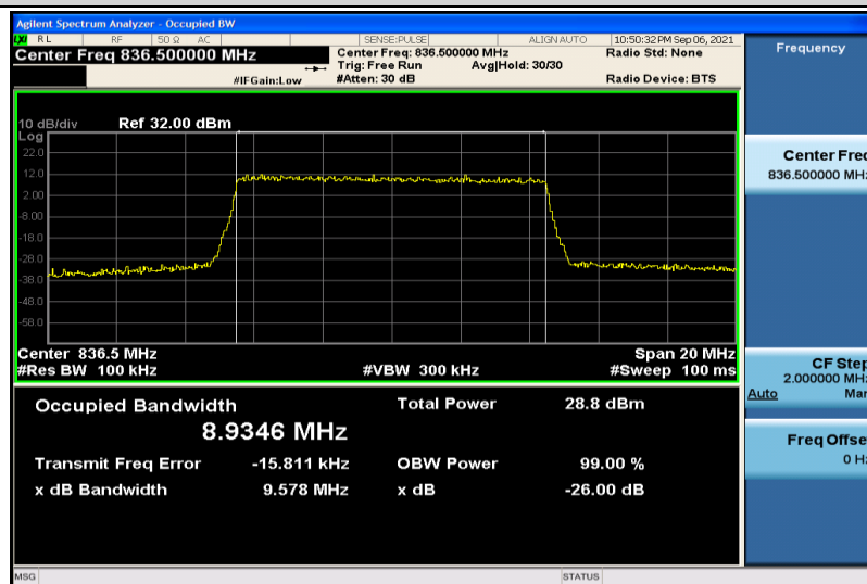
Band5-10MHz-16QAM-20525-50RB#0-8.9346
