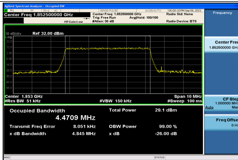
Band2-5MHz-16QAM-18625-25RB#0-4.4709
