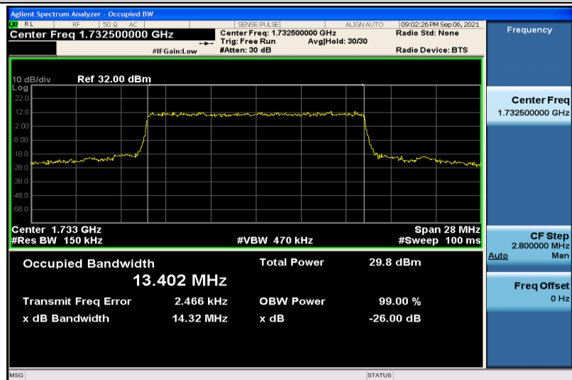
Band4-15MHz-QPSK-20175-75RB#0-13.402
