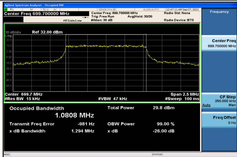
Band12-1.4MHz-QPSK-23017-6RB#0-1.0808
