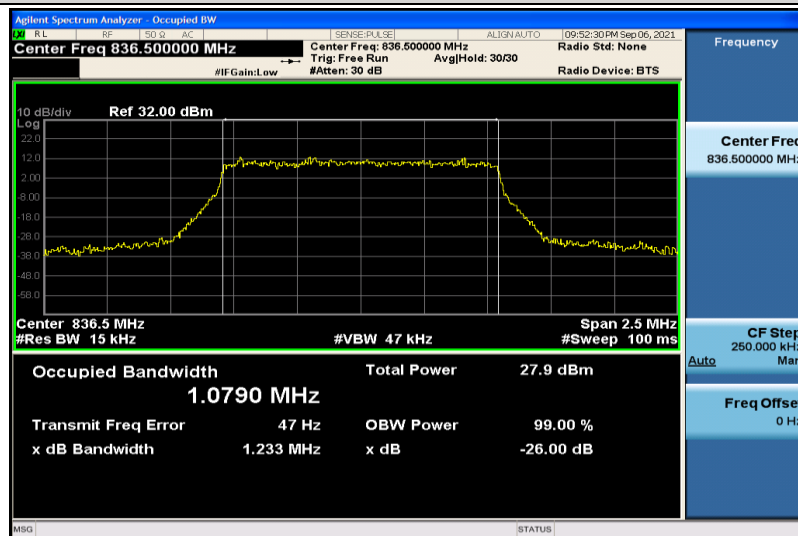
Band5-1.4MHz-16QAM-20525-6RB#0-1.0790
