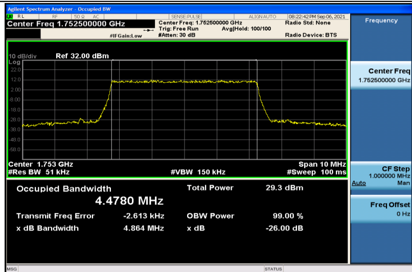
Band4-5MHz-QPSK-20375-25RB#0-4.4780
