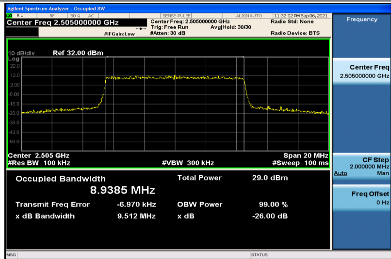
Band7-10MHz-QPSK-20800-50RB#0-8.9385
