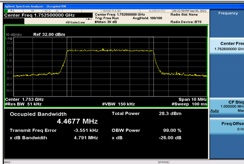
Band4-5MHz-16QAM-20375-25RB#0-4.4677
