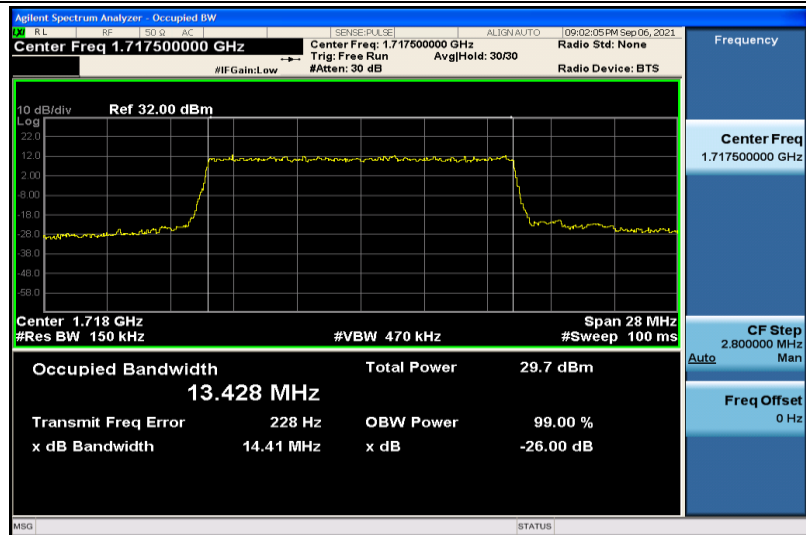
Band4-15MHz-QPSK-20025-75RB#0-13.428
