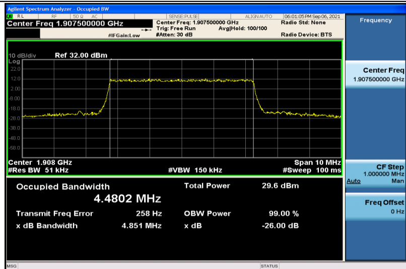
Band2-5MHz-QPSK-19175-25RB#0-4.4802
