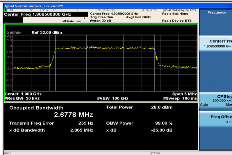
Band2-3MHz-16QAM-19185-15RB#0-2.6778
