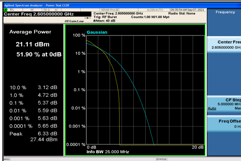
Band41-5MHz-QPSK-40740-1RB#0
