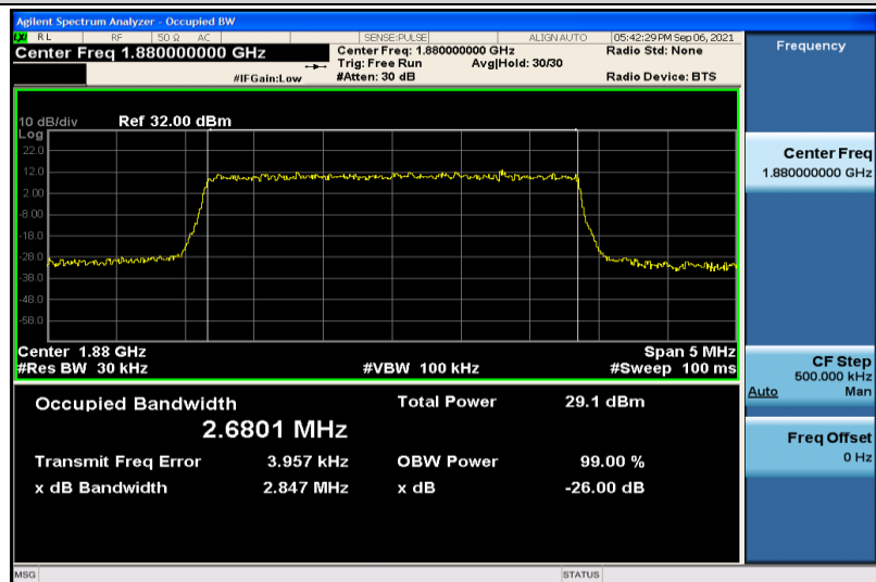
Band2-3MHz-QPSK-18900-15RB#0-2.6801
