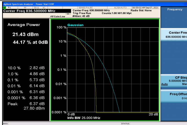
Band26-10MHz-16QAM-26915-1RB#0
