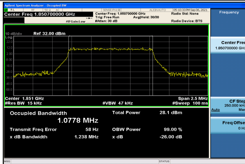
Band2-1.4MHz-16QAM-18607-6RB#0-1.0778
