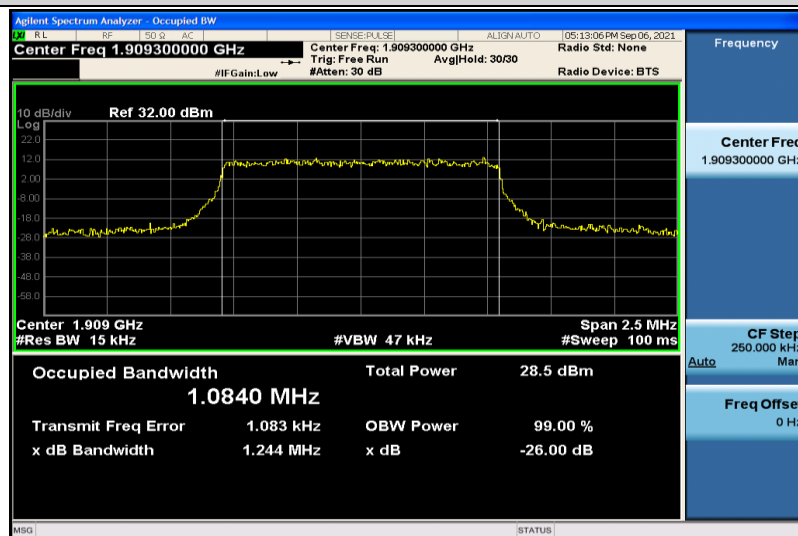
Band2-1.4MHz-QPSK-19193-6RB#0-1.0840
