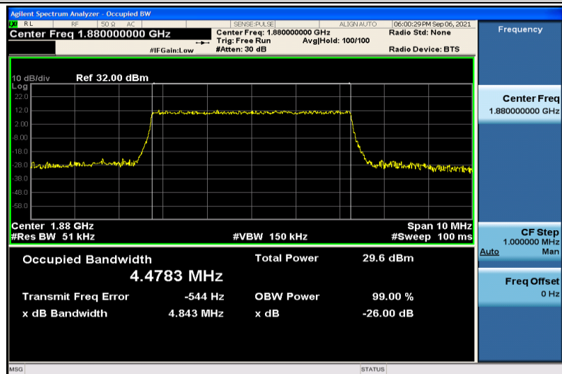
Band2-5MHz-QPSK-18900-25RB#0-4.4783
