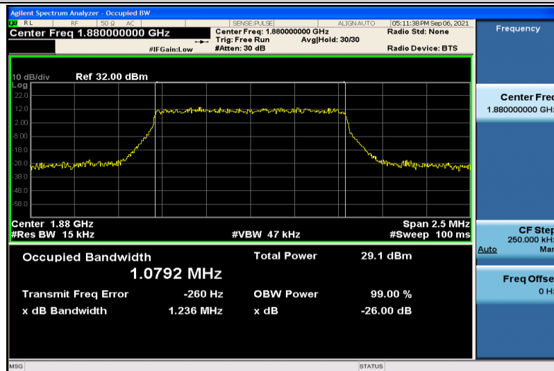
Band2-1.4MHz-QPSK-18900-6RB#0-1.0792
