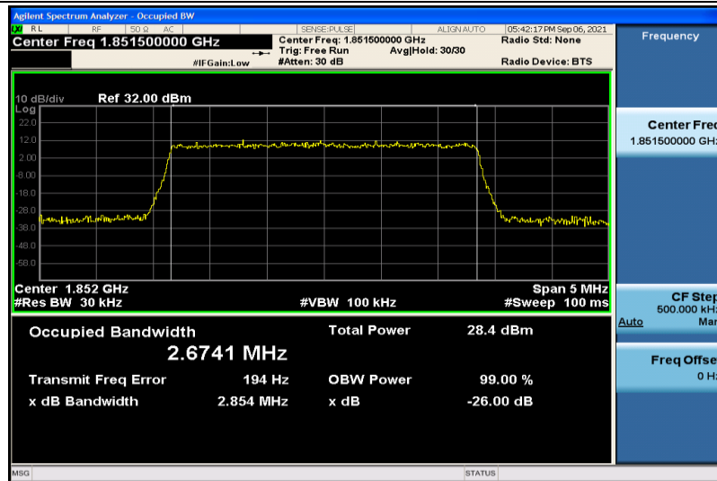
Band2-3MHz-16QAM-18615-15RB#0-2.6741
