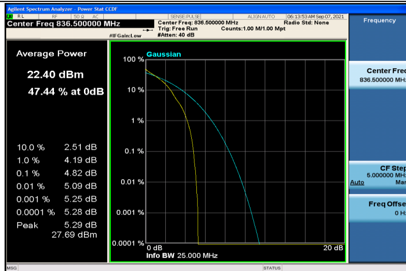
Band26-3MHz-QPSK-26915-1RB#0
