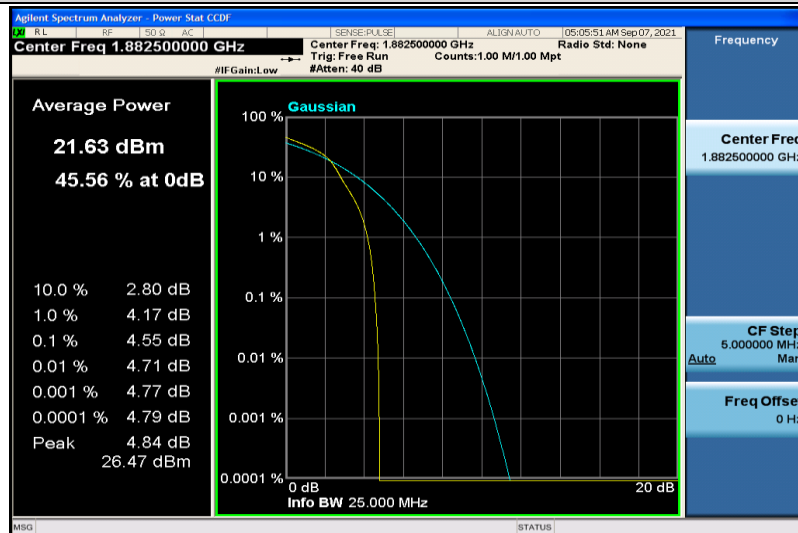
Band25-15MHz-16QAM-26365-1RB#0
