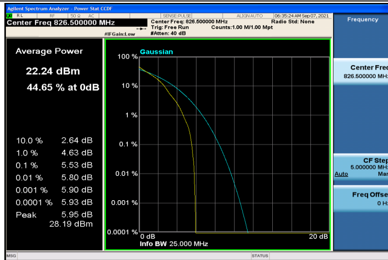
Band26-5MHz-QPSK-26815-1RB#0
