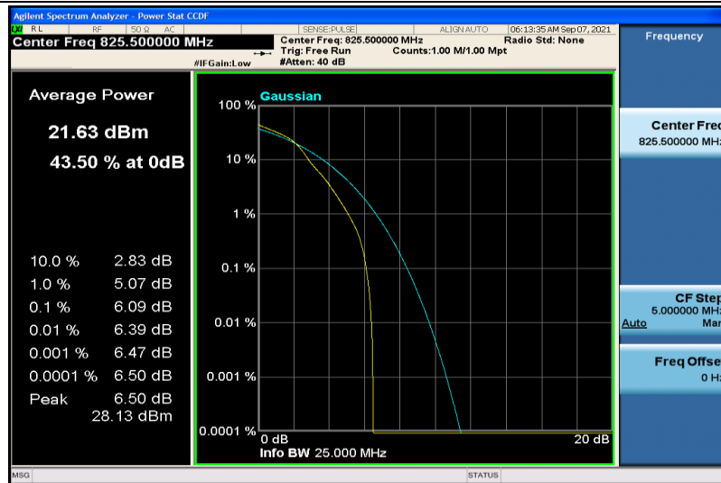
Band26-3MHz-16QAM-26805-1RB#0
