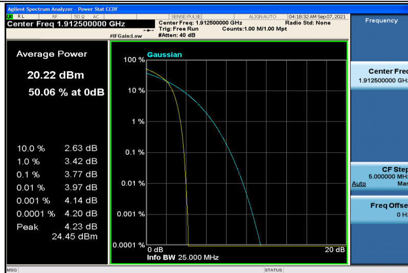
Band25-5MHz-16QAM-26665-25RB#0
