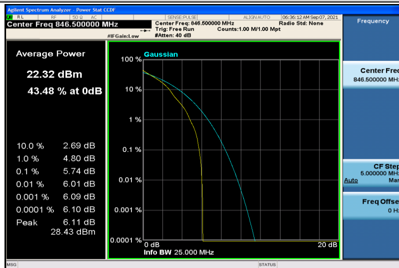
Band26-5MHz-QPSK-27015-1RB#0
