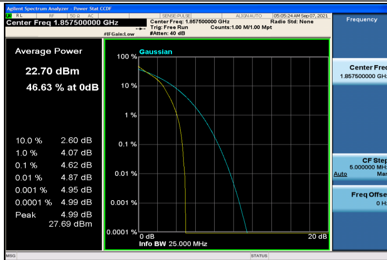
Band25-15MHz-QPSK-26115-1RB#0
