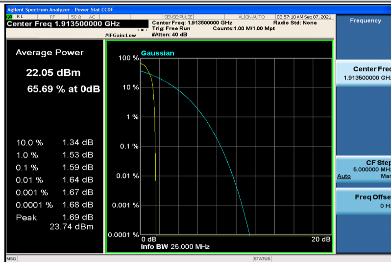
Band25-3MHz-QPSK-26675-1RB#0
