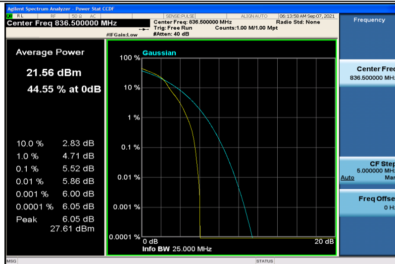
Band26-3MHz-16QAM-26915-1RB#0
