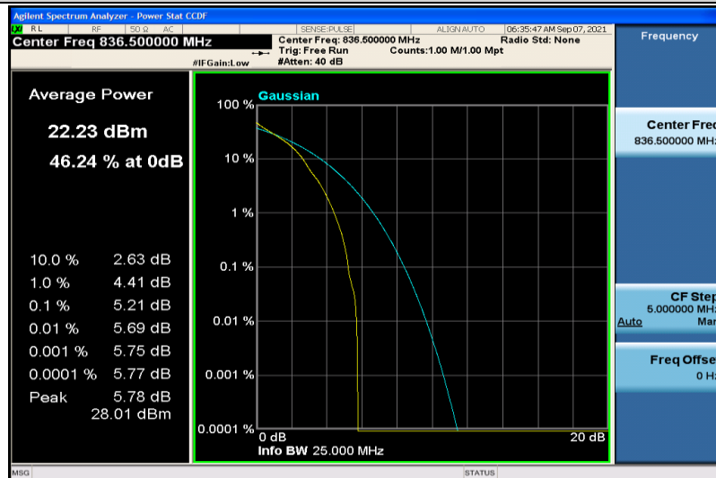
Band26-5MHz-QPSK-26915-1RB#0
