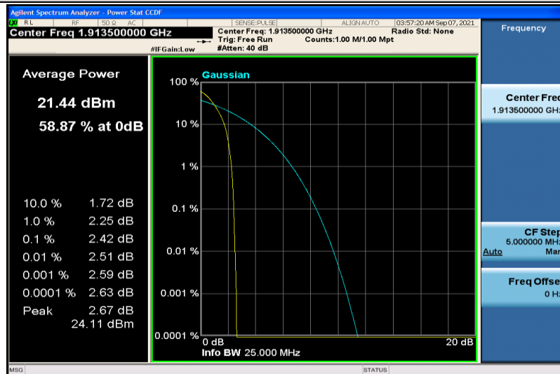
Band25-3MHz-QPSK-26675-15RB#0
