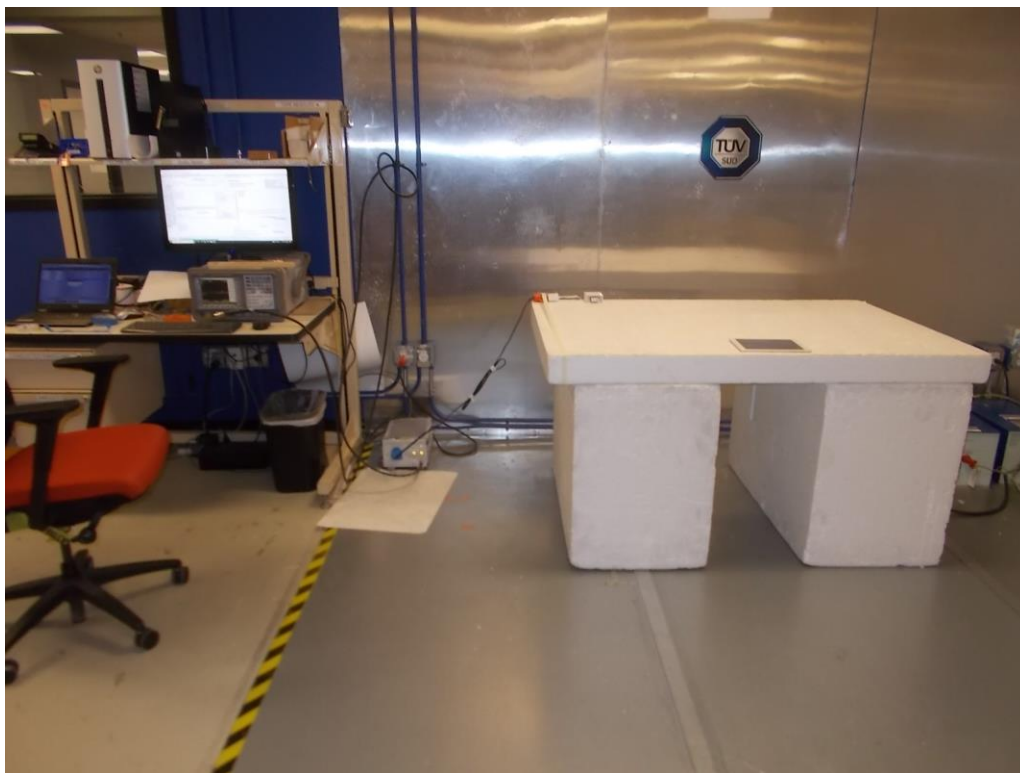
Figure A-8: Test Setup – Conducted AC power line emission
