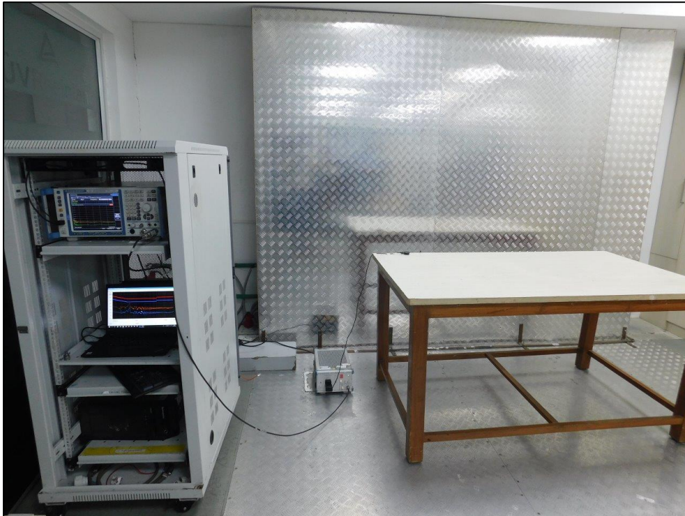
Conducted AC power lines setup photo
