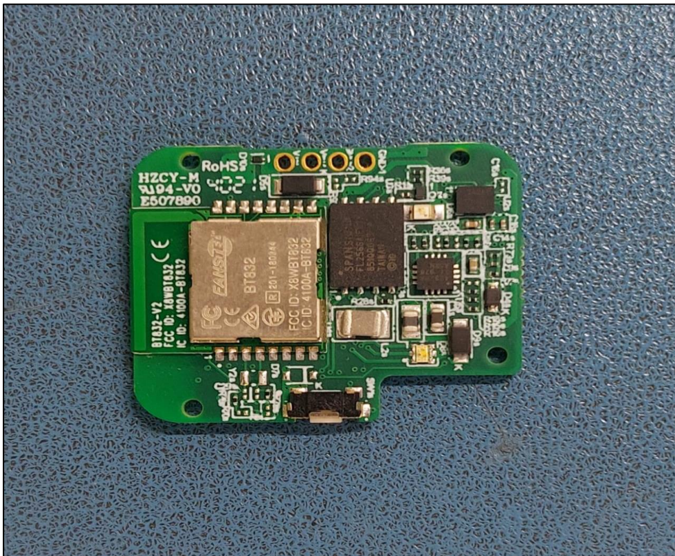
Figure 2: Front view of the PCB
