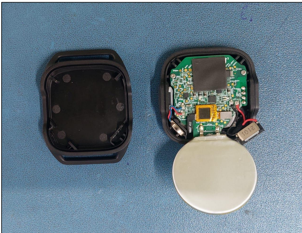
Figure 1: EUT Front panel removed
