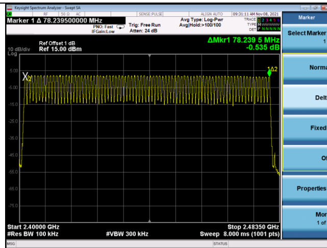
GFSK Modulation
