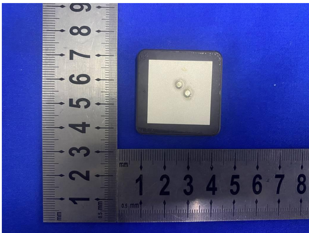
Photo 2: Antenna
