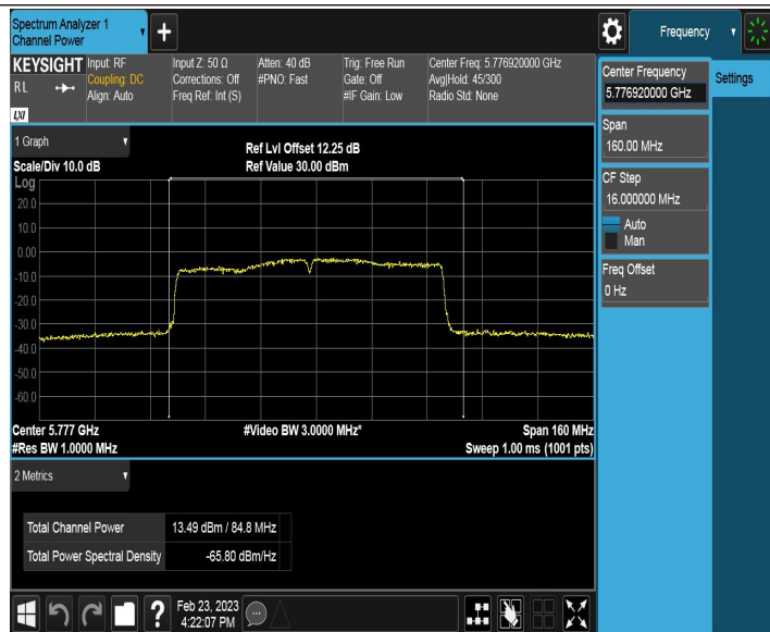
11AC80CDD_Ant2_5775
