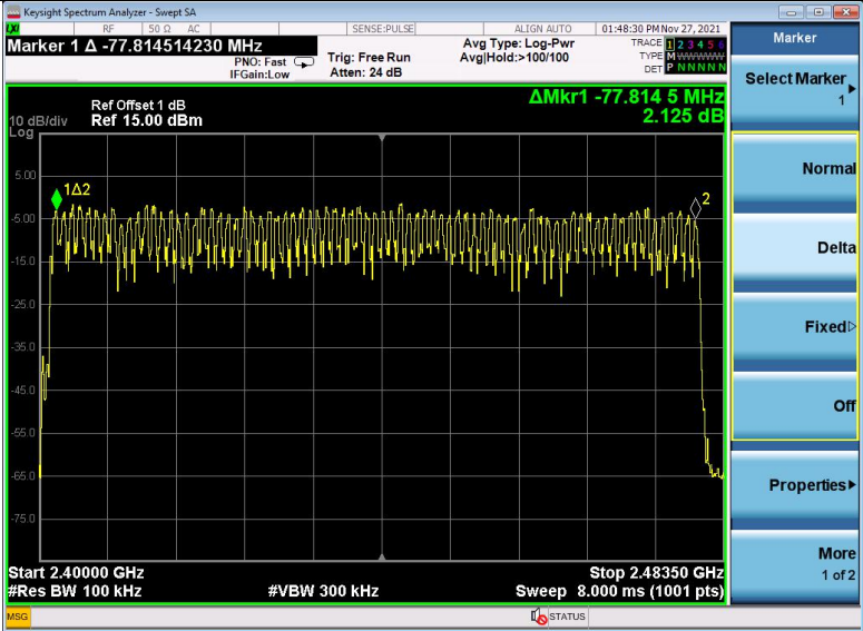
8DPSK Modulation
