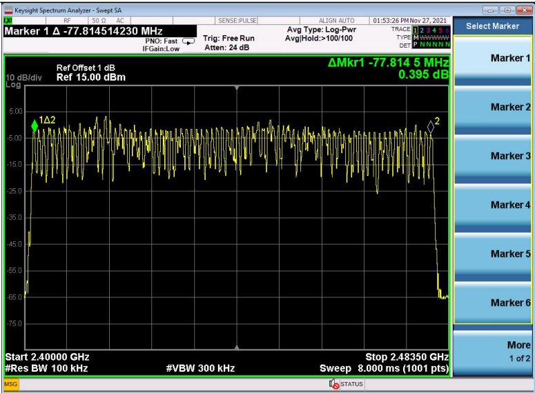
GFSK Modulation
