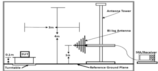
Below 1GHz
