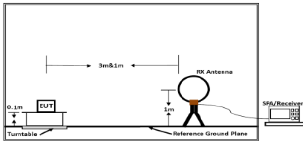
Below 30MHz
