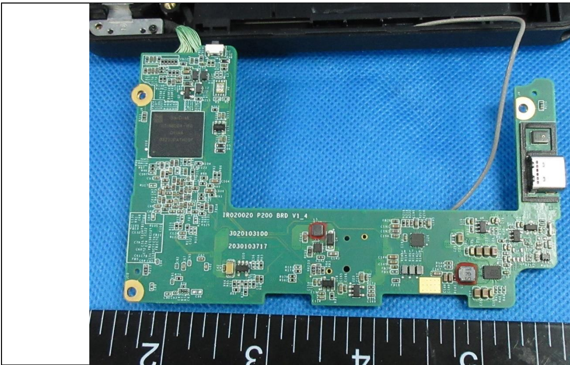
Details of: Internal view 4 of main unit
