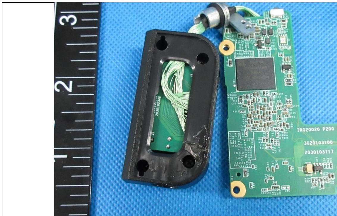
Details of: Internal view 7 of main unit
