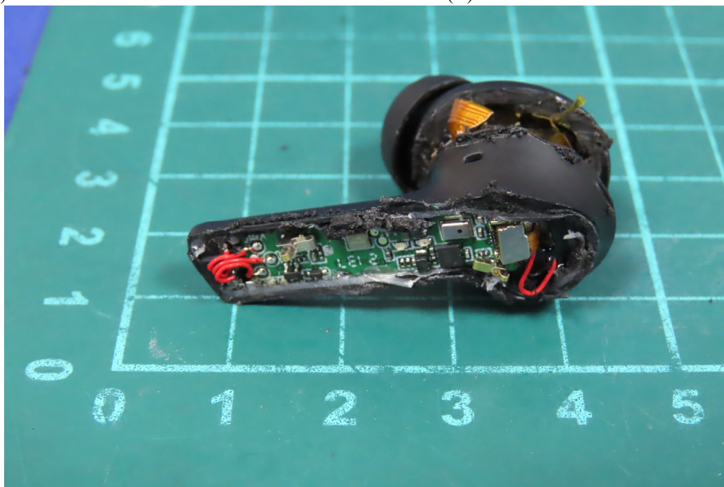
(11) EUT Photo - M/N: ROG CETRA TRUE WIRELESS(R)
