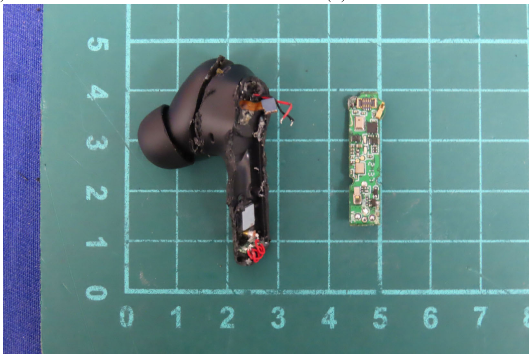
(12) EUT Photo - M/N: ROG CETRA TRUE WIRELESS(R)
