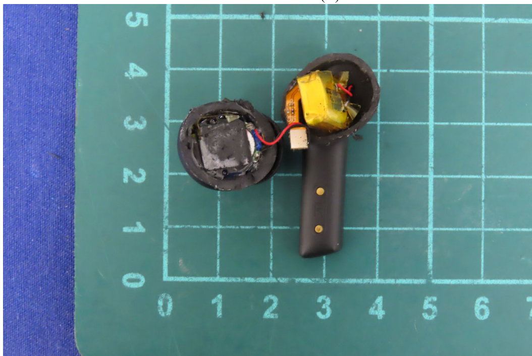
(7) EUT Photo - M/N: ROG CETRA TRUE WIRELESS(R)
